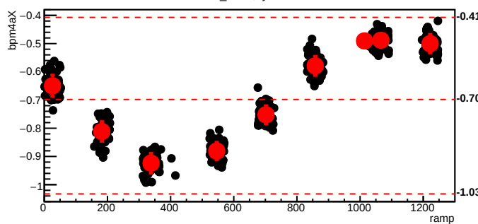
bmod_trim3,cyc=7703
