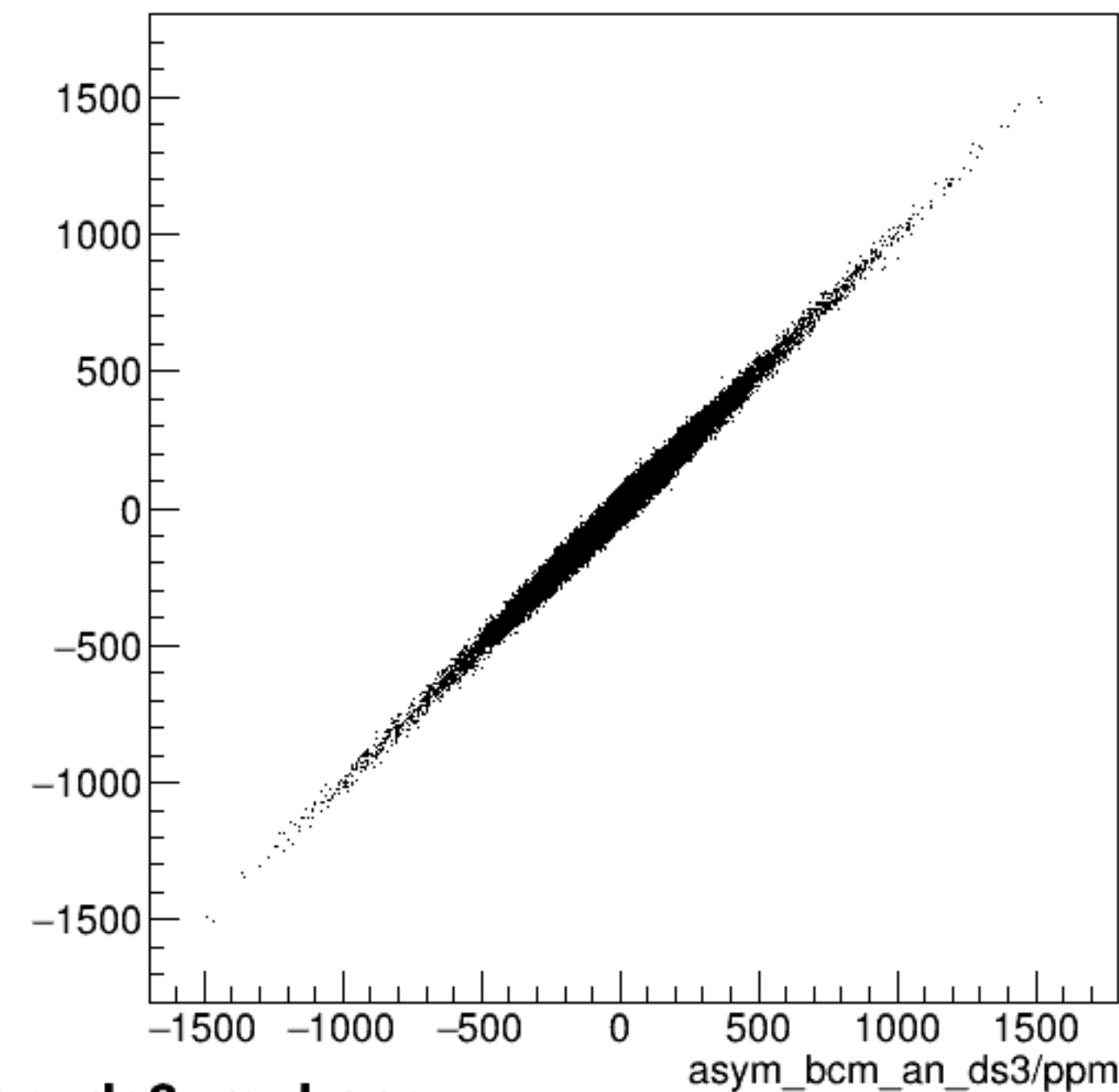
run7017_000_asym_bcm_an_us_vs_asym_bcm_an_ds3_mul.png
