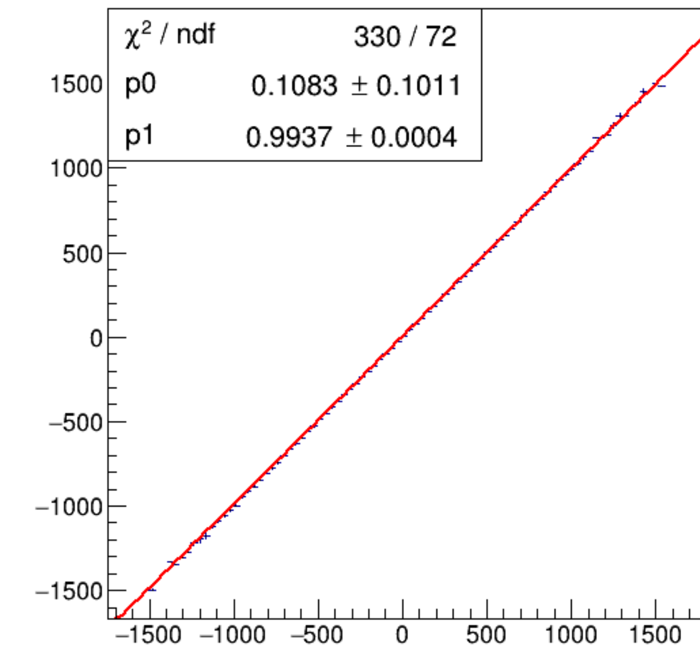
run7017_000_asym_bcm_an_us_vs_asym_bcm_an_ds3_mul.png
