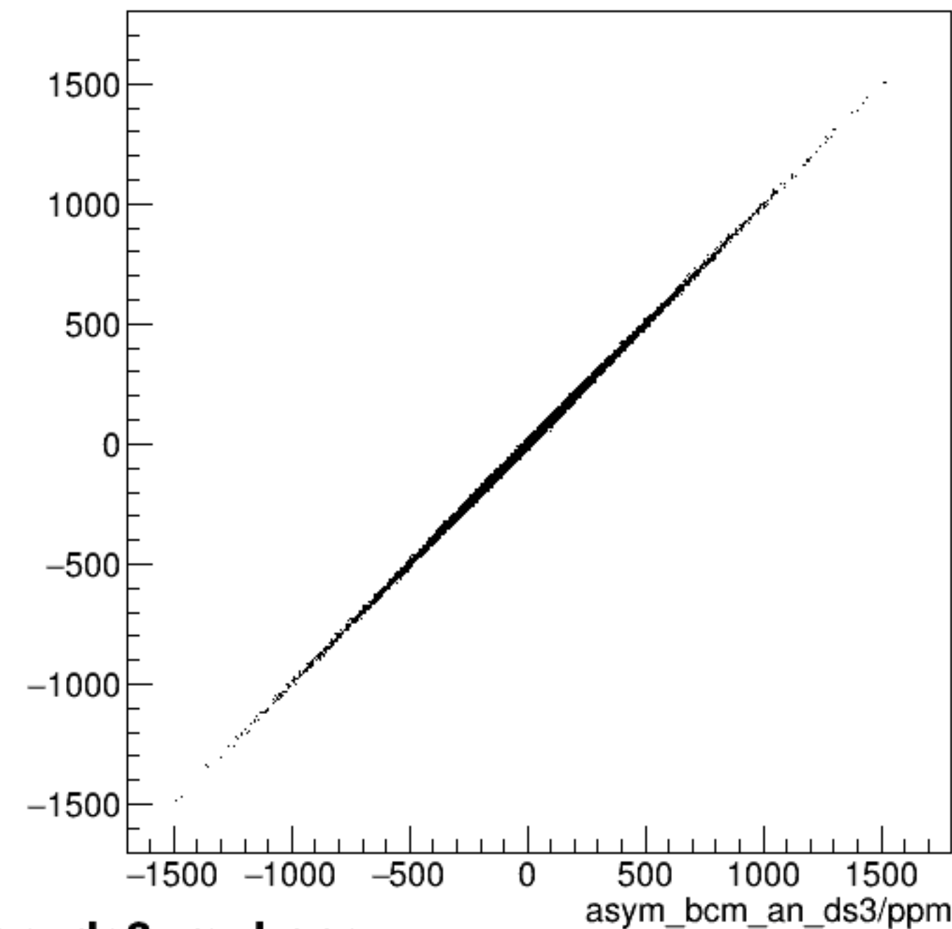
run7017_000_asym_bcm_an_ds_vs_asym_bcm_an_ds3_mul.png
