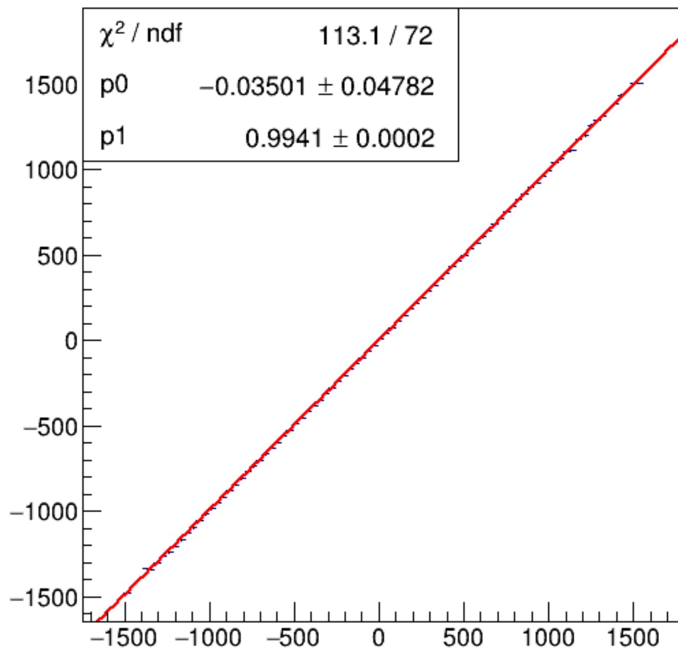
run7017_000_asym_bcm_an_ds_vs_asym_bcm_an_ds3_mul.png
