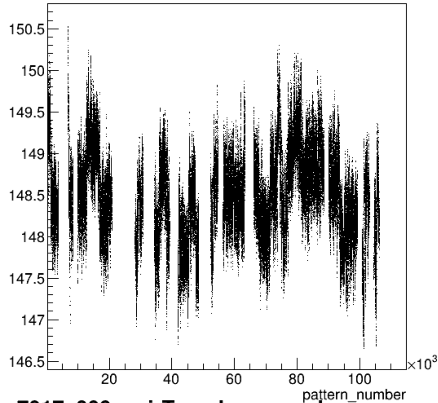
yield_bcm_an_ds:pattern_number {ErrorFlag==0}
