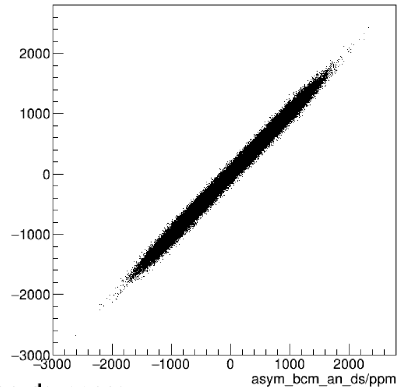
run7020_000_asym_bcm_dg_us_vs_asym_bcm_an_ds_pr.png
