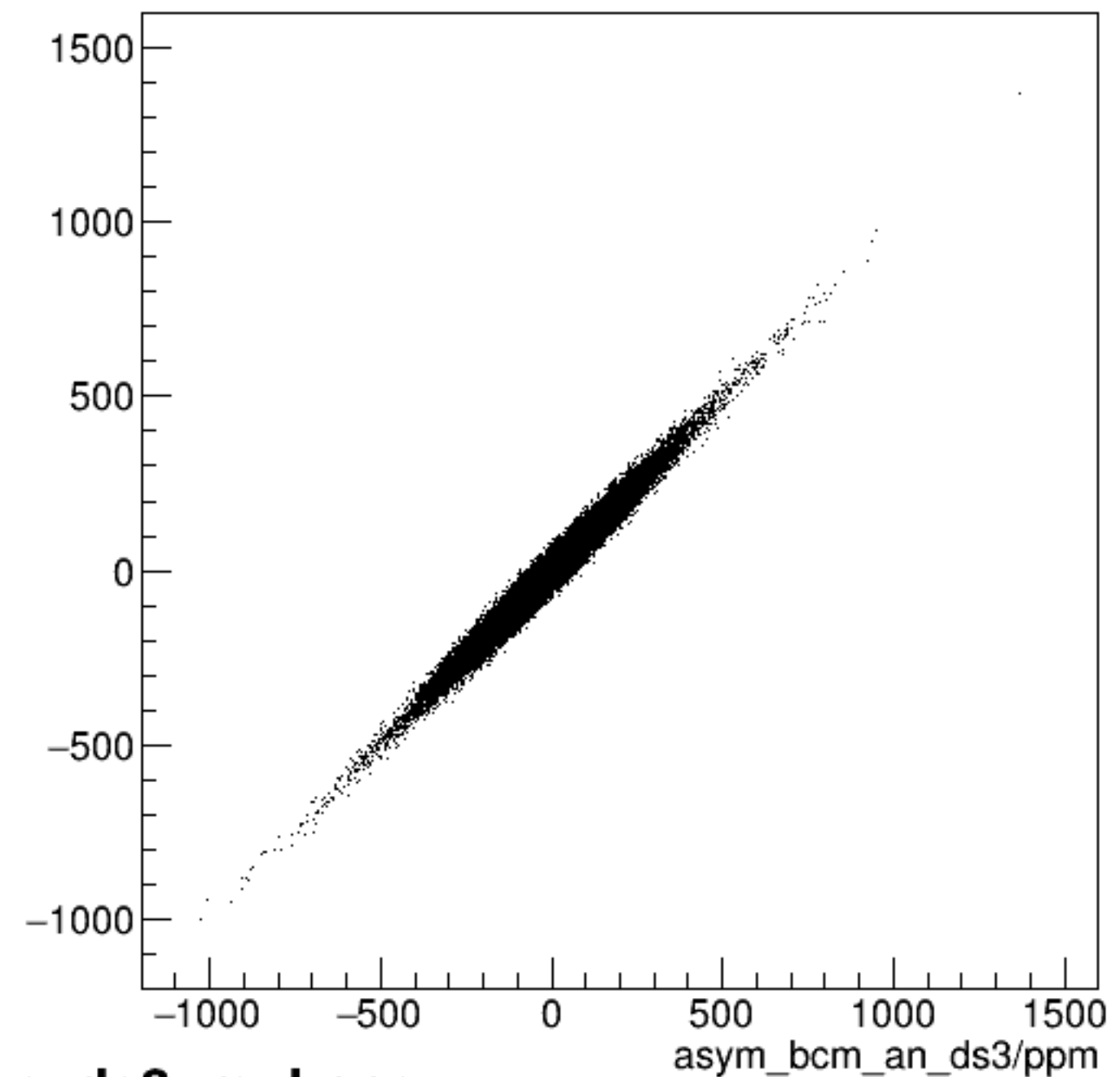
run7020_000_asym_bcm_an_us_vs_asym_bcm_an_ds3_mul.png
