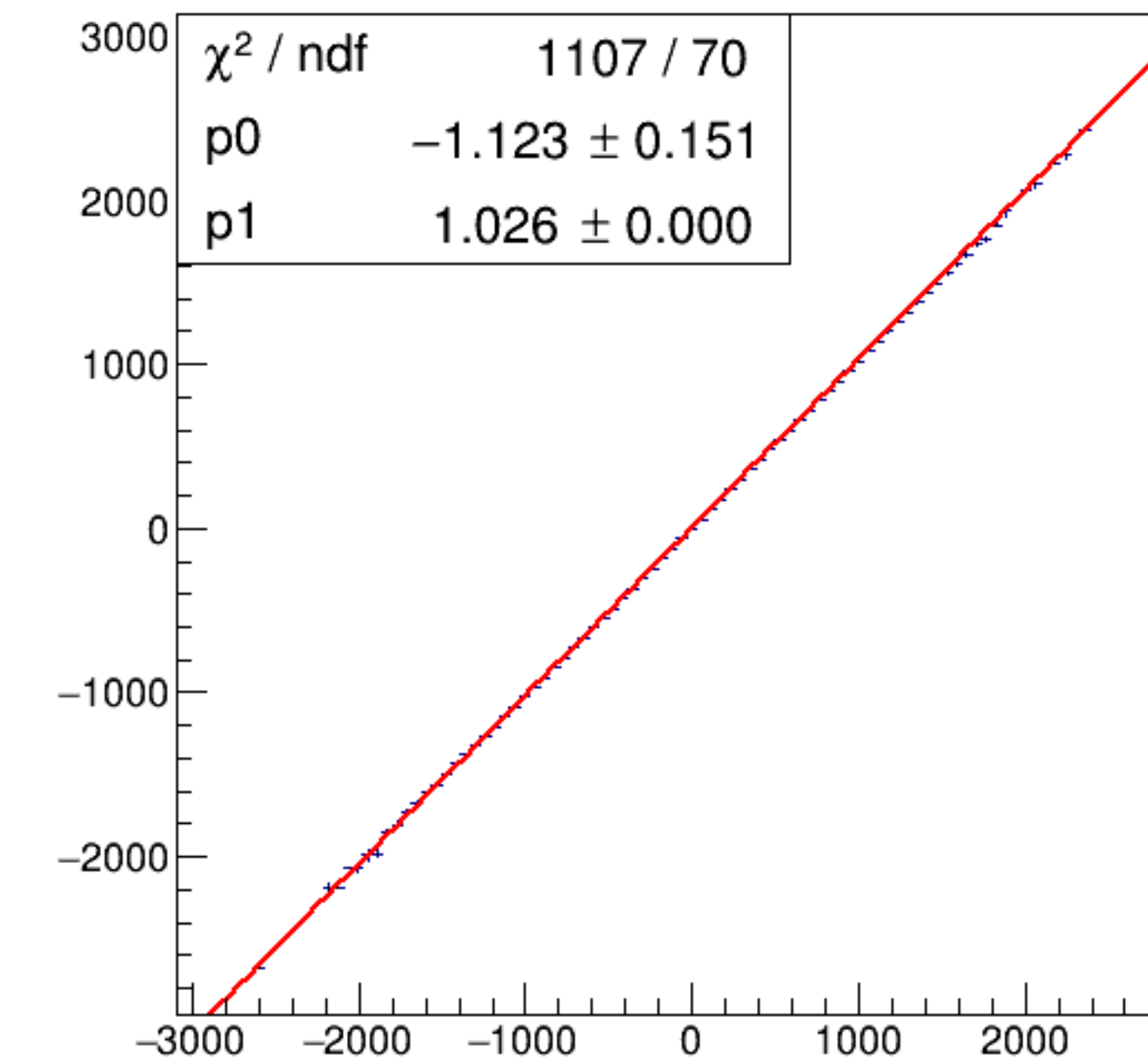
run7020_000_asym_bcm_dg_us_vs_asym_bcm_an_ds_pr.png
