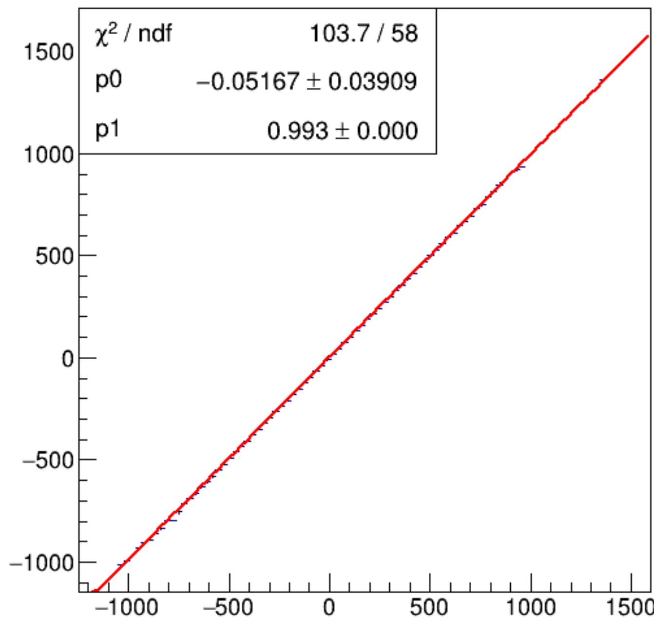
run7020_000_asym_bcm_an_ds_vs_asym_bcm_an_ds3_mul.png
