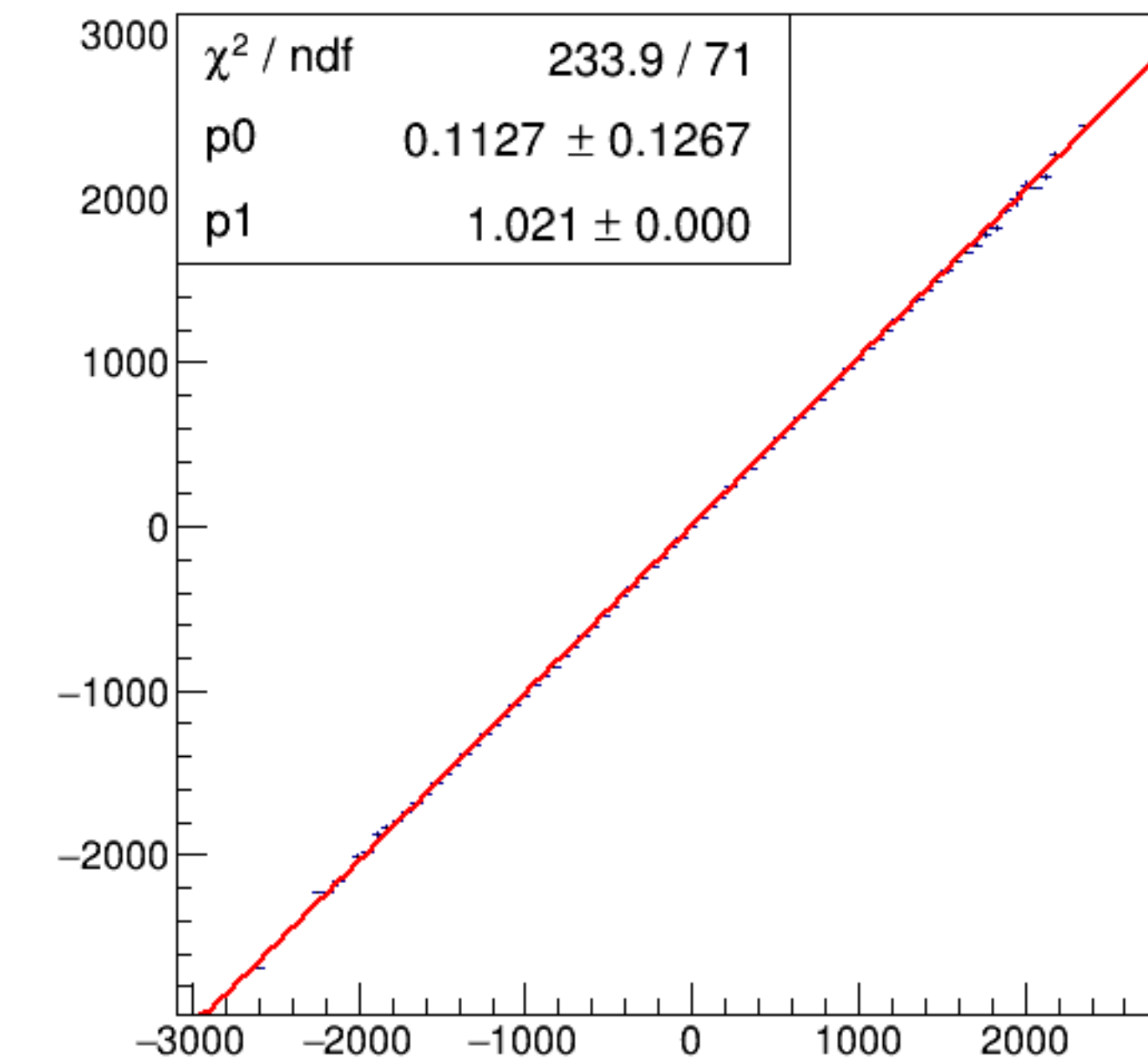
run7020_000_asym_bcm_dg_ds_vs_asym_bcm_an_us_pr.png
