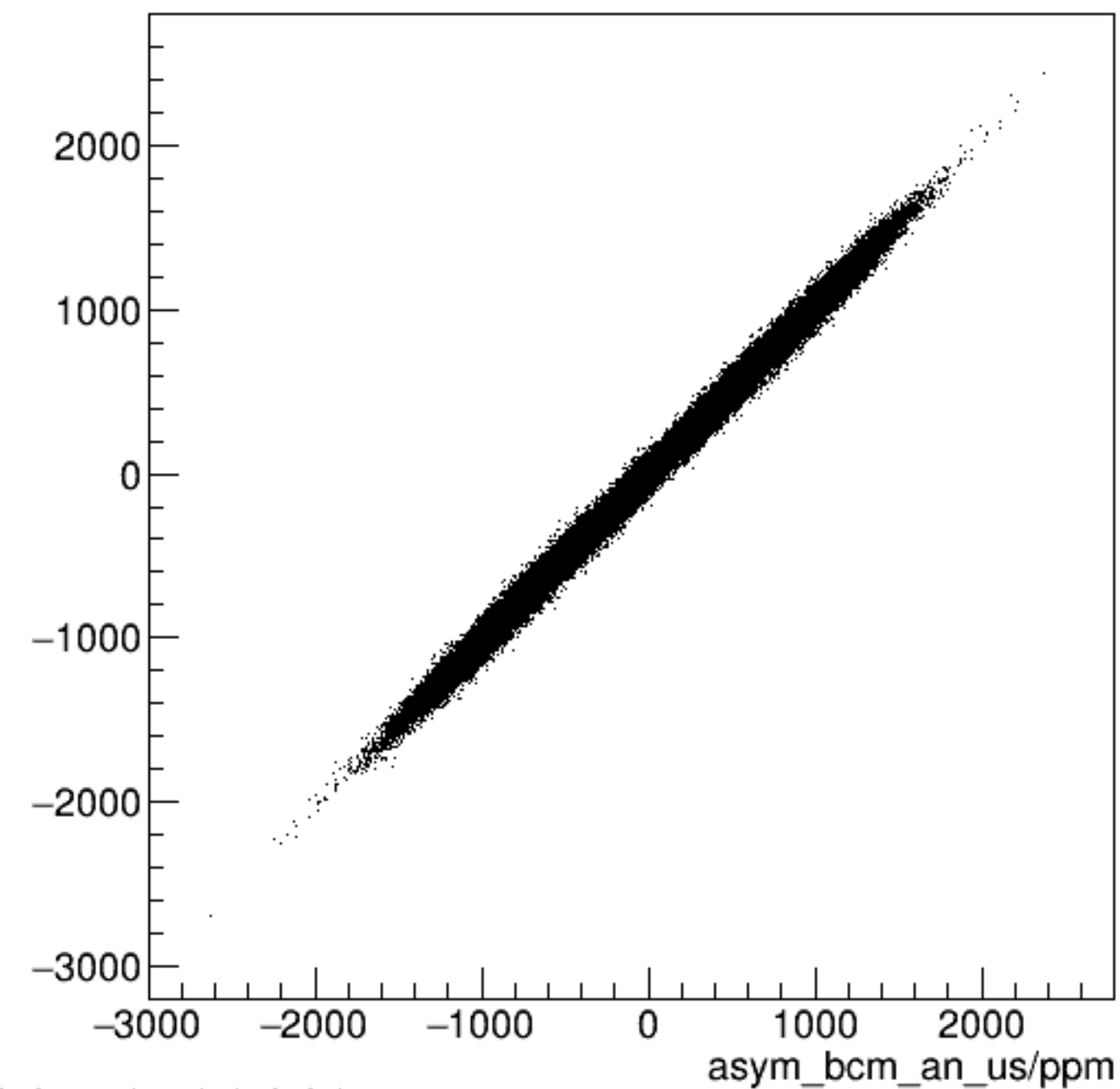
run7020_000_asym_bcm_dg_ds_vs_asym_bcm_an_us_pr.png
