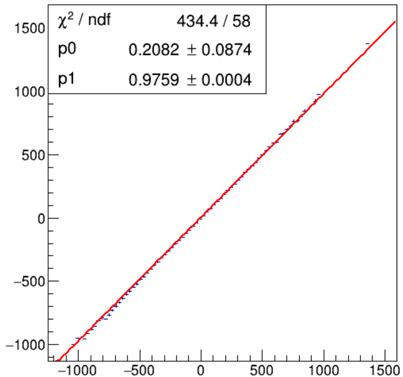
run7020_000_asym_bcm_an_us_vs_asym_bcm_an_ds3_mul.png
