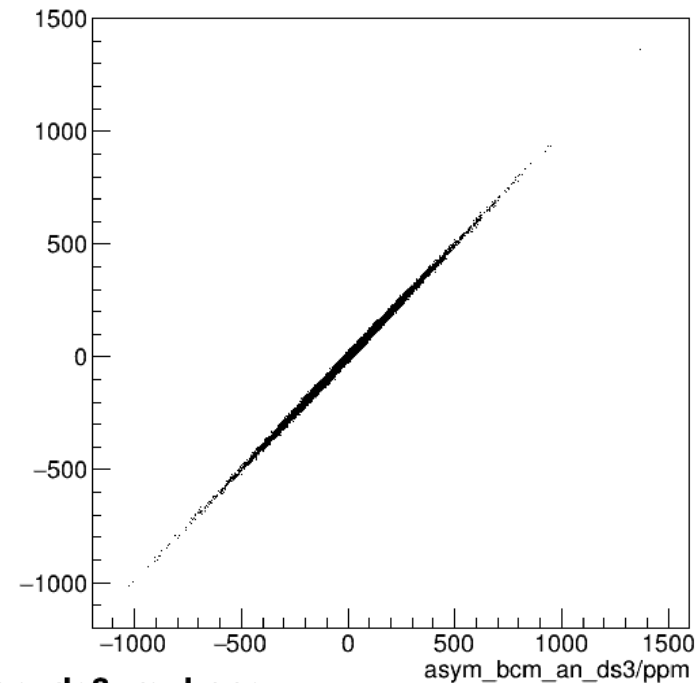
run7020_000_asym_bcm_an_ds_vs_asym_bcm_an_ds3_mul.png
