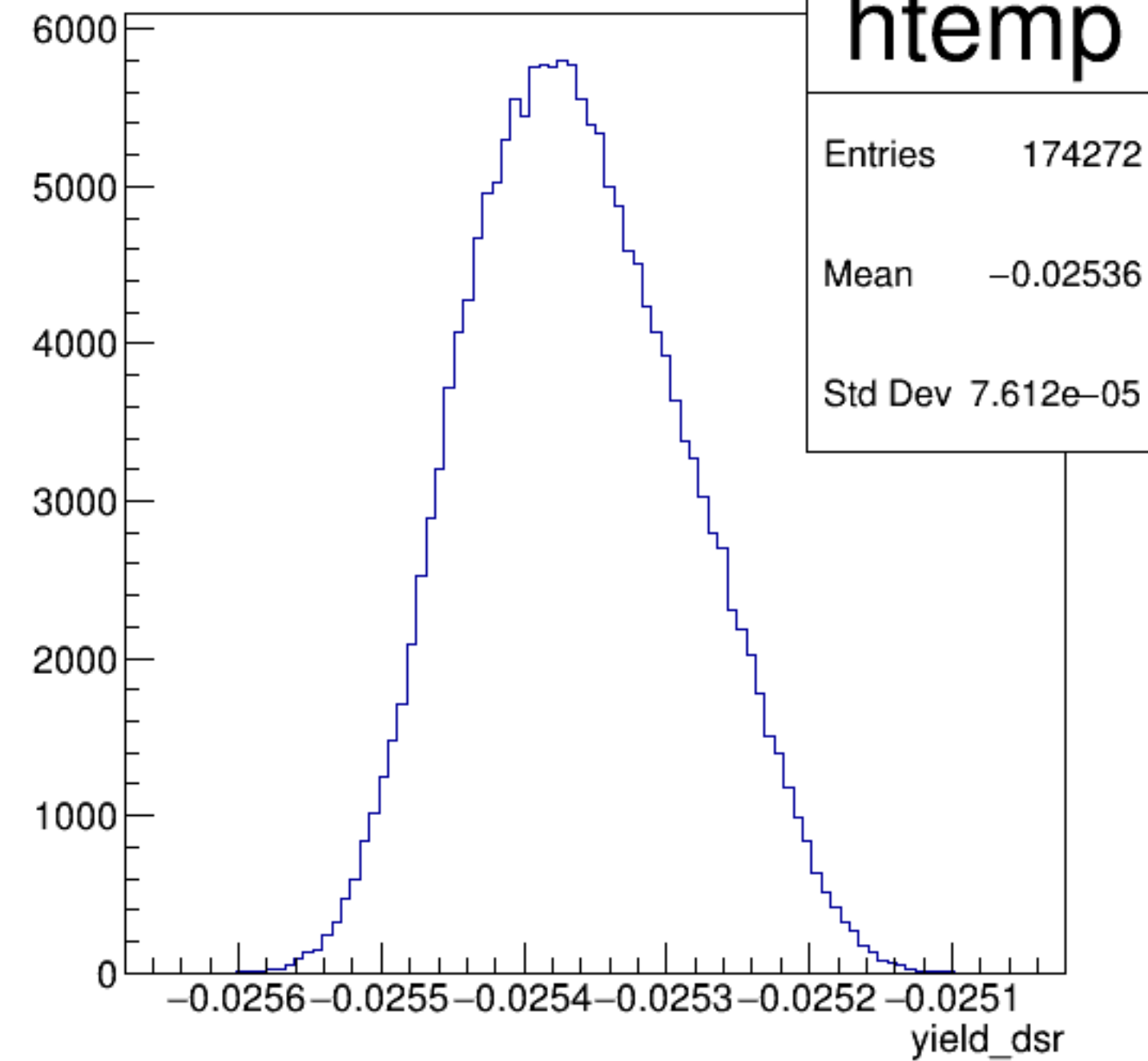
yield_dsr {ErrorFlag==0}
