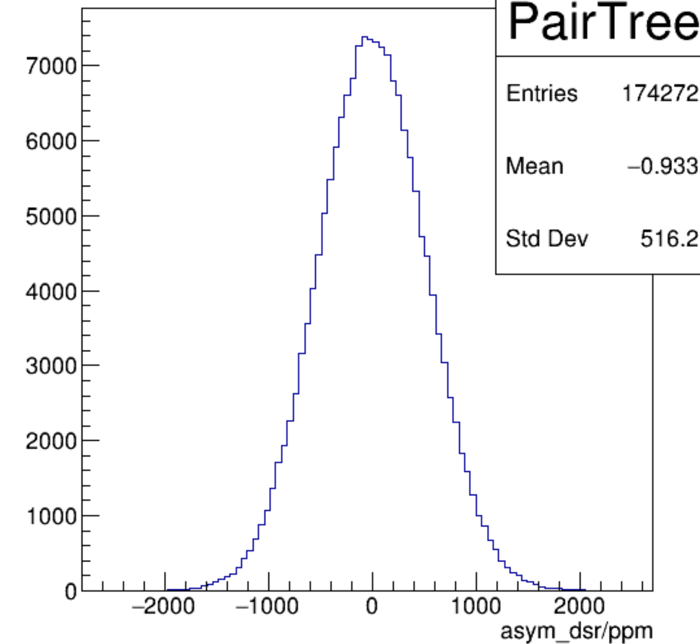
asym_dsr/ppm {ErrorFlag==0}
