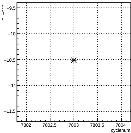
4eY_coil7:cyclenum {run == 7040}
