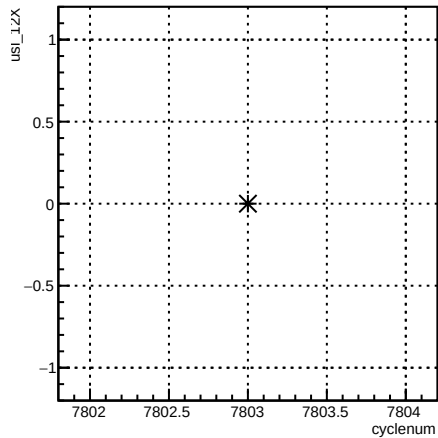
usl_12X:cyclenum {run == 7040}
