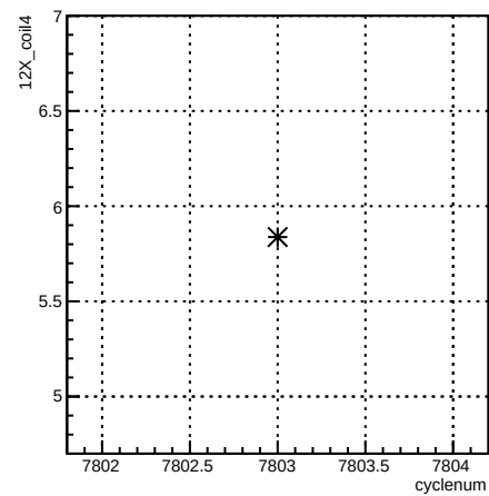
12X_coil4:cyclenum {run == 7040}
