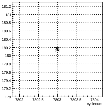
4eY_coil4:cyclenum {run == 7040}
