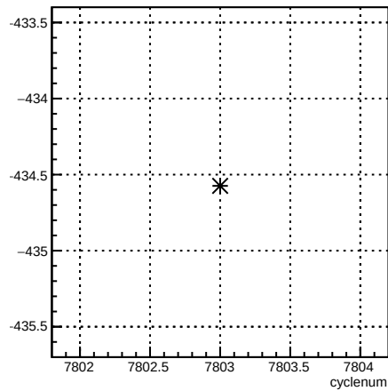
4eX_coil1:cyclenum {run == 7040}
