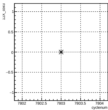
12X_coil3:cyclenum {run == 7040}
