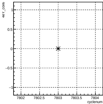
4eY_coil6:cyclenum {run == 7040}
