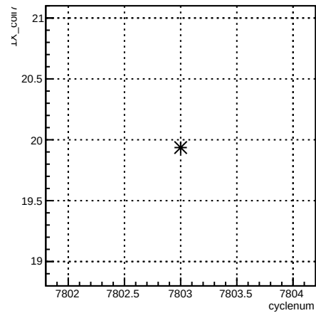
4eX_coil7:cyclenum {run == 7040}
