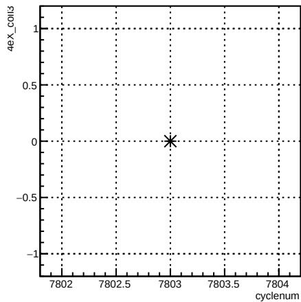
4eX_coil3:cyclenum {run == 7040}
