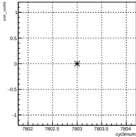
usr_coil6:cyclenum {run == 7040}
