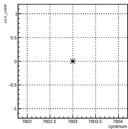
12X_coil6:cyclenum {run == 7040}
