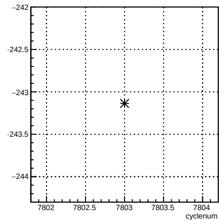
12X_coil1:cyclenum {run == 7040}
