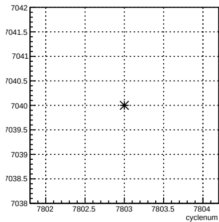
run:cyclenum {run == 7040}
