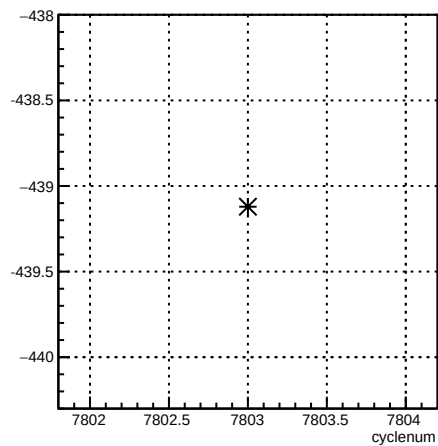
12X_coil7:cyclenum {run == 7040}
