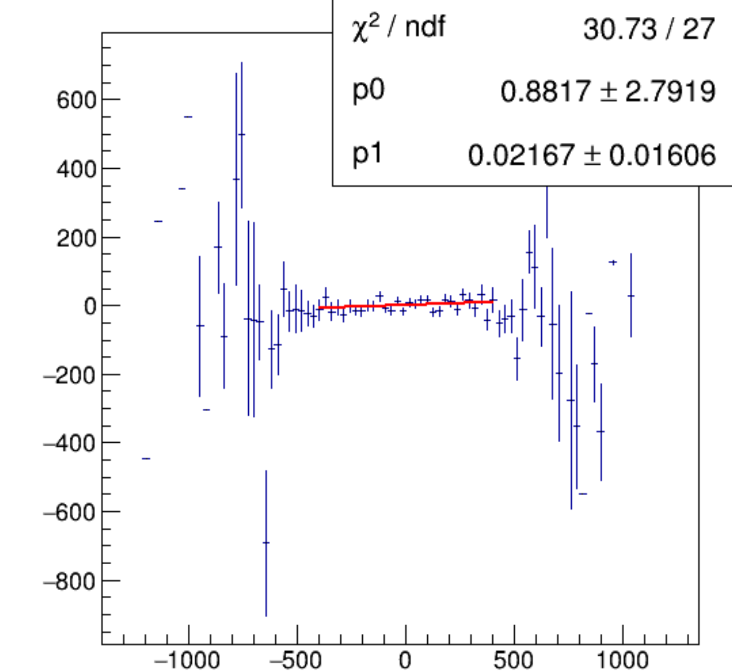
reg_asym_dsr/ppm:AqUS/ppm {ok_cut}
