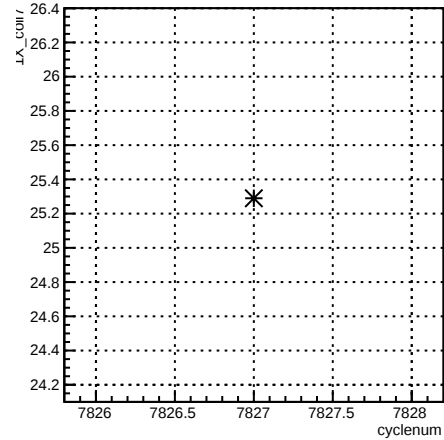
4eX_coil7:cyclenum {run == 7047}
