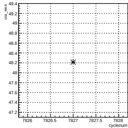
usl_4eX:cyclenum {run == 7047}
