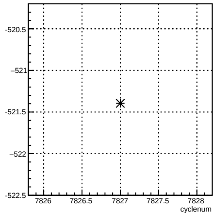
4eX_coil1:cyclenum {run == 7047}
