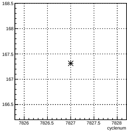
4aY_coil4:cyclenum {run == 7047}
