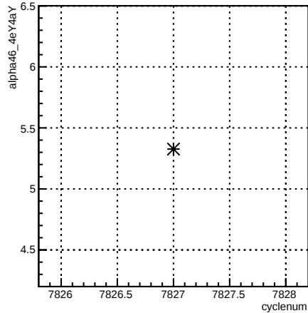
alpha46_4eY4aY:cyclenum {run == 7047}
