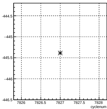
12X_coil7:cyclenum {run == 7047}
