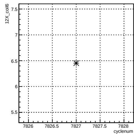
12X_coil6:cyclenum {run == 7047}
