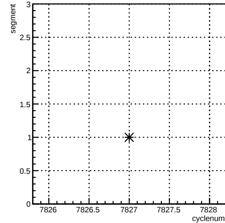
segment:cyclenum {run == 7047}
