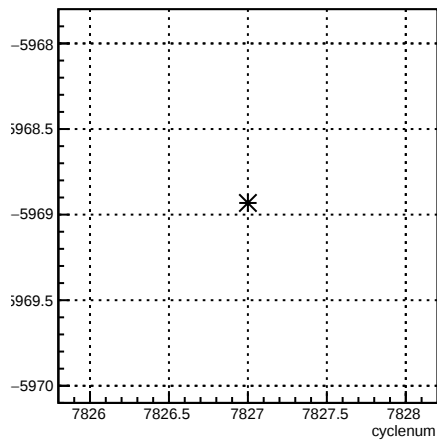
usr_coil7:cyclenum {run == 7047}
