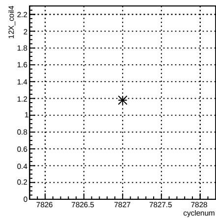
12X_coil4:cyclenum {run == 7047}
