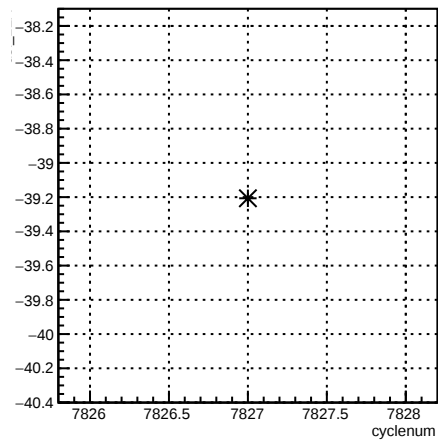
usl_12X:cyclenum {run == 7047}
