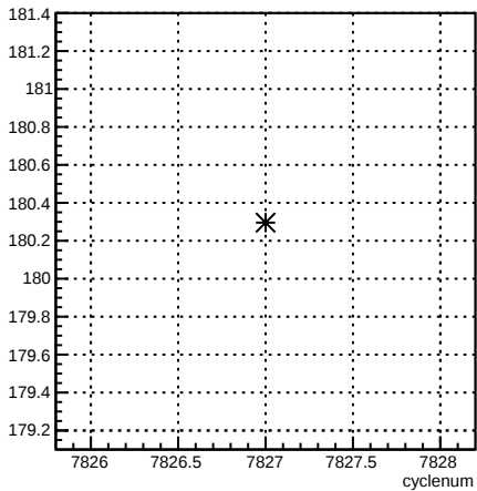
4eY_coil4:cyclenum {run == 7047}
