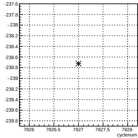
12X_coil1:cyclenum {run == 7047}
