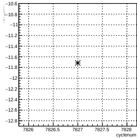
4aY_coil7:cyclenum {run == 7047}
