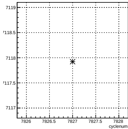
usl_coil7:cyclenum {run == 7047}
