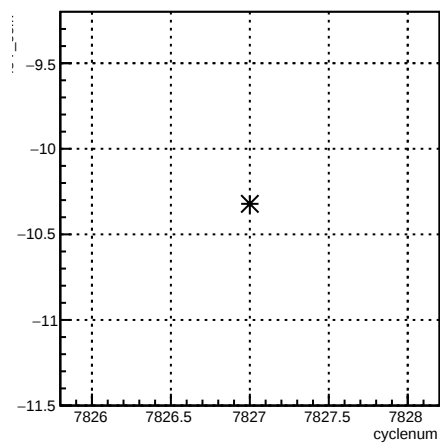
4eY_coil7:cyclenum {run == 7047}
