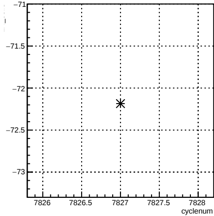
4eX_coil3:cyclenum {run == 7047}
