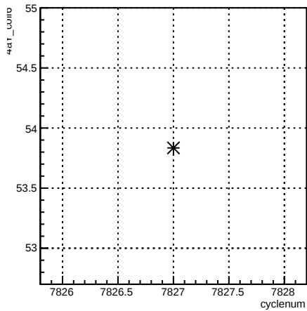
4aY_coil6:cyclenum {run == 7047}
