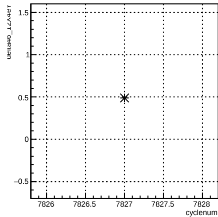
delta46_12X4eY:cyclenum {run == 7047}
