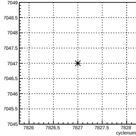
run:cyclenum {run == 7047}
