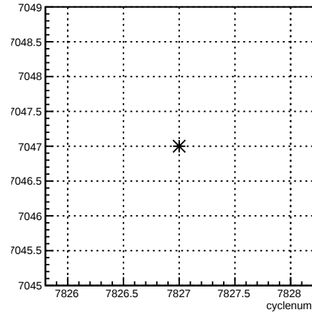
run:cyclenum {run == 7047}
