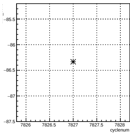
12X_coil3:cyclenum {run == 7047}
