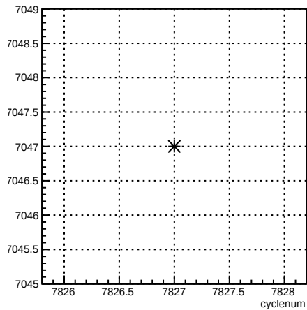
run:cyclenum {run == 7047}
