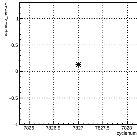
alpha13_4eX1X:cyclenum {run == 7047}
