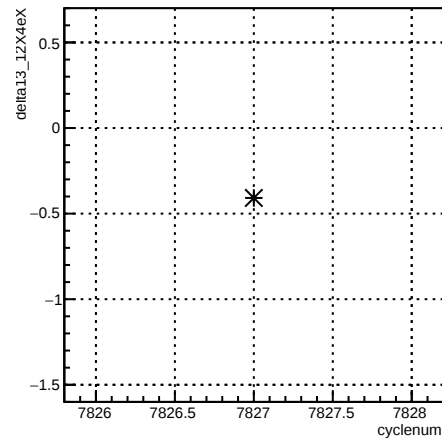
delta13_12X4eX:cyclenum {run == 7047}
