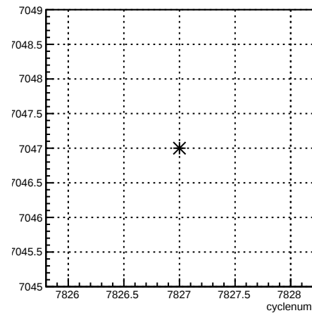
run:cyclenum {run == 7047}
