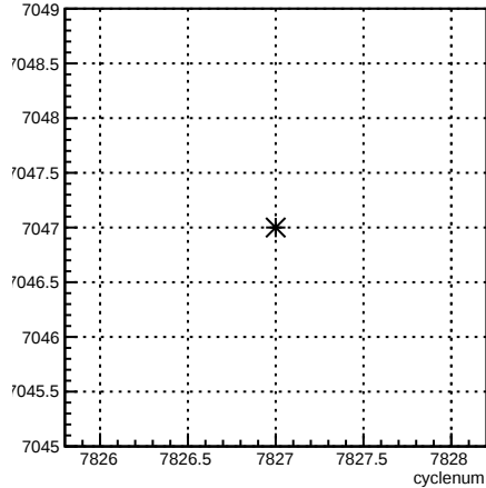
run:cyclenum {run == 7047}
