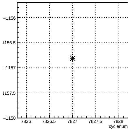
usl_coil6:cyclenum {run == 7047}
