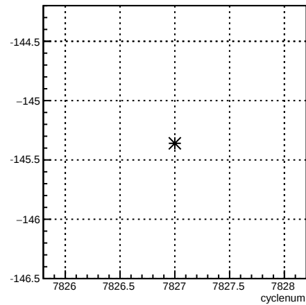
usr_4eY:cyclenum {run == 7047}
