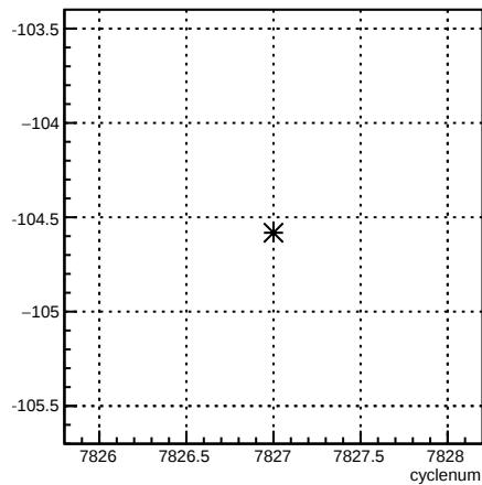
usr_coil6:cyclenum {run == 7047}
