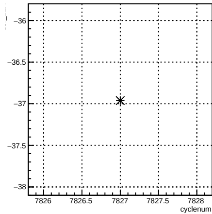
usr_12X:cyclenum {run == 7047}
