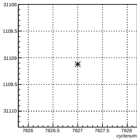
usr_coil1:cyclenum {run == 7047}
