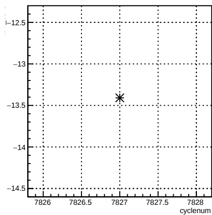
4eY_coil6:cyclenum {run == 7047}
