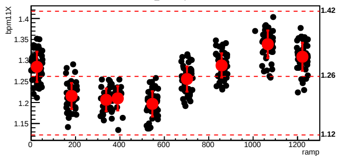
bmod_trim3,cyc=7828
