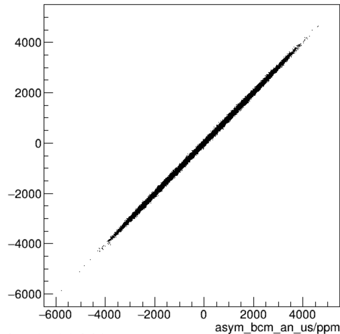
run7063_000_asym_bcm_dg_ds_vs_asym_bcm_an_us_pr.png
