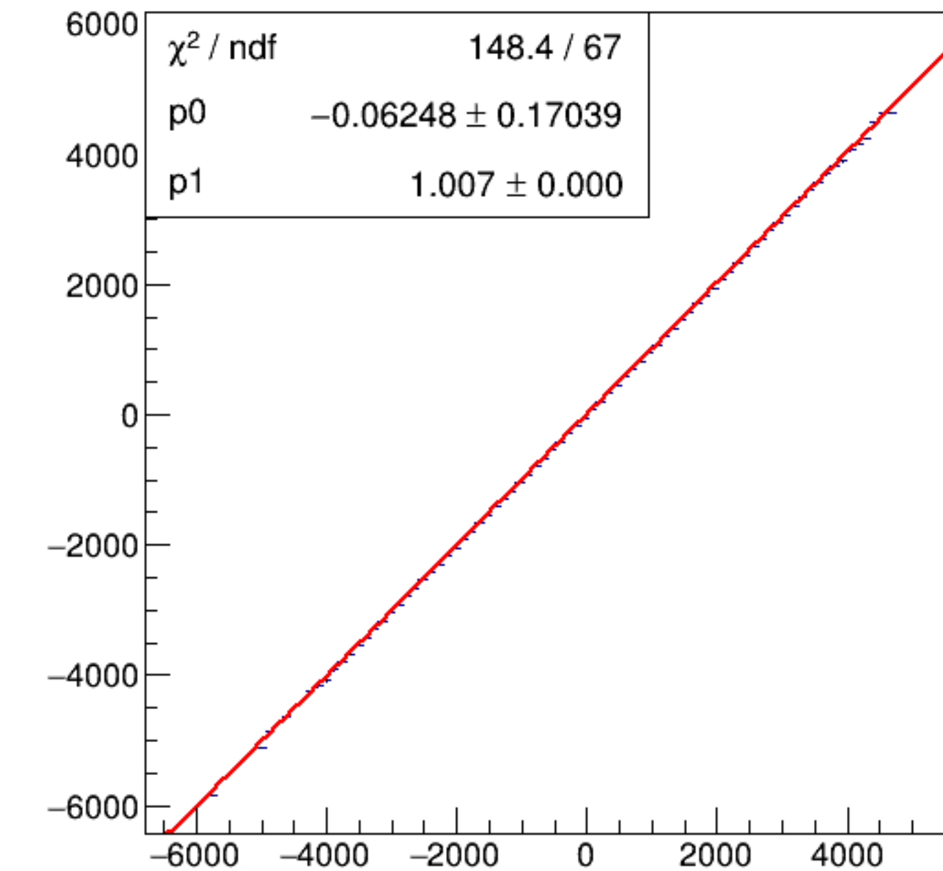
run7063_000_asym_bcm_dg_ds_vs_asym_bcm_an_us_pr.png
