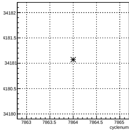
usl_coil6:cyclenum {run == 7064}
