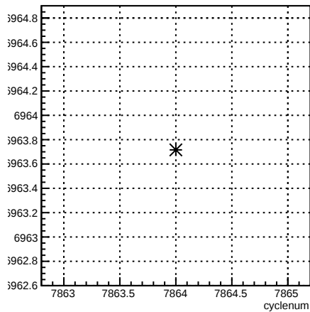
usl_coil7:cyclenum {run == 7064}
