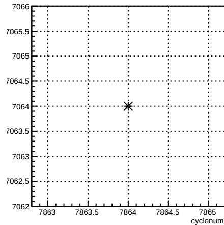
run:cyclenum {run == 7064}
