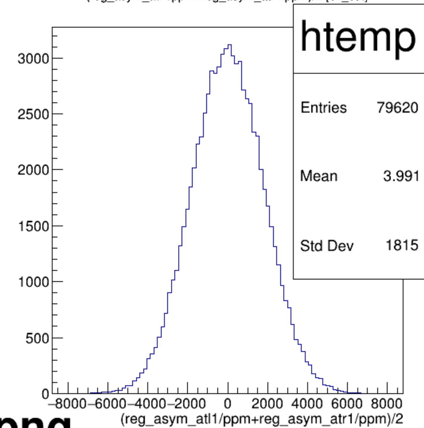
(reg_asym_atl1/ppm+reg_asym_atr1/ppm)/2 {ok_cut}
