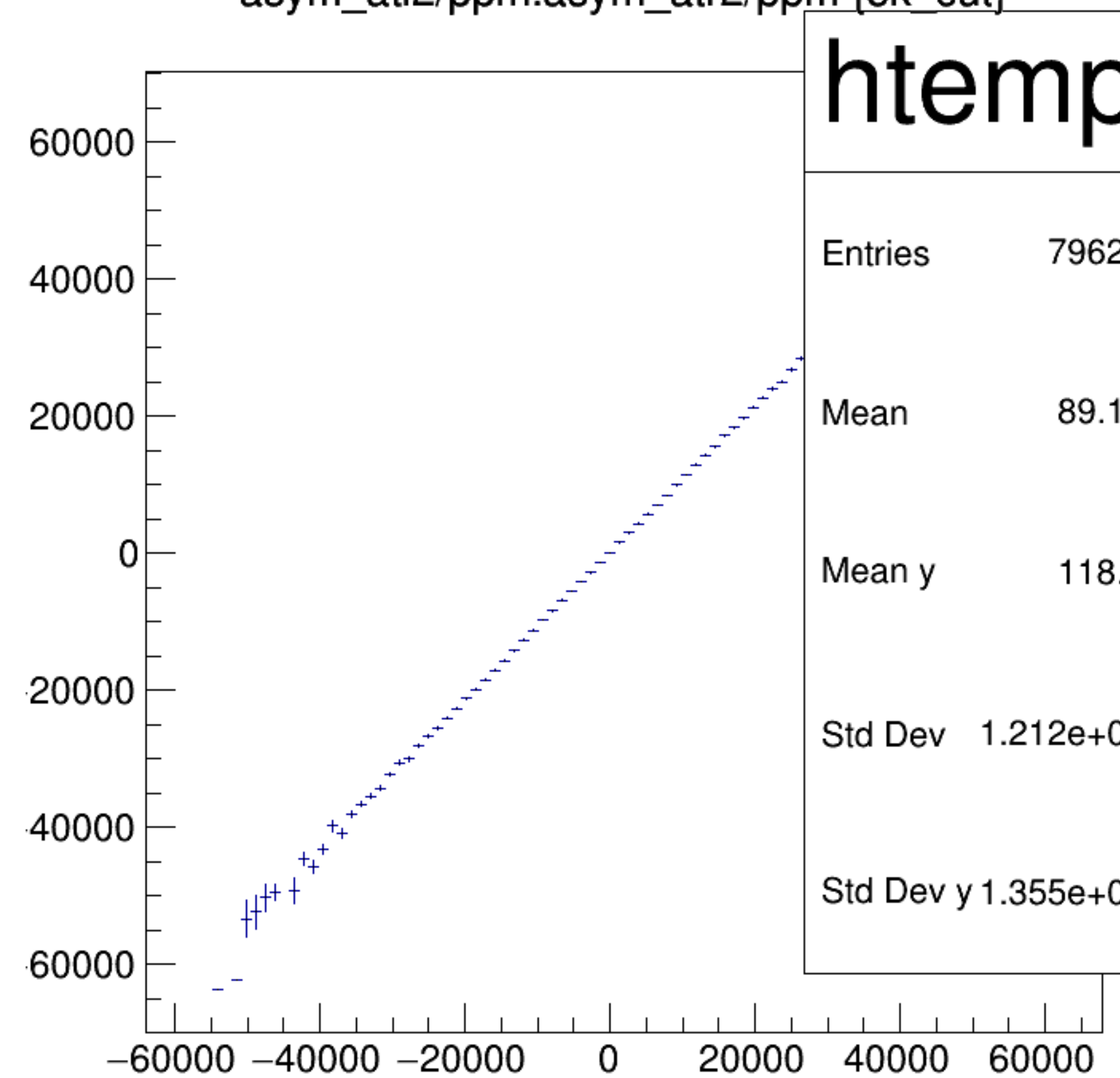
asym_atl2/ppm:asym_atr2/ppm {ok_cut}
