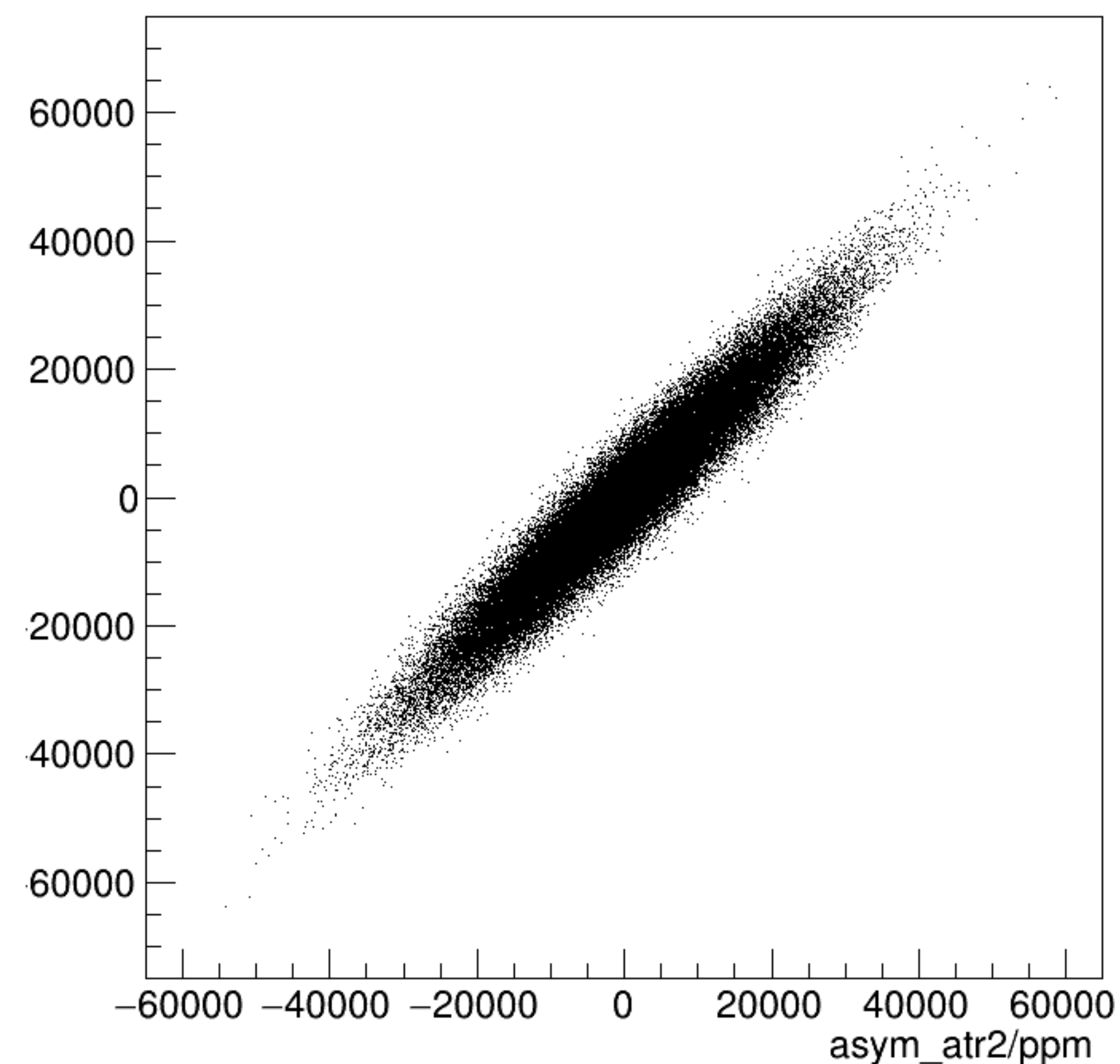
asym_atl2/ppm:asym_atr2/ppm {ok_cut}
