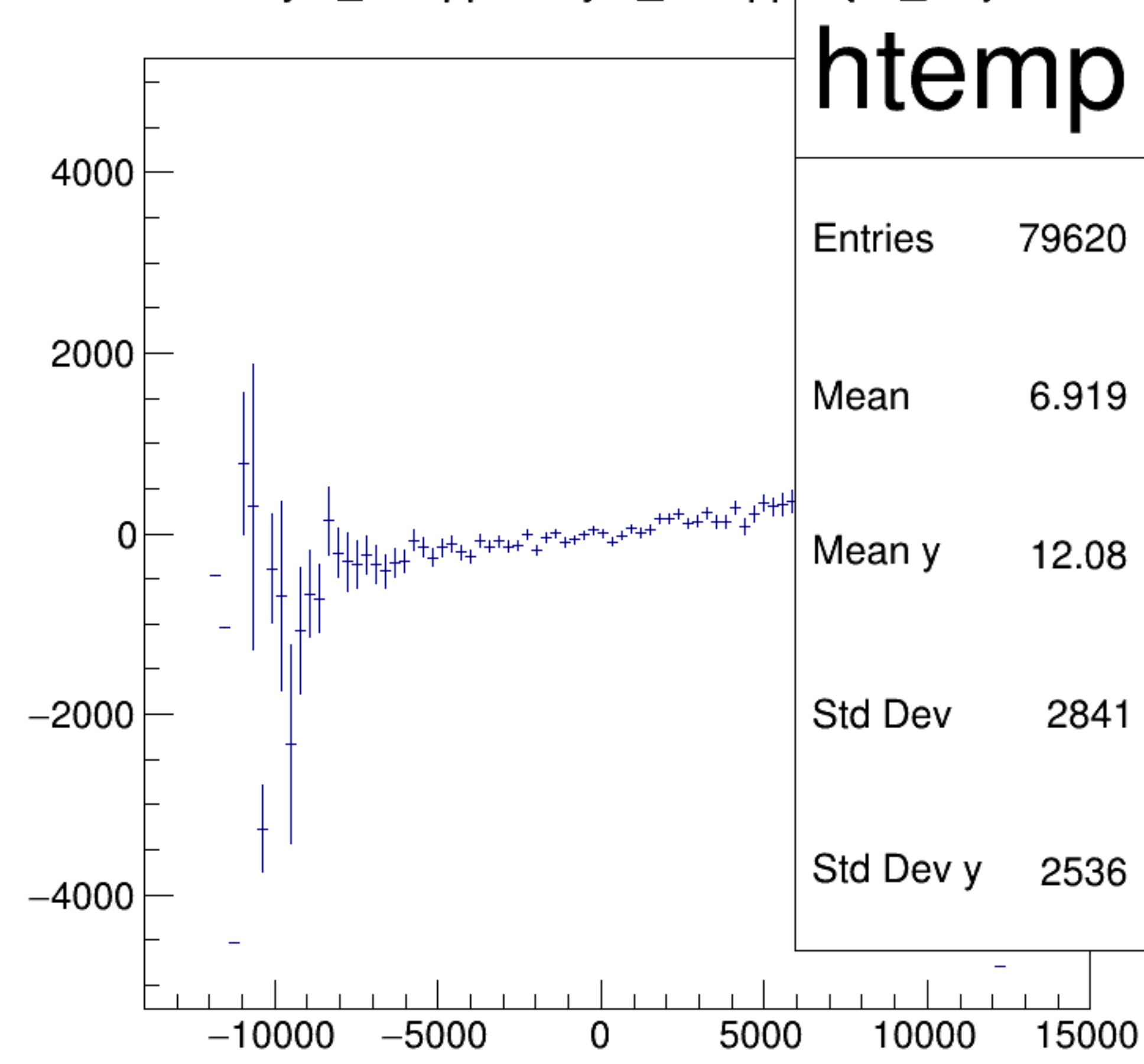
asym_atl1/ppm:asym_atr1/ppm {ok_cut}
