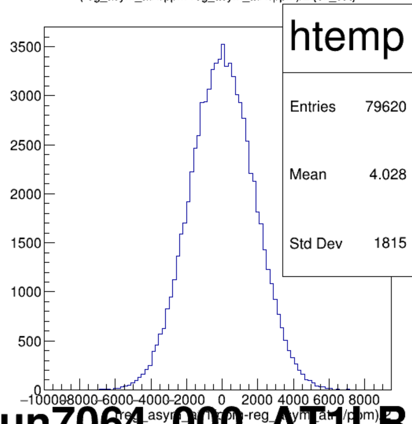
(reg_asym_atl1/ppm-reg_asym_atr1/ppm)/2 {ok_cut}
