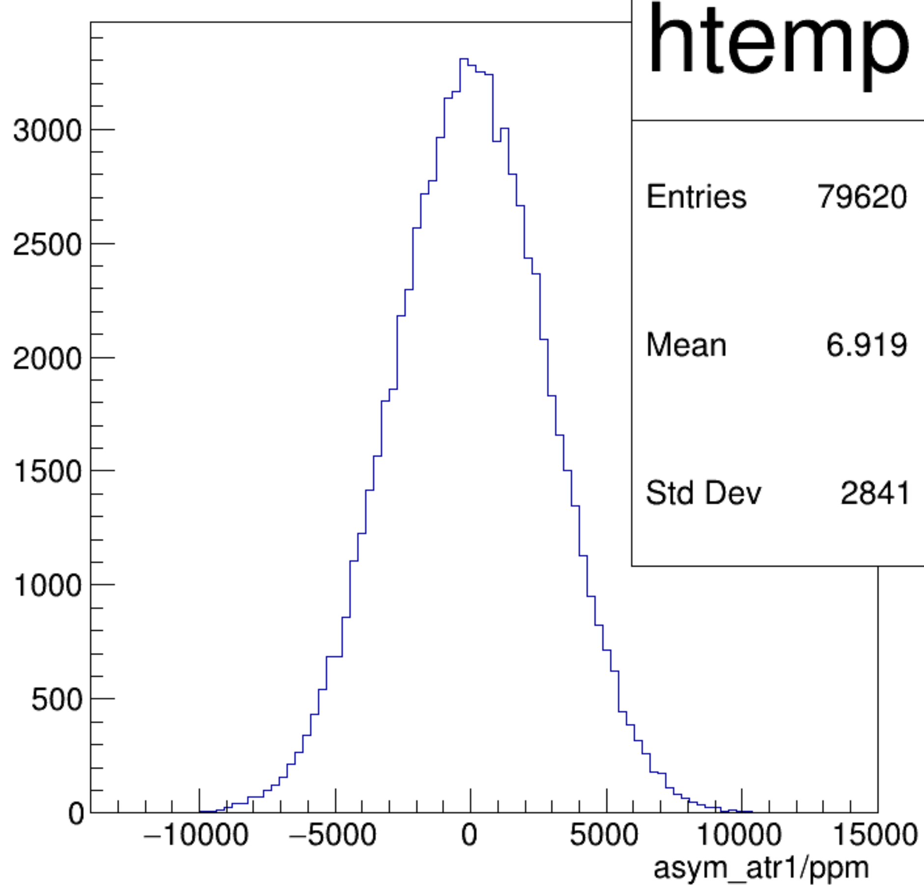
asym_atr1/ppm {ok_cut}
