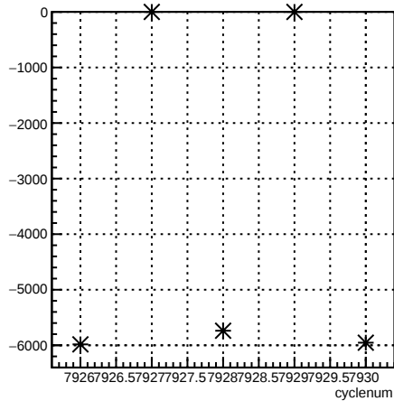
usr_coil3:cyclenum {run == 7077}
