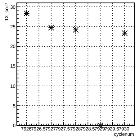
1X_coil7:cyclenum {run == 7077}
