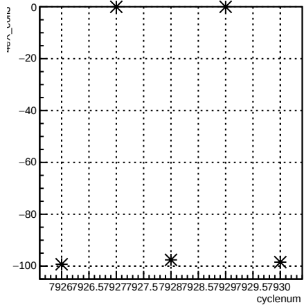
4eX_coil3:cyclenum {run == 7077}
