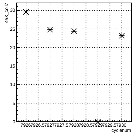
4eX_coil7:cyclenum {run == 7077}
