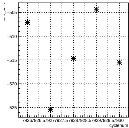
4eX_coil1:cyclenum {run == 7077}
