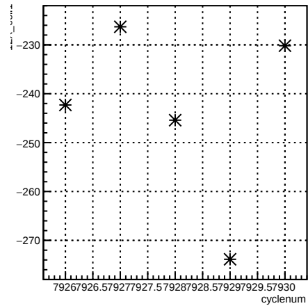
12X_coil6:cyclenum {run == 7077}
