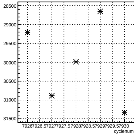
usr_coil6:cyclenum {run == 7077}
