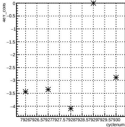
4eY_coil6:cyclenum {run == 7077}
