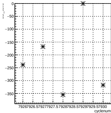
usr_coil6:cyclenum {run == 7077}
