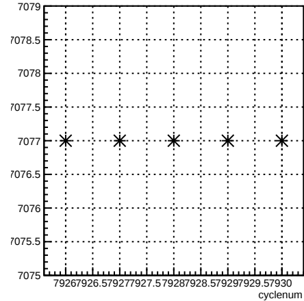
run:cyclenum {run == 7077}
