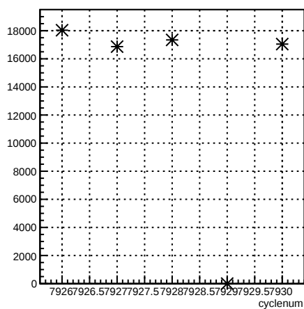
usr_coil7:cyclenum {run == 7077}
