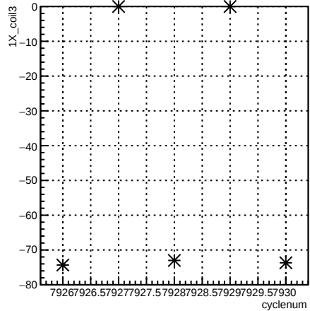
1X_coil3:cyclenum {run == 7077}
