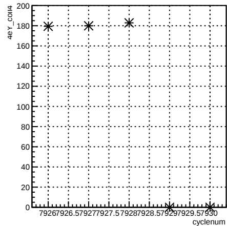
4eY_coil4:cyclenum {run == 7077}
