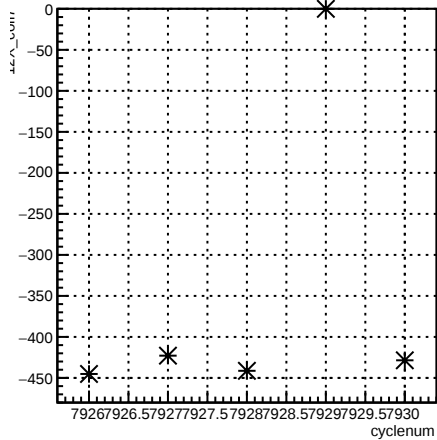
12X_coil7:cyclenum {run == 7077}
