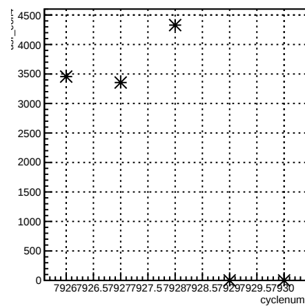
usr_coil4:cyclenum {run == 7077}
