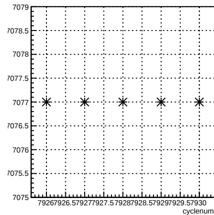
run:cyclenum {run == 7077}
