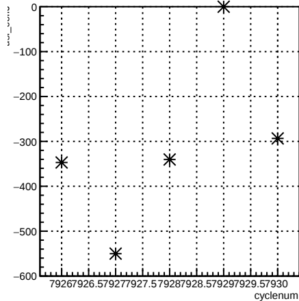
usl_coil6:cyclenum {run == 7077}
