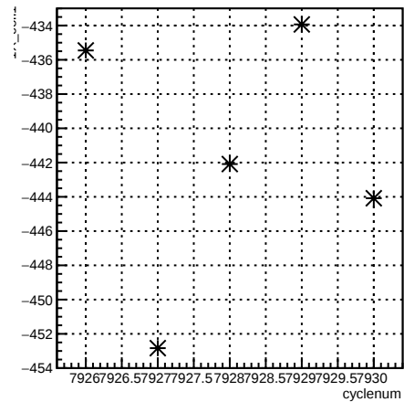
1X_coil1:cyclenum {run == 7077}
