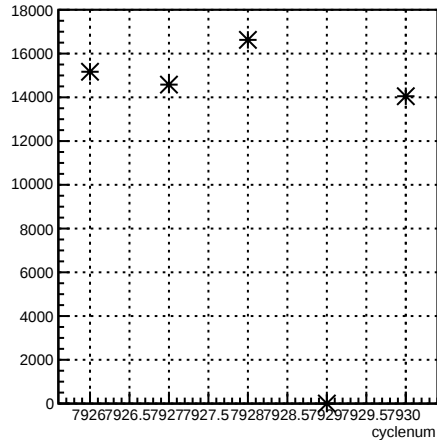
usl_coil7:cyclenum {run == 7077}
