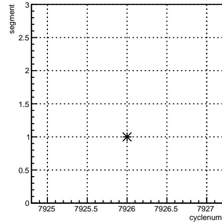
segment:cyclenum {run == 7077}
