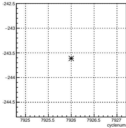
12X_coil1:cyclenum {run == 7077}
