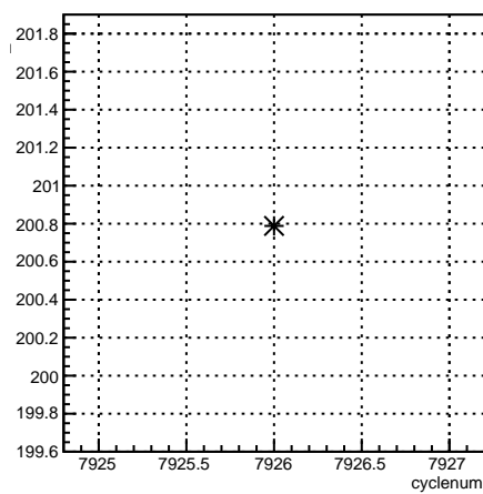
usr_4eX:cyclenum {run == 7077}
