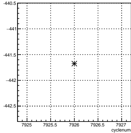
1X_coil1:cyclenum {run == 7077}
