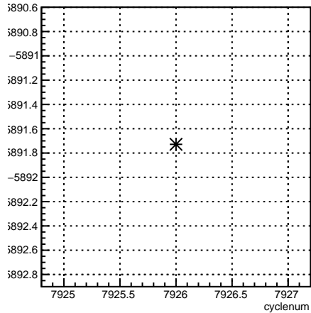
usr_coil3:cyclenum {run == 7077}
