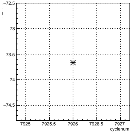
1X_coil3:cyclenum {run == 7077}
