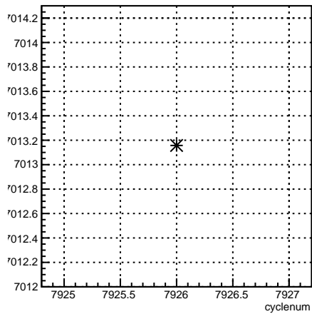
usl_coil7:cyclenum {run == 7077}
