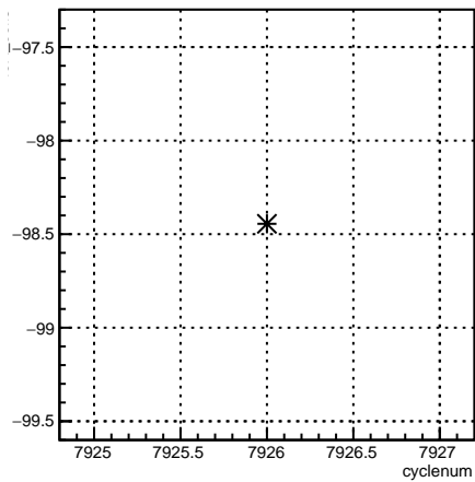
4eX_coil3:cyclenum {run == 7077}
