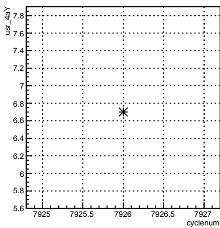
usr_4aY:cyclenum {run == 7077}
