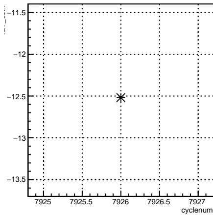
4eY_coil7:cyclenum {run == 7077}
