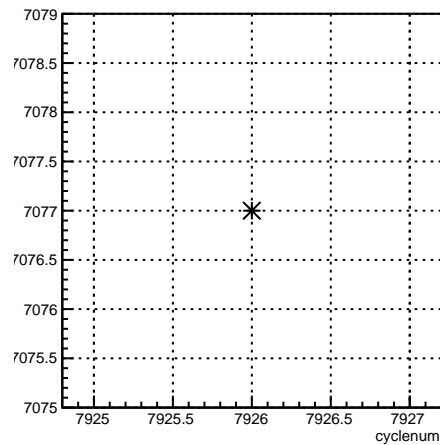
run:cyclenum {run == 7077}
