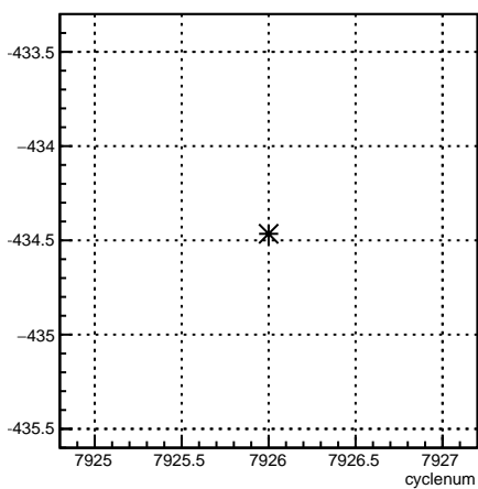
12X_coil7:cyclenum {run == 7077}
