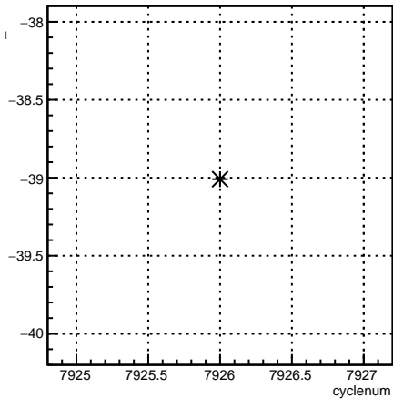
usl_12X:cyclenum {run == 7077}
