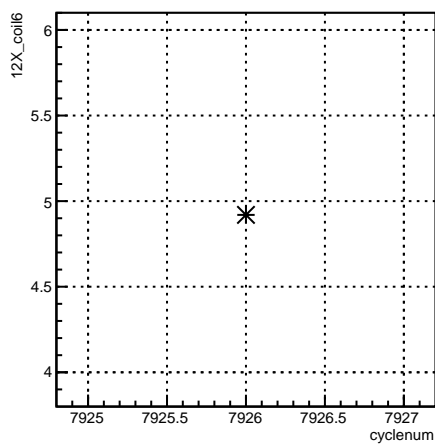
12X_coil6:cyclenum {run == 7077}
