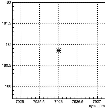
4eY_coil4:cyclenum {run == 7077}
