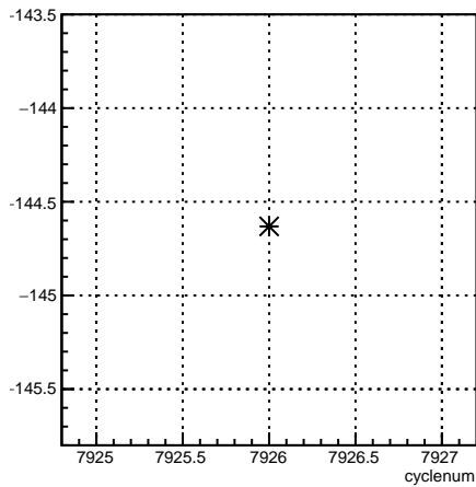
usr_1X:cyclenum {run == 7077}
