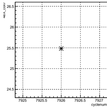
4eX_coil7:cyclenum {run == 7077}
