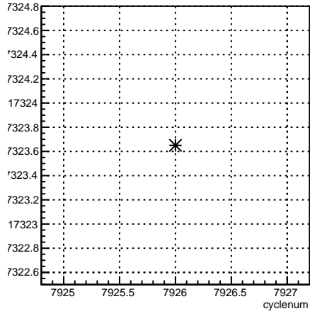
usr_coil7:cyclenum {run == 7077}
