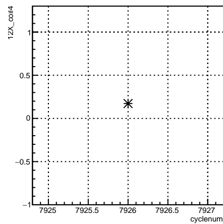
12X_coil4:cyclenum {run == 7077}
