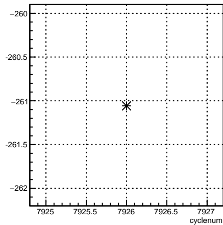
usr_coil6:cyclenum {run == 7077}
