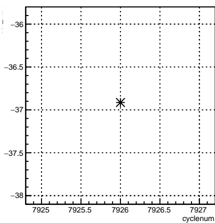
usr_12X:cyclenum {run == 7077}
