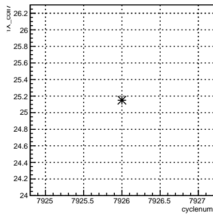
1X_coil7:cyclenum {run == 7077}
