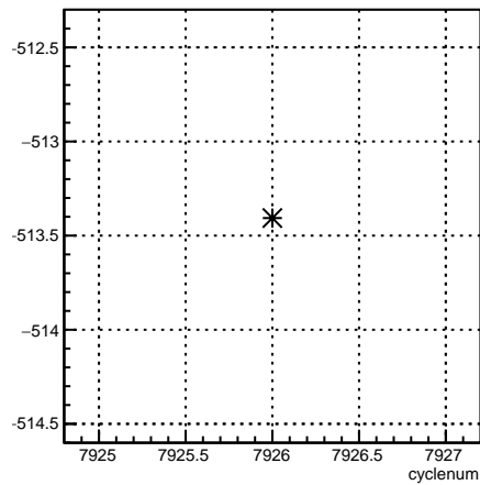
4eX_coil1:cyclenum {run == 7077}
