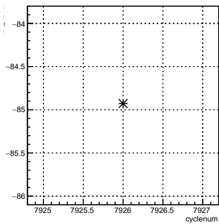
12X_coil3:cyclenum {run == 7077}
