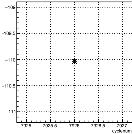
usl_4eY:cyclenum {run == 7077}
