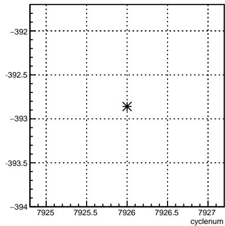
usl_coil6:cyclenum {run == 7077}
