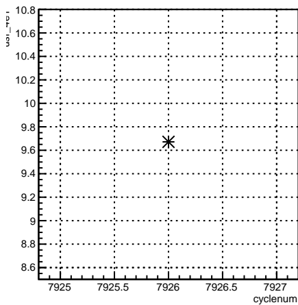
usr_4eY:cyclenum {run == 7077}
