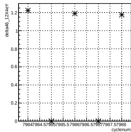
delta46_12X4eY:cyclenum {run == 7092}
