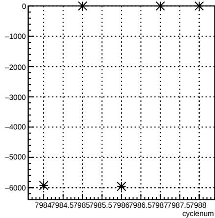
usr_coil3:cyclenum {run == 7092}
