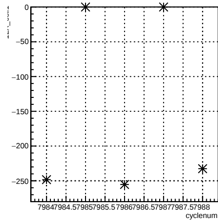
12X_coil1:cyclenum {run == 7092}
