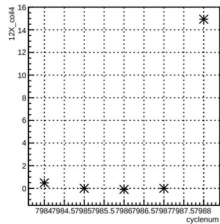
12X_coil4:cyclenum {run == 7092}
