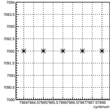
run:cyclenum {run == 7092}
