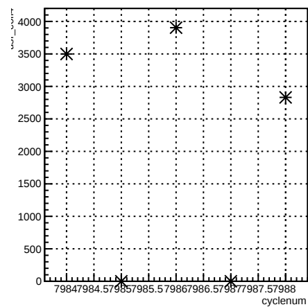
usr_coil4:cyclenum {run == 7092}
