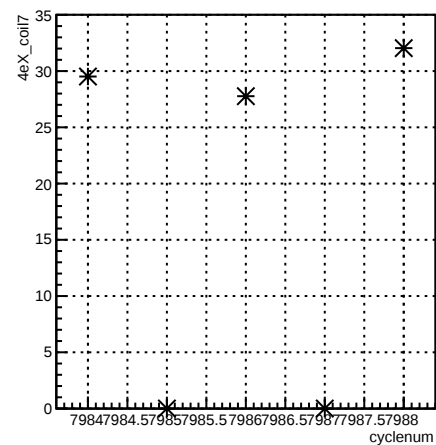
4eX_coil7:cyclenum {run == 7092}
