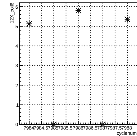
12X_coil6:cyclenum {run == 7092}
