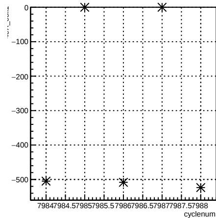
4eX_coil1:cyclenum {run == 7092}
