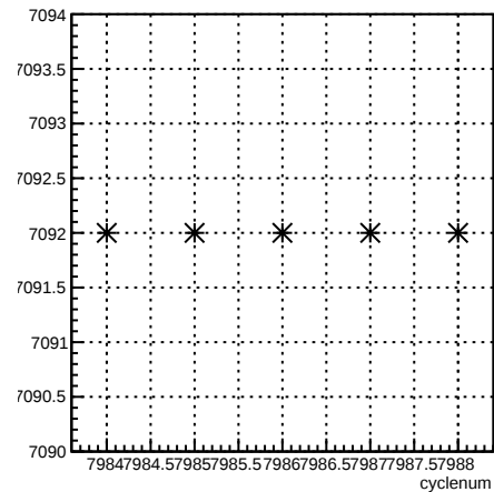
run:cyclenum {run == 7092}
