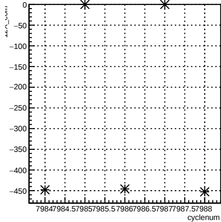
12X_coil7:cyclenum {run == 7092}
