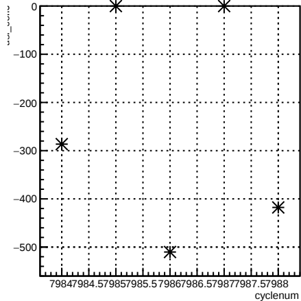
usl_coil6:cyclenum {run == 7092}
