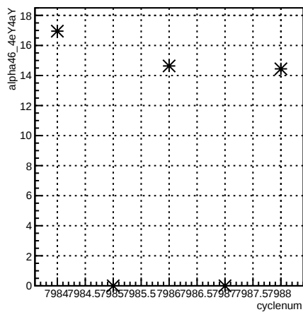
alpha46_4eY4aY:cyclenum {run == 7092}
