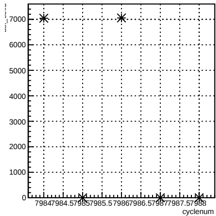
usl_coil7:cyclenum {run == 7092}
