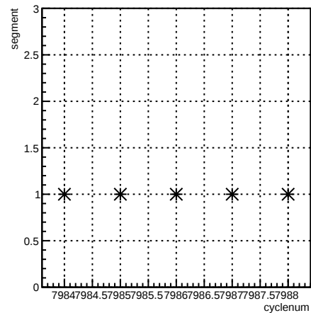
segment:cyclenum {run == 7092}
