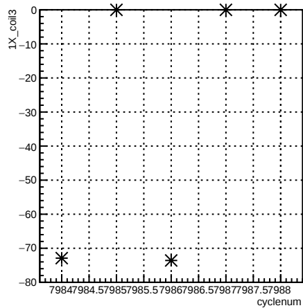
1X_coil3:cyclenum {run == 7092}
