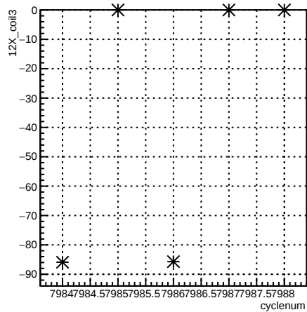
12X_coil3:cyclenum {run == 7092}
