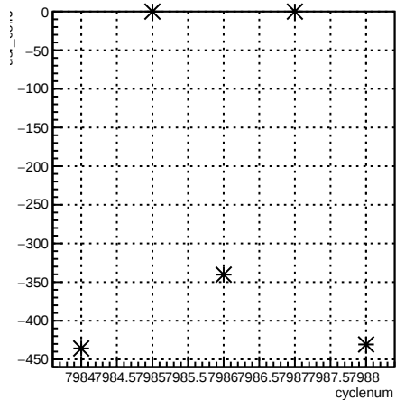
usr_coil6:cyclenum {run == 7092}
