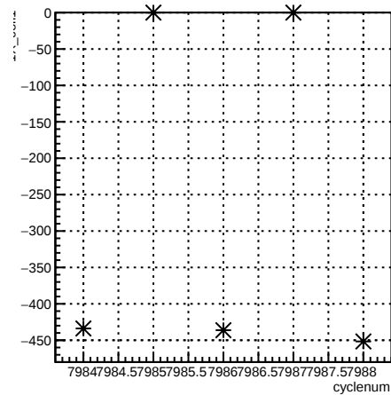
1X_coil1:cyclenum {run == 7092}
