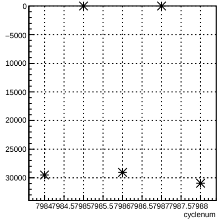
usr_coil1:cyclenum {run == 7092}
