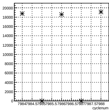
usr_coil7:cyclenum {run == 7092}
