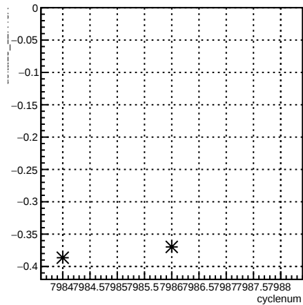
delta13_12X4eX:cyclenum {run == 7092}
