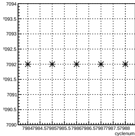
run:cyclenum {run == 7092}
