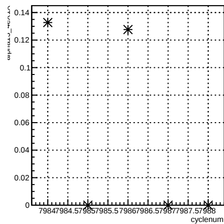
alpha13_4eX1X:cyclenum {run == 7092}
