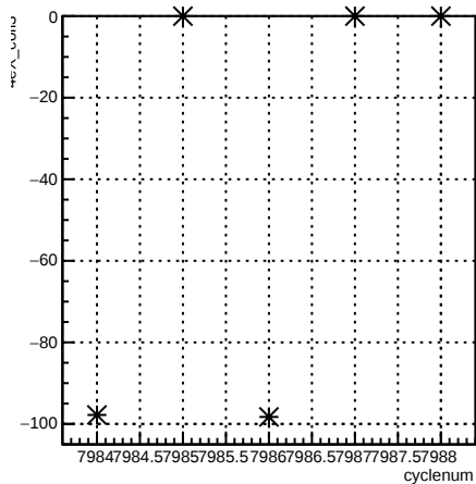
4eX_coil3:cyclenum {run == 7092}
