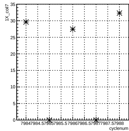
1X_coil7:cyclenum {run == 7092}
