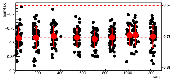
bmod_trim4,cyc=7994
