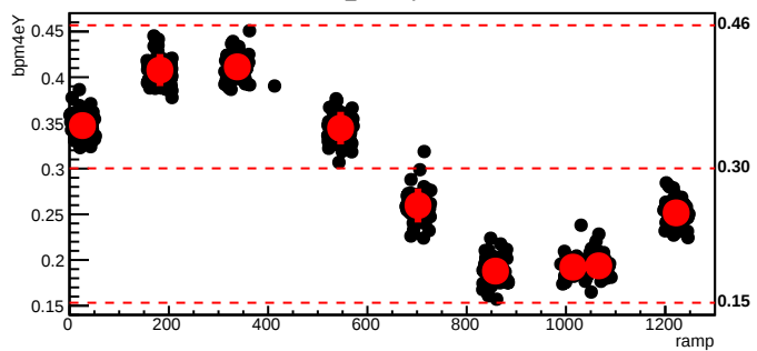
bmod_trim4,cyc=7994
