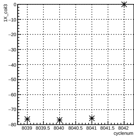
1X_coil3:cyclenum {run == 7110}
