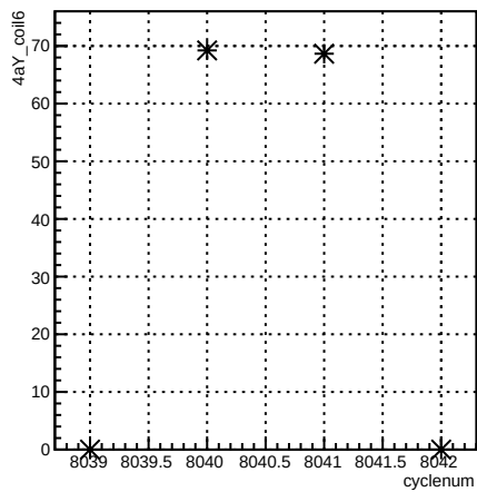
4aY_coil6:cyclenum {run == 7110}
