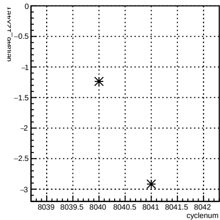
delta46_12X4eY:cyclenum {run == 7110}
