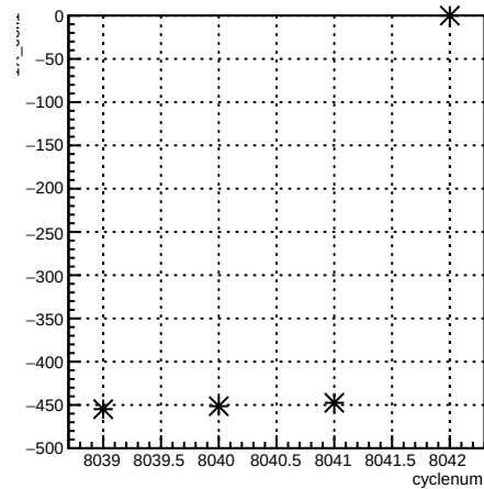
1X_coil1:cyclenum {run == 7110}
