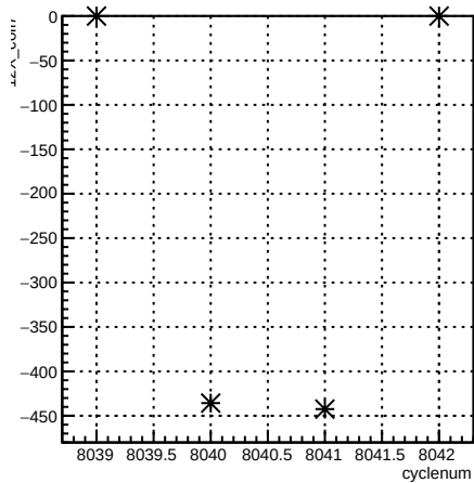
12X_coil7:cyclenum {run == 7110}
