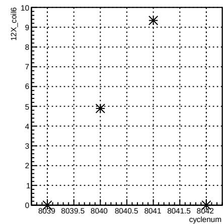
12X_coil6:cyclenum {run == 7110}
