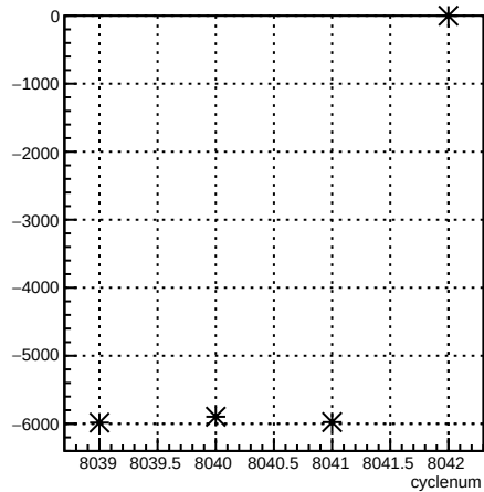
usr_coil3:cyclenum {run == 7110}
