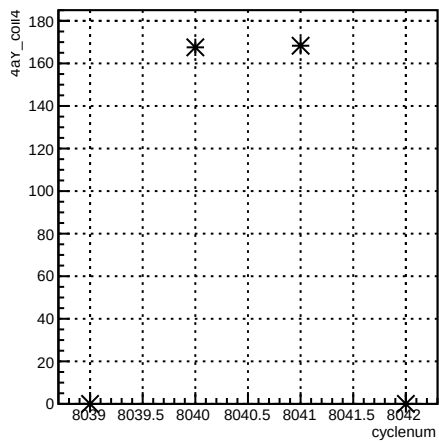
4aY_coil4:cyclenum {run == 7110}
