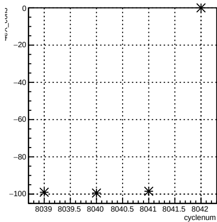
4eX_coil3:cyclenum {run == 7110}
