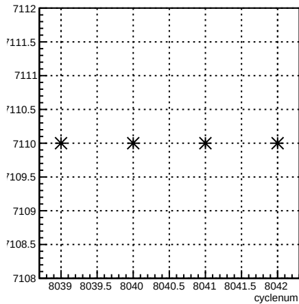
run:cyclenum {run == 7110}
