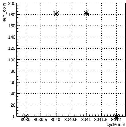
4eY_coil4:cyclenum {run == 7110}
