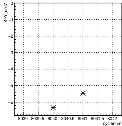
4eY_coil7:cyclenum {run == 7110}
