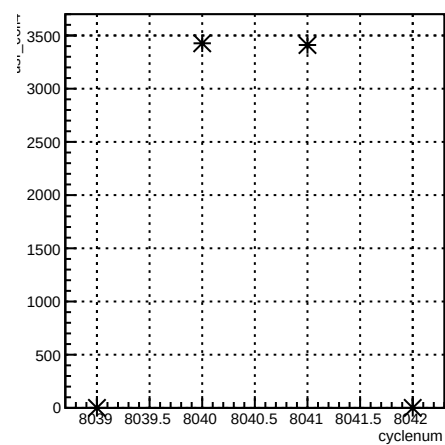
usr_coil4:cyclenum {run == 7110}
