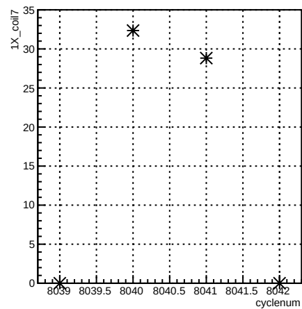
1X_coil7:cyclenum {run == 7110}
