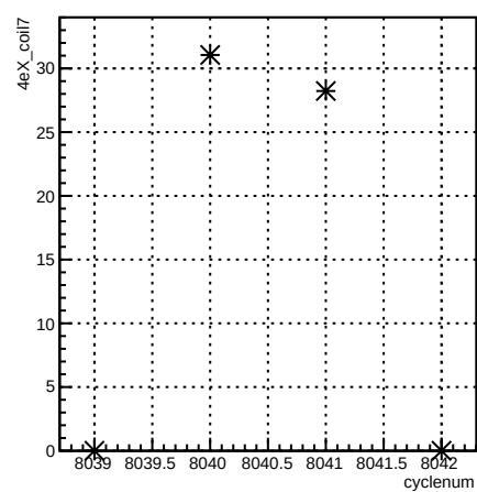
4eX_coil7:cyclenum {run == 7110}
