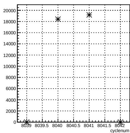
usr_coil7:cyclenum {run == 7110}
