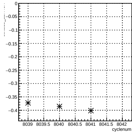
delta13_12X4eX:cyclenum {run == 7110}
