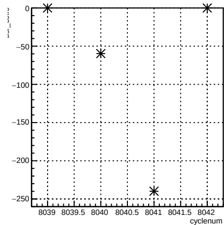
usr_coil6:cyclenum {run == 7110}
