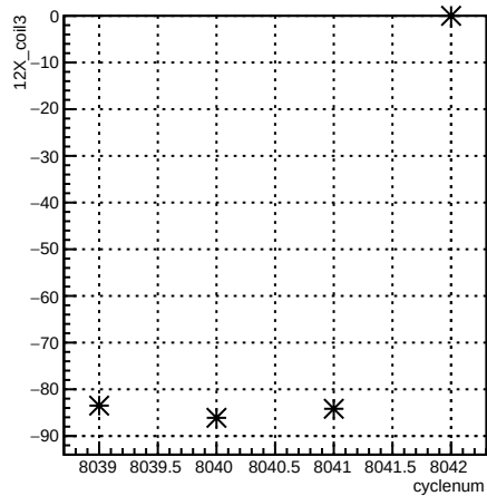
12X_coil3:cyclenum {run == 7110}
