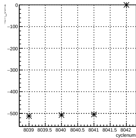
4eX_coil1:cyclenum {run == 7110}
