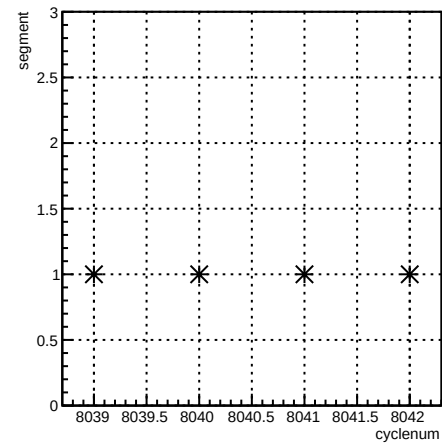
segment:cyclenum {run == 7110}
