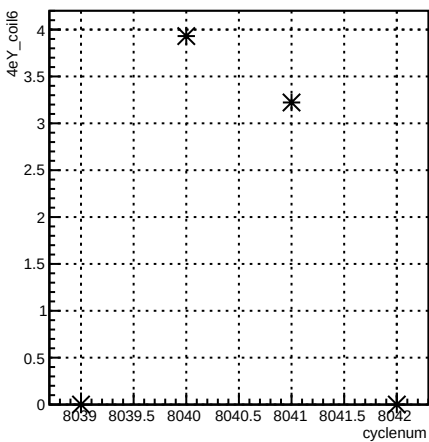
4eY_coil6:cyclenum {run == 7110}
