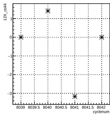
12X_coil4:cyclenum {run == 7110}
