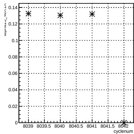
alpha13_4eX1X:cyclenum {run == 7110}
