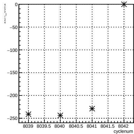
12X_coil1:cyclenum {run == 7110}
