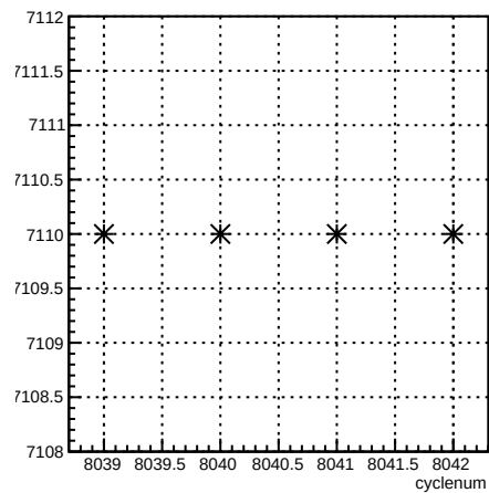
run:cyclenum {run == 7110}
