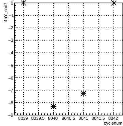
4aY_coil7:cyclenum {run == 7110}
