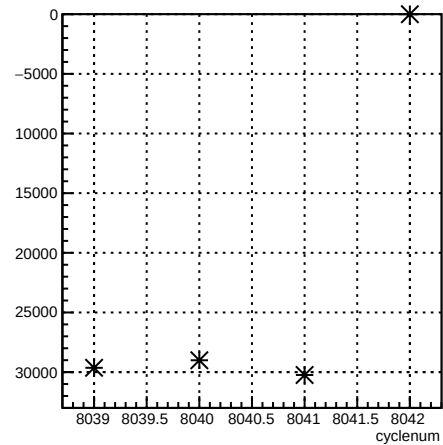
usr_coil1:cyclenum {run == 7110}
