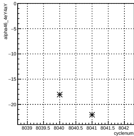
alpha46_4eY4aY:cyclenum {run == 7110}
