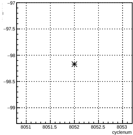
4eX_coil3:cyclenum {run == 7114}
