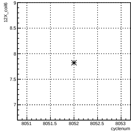
12X_coil6:cyclenum {run == 7114}
