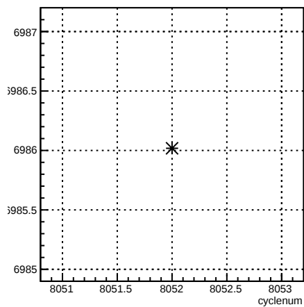
usl_coil3:cyclenum {run == 7114}
