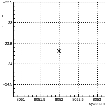
alpha46_4eY4aY:cyclenum {run == 7114}
