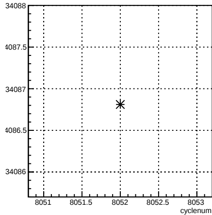
usl_coil1:cyclenum {run == 7114}
