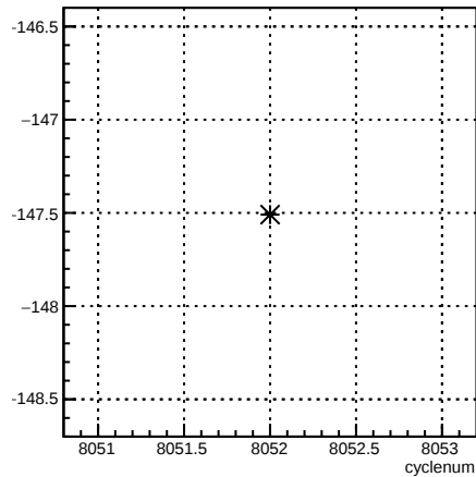
usr_4eY:cyclenum {run == 7114}
