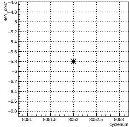
4eY_coil7:cyclenum {run == 7114}
