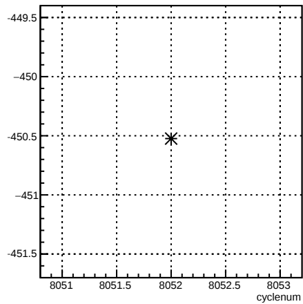
4eX_coil1:cyclenum {run == 7114}
