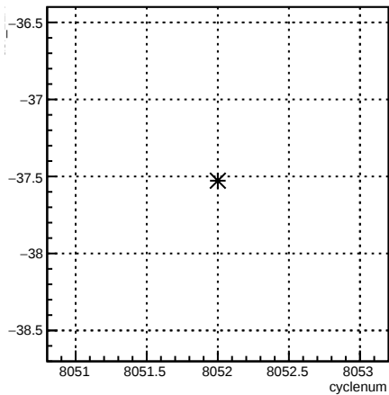
usr_12X:cyclenum {run == 7114}
