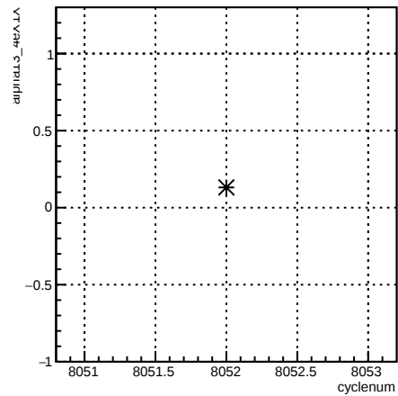
alpha13_4eX1X:cyclenum {run == 7114}
