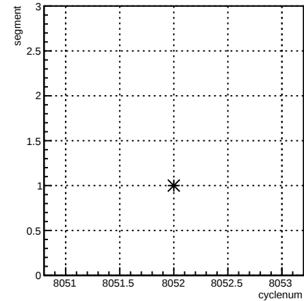
segment:cyclenum {run == 7114}
