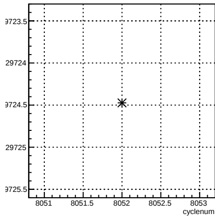
usr_coil6:cyclenum {run == 7114}
