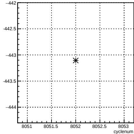
12X_coil7:cyclenum {run == 7114}
