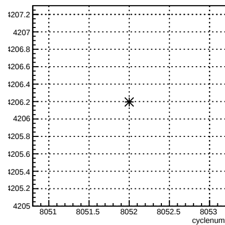
usl_coil4:cyclenum {run == 7114}
