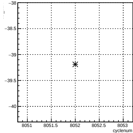
usl_12X:cyclenum {run == 7114}
