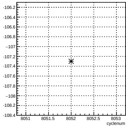
usl_4eY:cyclenum {run == 7114}
