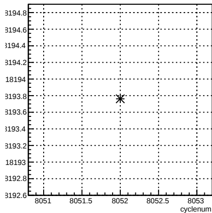
usr_coil7:cyclenum {run == 7114}
