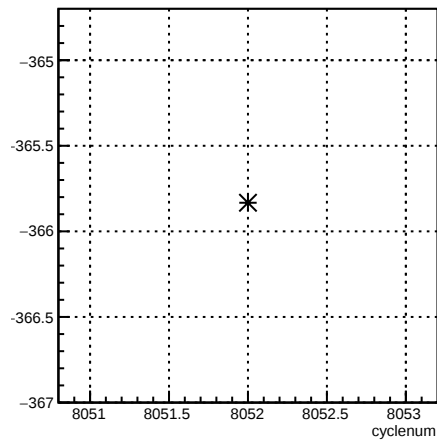
usl_coil6:cyclenum {run == 7114}
