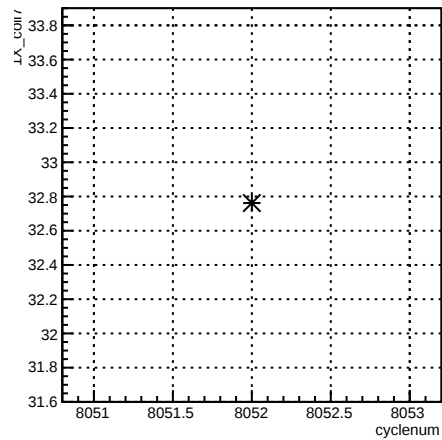
4eX_coil7:cyclenum {run == 7114}
