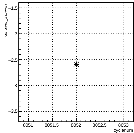
delta46_12X4eY:cyclenum {run == 7114}
