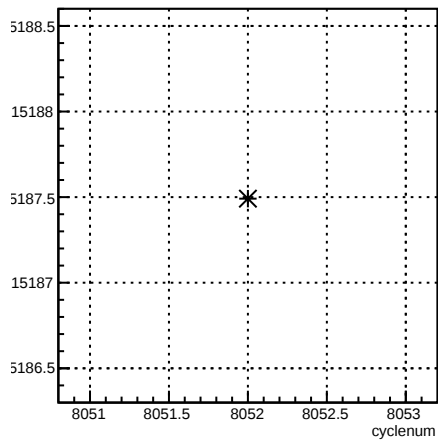
usl_coil7:cyclenum {run == 7114}
