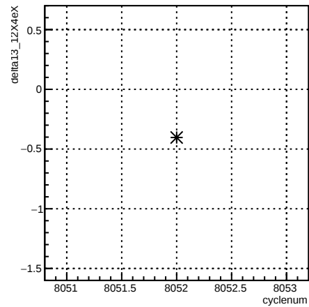
delta13_12X4eX:cyclenum {run == 7114}
