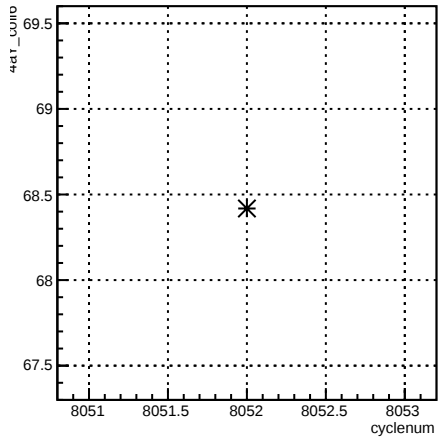
4eY_coil6:cyclenum {run == 7114}
