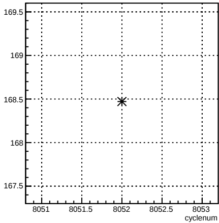
4eY_coil4:cyclenum {run == 7114}
