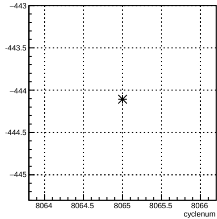
1X_coil1:cyclenum {run == 7120}
