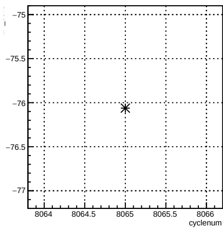
1X_coil3:cyclenum {run == 7120}
