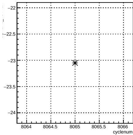
alpha46_4eY4aY:cyclenum {run == 7120}
