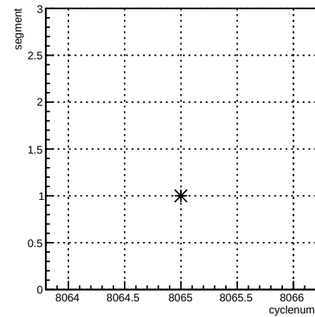
segment:cyclenum {run == 7120}
