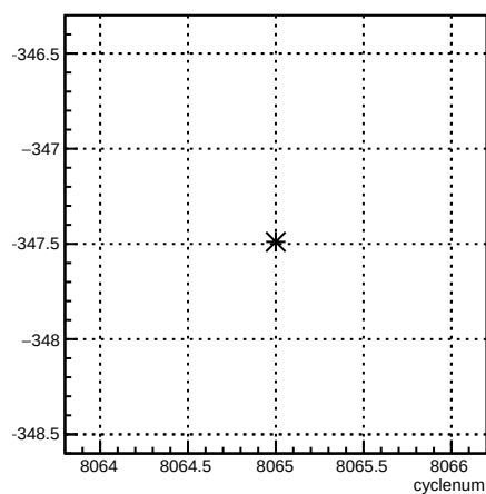
usr_coil6:cyclenum {run == 7120}
