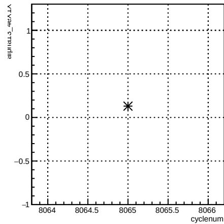
alpha13_4eX1X:cyclenum {run == 7120}
