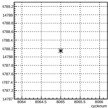
usl_coil7:cyclenum {run == 7120}
