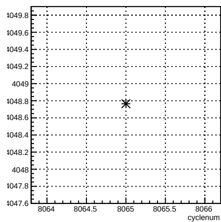
usr_coil4:cyclenum {run == 7120}
