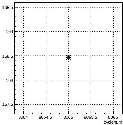
4eY_coil4:cyclenum {run == 7120}
