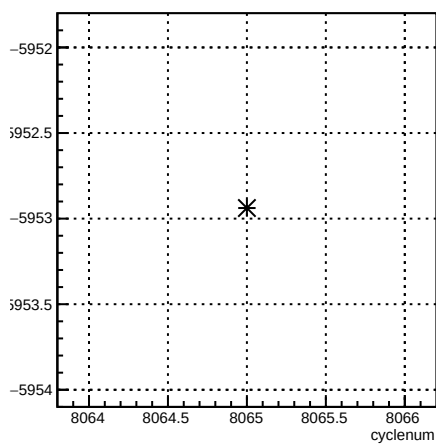
usr_coil3:cyclenum {run == 7120}
