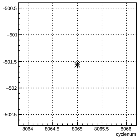
4eX_coil1:cyclenum {run == 7120}
