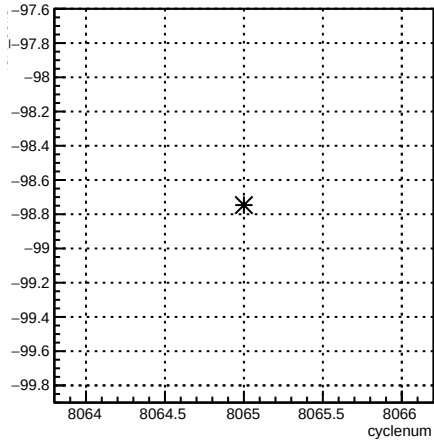
4eX_coil3:cyclenum {run == 7120}
