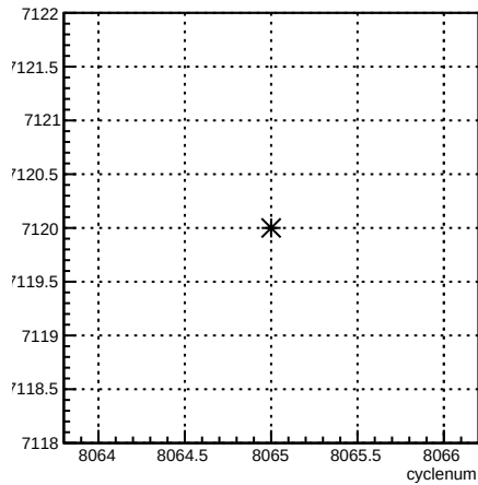
run:cyclenum {run == 7120}
