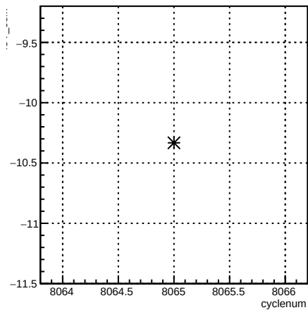
4eY_coil7:cyclenum {run == 7120}
