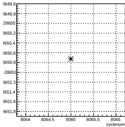
usr_coil1:cyclenum {run == 7120}
