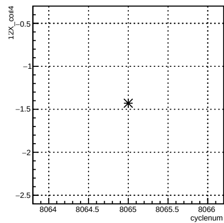
12X_coil4:cyclenum {run == 7120}
