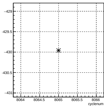
12X_coil7:cyclenum {run == 7120}
