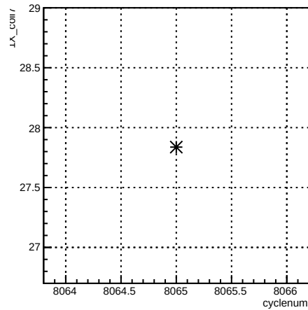
1X_coil7:cyclenum {run == 7120}
