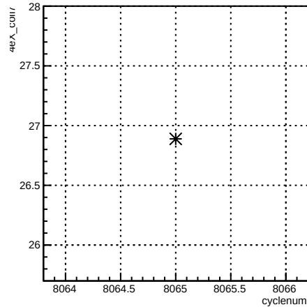
4eX_coil7:cyclenum {run == 7120}
