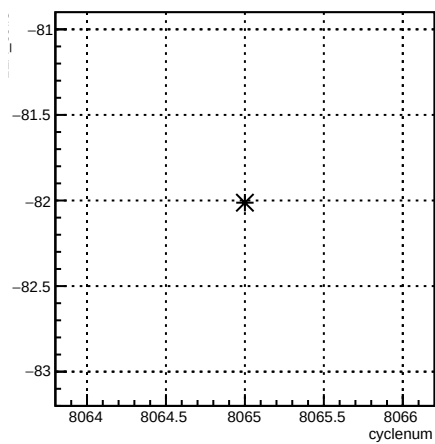
12X_coil3:cyclenum {run == 7120}
