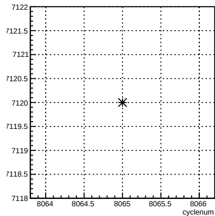
run:cyclenum {run == 7120}
