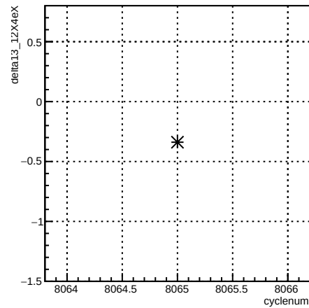
delta13_12X4eX:cyclenum {run == 7120}
