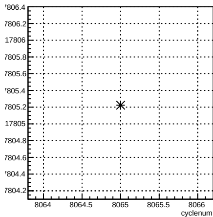
usr_coil7:cyclenum {run == 7120}
