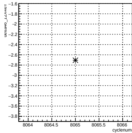
delta46_12X4eY:cyclenum {run == 7120}
