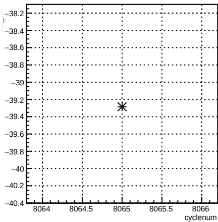
usl_12X:cyclenum {run == 7120}
