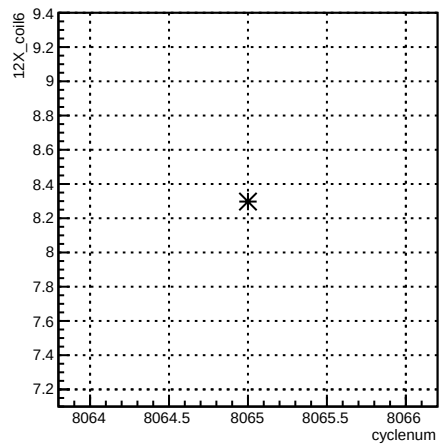
12X_coil6:cyclenum {run == 7120}
