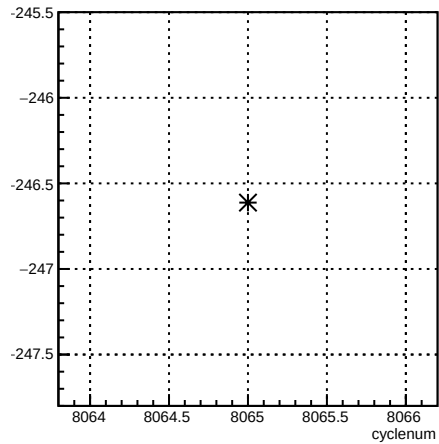
12X_coil1:cyclenum {run == 7120}
