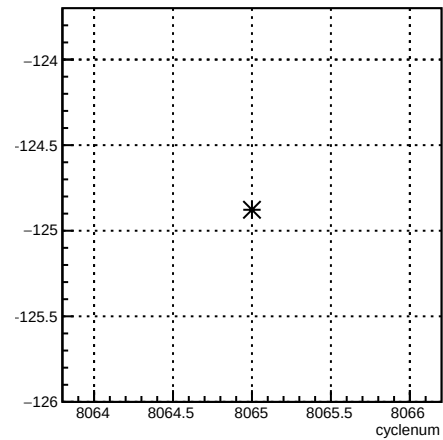
usl_4eY:cyclenum {run == 7120}
