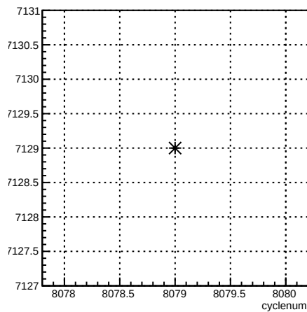
run:cyclenum {run == 7129}
