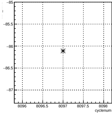
12X_coil7:cyclenum {run == 7140}
