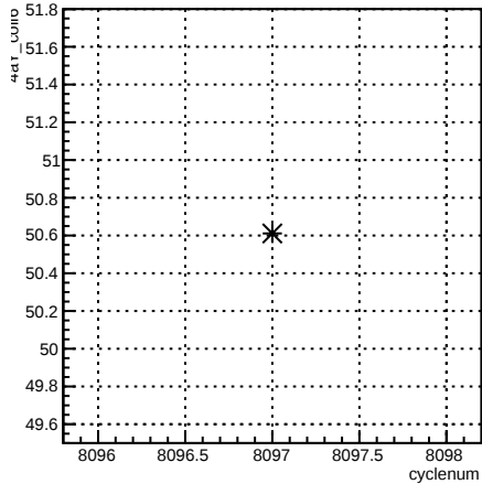
4eY_coil6:cyclenum {run == 7140}
