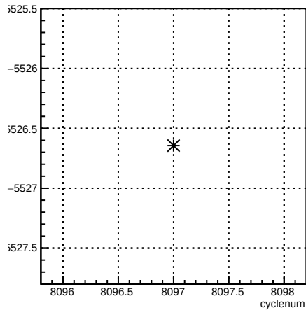
usr_coil3:cyclenum {run == 7140}
