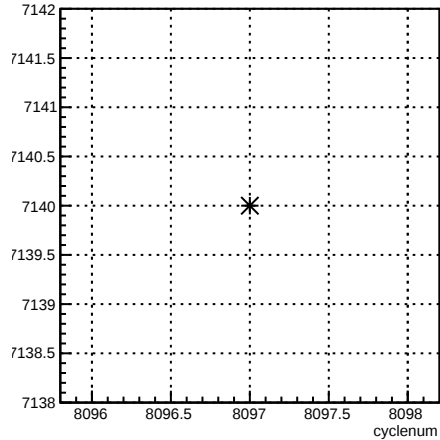
run:cyclenum {run == 7140}
