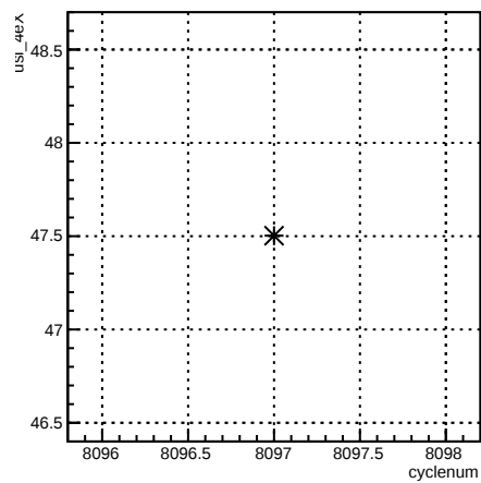
usl_4eX:cyclenum {run == 7140}
