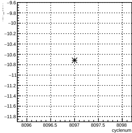
4eY_coil7:cyclenum {run == 7140}
