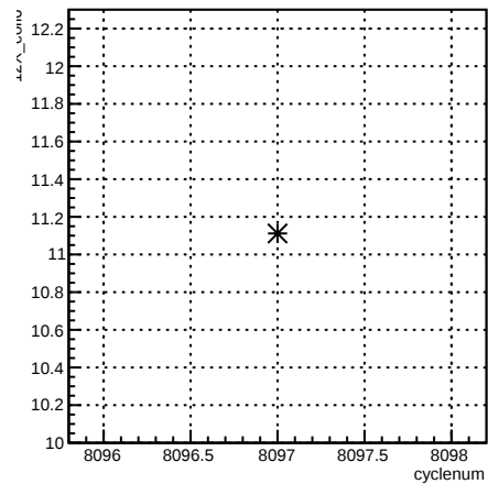
12X_coil6:cyclenum {run == 7140}
