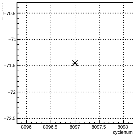
4eX_coil3:cyclenum {run == 7140}
