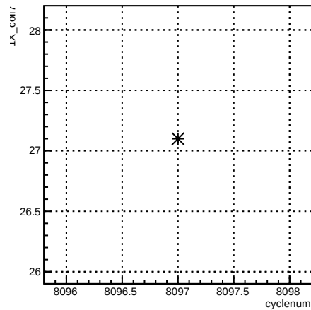
4eX_coil7:cyclenum {run == 7140}
