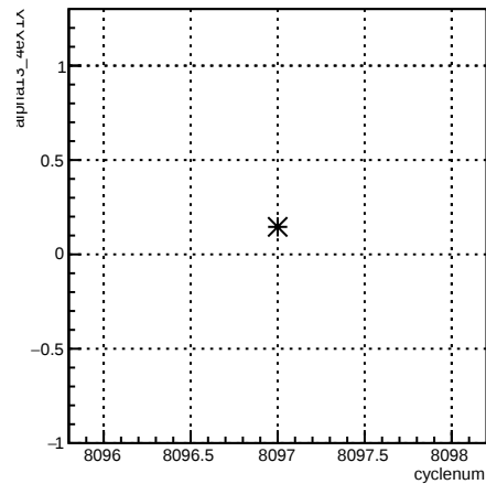
alpha13_4eX1X:cyclenum {run == 7140}
