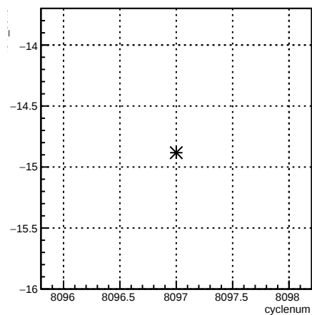
4eY_coil6:cyclenum {run == 7140}
