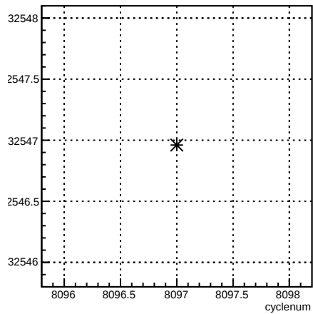
usl_coil6:cyclenum {run == 7140}
