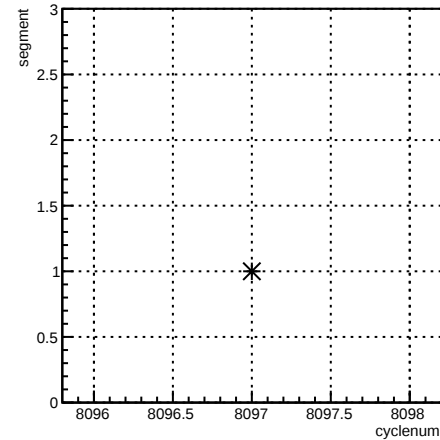
segment:cyclenum {run == 7140}
