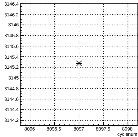
usr_coil4:cyclenum {run == 7140}
