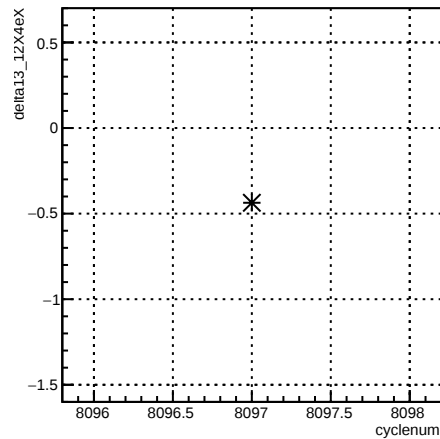
delta13_12X4eX:cyclenum {run == 7140}
