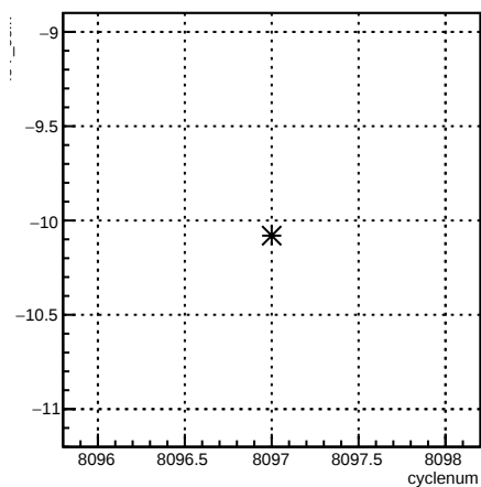
4eY_coil7:cyclenum {run == 7140}
