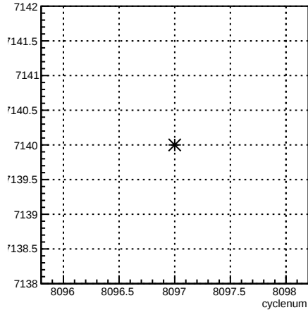
run:cyclenum {run == 7140}
