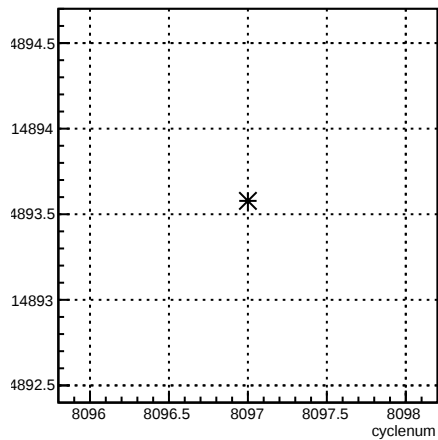
usl_coil7:cyclenum {run == 7140}
