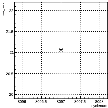
usl_4eY:cyclenum {run == 7140}
