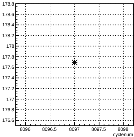
4eY_coil4:cyclenum {run == 7140}
