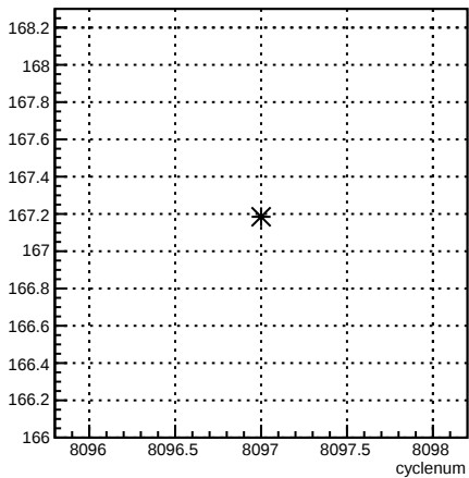
4eY_coil4:cyclenum {run == 7140}
