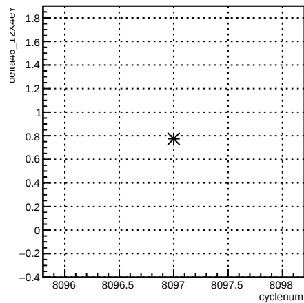
delta46_12X4eY:cyclenum {run == 7140}
