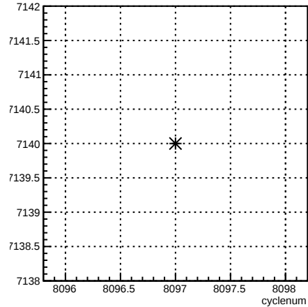
run:cyclenum {run == 7140}
