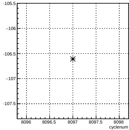
usl_1X:cyclenum {run == 7140}
