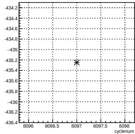
4eX_coil1:cyclenum {run == 7140}
