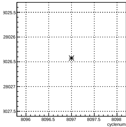
usr_coil1:cyclenum {run == 7140}
