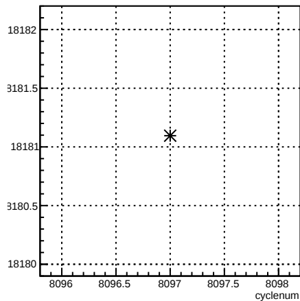
usr_coil7:cyclenum {run == 7140}
