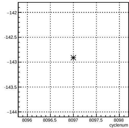
usr_4eY:cyclenum {run == 7140}
