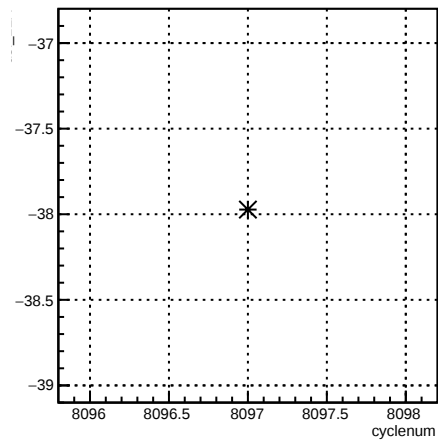
usl_12X:cyclenum {run == 7140}
