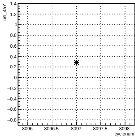
usl_4aY:cyclenum {run == 7140}
