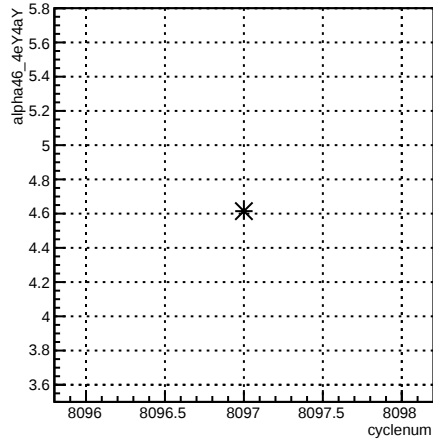
alpha46_4eY4aY:cyclenum {run == 7140}
