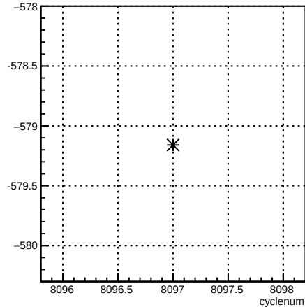
usr_coil6:cyclenum {run == 7140}
