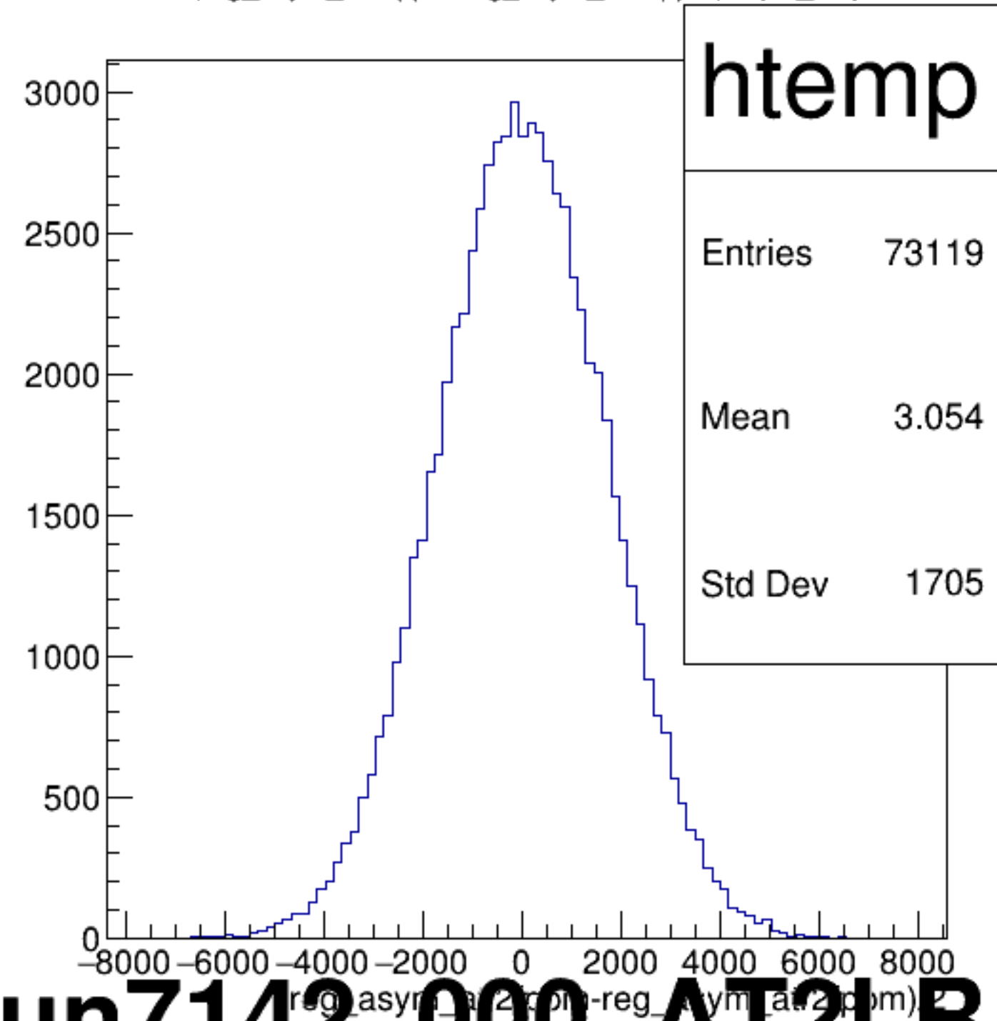
(reg_asym_atl2/ppm-reg_asym_atr2/ppm)/2 {ok_cut}
