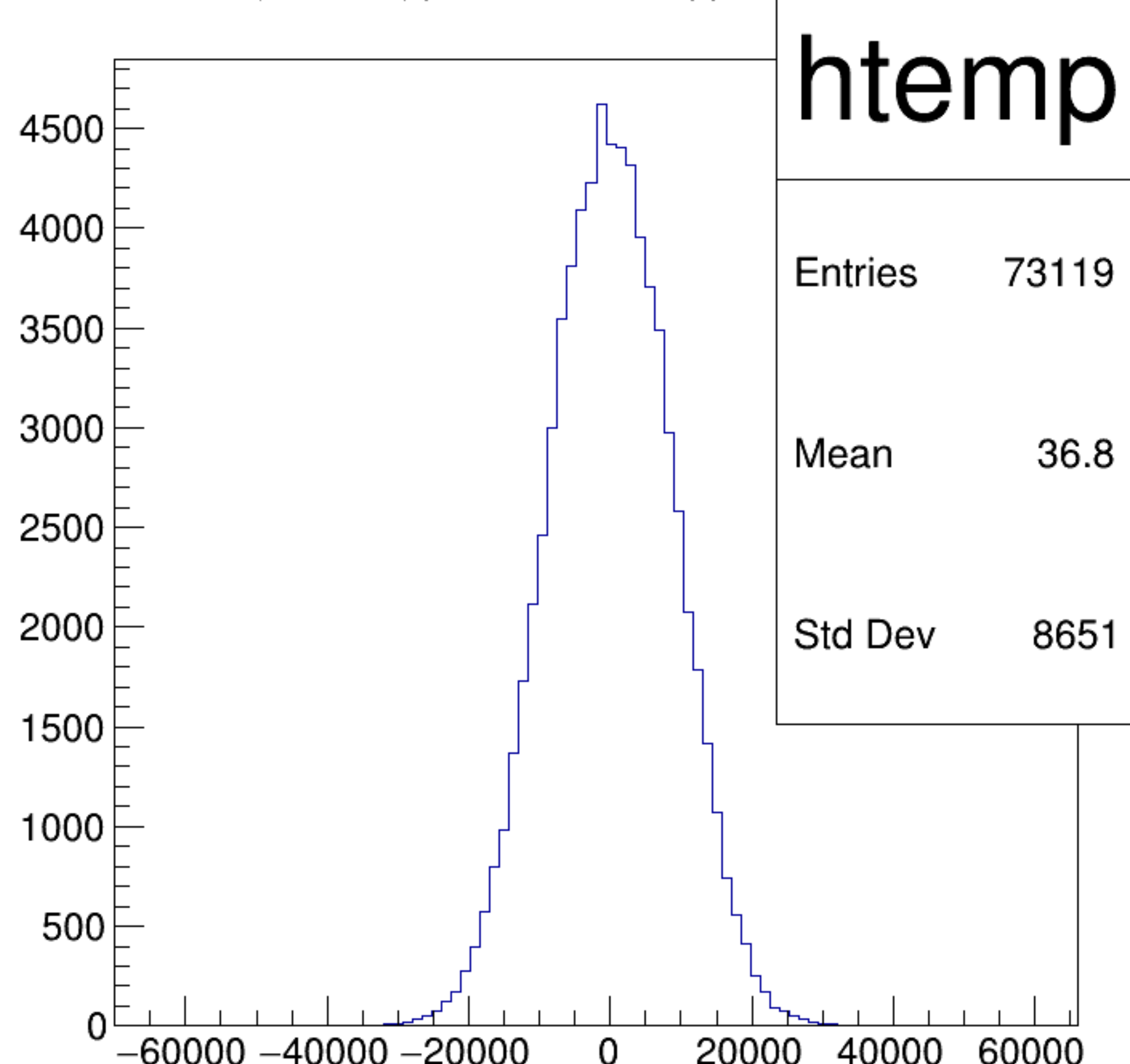
(asym_atl2/ppm+asym_atr2/ppm)/2 {ok_cut}
