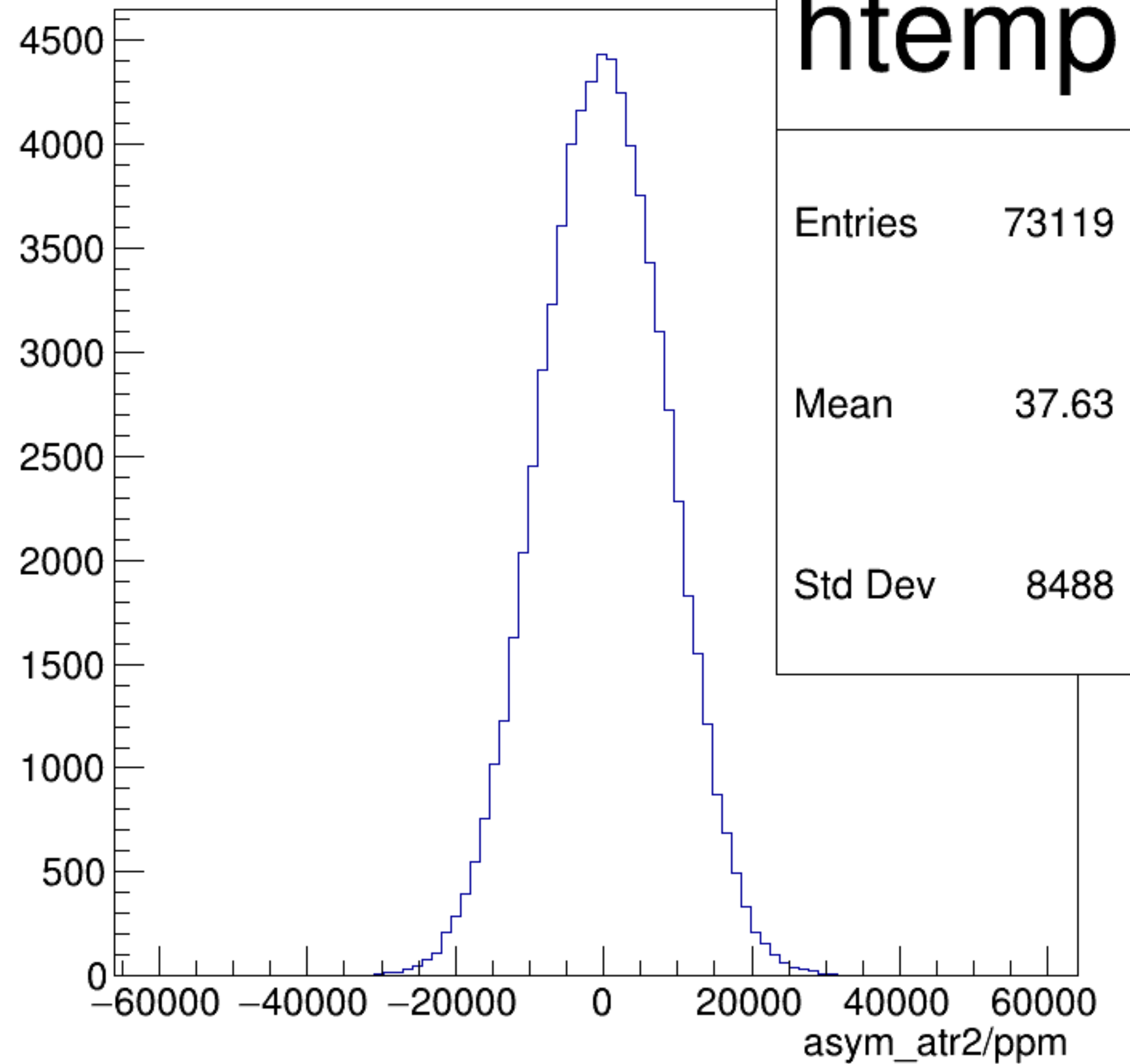
asym_atr2/ppm {ok_cut}
