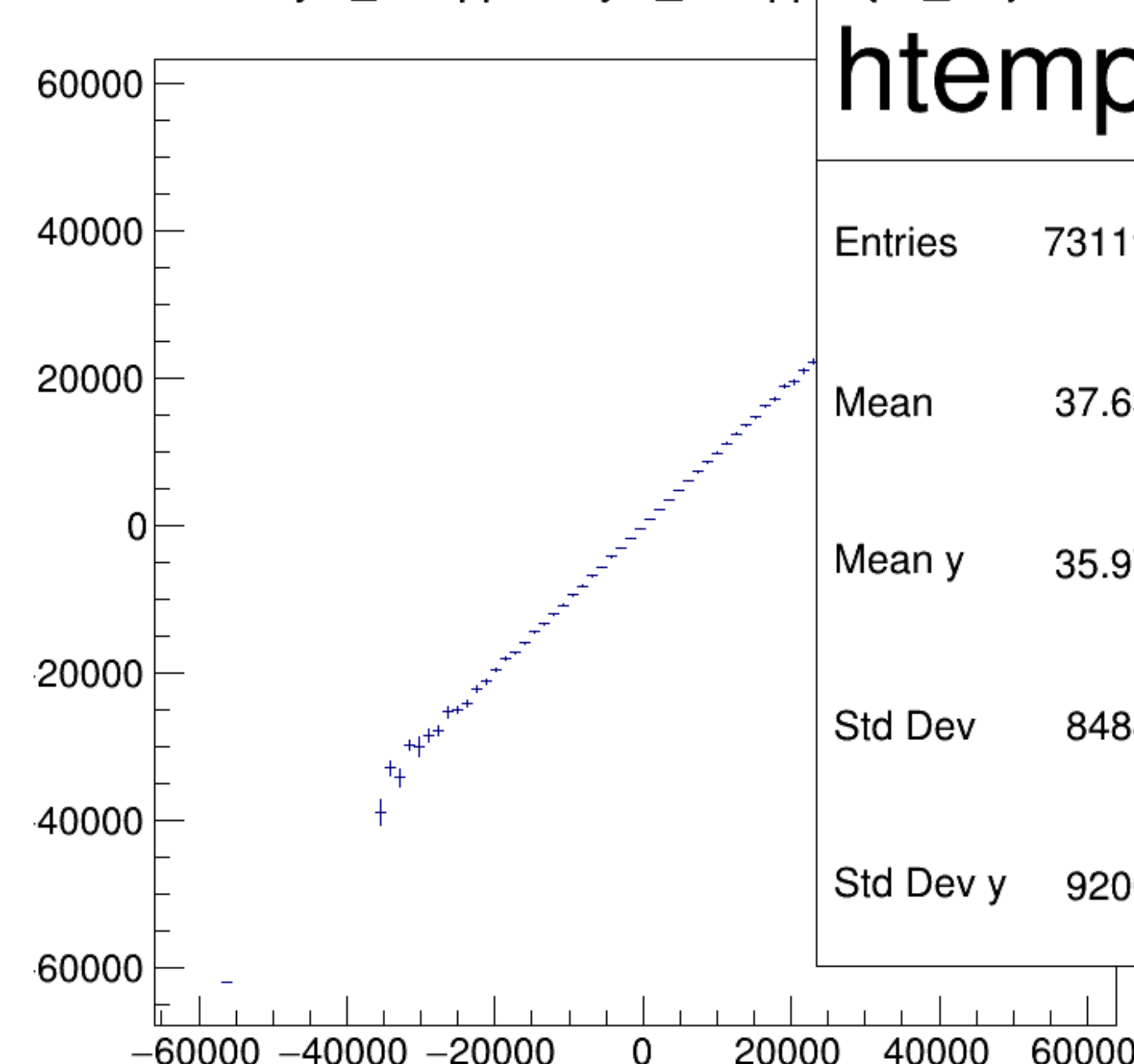
asym_atl2/ppm:asym_atr2/ppm {ok_cut}
