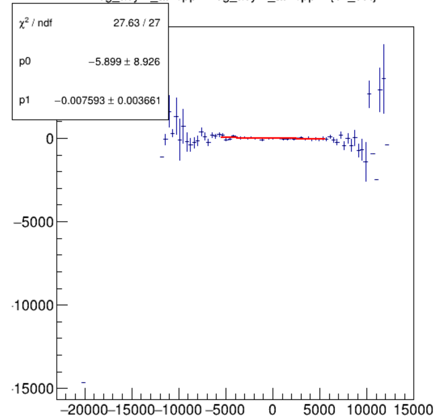
reg_asym_atl1/ppm:reg_asym_atr1/ppm {ok_cut}
