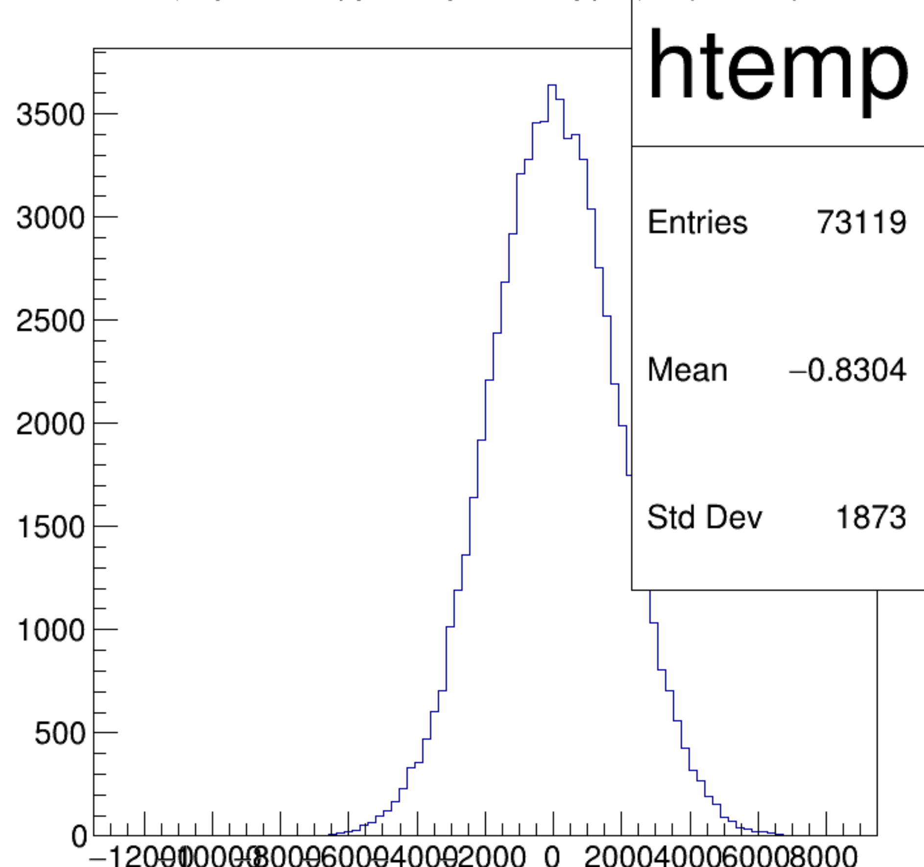
(asym_atl2/ppm-asym_atr2/ppm)/2 {ok_cut}
