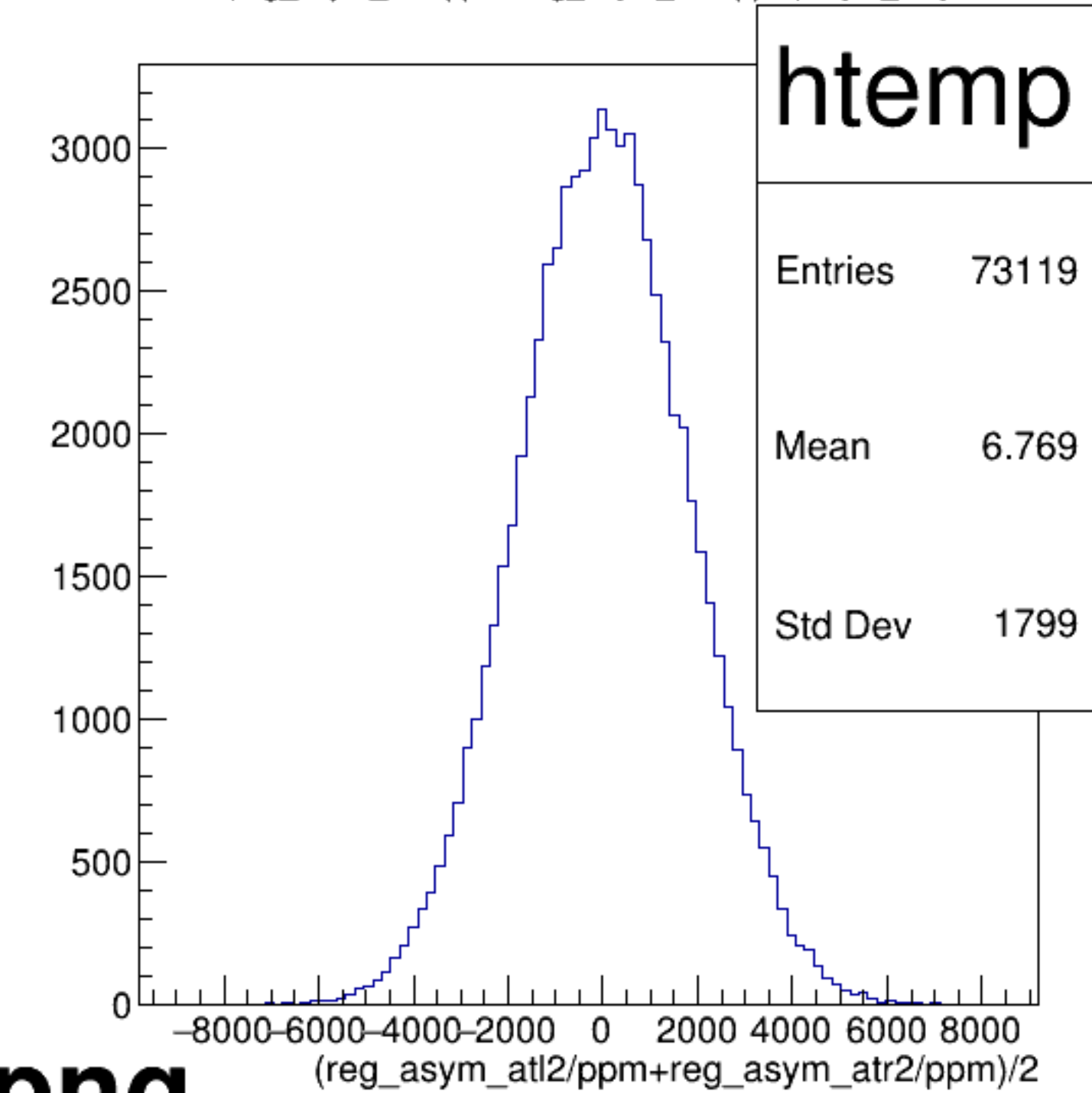
(reg_asym_atl2/ppm+reg_asym_atr2/ppm)/2 {ok_cut}
