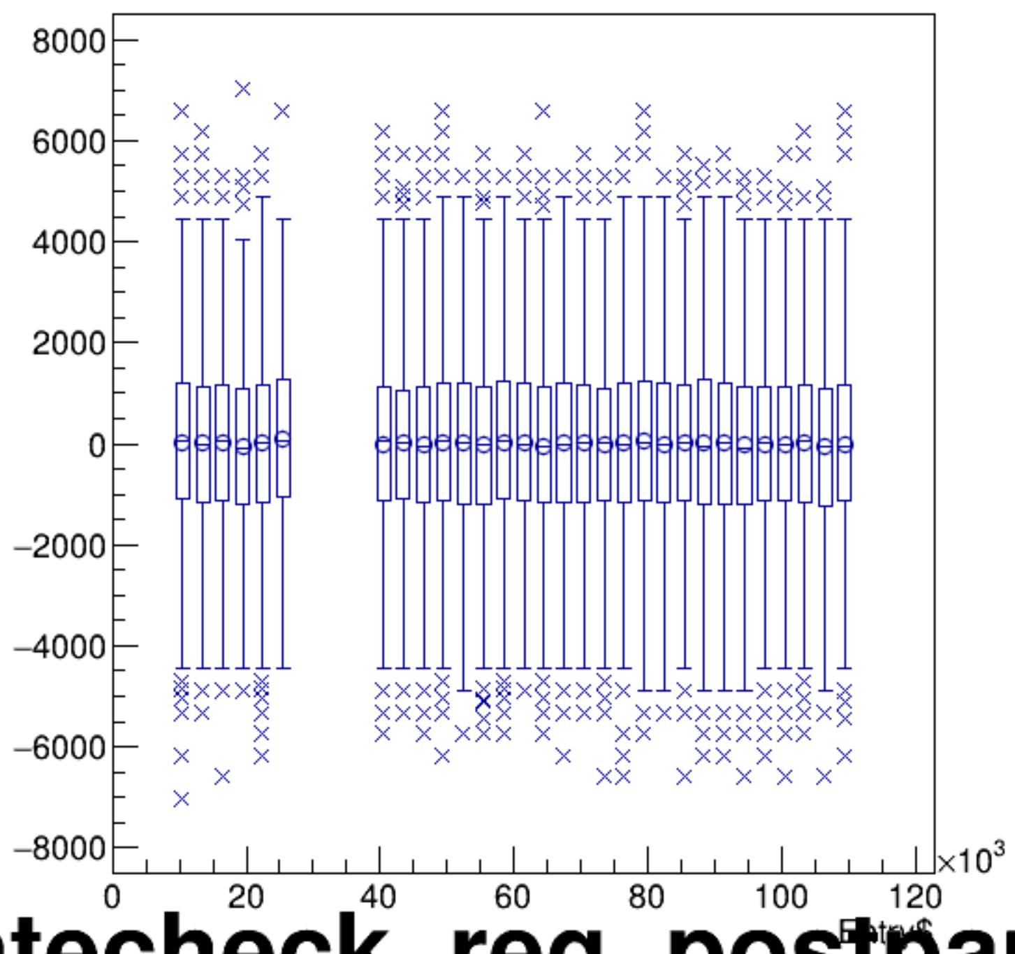
(reg_asym_atl2/ppm-reg_asym_atr2/ppm)/2:Entry$ {ok_cut}
