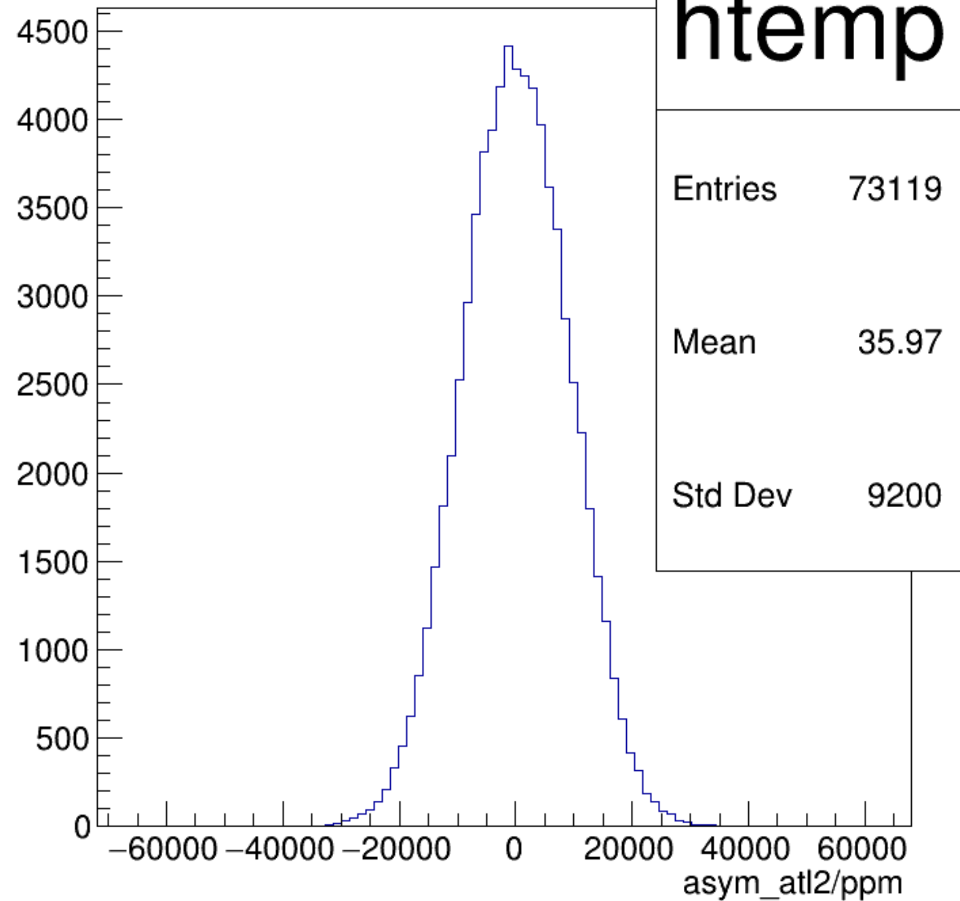
asym_atl2/ppm {ok_cut}
