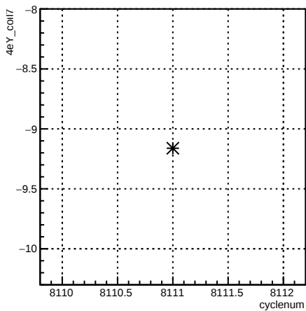
4eY_coil7:cyclenum {run == 7143}
