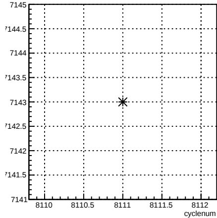
run:cyclenum {run == 7143}
