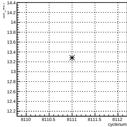
usr_4eY:cyclenum {run == 7143}
