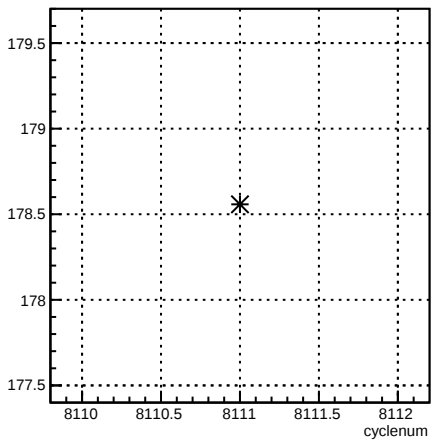
4eY_coil4:cyclenum {run == 7143}
