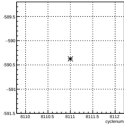
usr_coil6:cyclenum {run == 7143}
