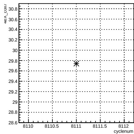
4eX_coil7:cyclenum {run == 7143}
