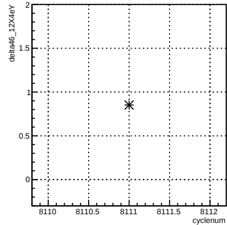
delta46_12X4eY:cyclenum {run == 7143}
