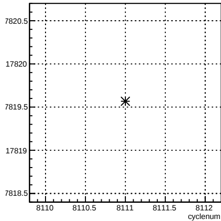
usr_coil7:cyclenum {run == 7143}
