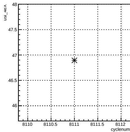
usl_4eX:cyclenum {run == 7143}
