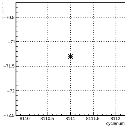
4eX_coil3:cyclenum {run == 7143}
