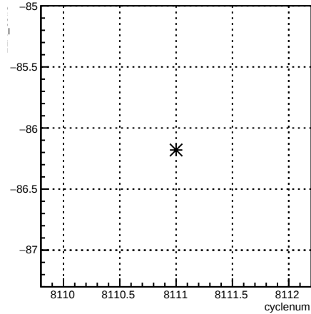
12X_coil7:cyclenum {run == 7143}
