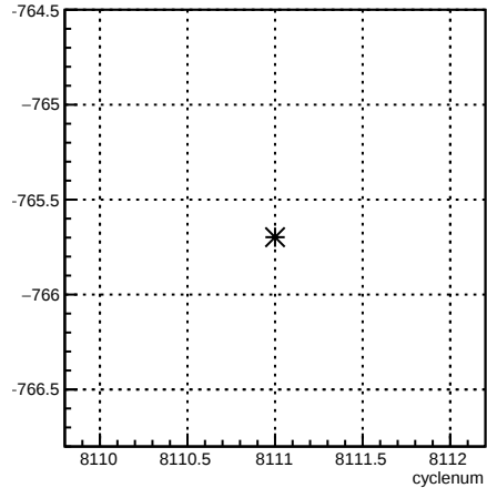
usl_coil6:cyclenum {run == 7143}
