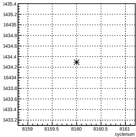
usl_coil7:cyclenum {run == 7153}
