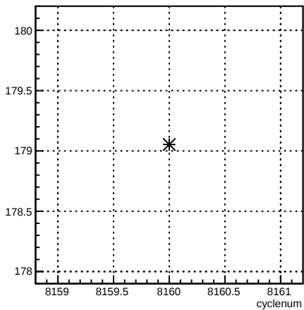
4eY_coil4:cyclenum {run == 7153}
