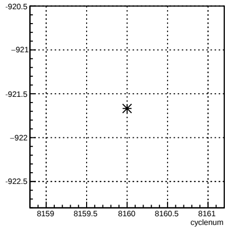
usl_coil6:cyclenum {run == 7153}
