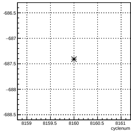
usr_coil6:cyclenum {run == 7153}
