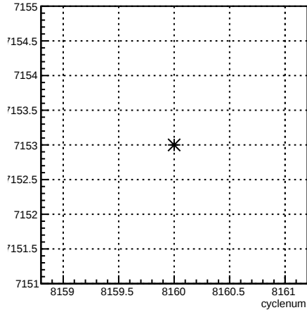
run:cyclenum {run == 7153}
