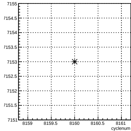
run:cyclenum {run == 7153}
