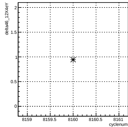
delta46_12X4eY:cyclenum {run == 7153}
