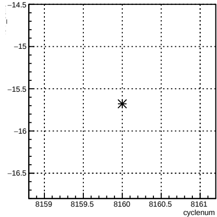
4eY_coil6:cyclenum {run == 7153}
