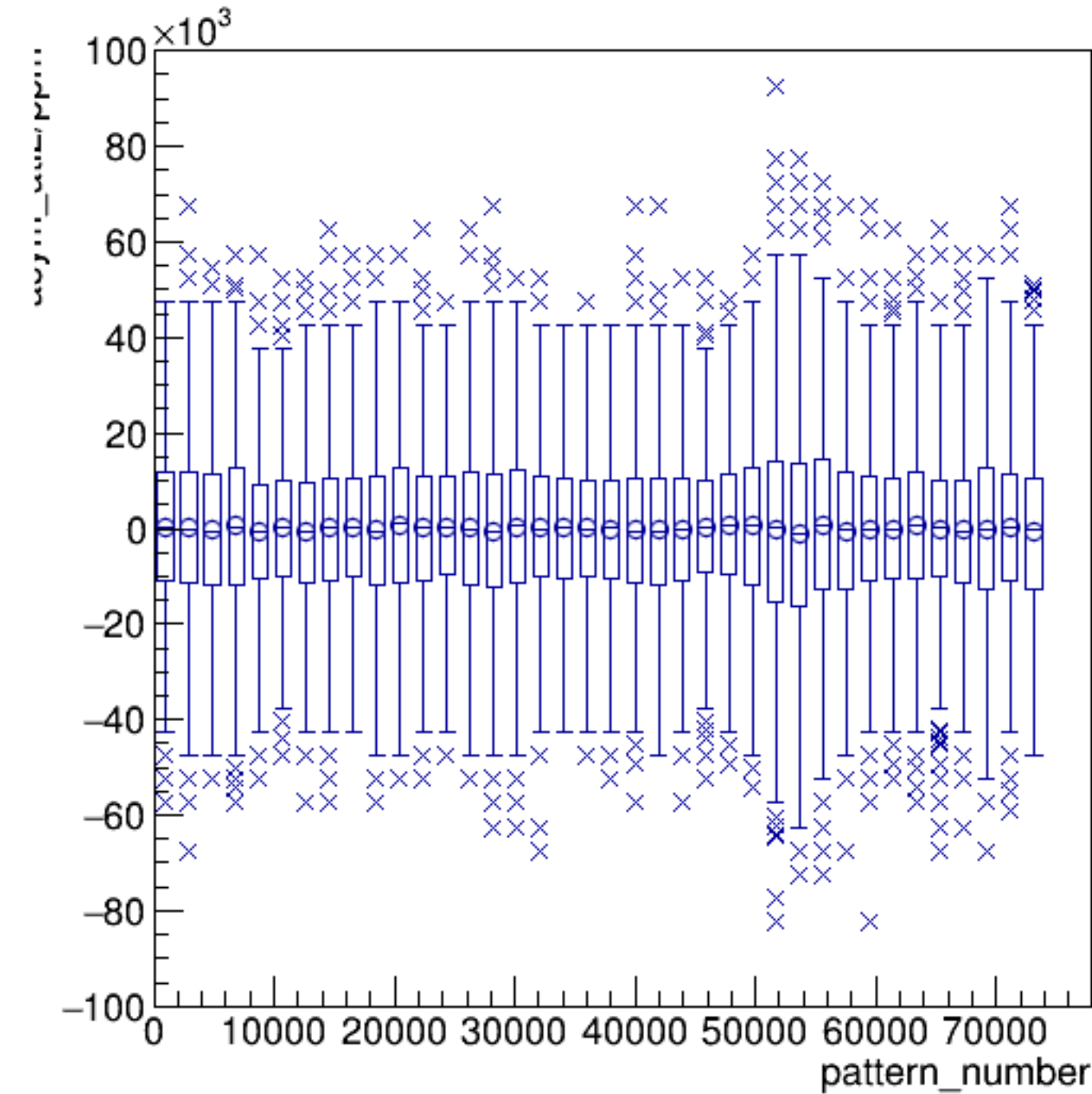
asym_atl2/ppm:pattern_number {ErrorFlag==0}
