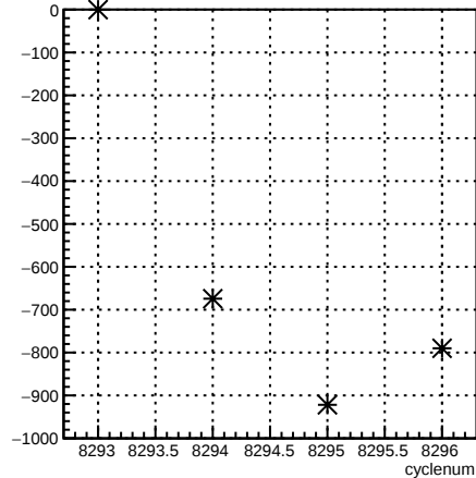
usr_coil6:cyclenum {run == 7185}
