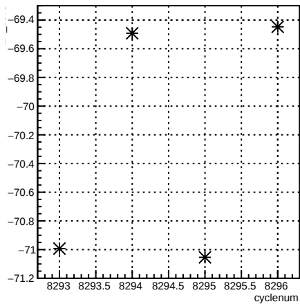
4eX_coil3:cyclenum {run == 7185}
