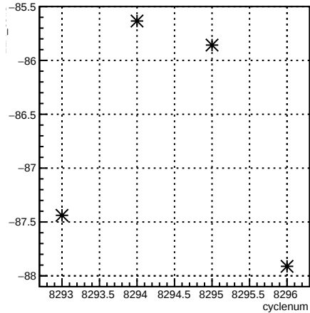
12X_coil3:cyclenum {run == 7185}
