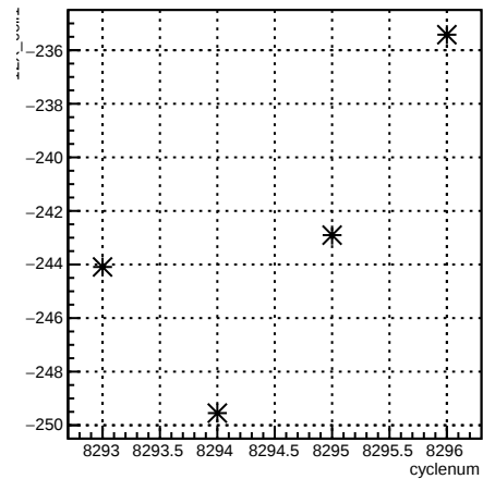
12X_coil1:cyclenum {run == 7185}
