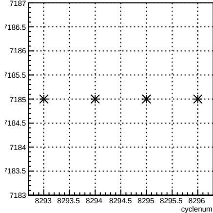
run:cyclenum {run == 7185}
