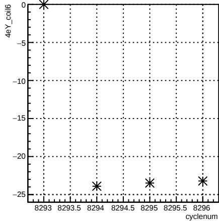
4eY_coil6:cyclenum {run == 7185}
