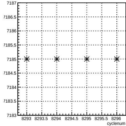
run:cyclenum {run == 7185}
