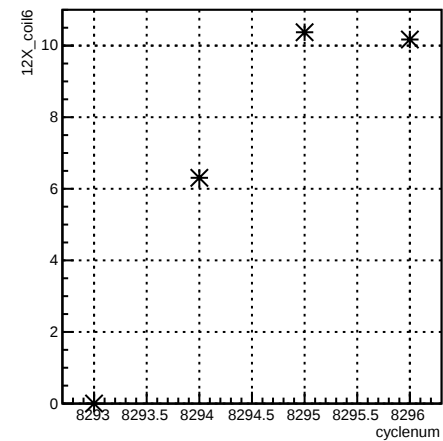
12X_coil6:cyclenum {run == 7185}
