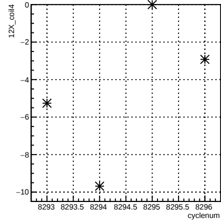
12X_coil4:cyclenum {run == 7185}
