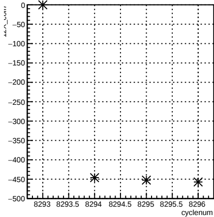
12X_coil7:cyclenum {run == 7185}
