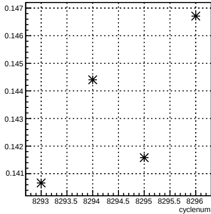
delta46_12X4eY:cyclenum {run == 7185}
