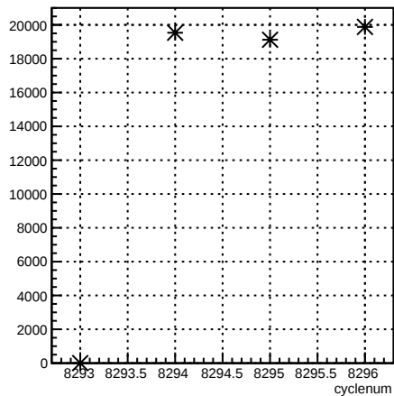
usr_coil7:cyclenum {run == 7185}
