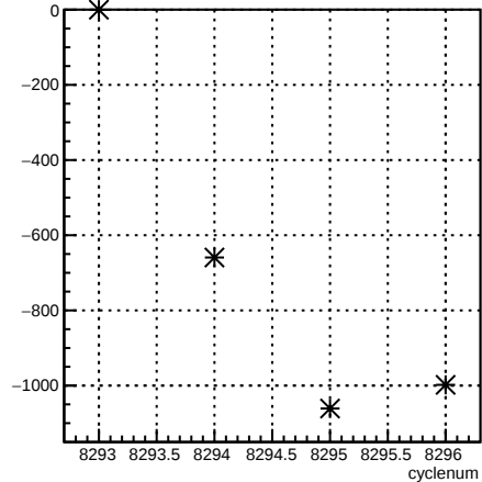
usl_coil6:cyclenum {run == 7185}
