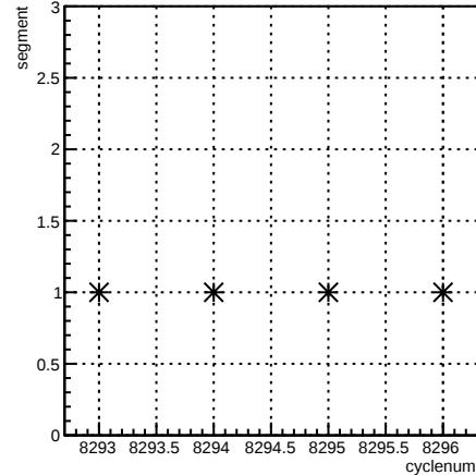
segment:cyclenum {run == 7185}
