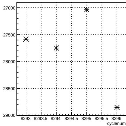
usr_coil1:cyclenum {run == 7185}
