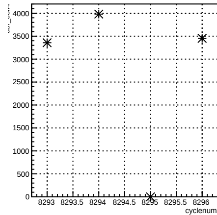
usr_coil4:cyclenum {run == 7185}
