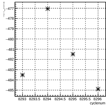
4eX_coil1:cyclenum {run == 7185}
