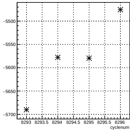
usr_coil3:cyclenum {run == 7185}
