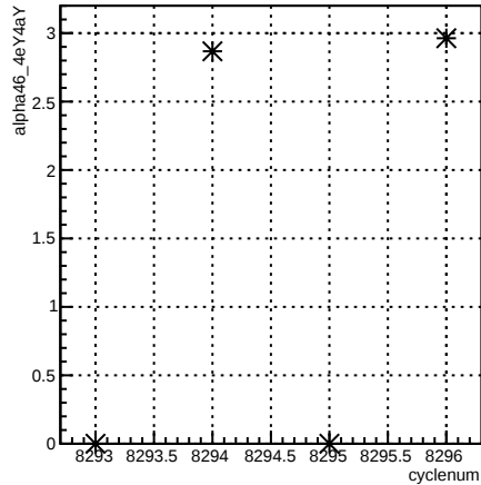
run:cyclenum {run == 7185}
