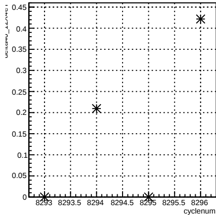
delta46_12X4eY:cyclenum {run == 7185}
