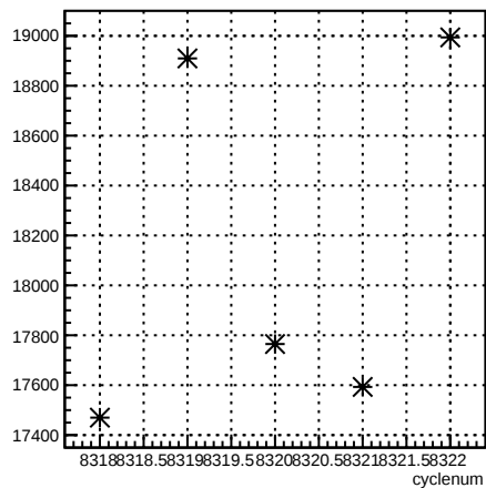
usr_coil7:cyclenum {run == 7190}
