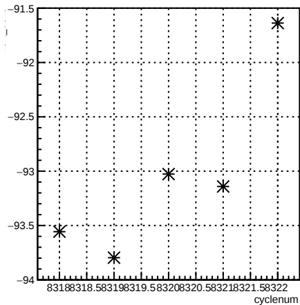
4eX_coil3:cyclenum {run == 7190}
