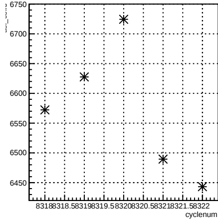
usl_coil7:cyclenum {run == 7190}
