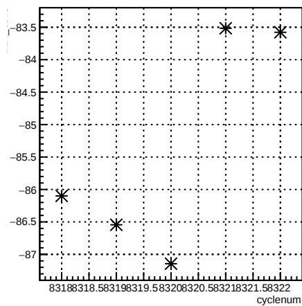
12X_coil3:cyclenum {run == 7190}
