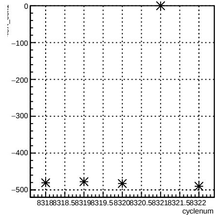
4eX_coil1:cyclenum {run == 7190}
