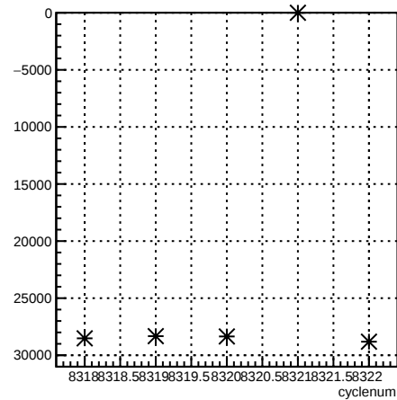
usr_coil1:cyclenum {run == 7190}
