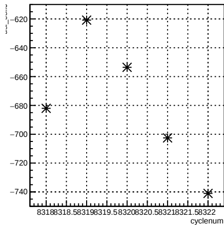
usl_coil6:cyclenum {run == 7190}
