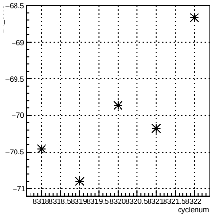
1X_coil3:cyclenum {run == 7190}
