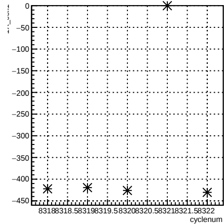
1X_coil1:cyclenum {run == 7190}
