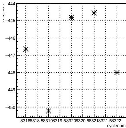
12X_coil7:cyclenum {run == 7190}
