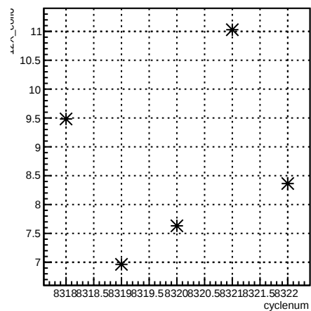
12X_coil6:cyclenum {run == 7190}
