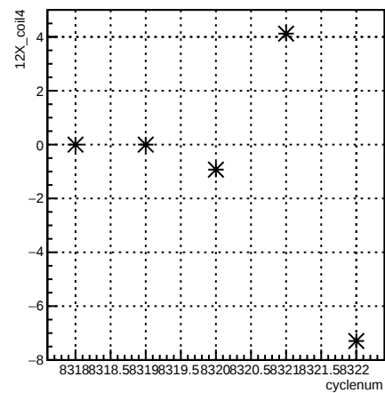
12X_coil4:cyclenum {run == 7190}
