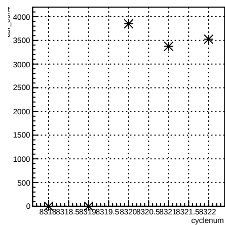
usr_coil4:cyclenum {run == 7190}
