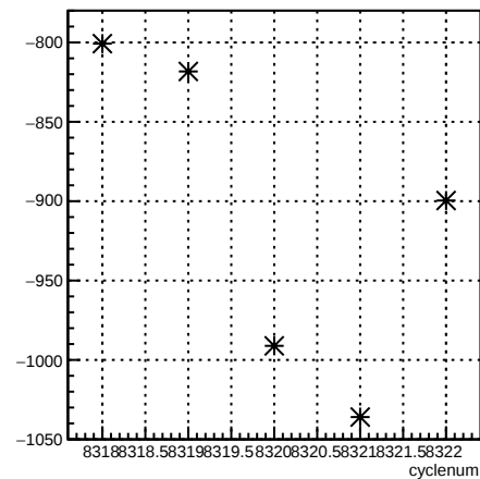
usr_coil6:cyclenum {run == 7190}
