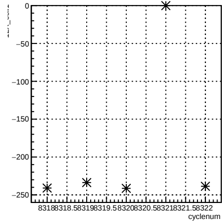
12X_coil1:cyclenum {run == 7190}
