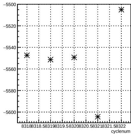
usr_coil3:cyclenum {run == 7190}
