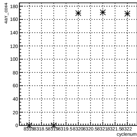
4eY_coil4:cyclenum {run == 7190}
