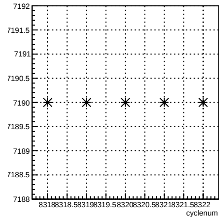
run:cyclenum {run == 7190}
