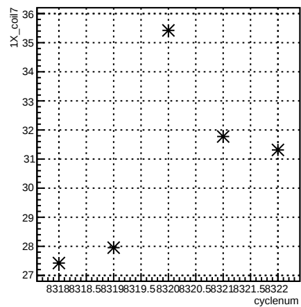
1X_coil7:cyclenum {run == 7190}
