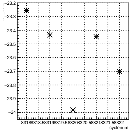
4eY_coil6:cyclenum {run == 7190}
