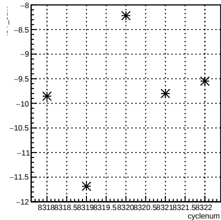
4eY_coil7:cyclenum {run == 7190}
