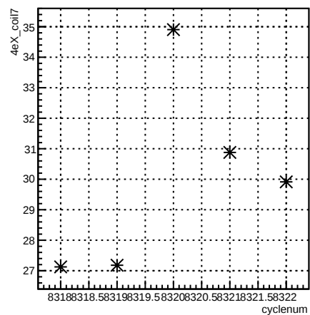
4eX_coil7:cyclenum {run == 7190}
