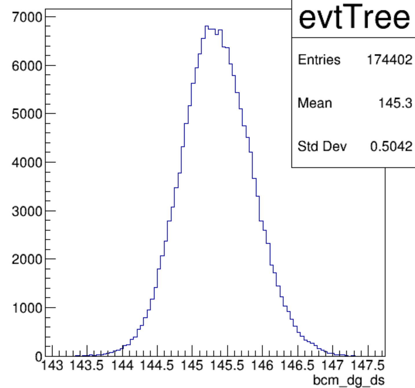
bcm_dg_ds {ErrorFlag==0}
