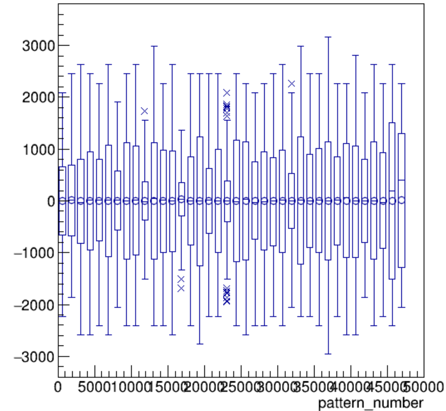
asym_bcm_an_ds3/ppm:pattern_number {ErrorFlag==0}
