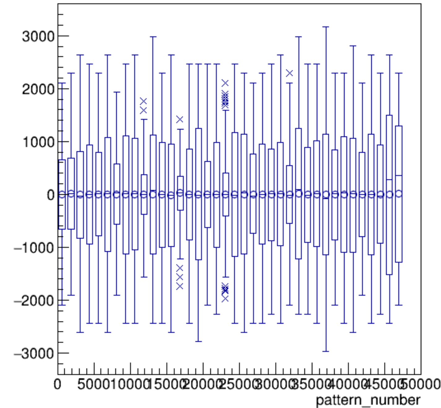
asym_bcm_an_ds/ppm:pattern_number {ErrorFlag==0}
