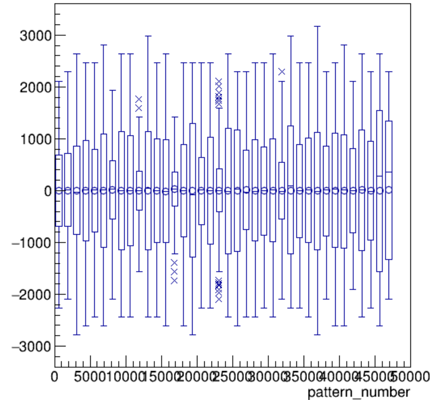
asym_bcm_dg_ds/ppm:pattern_number {ErrorFlag==0}
