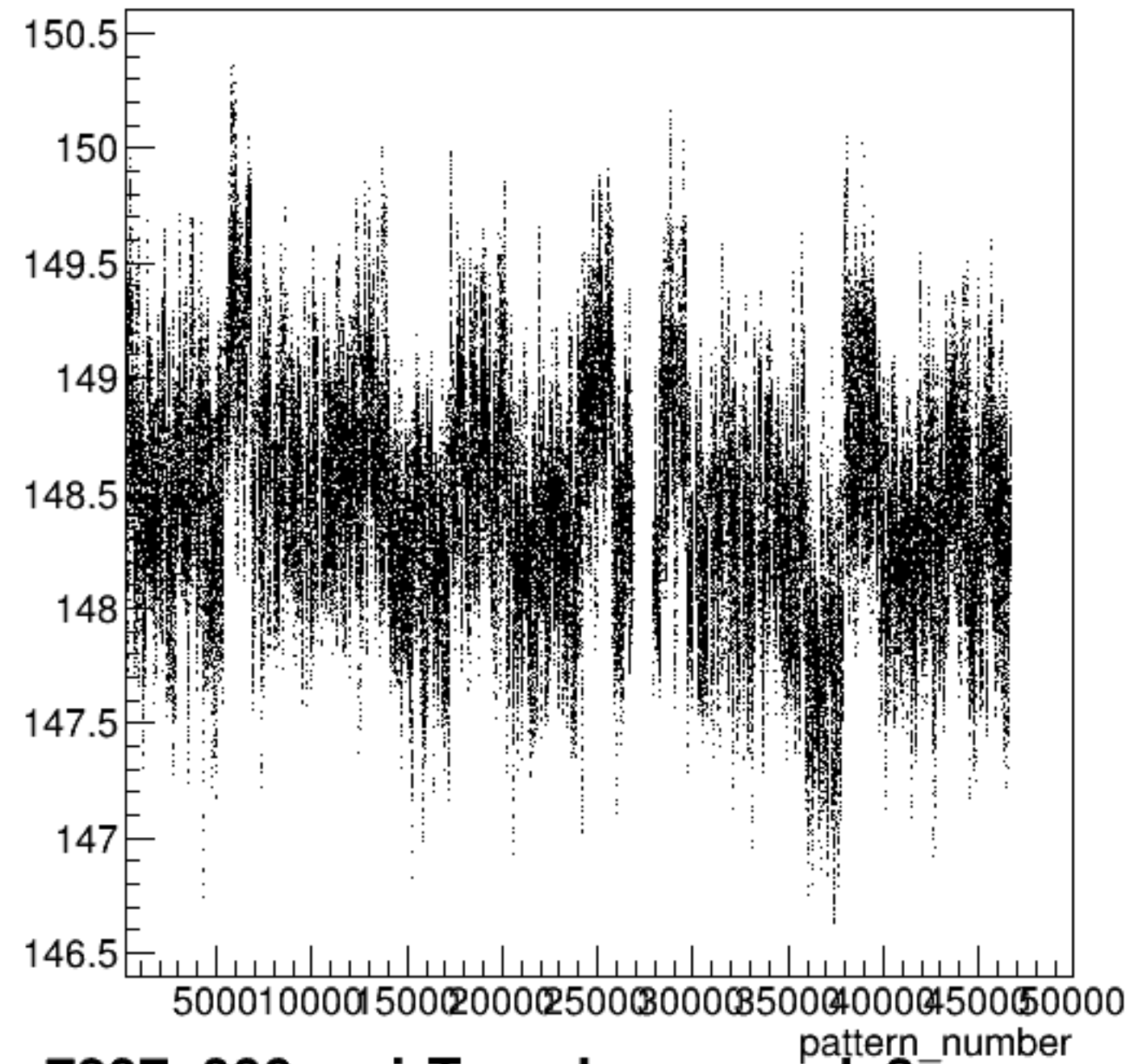
yield_bcm_an_ds3:pattern_number {ErrorFlag==0}
