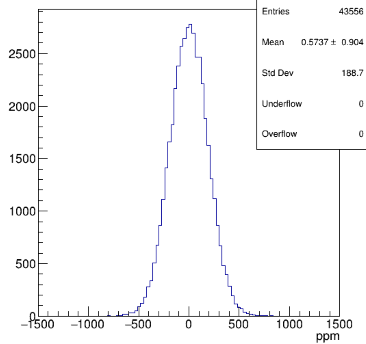
asym_bcm_dg_us
