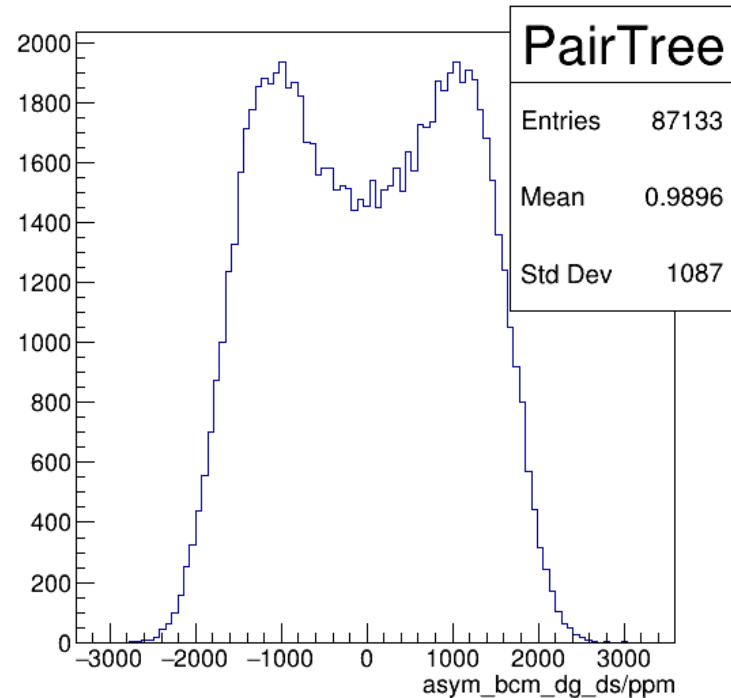
asym_bcm_dg_ds/ppm {ErrorFlag==0}
