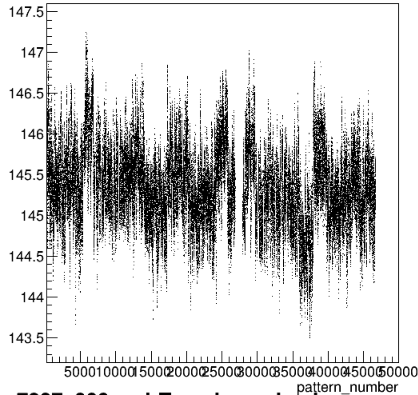
yield_bcm_dg_ds:pattern_number {ErrorFlag==0}
