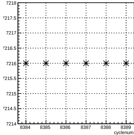
run:cyclenum {run == 7216}
