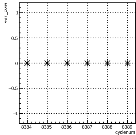
4eY_coil4:cyclenum {run == 7216}
