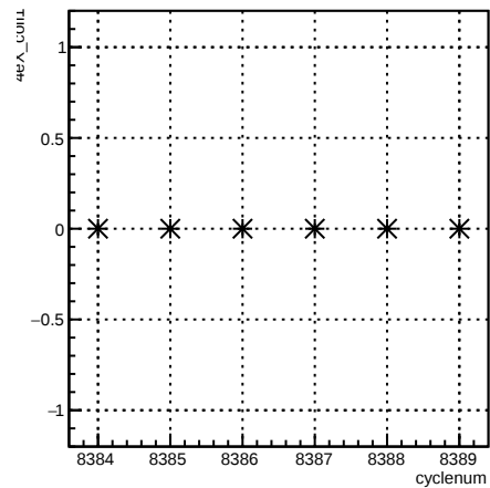
4eX_coil1:cyclenum {run == 7216}
