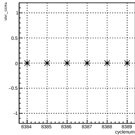
usr_coil6:cyclenum {run == 7216}
