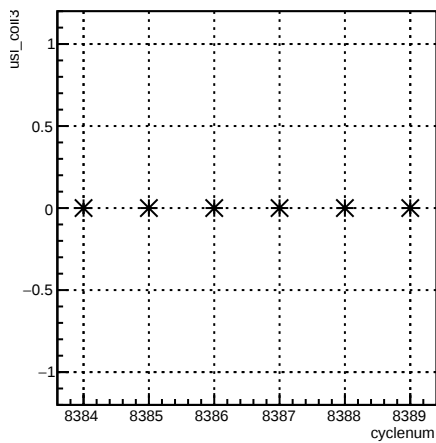
usl_coil3:cyclenum {run == 7216}
