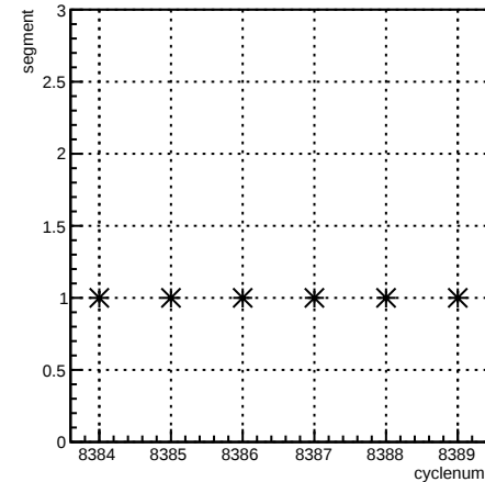
segment:cyclenum {run == 7216}
