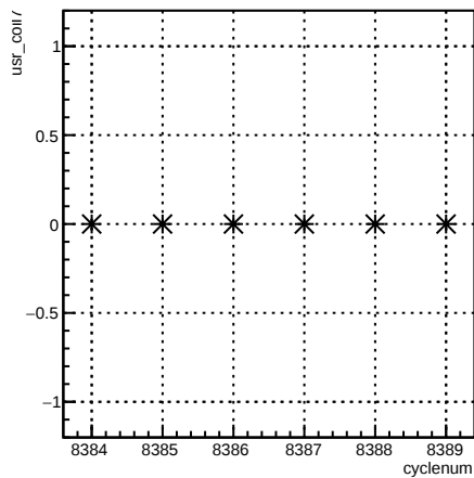
usr_coil7:cyclenum {run == 7216}
