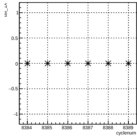
usl_4eY:cyclenum {run == 7216}
