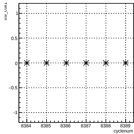
usl_coil1:cyclenum {run == 7216}
