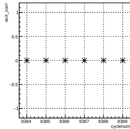
4eX_coil7:cyclenum {run == 7216}
