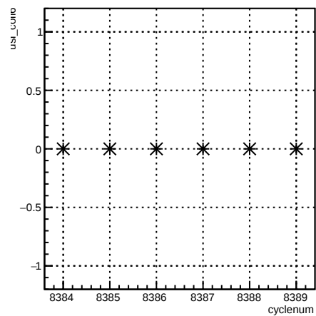
usl_coil6:cyclenum {run == 7216}
