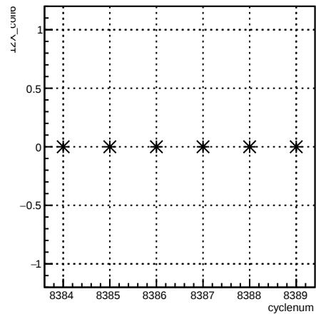
12X_coil6:cyclenum {run == 7216}
