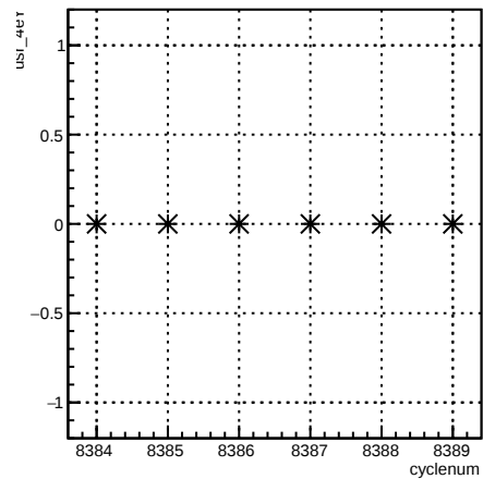
usr_4eY:cyclenum {run == 7216}
