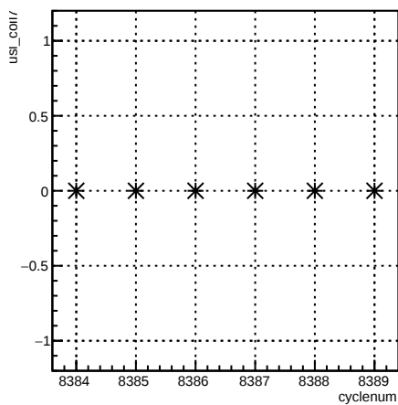
usl_coil7:cyclenum {run == 7216}
