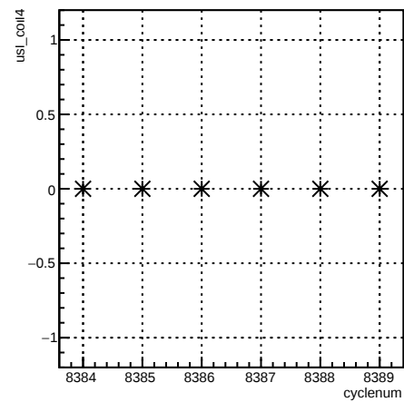
usl_coil4:cyclenum {run == 7216}
