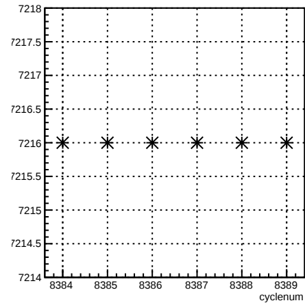
run:cyclenum {run == 7216}
