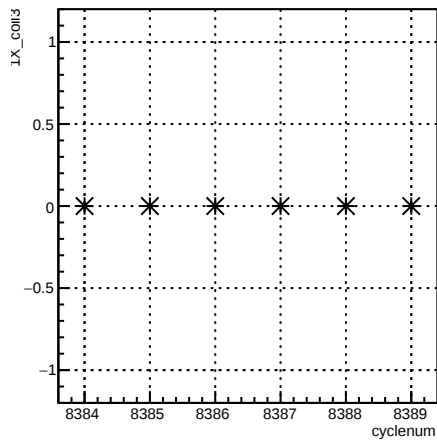
4eX_coil3:cyclenum {run == 7216}
