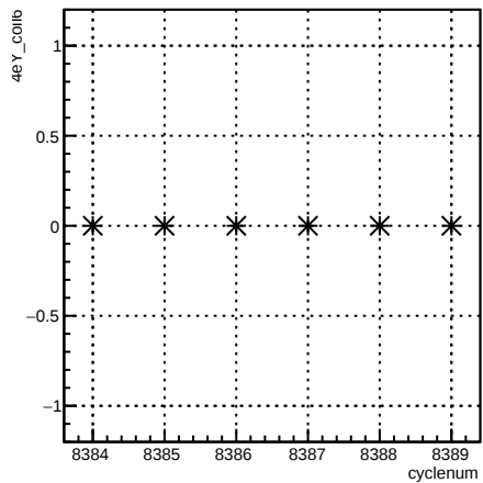
4eY_coil6:cyclenum {run == 7216}
