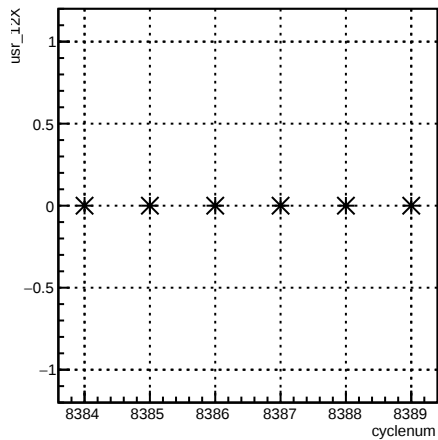
usr_12X:cyclenum {run == 7216}
