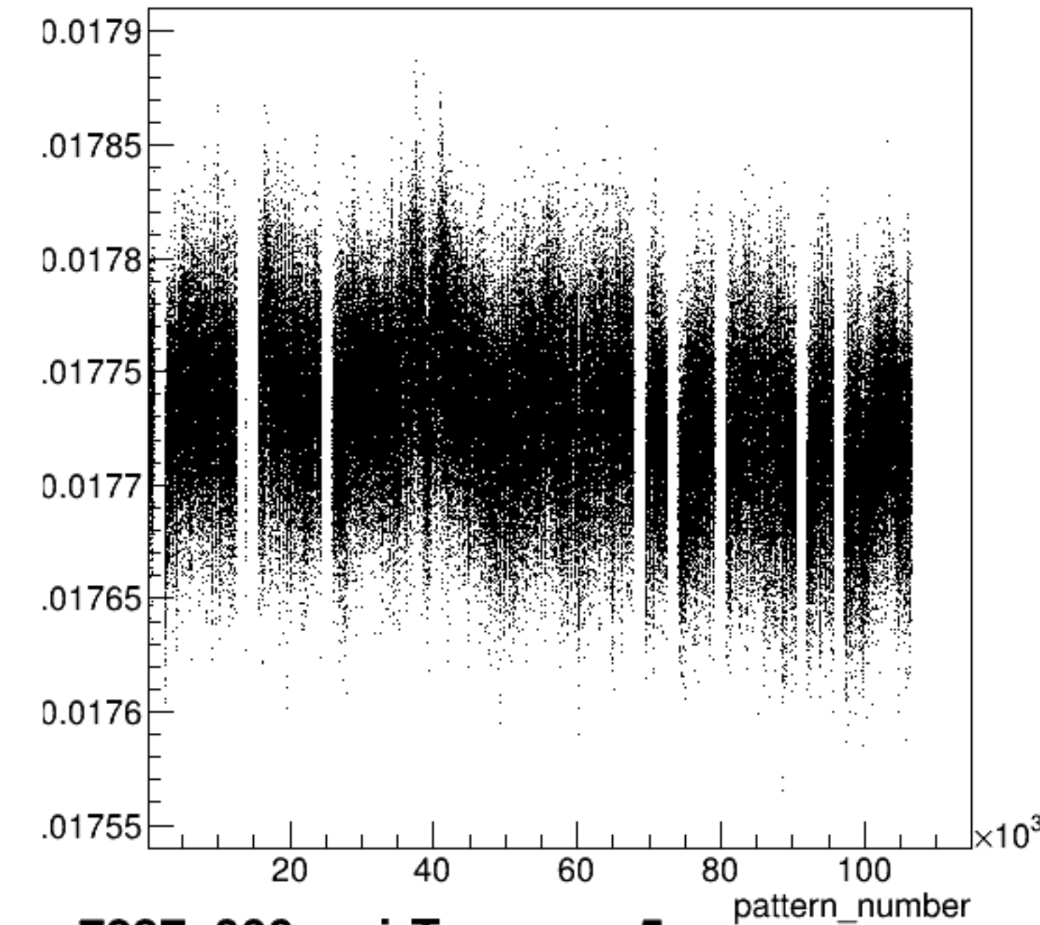
yield_sam5:pattern_number {ErrorFlag==0}
