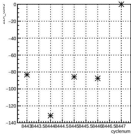
12X_coil3:cyclenum {run == 7238}
