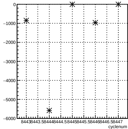
usr_coil6:cyclenum {run == 7238}
