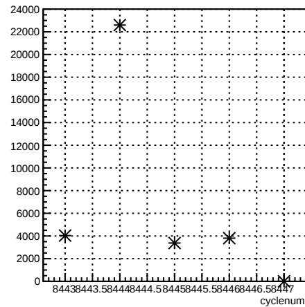
usl_coil4:cyclenum {run == 7238}
