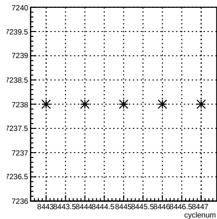
run:cyclenum {run == 7238}
