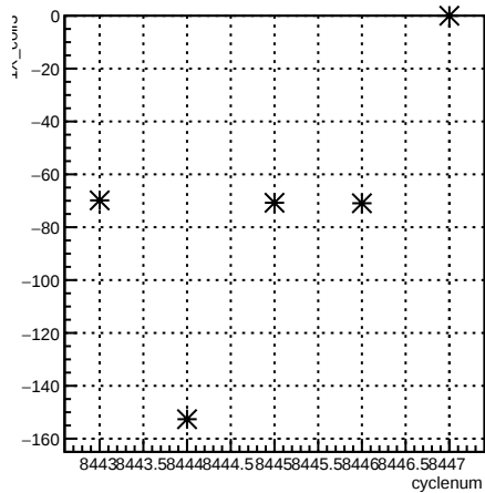
1X_coil3:cyclenum {run == 7238}
