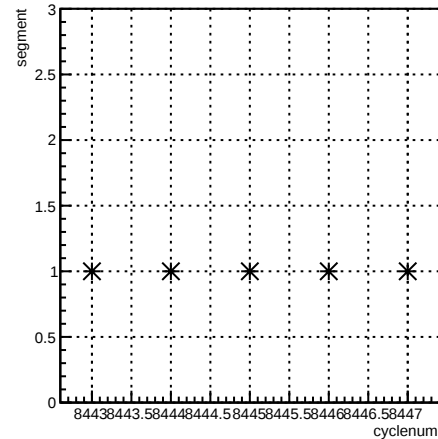
segment:cyclenum {run == 7238}
