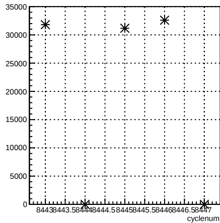
usl_coil1:cyclenum {run == 7238}
