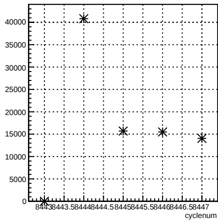
usl_coil7:cyclenum {run == 7238}
