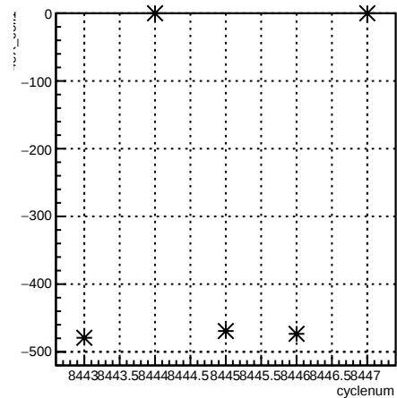
4eX_coil1:cyclenum {run == 7238}
