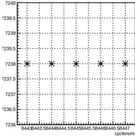
run:cyclenum {run == 7238}
