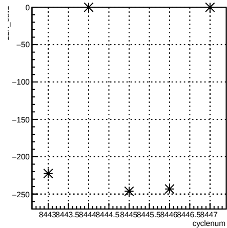
12X_coil1:cyclenum {run == 7238}
