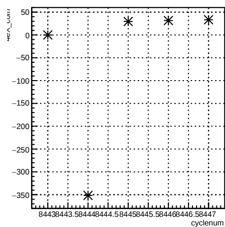
4eX_coil7:cyclenum {run == 7238}
