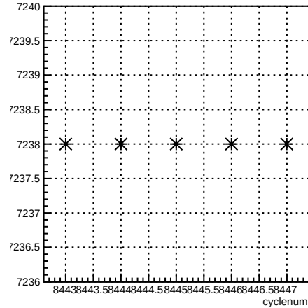
run:cyclenum {run == 7238}
