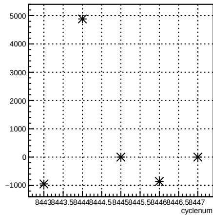
usl_coil6:cyclenum {run == 7238}
