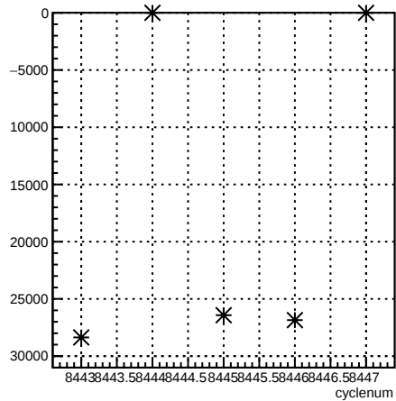
usr_coil1:cyclenum {run == 7238}
