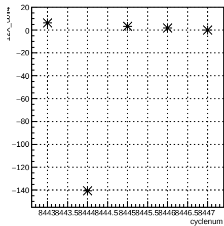
12X_coil4:cyclenum {run == 7238}
