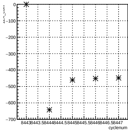
12X_coil7:cyclenum {run == 7238}
