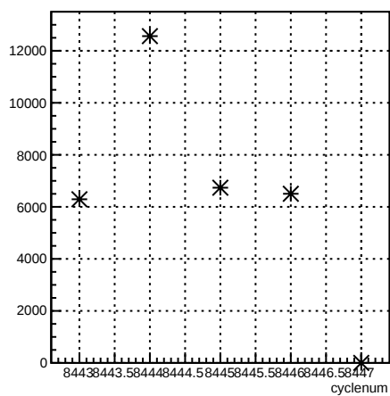
usl_coil3:cyclenum {run == 7238}
