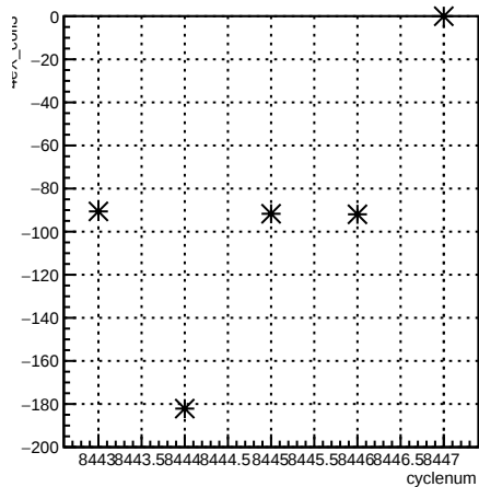
4eX_coil3:cyclenum {run == 7238}
