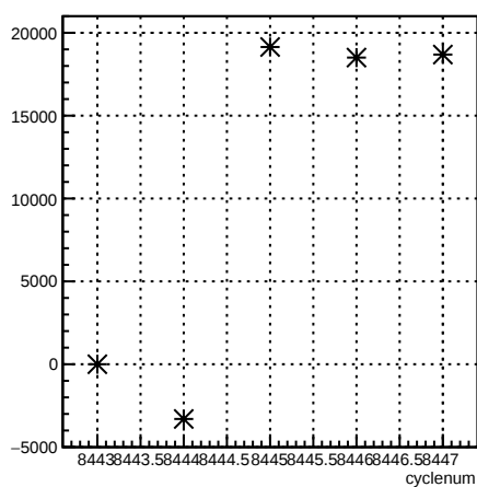
usr_coil7:cyclenum {run == 7238}
