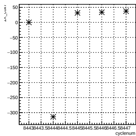
1X_coil7:cyclenum {run == 7238}
