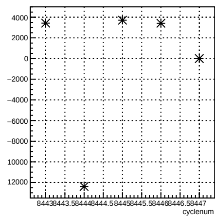
usr_coil4:cyclenum {run == 7238}
