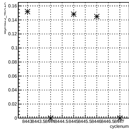
delta46_12X4eY:cyclenum {run == 7238}
