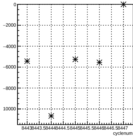
usr_coil3:cyclenum {run == 7238}
