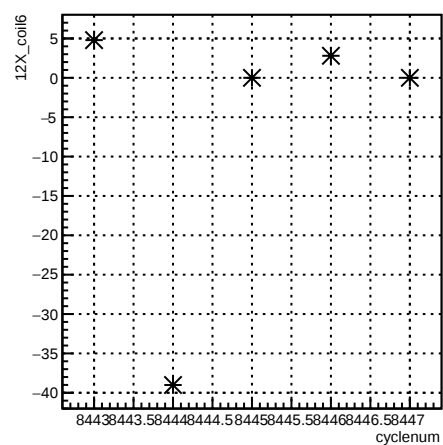
12X_coil6:cyclenum {run == 7238}
