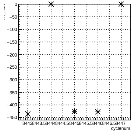
1X_coil1:cyclenum {run == 7238}
