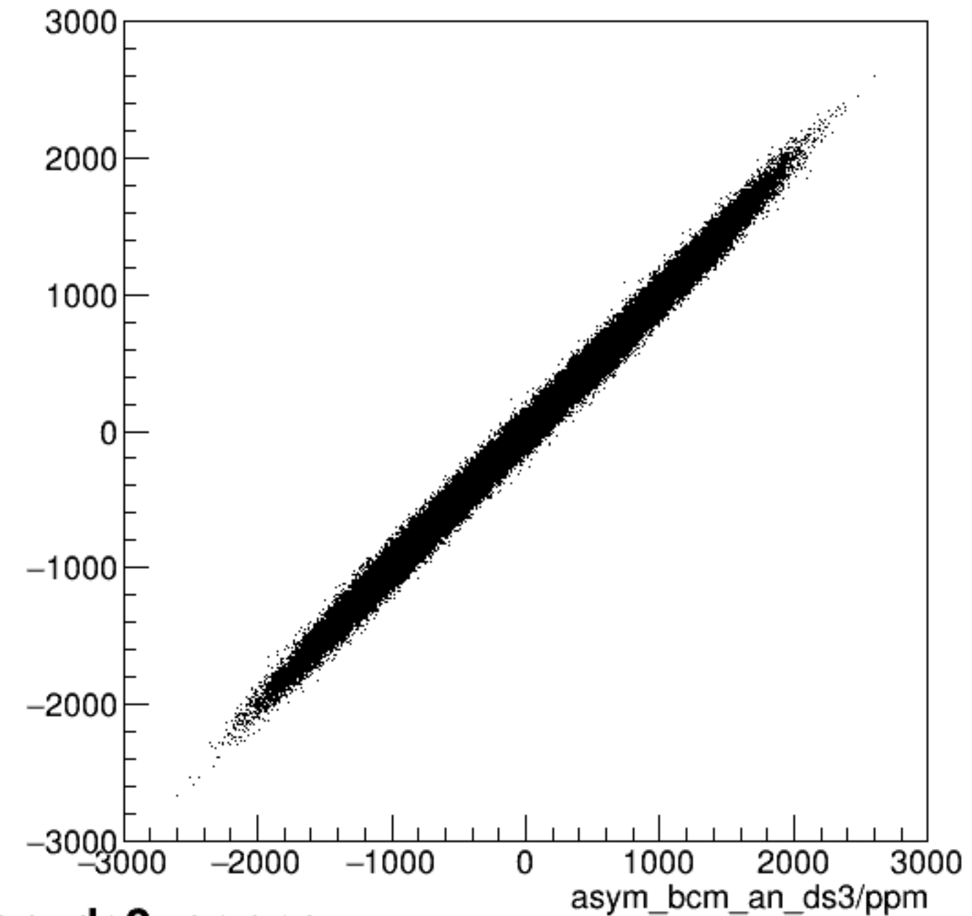
run7242_000_asym_bcm_dg_us_vs_asym_bcm_an_ds3_pr.png
