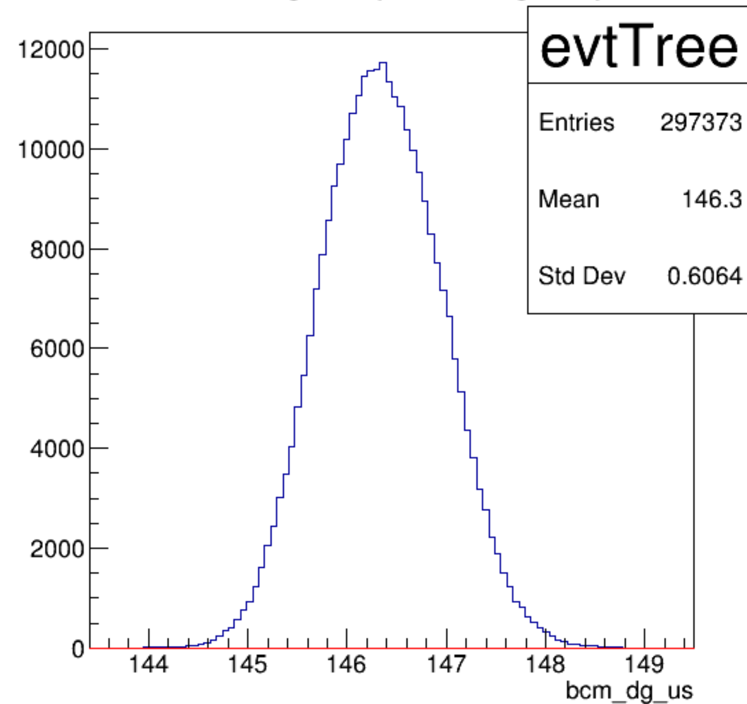
bcm_dg_us {ErrorFlag==0}
