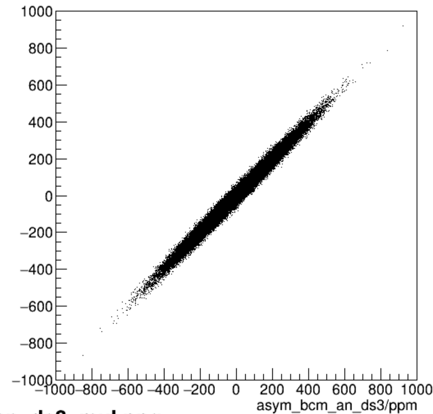
run7242_000_asym_bcm_an_us_vs_asym_bcm_an_ds3_mul.png
