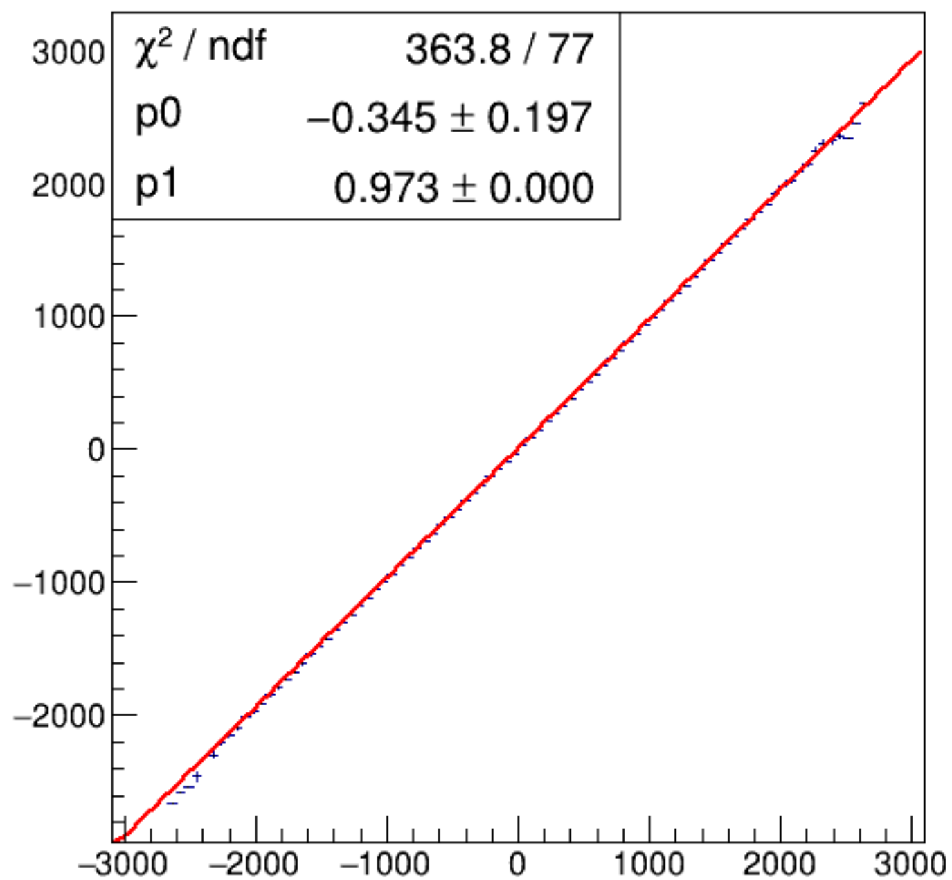
run7242_000_asym_bcm_dg_us_vs_asym_bcm_dg_ds_pr.png
