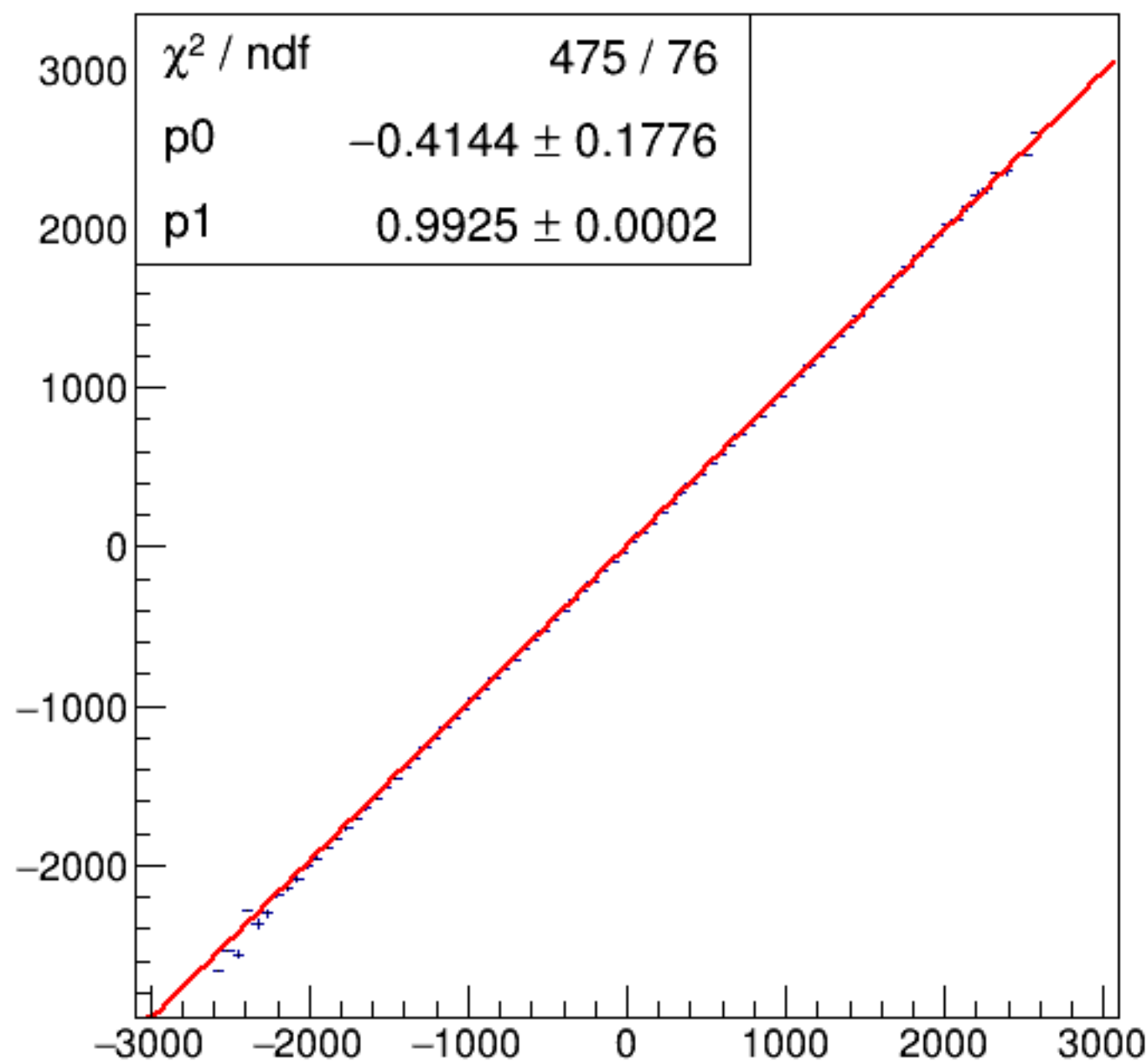
run7242_000_asym_bcm_dg_us_vs_asym_bcm_an_ds3_pr.png
