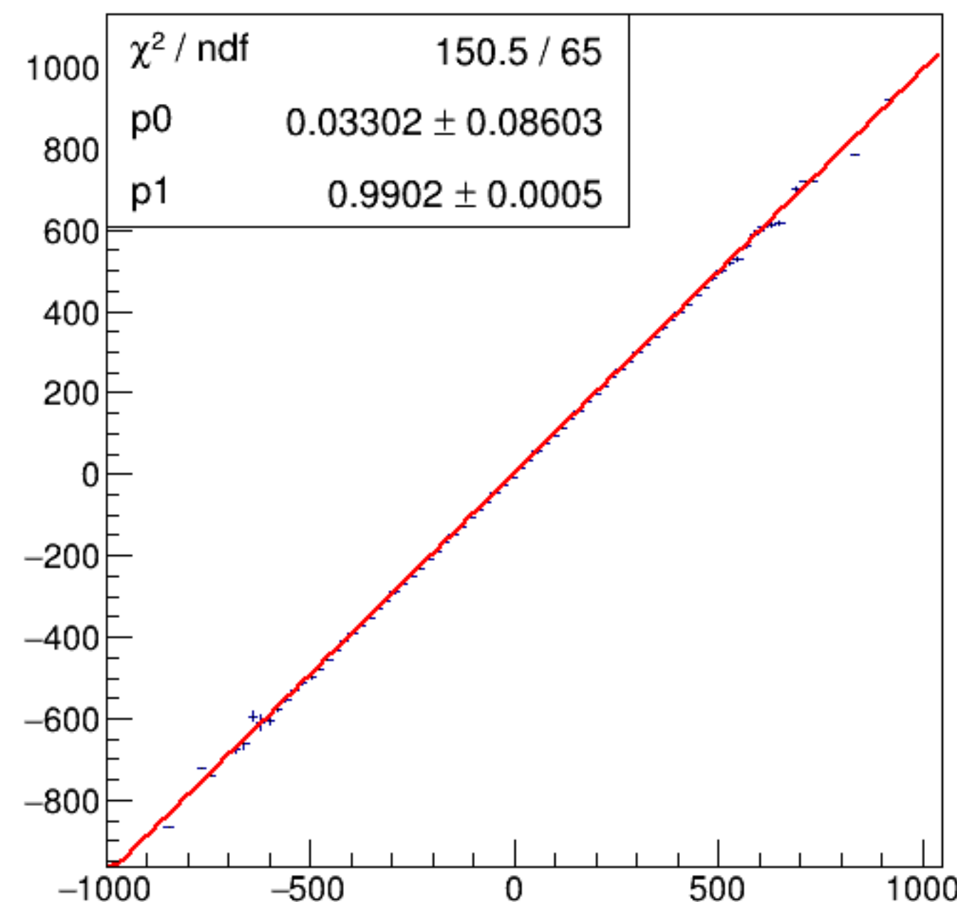
run7242_000_asym_bcm_an_us_vs_asym_bcm_an_ds3_mul.png
