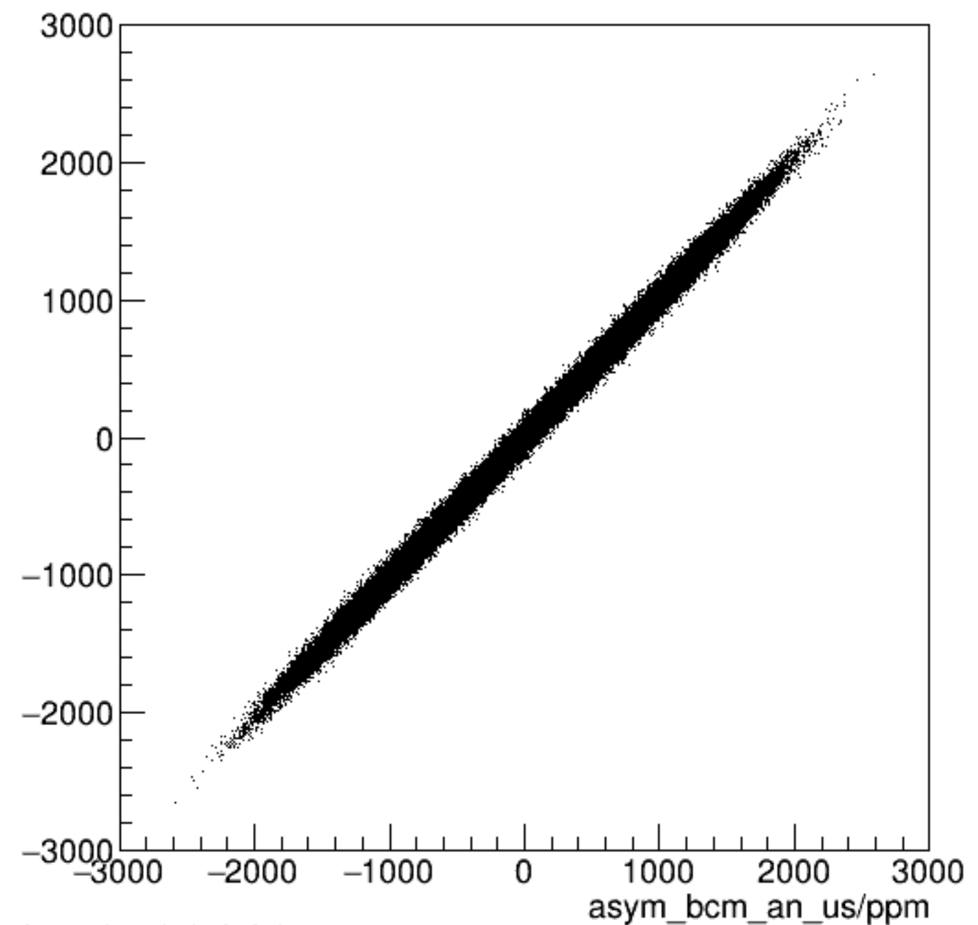
run7242_000_asym_bcm_dg_ds_vs_asym_bcm_an_us_pr.png
