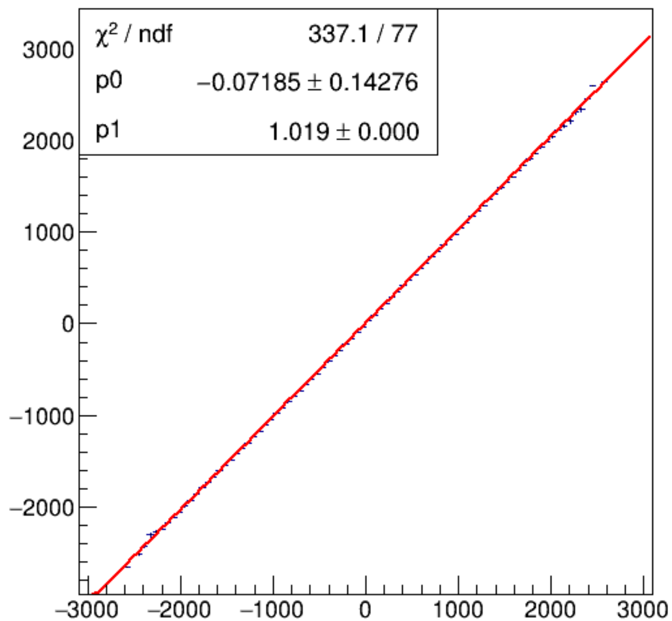
run7242_000_asym_bcm_dg_ds_vs_asym_bcm_an_us_pr.png
