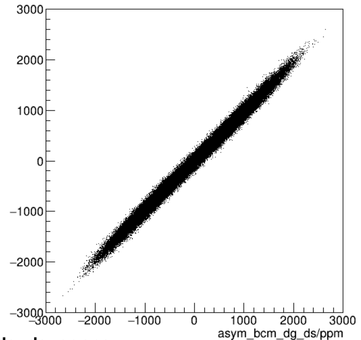
run7242_000_asym_bcm_dg_us_vs_asym_bcm_dg_ds_pr.png
