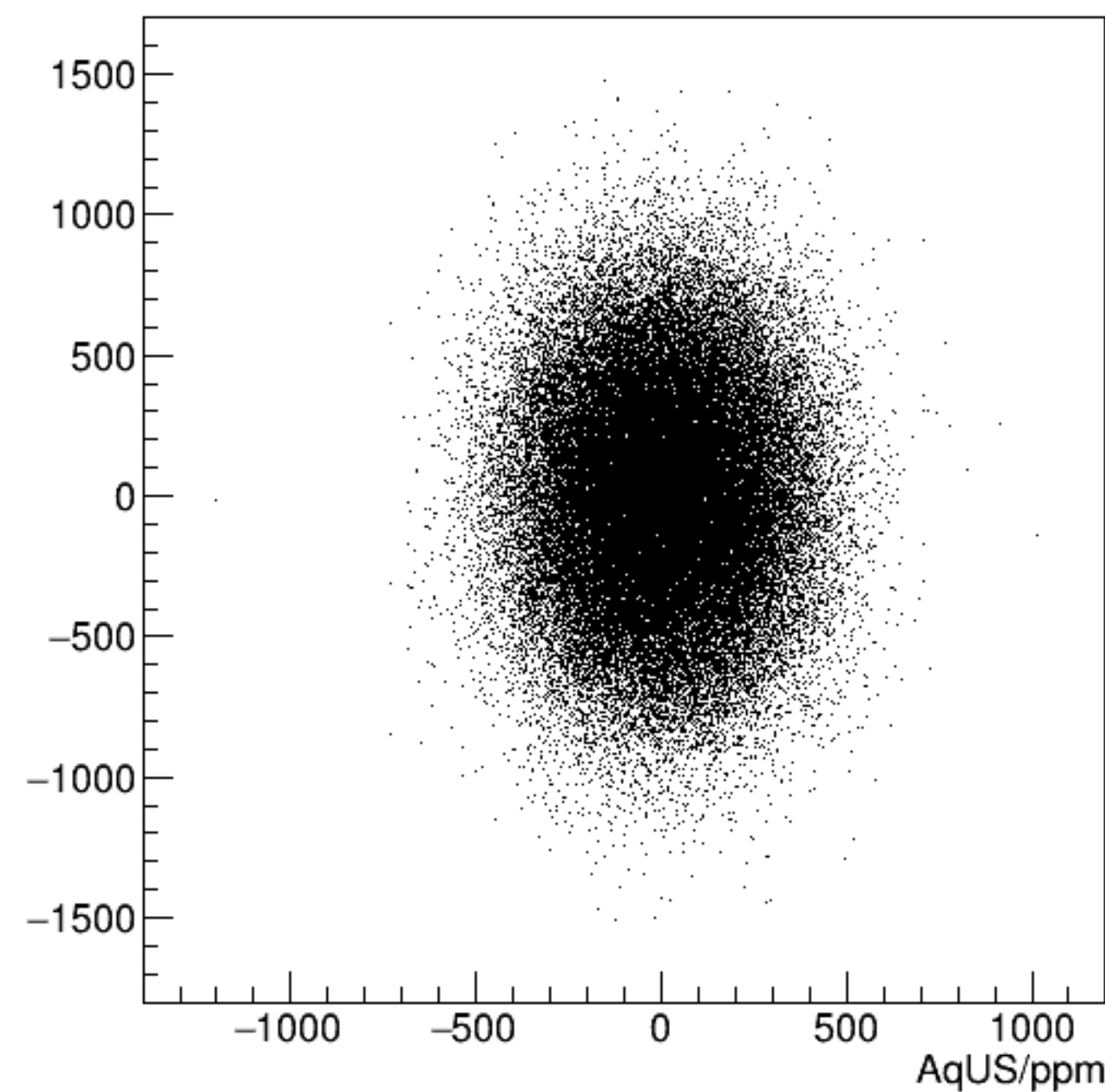
reg_asym_dsl/ppm:AqUS/ppm {ok_cut}
