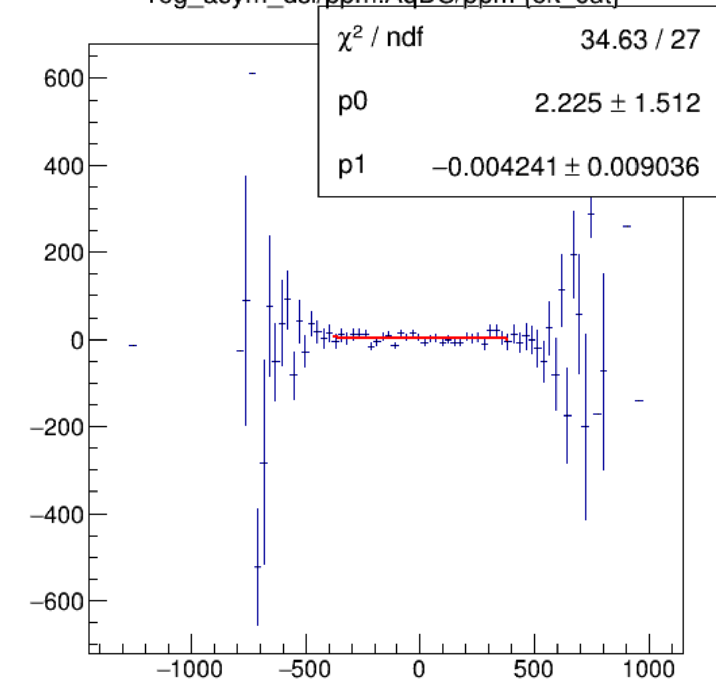
reg_asym_dsl/ppm:AqDS/ppm {ok_cut}
