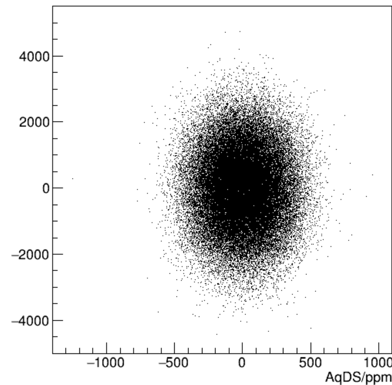
reg_asym_usr/ppm:AqDS/ppm {ok_cut}
