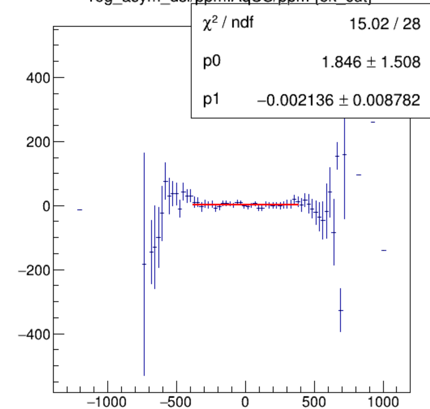
reg_asym_dsl/ppm:AqUS/ppm {ok_cut}
