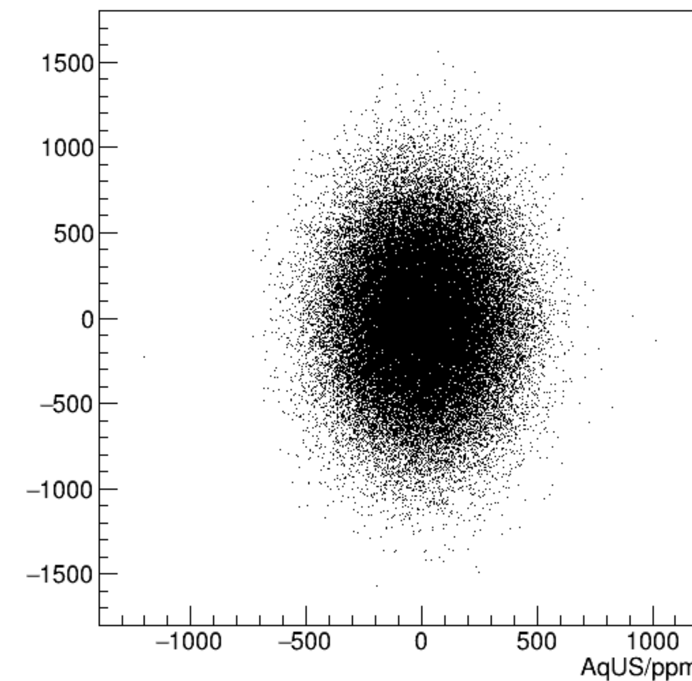
reg_asym_dsr/ppm:AqUS/ppm {ok_cut}
