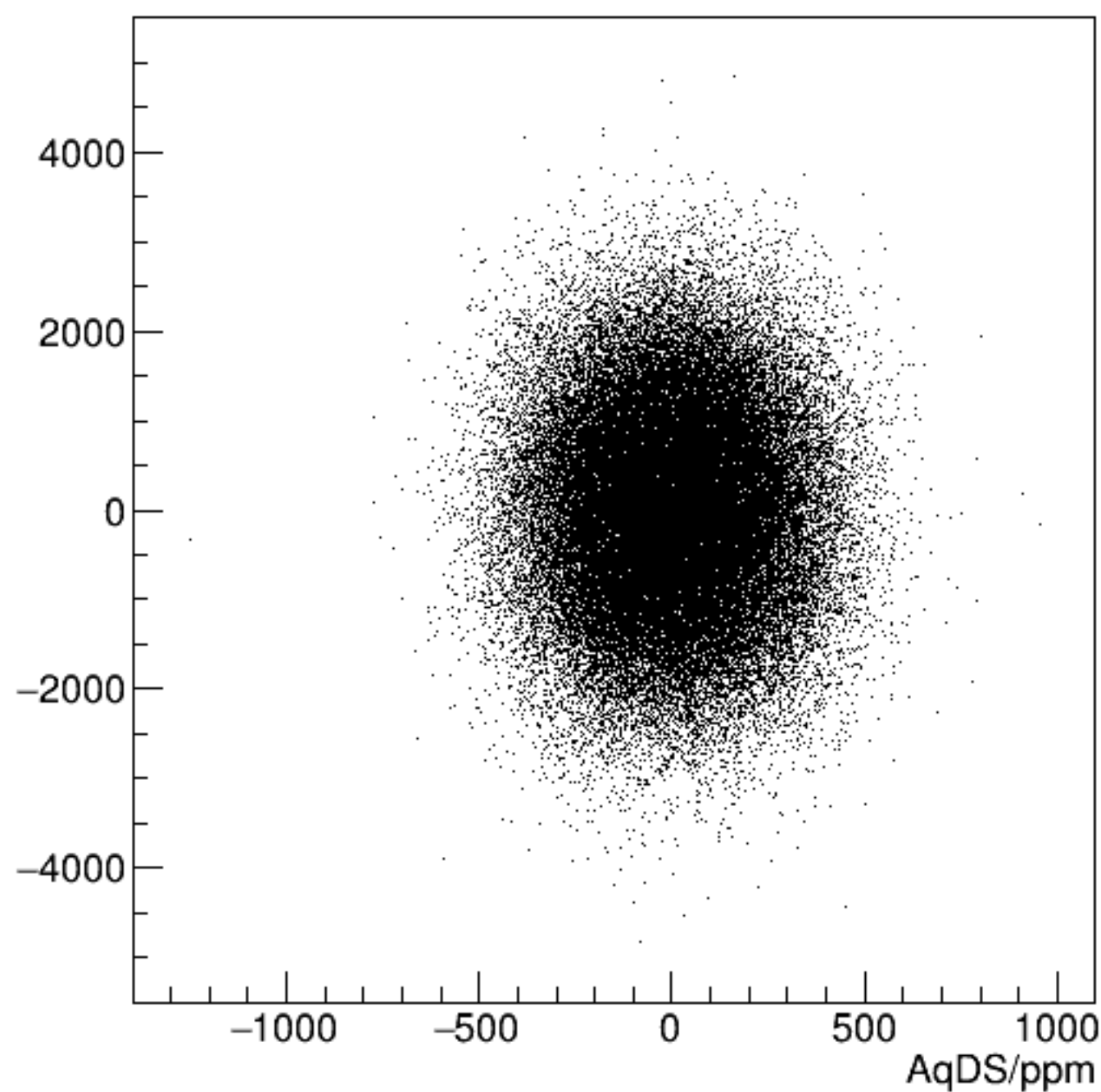
reg_asym_usl/ppm:AqDS/ppm {ok_cut}
