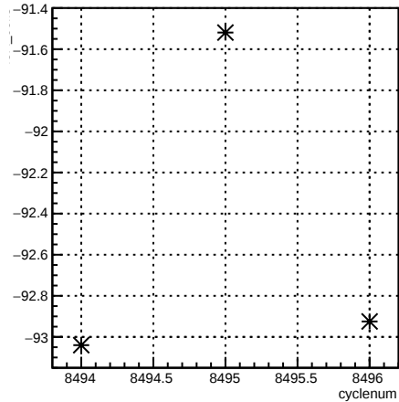
4eX_coil3:cyclenum {run == 7251}
