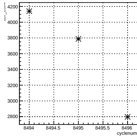
usr_coil4:cyclenum {run == 7251}
