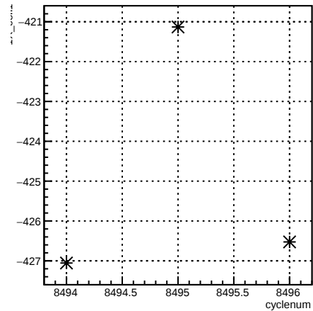
4eX_coil1:cyclenum {run == 7251}
