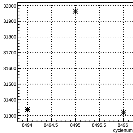
usl_coil6:cyclenum {run == 7251}
