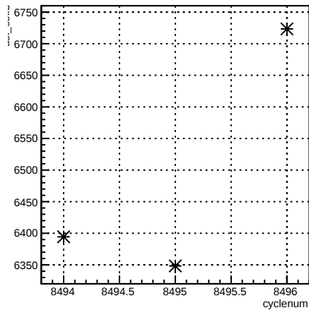
usl_coil7:cyclenum {run == 7251}
