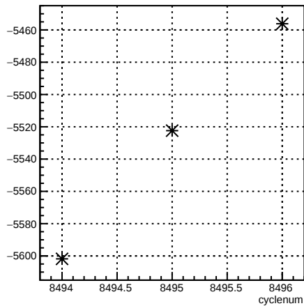
usr_coil3:cyclenum {run == 7251}
