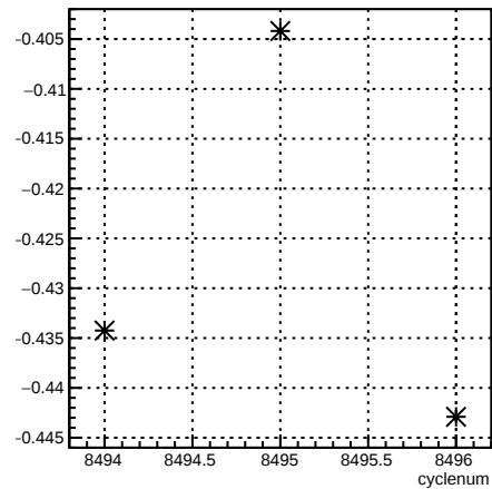
delta13_12X4eX:cyclenum {run == 7251}
