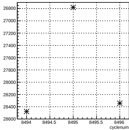
usr_coil1:cyclenum {run == 7251}
