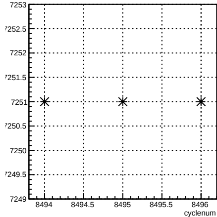
run:cyclenum {run == 7251}
