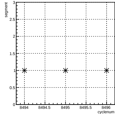
segment:cyclenum {run == 7251}
