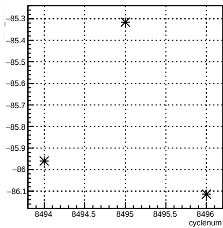
12X_coil3:cyclenum {run == 7251}
