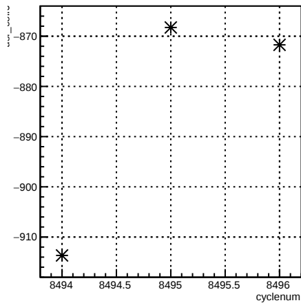
usr_coil6:cyclenum {run == 7251}
