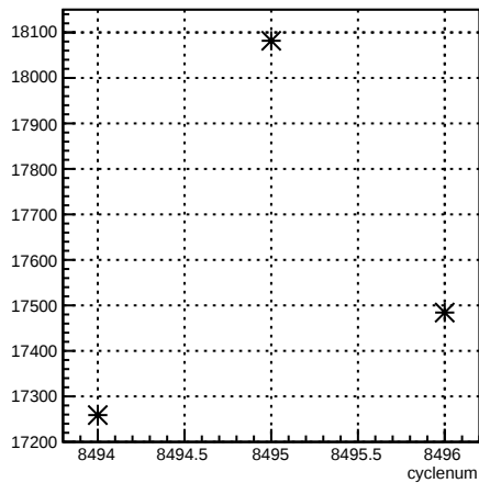
usr_coil7:cyclenum {run == 7251}
