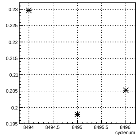
delta6_12X4eY:cyclenum {run == 7251}
