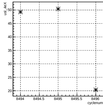
run:cyclenum {run == 7251}
