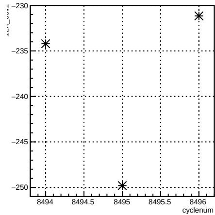
12X_coil1:cyclenum {run == 7251}
