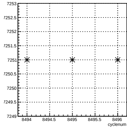
run:cyclenum {run == 7251}
