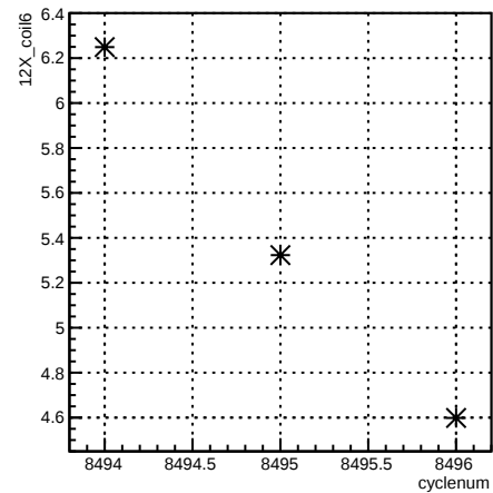
12X_coil6:cyclenum {run == 7251}
