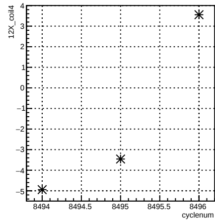
12X_coil4:cyclenum {run == 7251}
