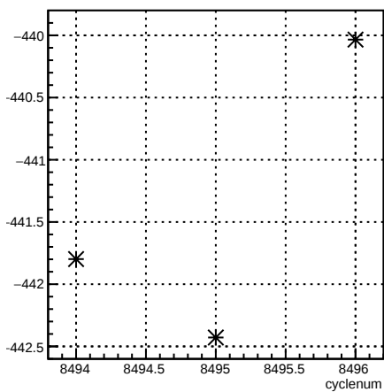
12X_coil7:cyclenum {run == 7251}
