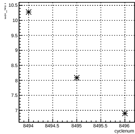
usr_4eY:cyclenum {run == 7251}
