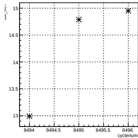
usl_4eY:cyclenum {run == 7251}
