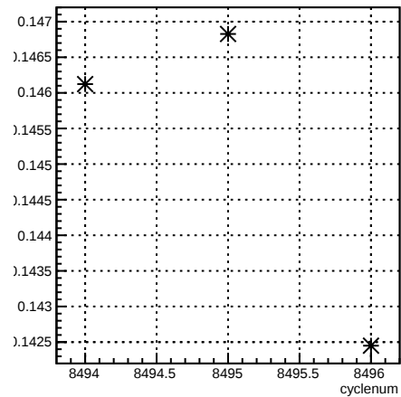
alpha13_4eX1X:cyclenum {run == 7251}
