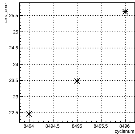
4eX_coil7:cyclenum {run == 7251}
