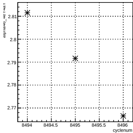
alpha46_4eY4aY:cyclenum {run == 7251}
