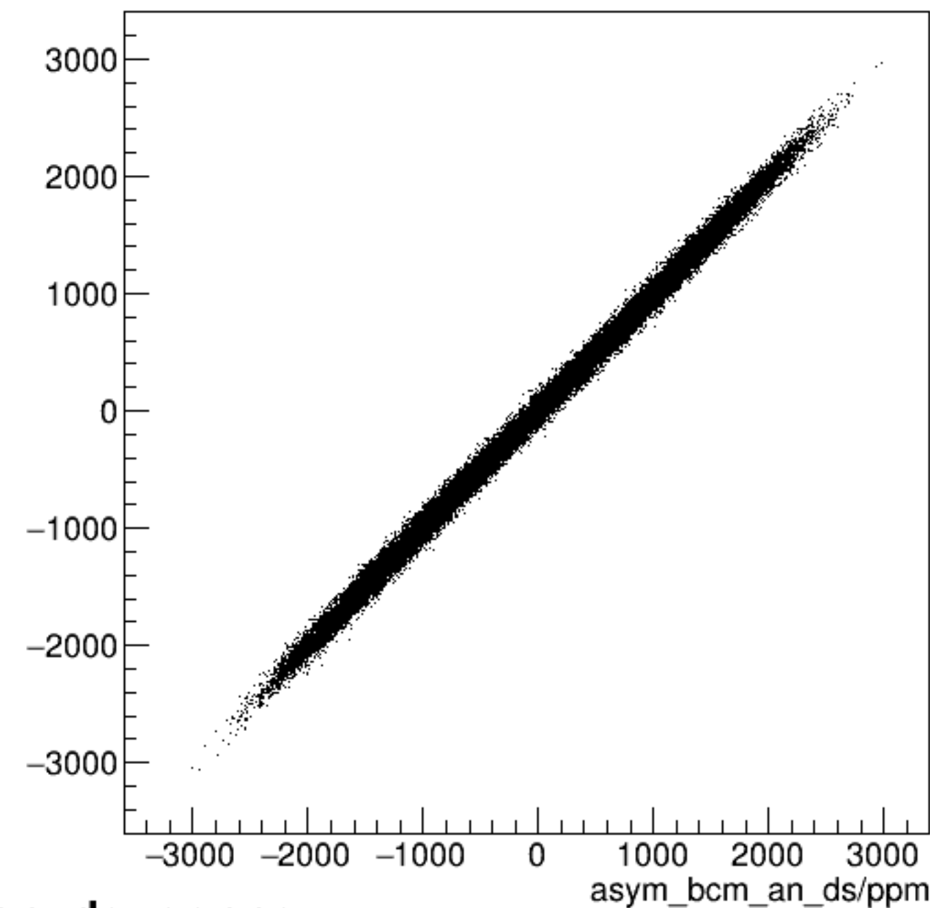
run7256_000_asym_bcm_dg_us_vs_asym_bcm_an_ds_pr.png
