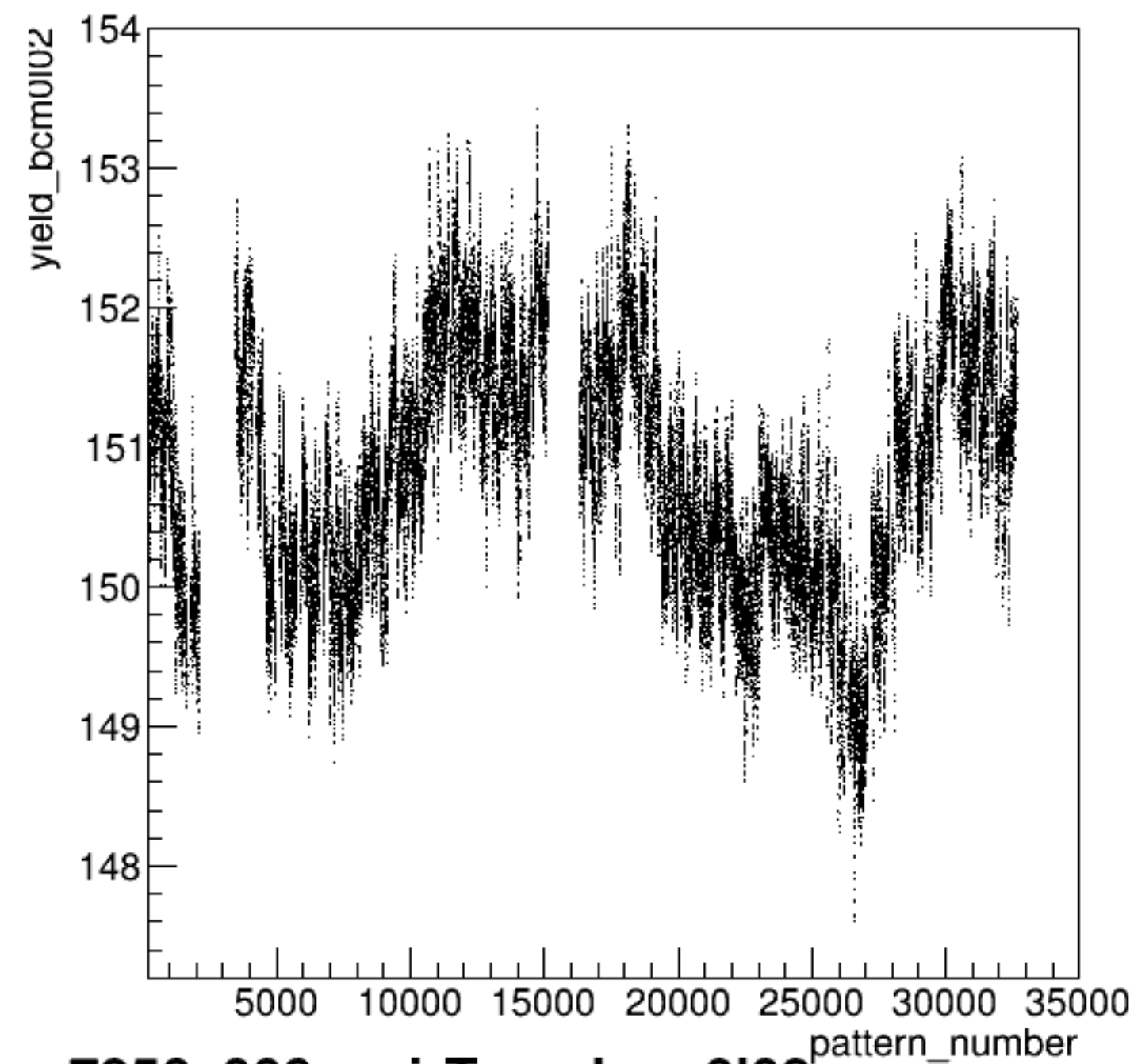
yield_bcm0l02:pattern_number {ErrorFlag==0}
