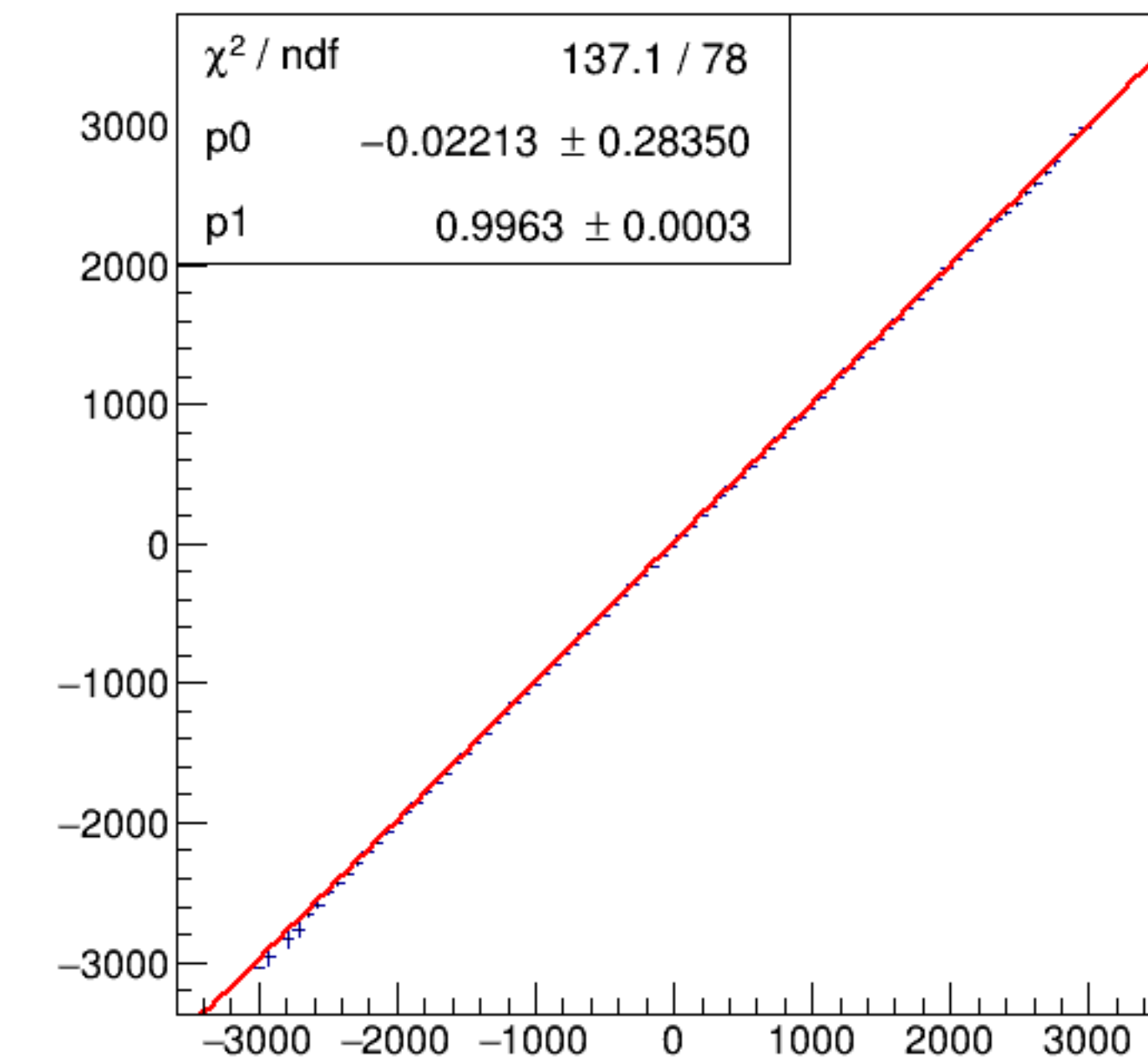
run7256_000_asym_bcm_dg_us_vs_asym_bcm_an_ds_pr.png
