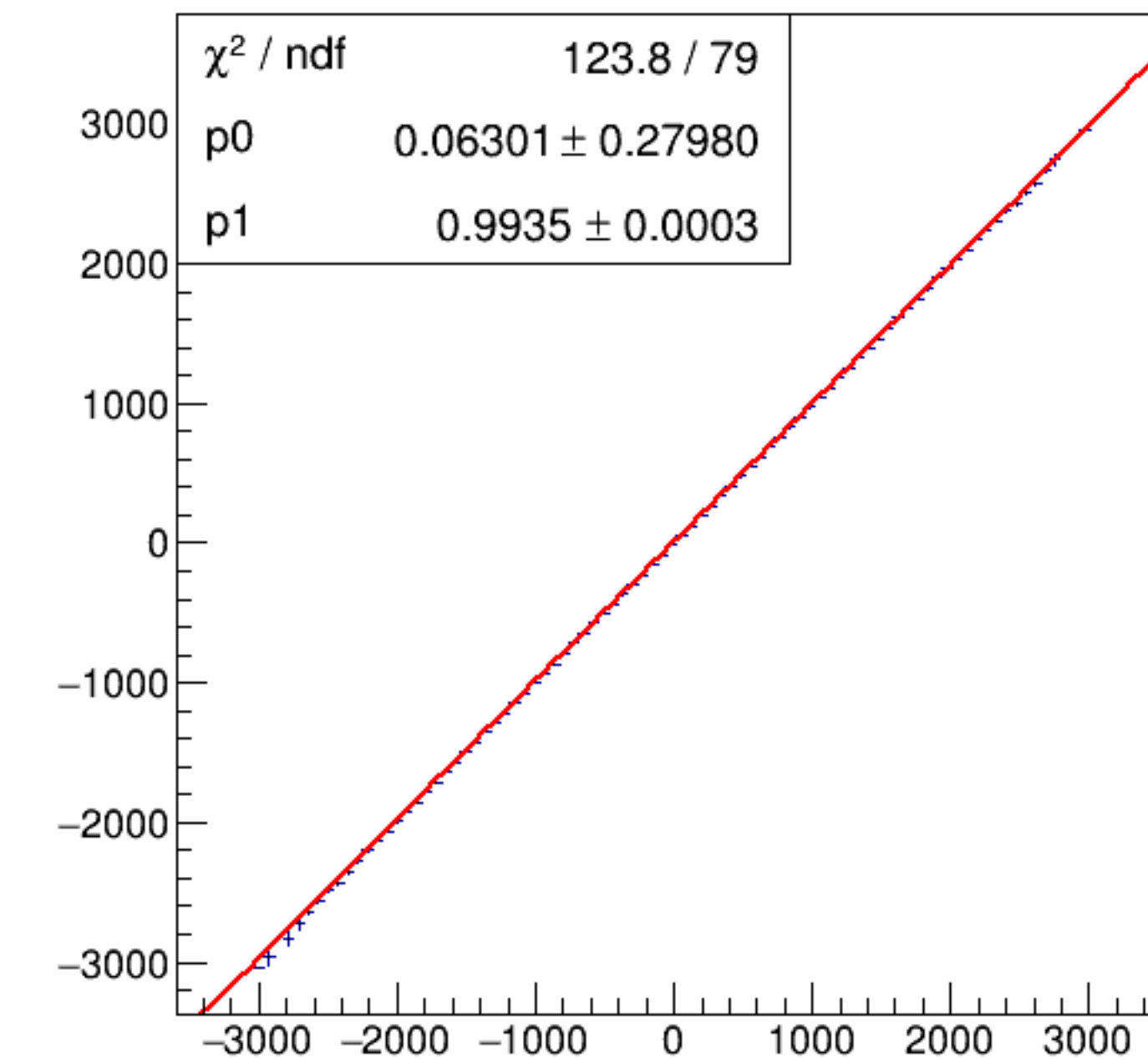
run7256_000_asym_bcm_dg_us_vs_asym_bcm_an_ds3_pr.png
