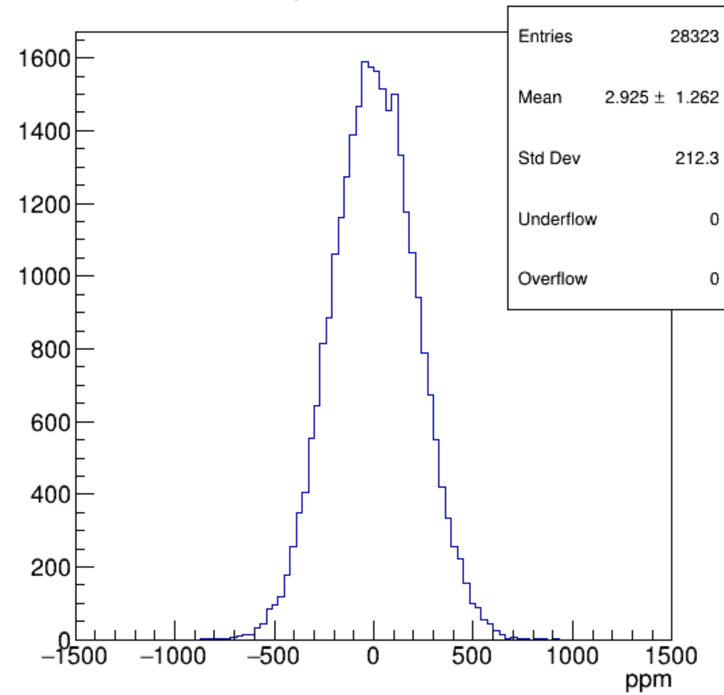
asym_bcm0l02
