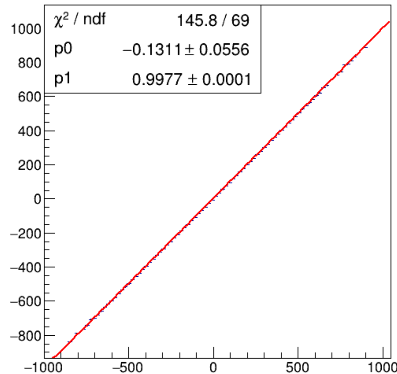
run7256_000_asym_bcm_an_ds_vs_asym_bcm_an_ds3_mul.png
