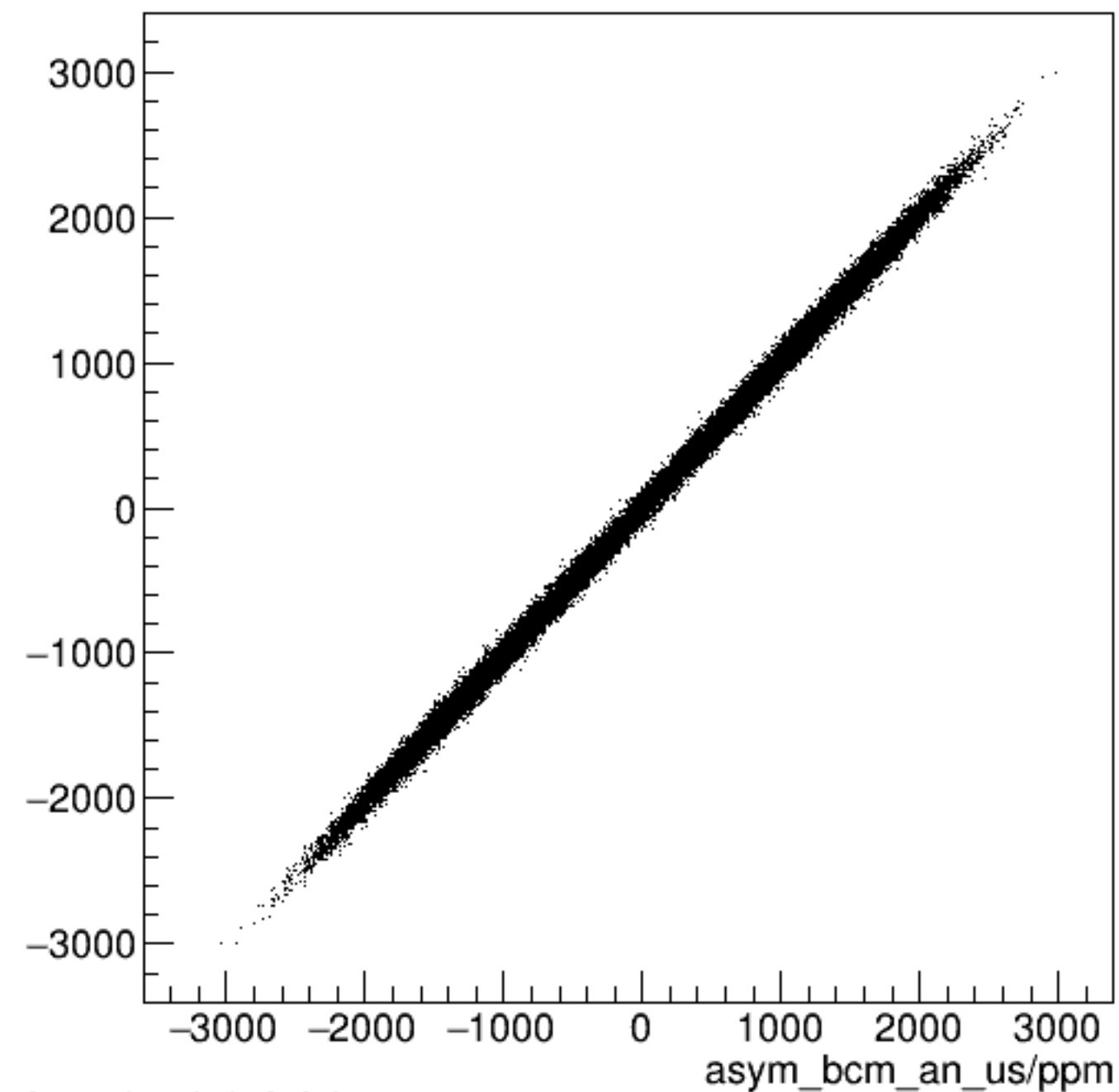
run7256_000_asym_bcm_dg_ds_vs_asym_bcm_an_us_pr.png
