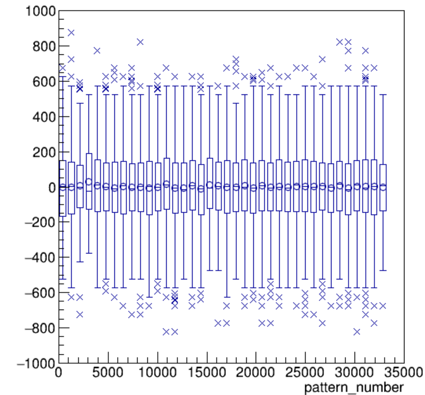
asym_bcm_dg_us/ppm:pattern_number {ErrorFlag==0}
