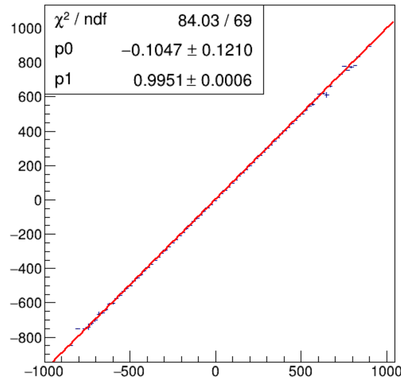
run7256_000_asym_bcm_an_us_vs_asym_bcm_an_ds3_mul.png
