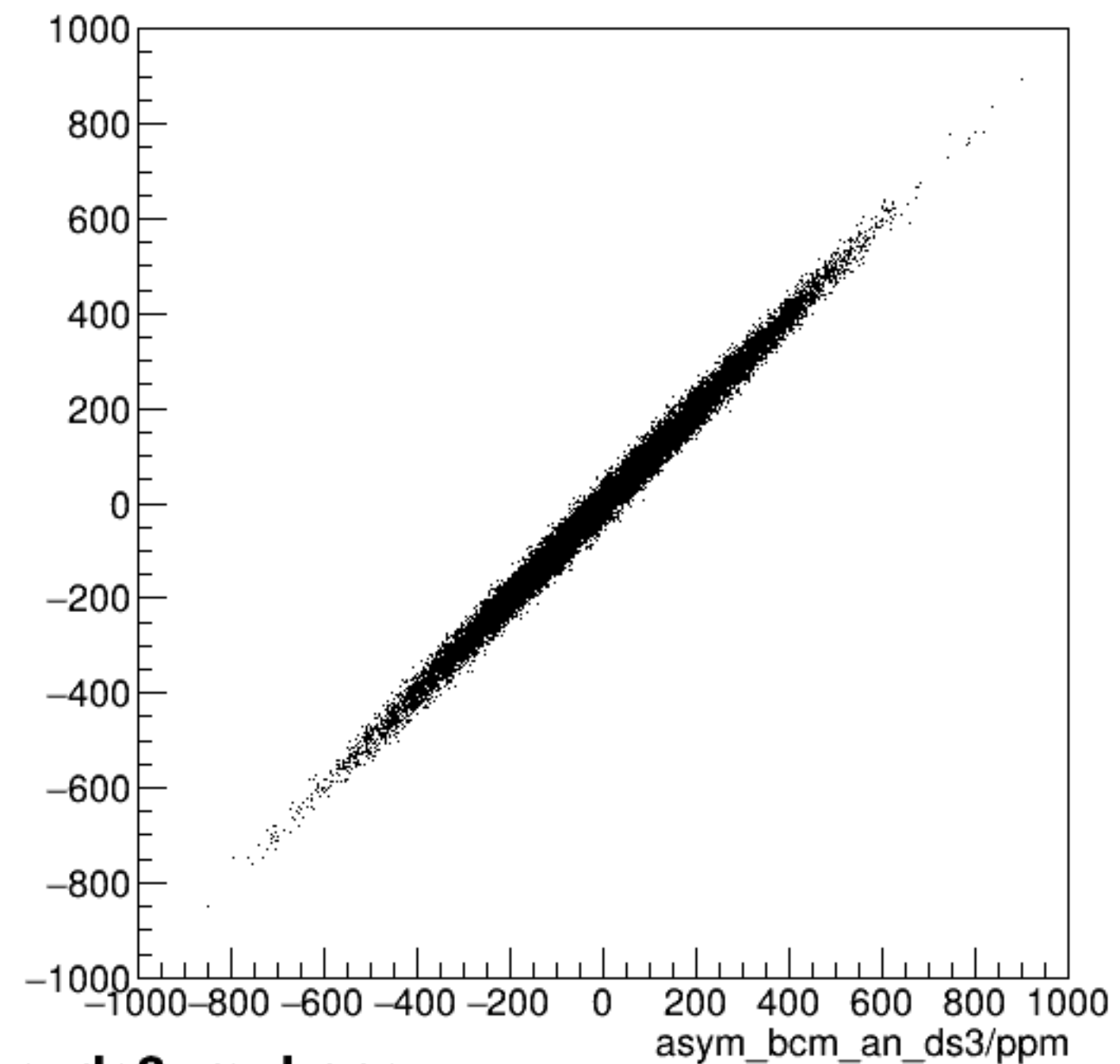
run7256_000_asym_bcm_an_us_vs_asym_bcm_an_ds3_mul.png
