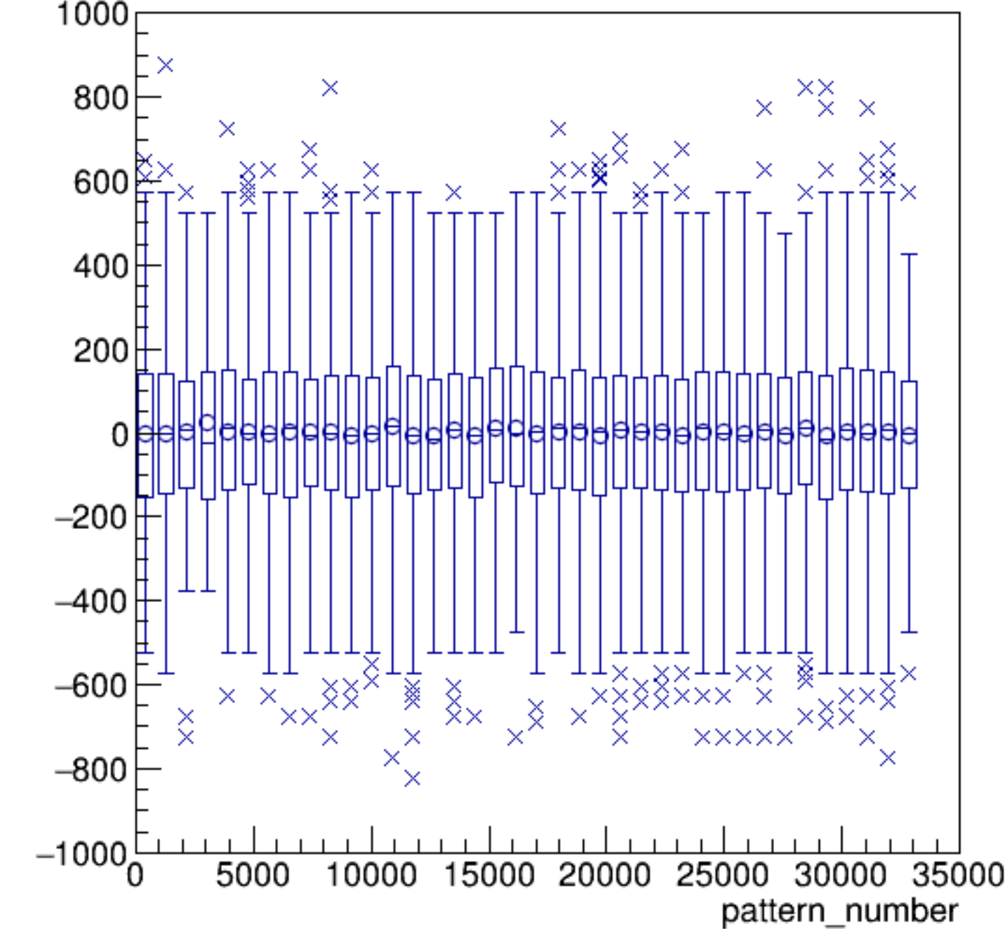
asym_bcm_an_ds/ppm:pattern_number {ErrorFlag==0}
