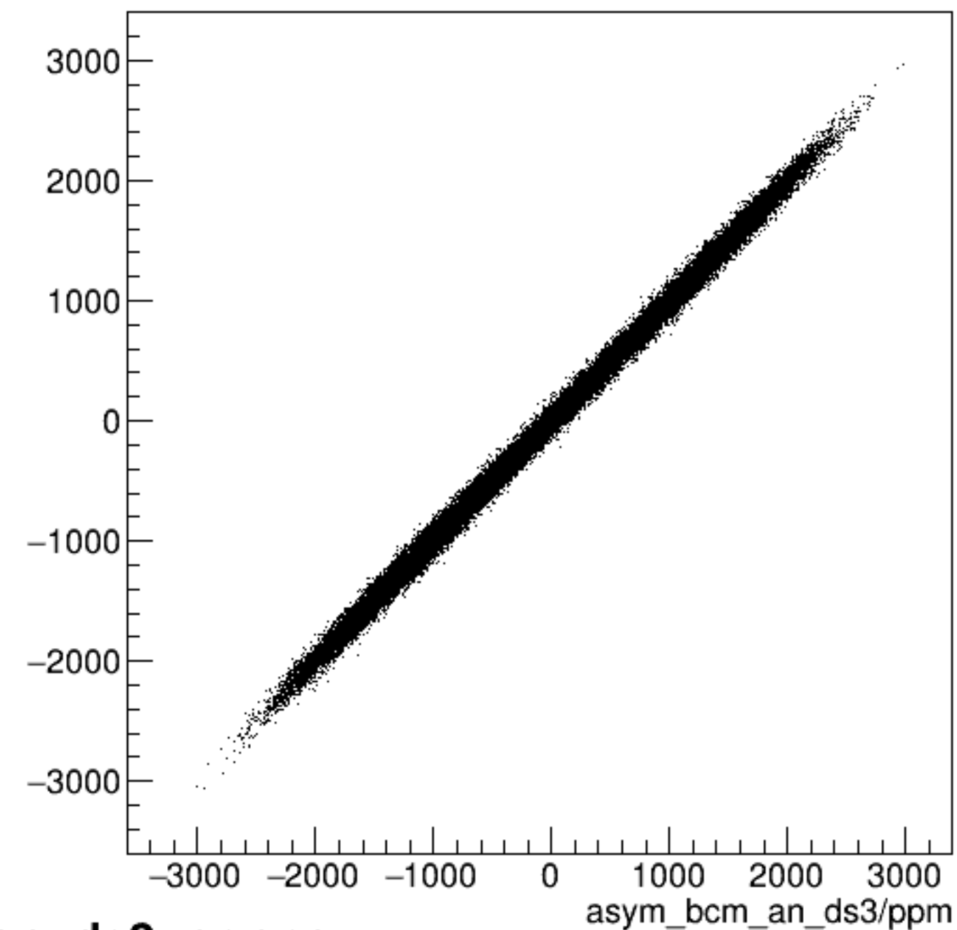
run7256_000_asym_bcm_dg_us_vs_asym_bcm_an_ds3_pr.png
