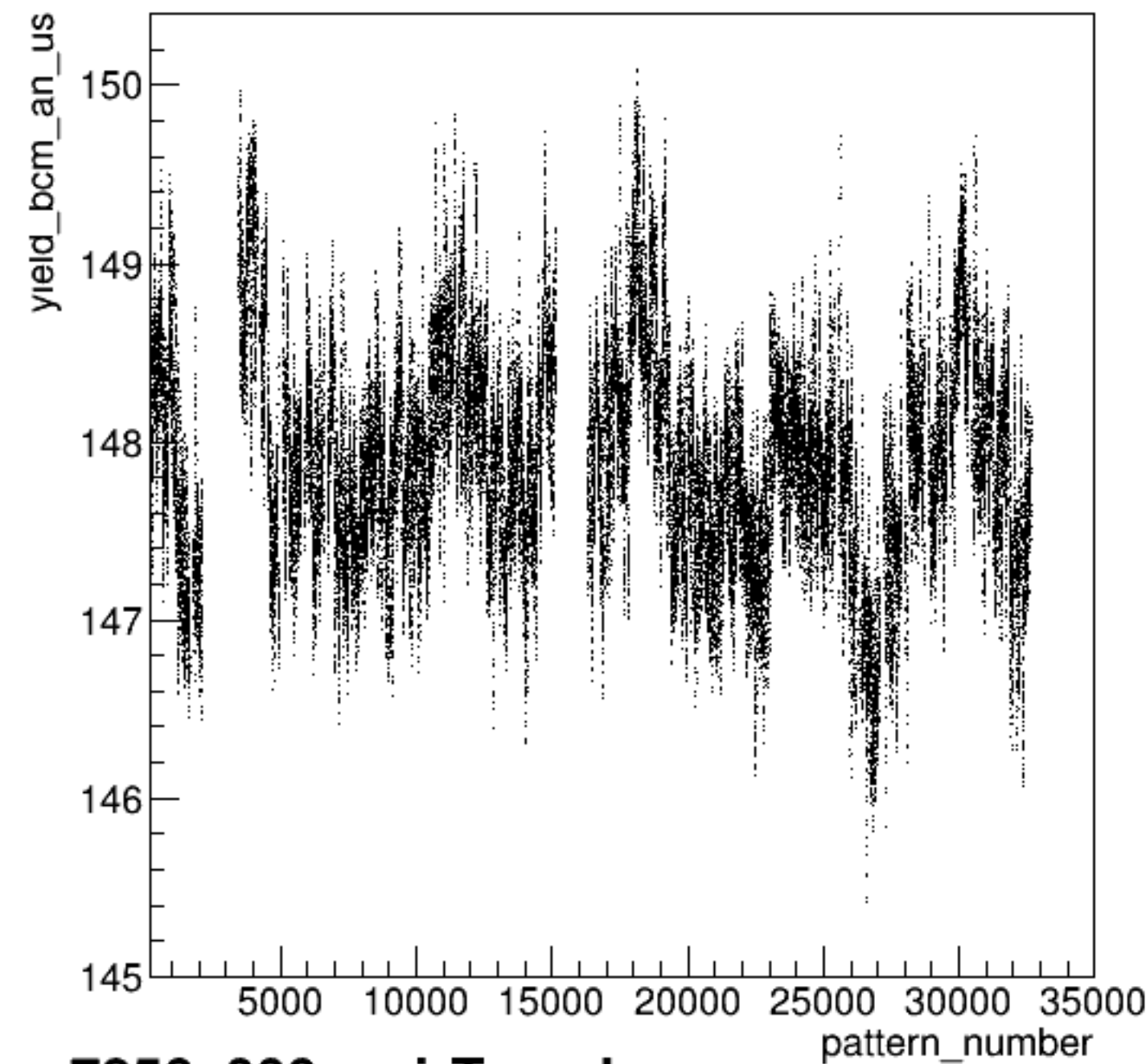
yield_bcm_an_us:pattern_number {ErrorFlag==0}
