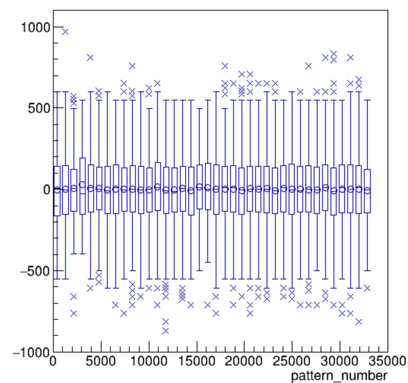
asym_bcm_dg_ds/ppm:pattern_number {ErrorFlag==0}
