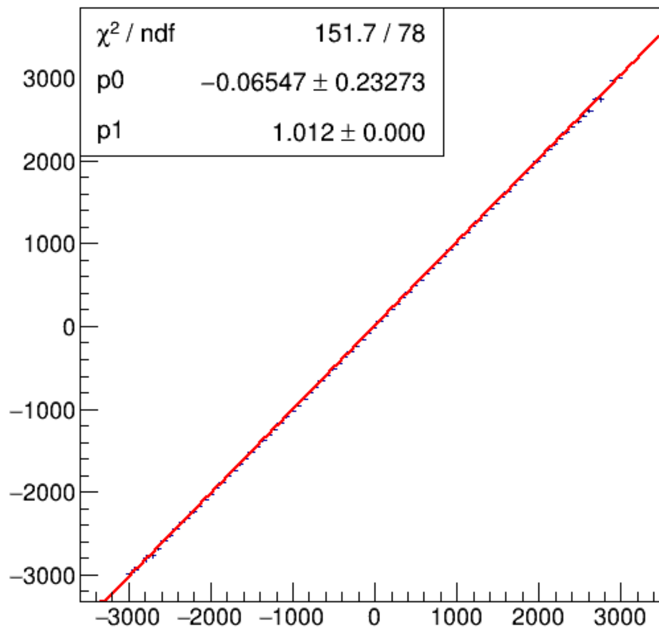
run7256_000_asym_bcm_dg_ds_vs_asym_bcm_an_us_pr.png
