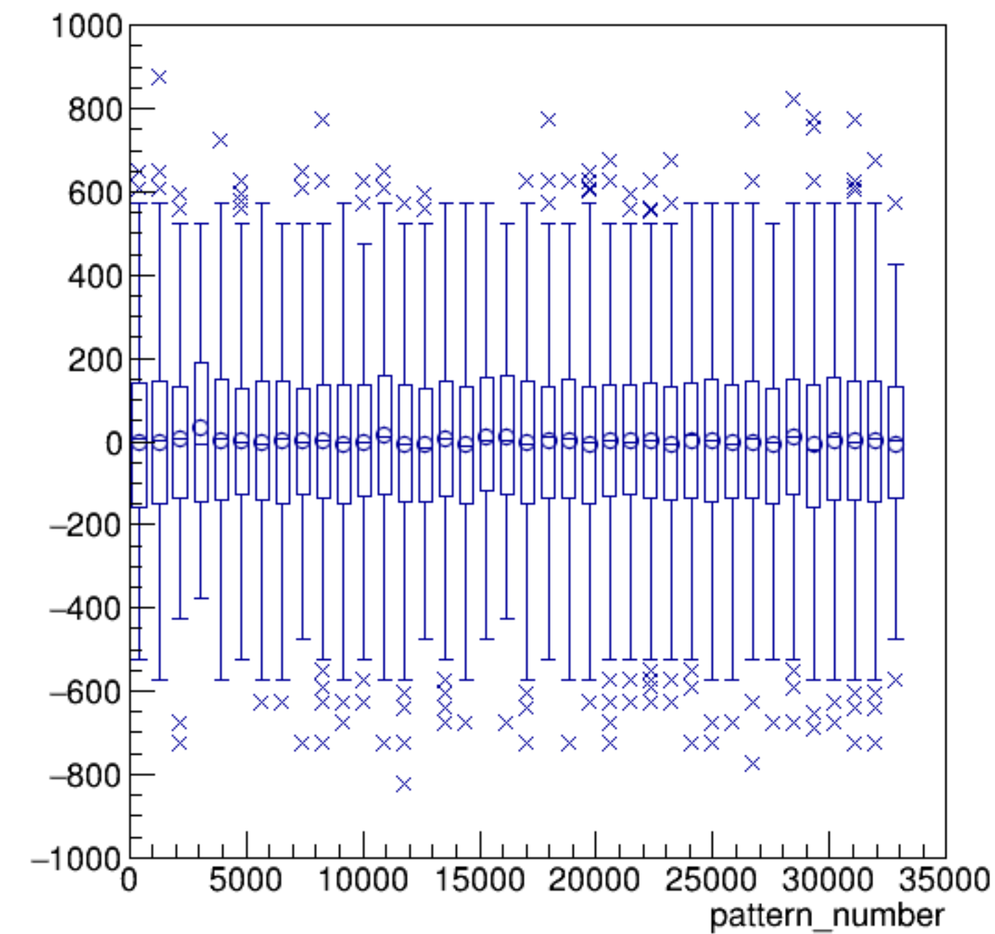
asym_bcm_an_us/ppm:pattern_number {ErrorFlag==0}
