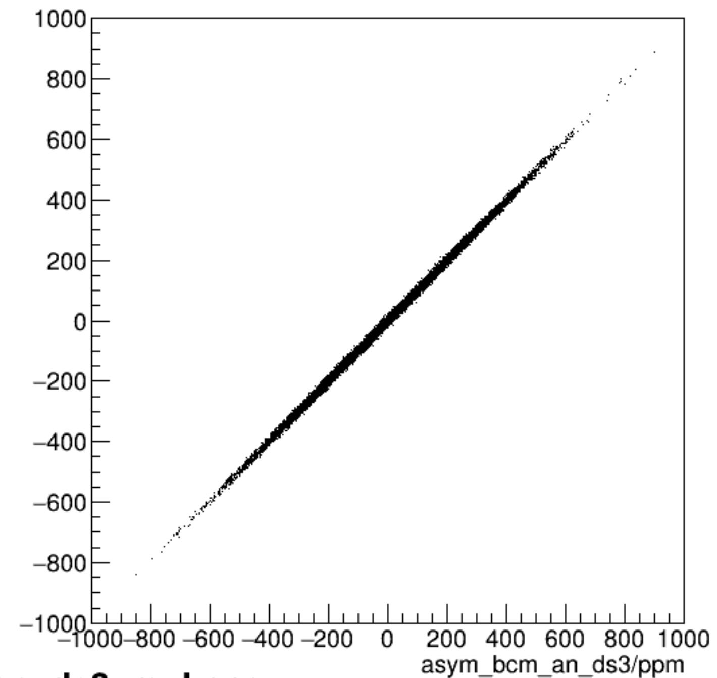
run7256_000_asym_bcm_an_ds_vs_asym_bcm_an_ds3_mul.png
