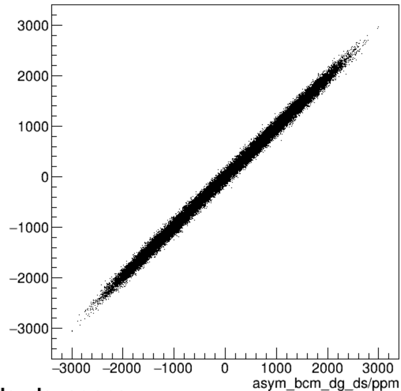
run7256_000_asym_bcm_dg_us_vs_asym_bcm_dg_ds_pr.png
