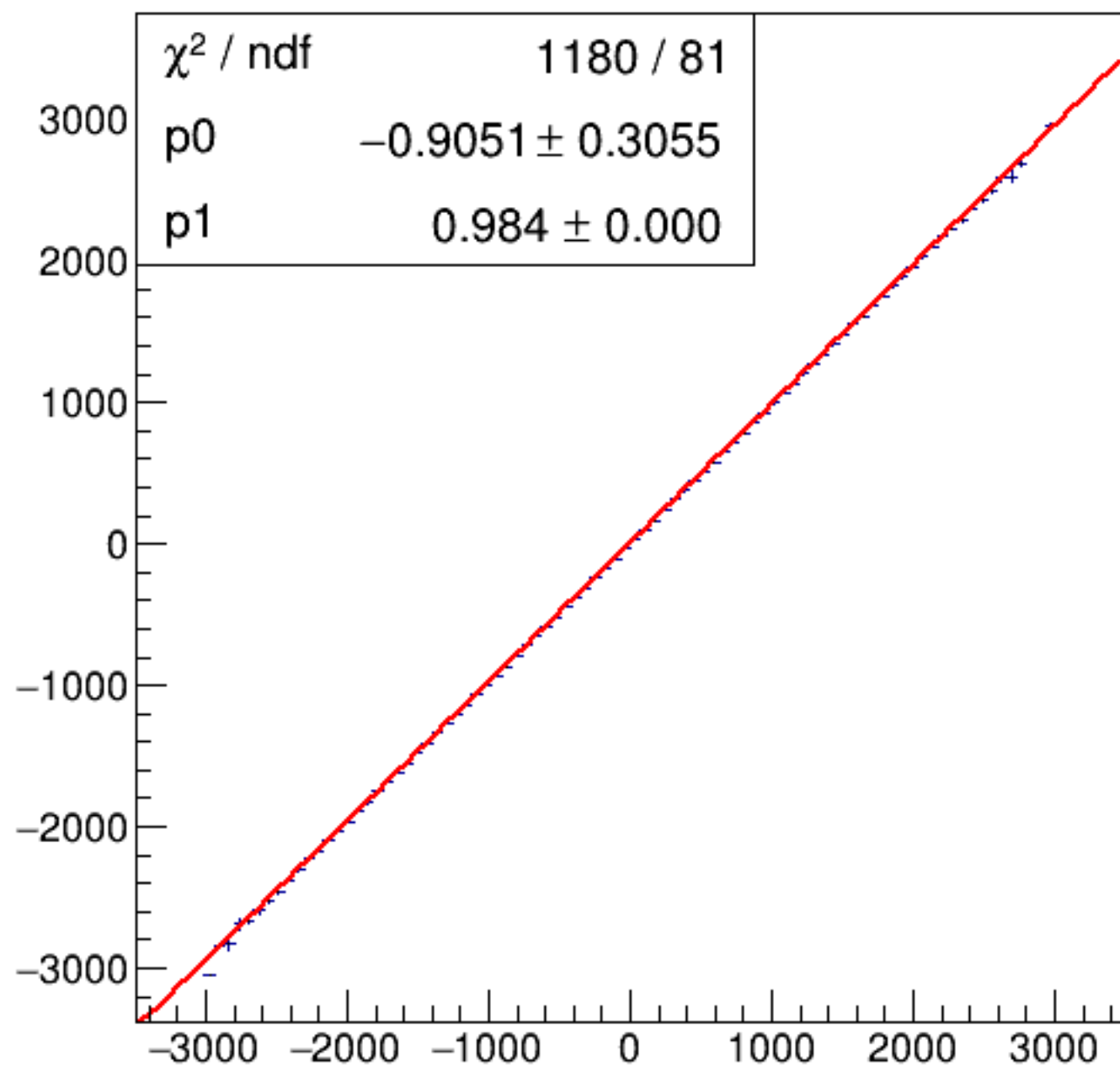
run7256_000_asym_bcm_dg_us_vs_asym_bcm_dg_ds_pr.png
