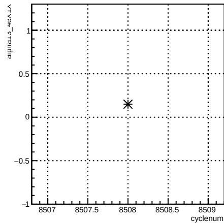
alpha13_4eX1X:cyclenum {run == 7257}
