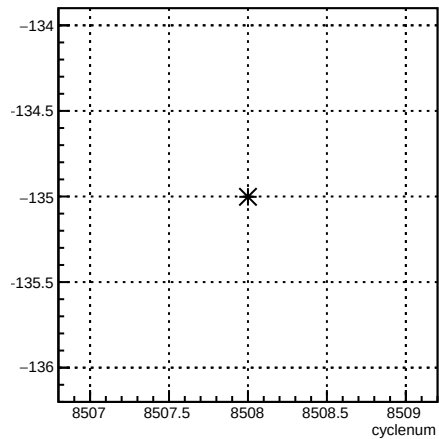
usr_4eY:cyclenum {run == 7257}
