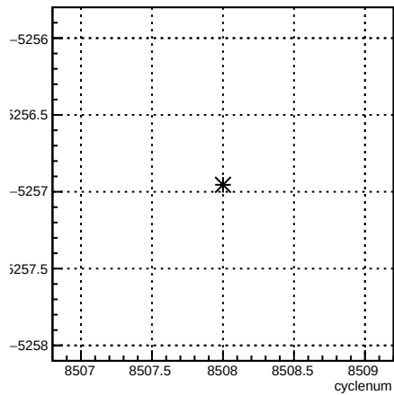
usr_coil7:cyclenum {run == 7257}
