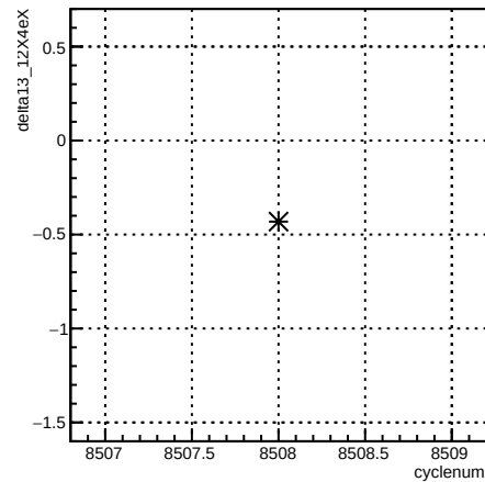
delta13_12X4eX:cyclenum {run == 7257}
