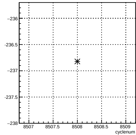
12X_coil6:cyclenum {run == 7257}
