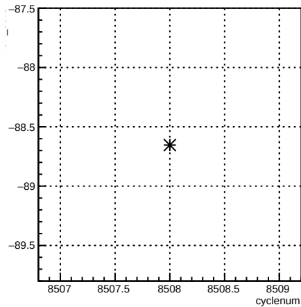
4eX_coil3:cyclenum {run == 7257}
