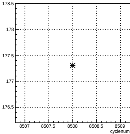
4aY_coil4:cyclenum {run == 7257}
