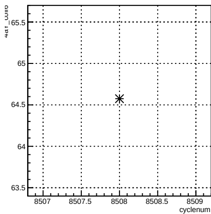
4aY_coil6:cyclenum {run == 7257}
