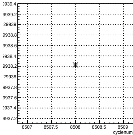
usl_coil1:cyclenum {run == 7257}
