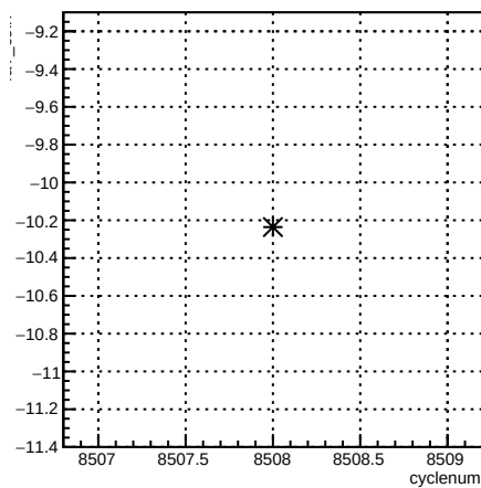
4aY_coil7:cyclenum {run == 7257}
