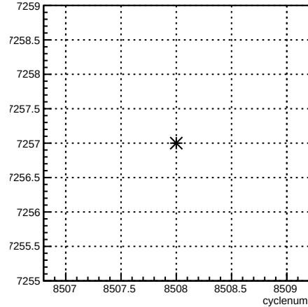
run:cyclenum {run == 7257}
