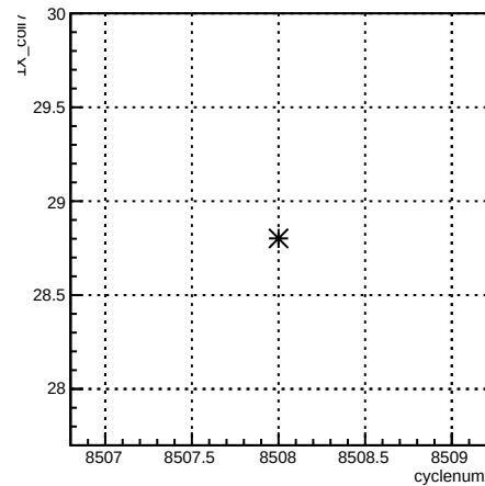
1X_coil7:cyclenum {run == 7257}
