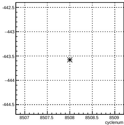
12X_coil7:cyclenum {run == 7257}
