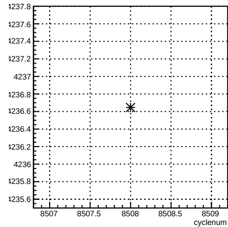
usl_coil4:cyclenum {run == 7257}
