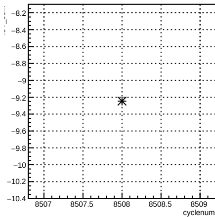
4eY_coil7:cyclenum {run == 7257}
