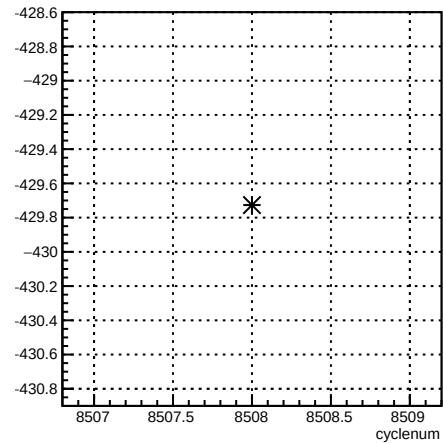
1X_coil1:cyclenum {run == 7257}
