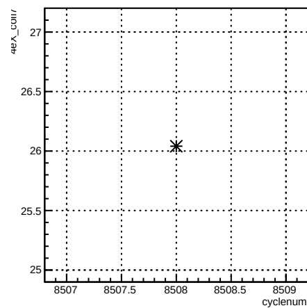
4eX_coil7:cyclenum {run == 7257}
