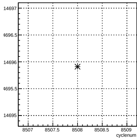
usl_coil7:cyclenum {run == 7257}
