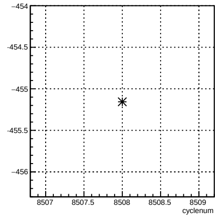
4eX_coil1:cyclenum {run == 7257}
