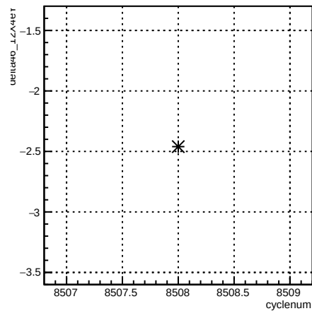
delta46_12X4eY:cyclenum {run == 7257}
