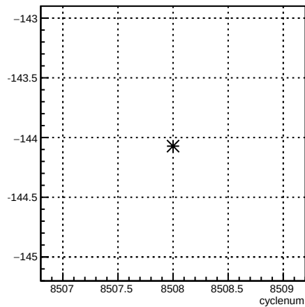
usl_coil6:cyclenum {run == 7257}
