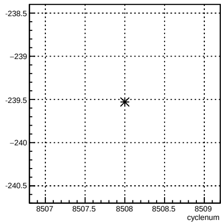
usr_coil6:cyclenum {run == 7257}
