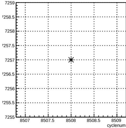
run:cyclenum {run == 7257}
