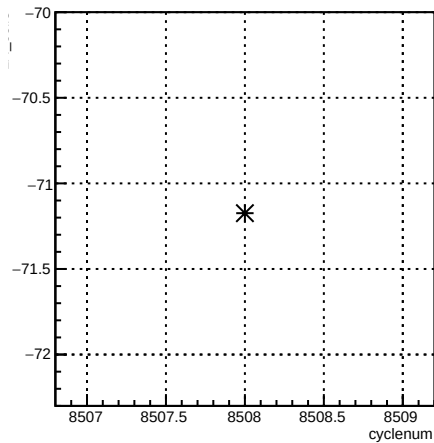
1X_coil3:cyclenum {run == 7257}
