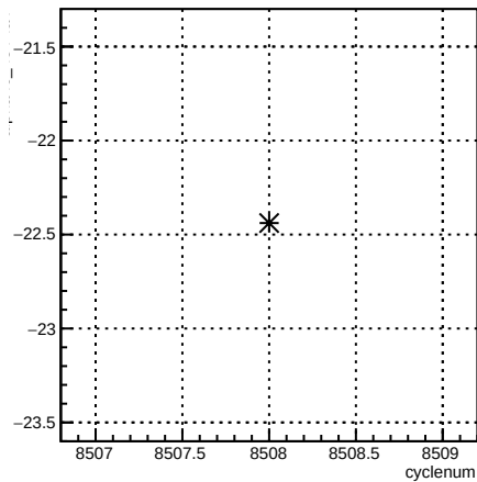
alpha46_4eY4aY:cyclenum {run == 7257}
