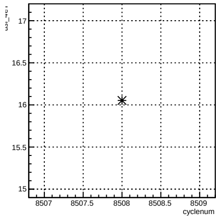
usl_4eY:cyclenum {run == 7257}
