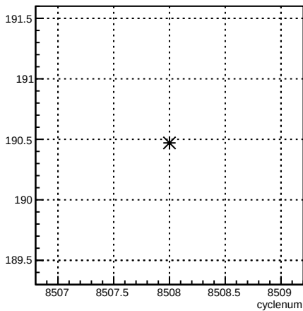
4eY_coil4:cyclenum {run == 7257}
