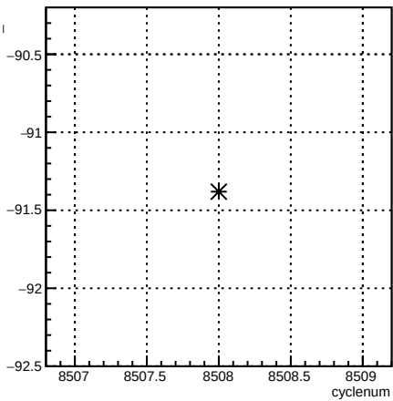
usl_4eY:cyclenum {run == 7257}
