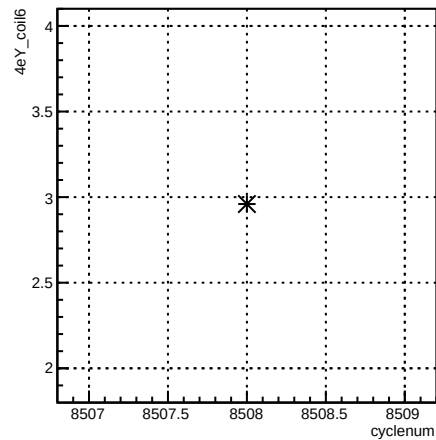
4eY_coil6:cyclenum {run == 7257}
