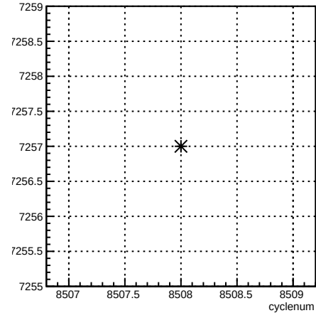
run:cyclenum {run == 7257}
