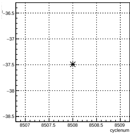
usr_12X:cyclenum {run == 7257}
