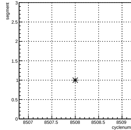
segment:cyclenum {run == 7257}
