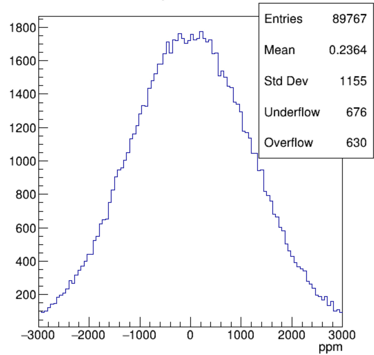
asym_sam6
