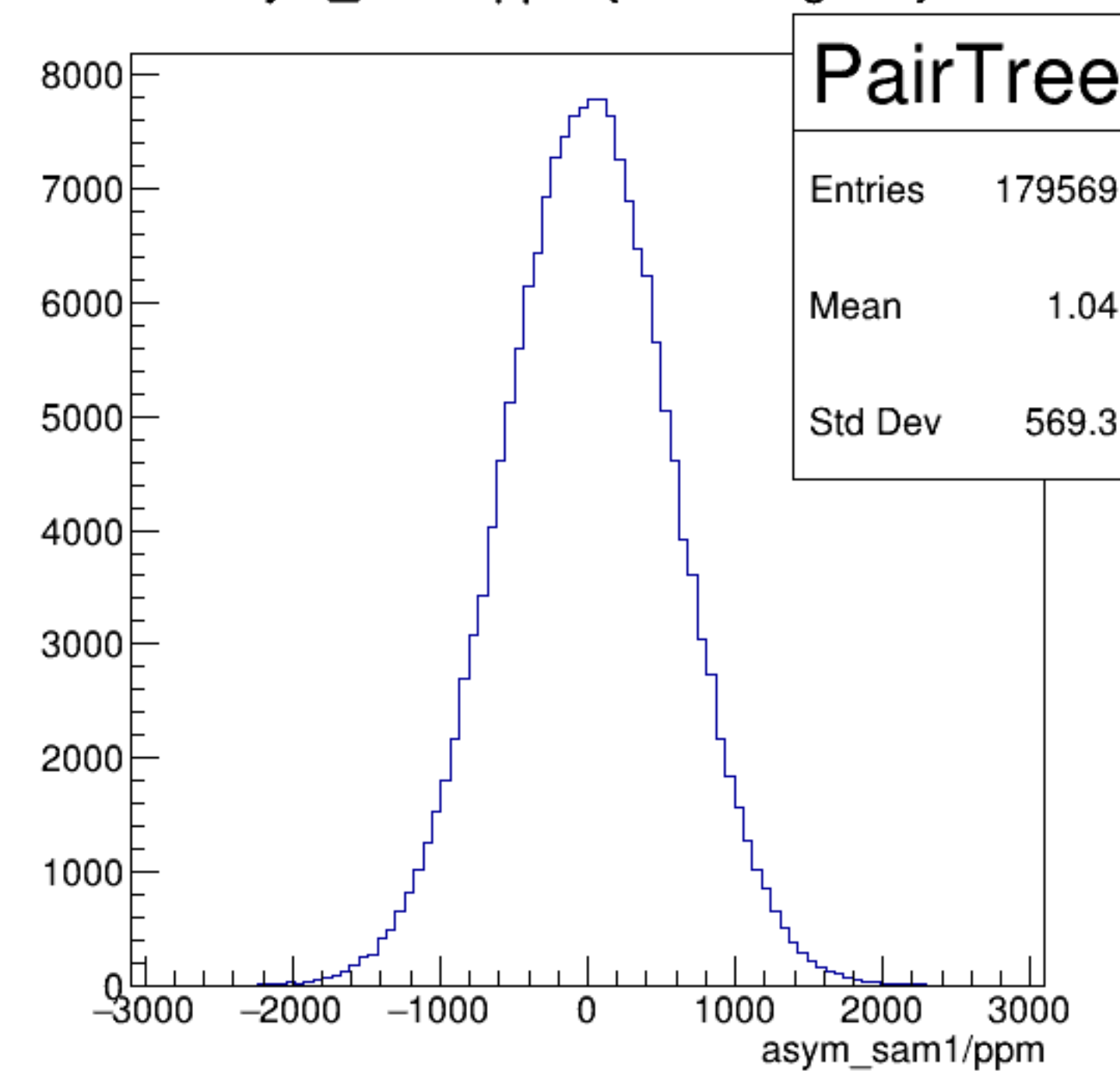
asym_sam1/ppm {ErrorFlag==0}
