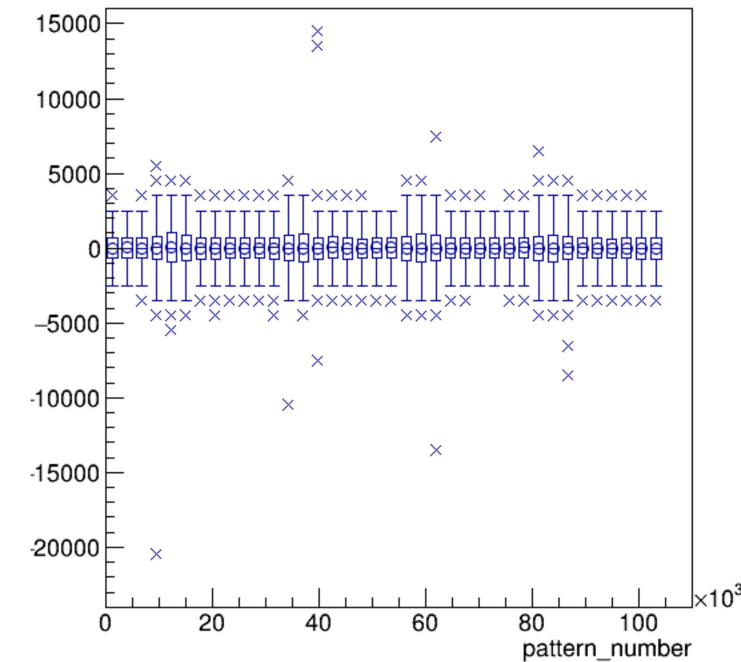
asym_sam3/ppm:pattern_number {ErrorFlag==0}
