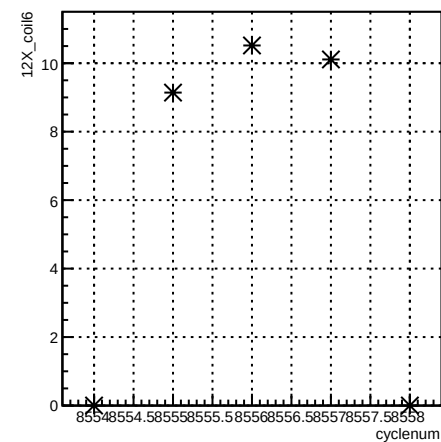
12X_coil6:cyclenum {run == 7266}
