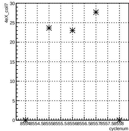
4eX_coil7:cyclenum {run == 7266}
