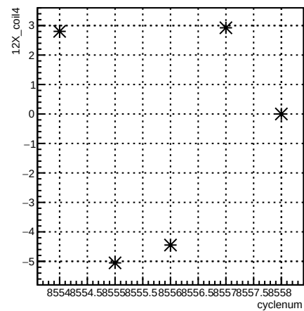
12X_coil4:cyclenum {run == 7266}
