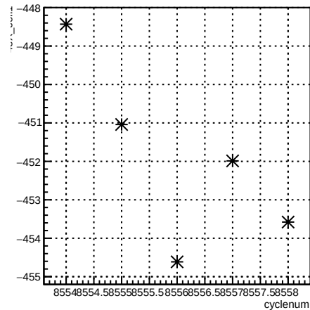
4eX_coil1:cyclenum {run == 7266}
