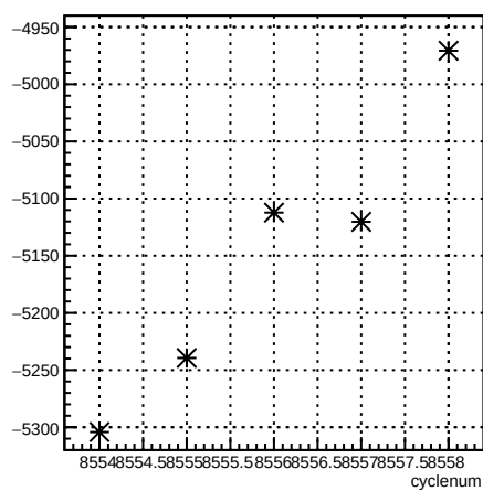
usr_coil3:cyclenum {run == 7266}
