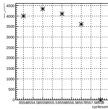
usr_coil4:cyclenum {run == 7266}
