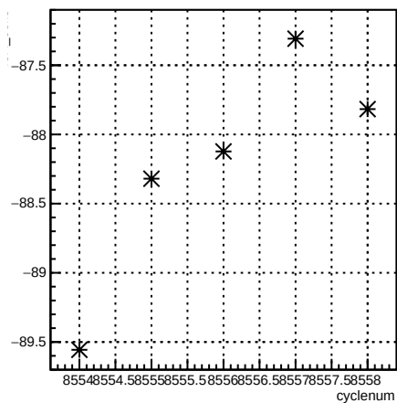
4eX_coil3:cyclenum {run == 7266}
