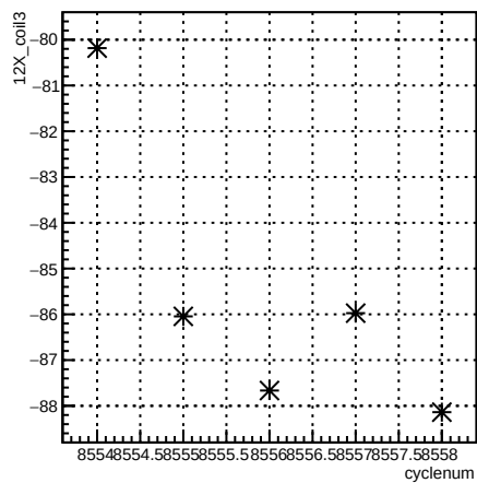
12X_coil3:cyclenum {run == 7266}
