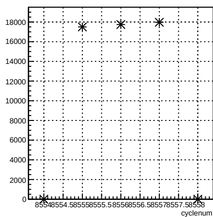
usr_coil7:cyclenum {run == 7266}
