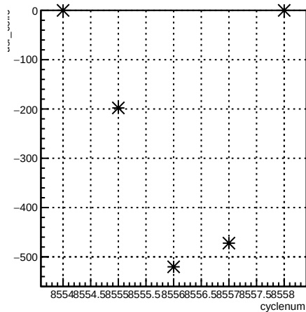
usr_coil6:cyclenum {run == 7266}
