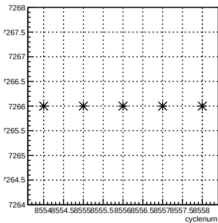
run:cyclenum {run == 7266}
