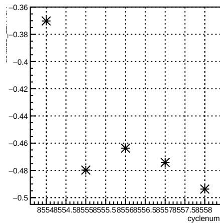
delta13_12X4eX:cyclenum {run == 7266}
