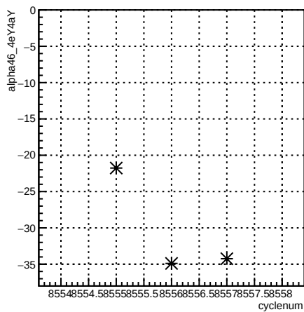
alpha46_4eY4aY:cyclenum {run == 7266}
