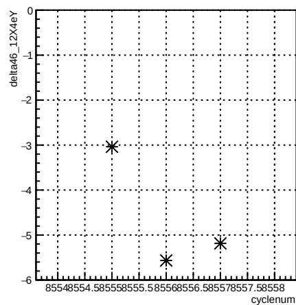
delta46_12X4eY:cyclenum {run == 7266}
