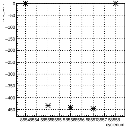
12X_coil7:cyclenum {run == 7266}
