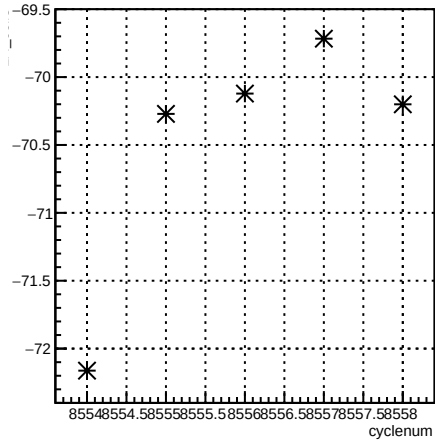
1X_coil3:cyclenum {run == 7266}
