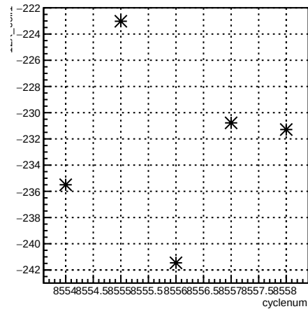
12X_coil1:cyclenum {run == 7266}
