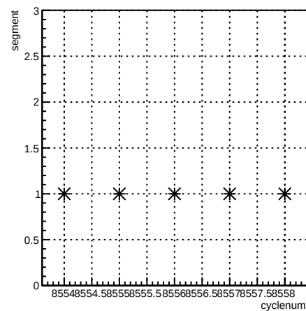
segment:cyclenum {run == 7266}
