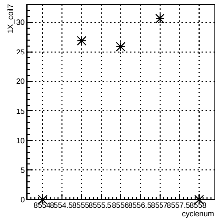
1X_coil7:cyclenum {run == 7266}
