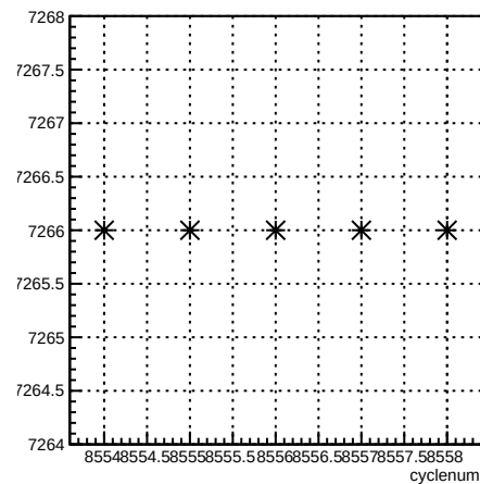
run:cyclenum {run == 7266}
