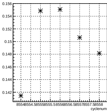
alpha13_4eX1X:cyclenum {run == 7266}
