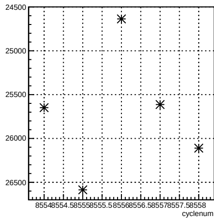
usr_coil1:cyclenum {run == 7266}
