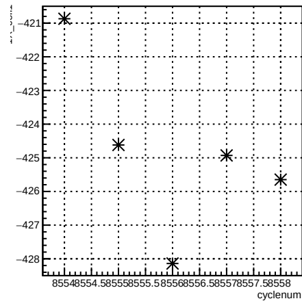
1X_coil1:cyclenum {run == 7266}
