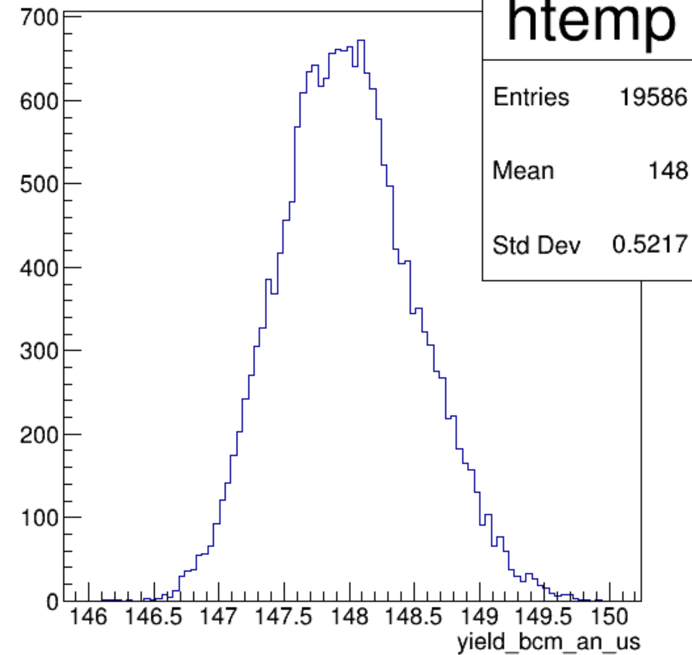
yield_bcm_an_us {ErrorFlag==0}
