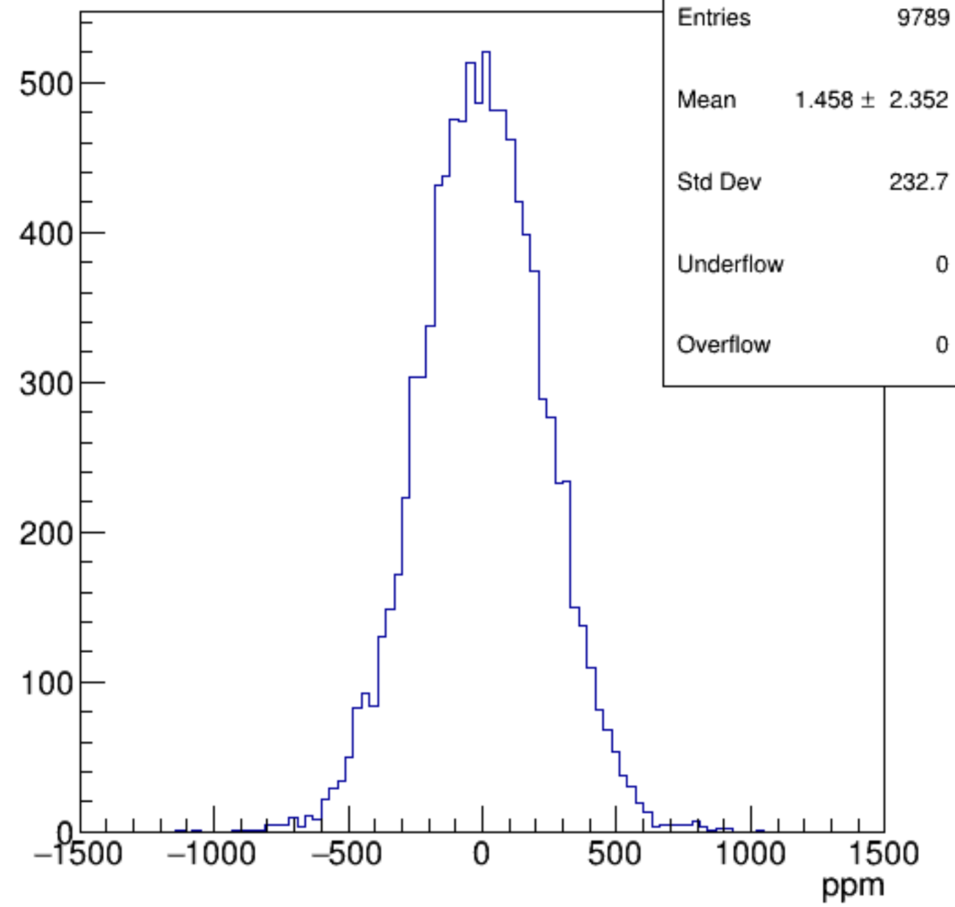
asym_bcm_an_ds3
