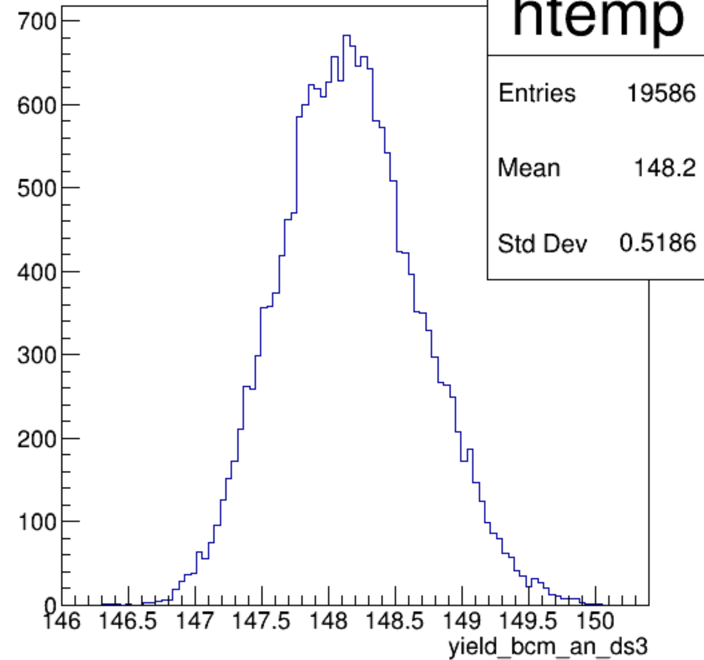
yield_bcm_an_ds3 {ErrorFlag==0}
