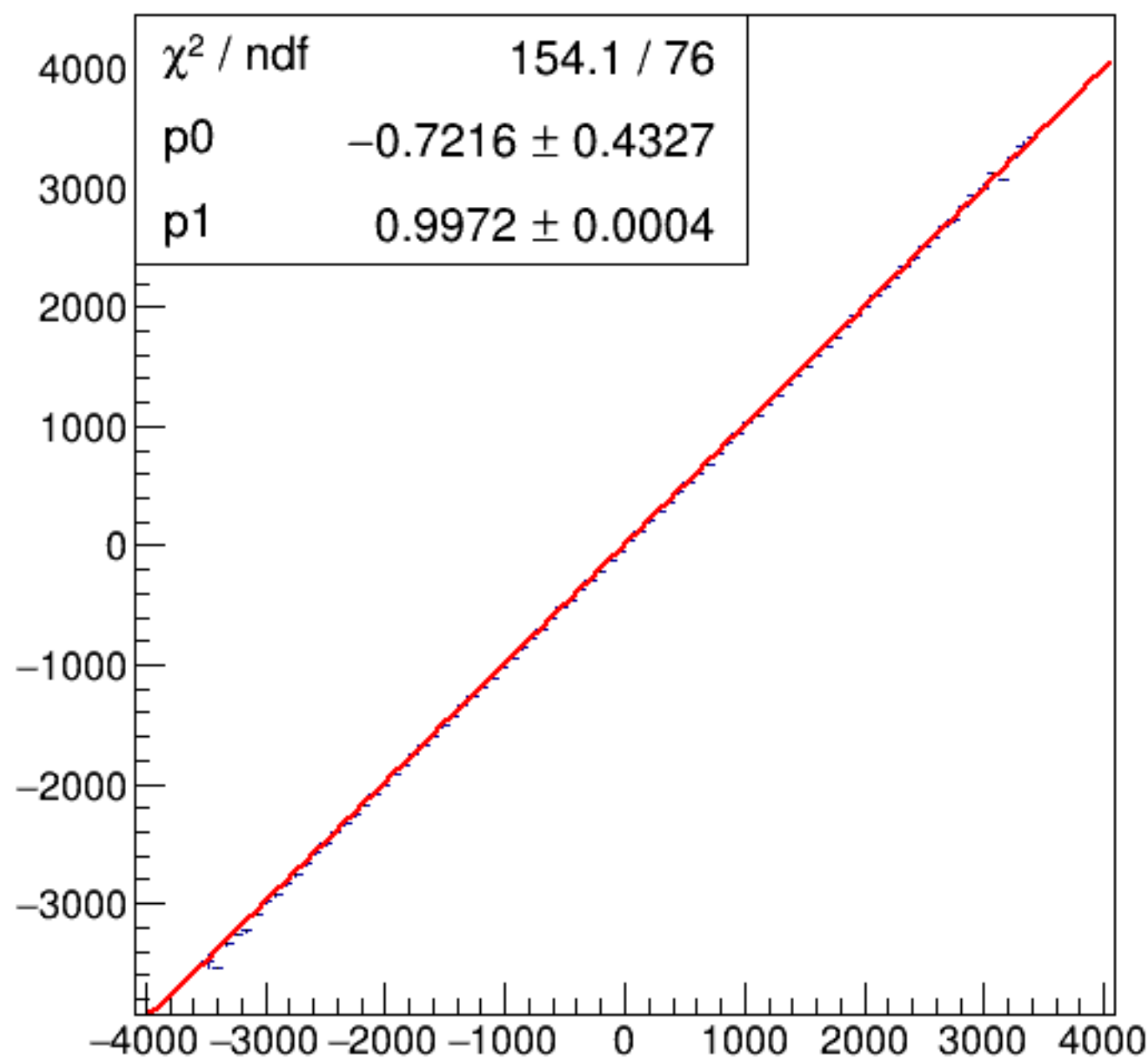
run7268_000_asym_bcm_dg_ds_vs_asym_bcm_an_us_pr.png
