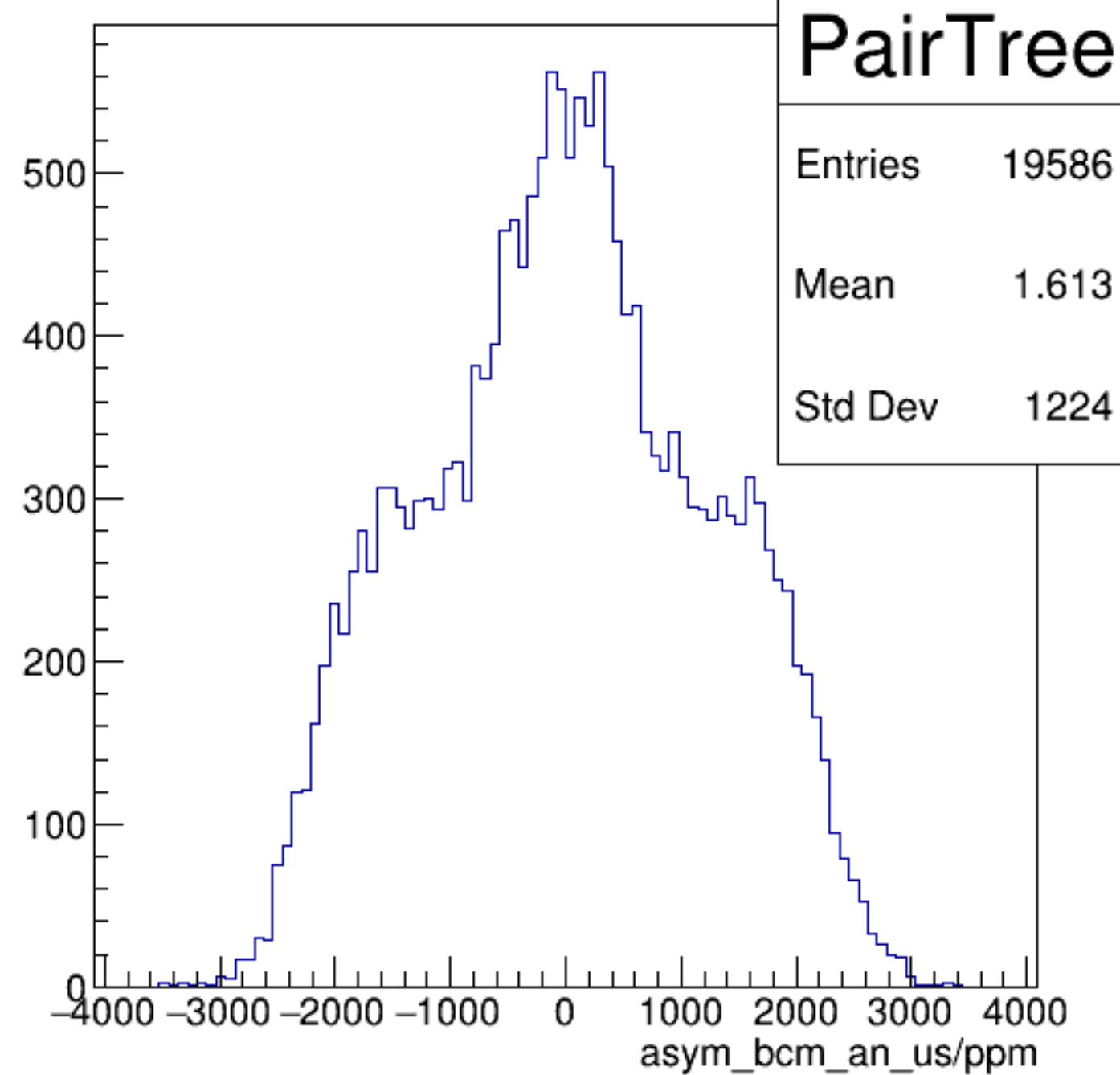
asym_bcm_an_us/ppm {ErrorFlag==0}
