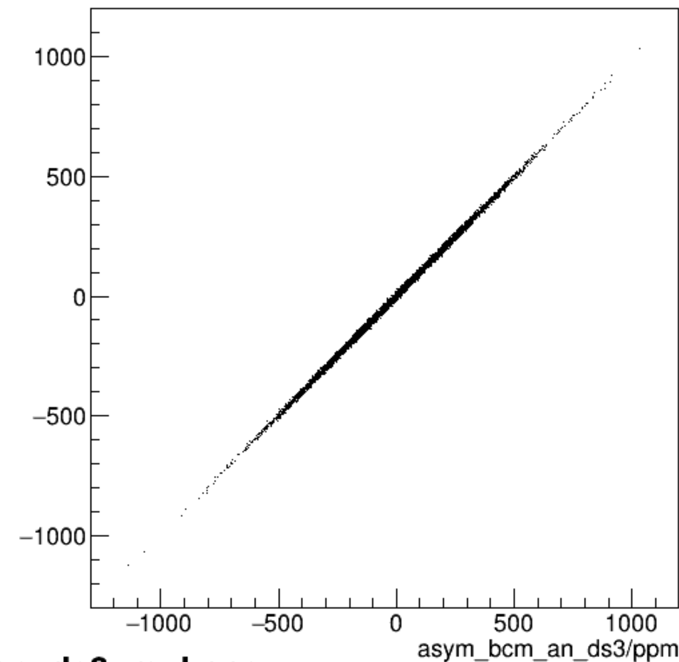
run7268_000_asym_bcm_an_ds_vs_asym_bcm_an_ds3_mul.png
