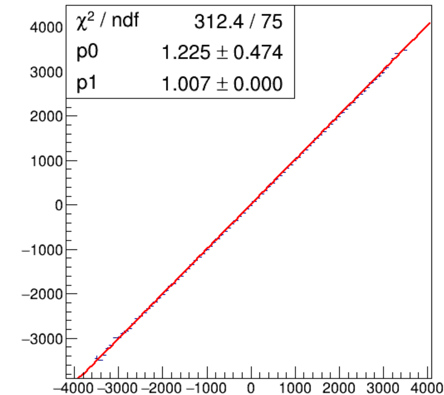
run7268_000_asym_bcm_dg_us_vs_asym_bcm_an_ds3_pr.png
