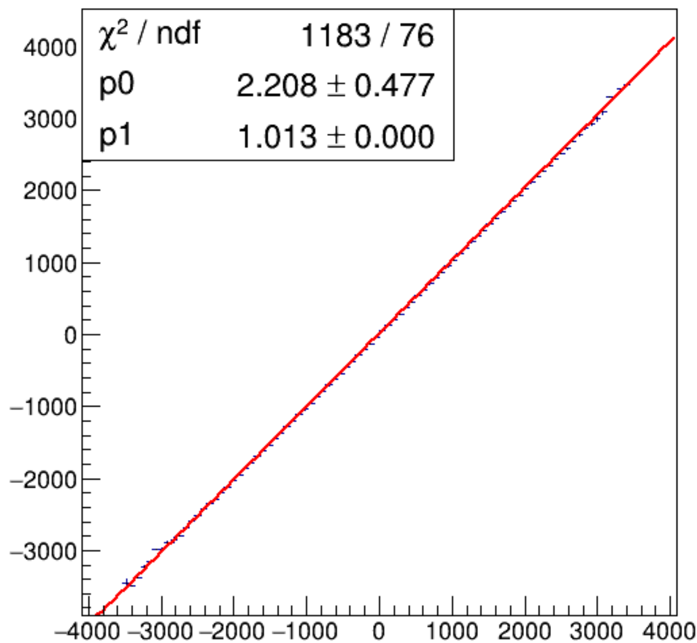
run7268_000_asym_bcm_dg_us_vs_asym_bcm_an_ds_pr.png
