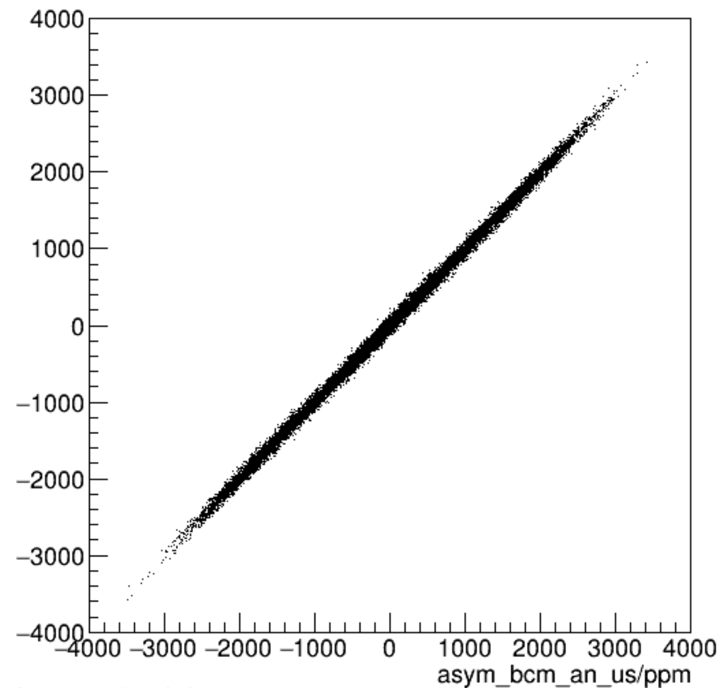
run7268_000_asym_bcm_dg_ds_vs_asym_bcm_an_us_pr.png
