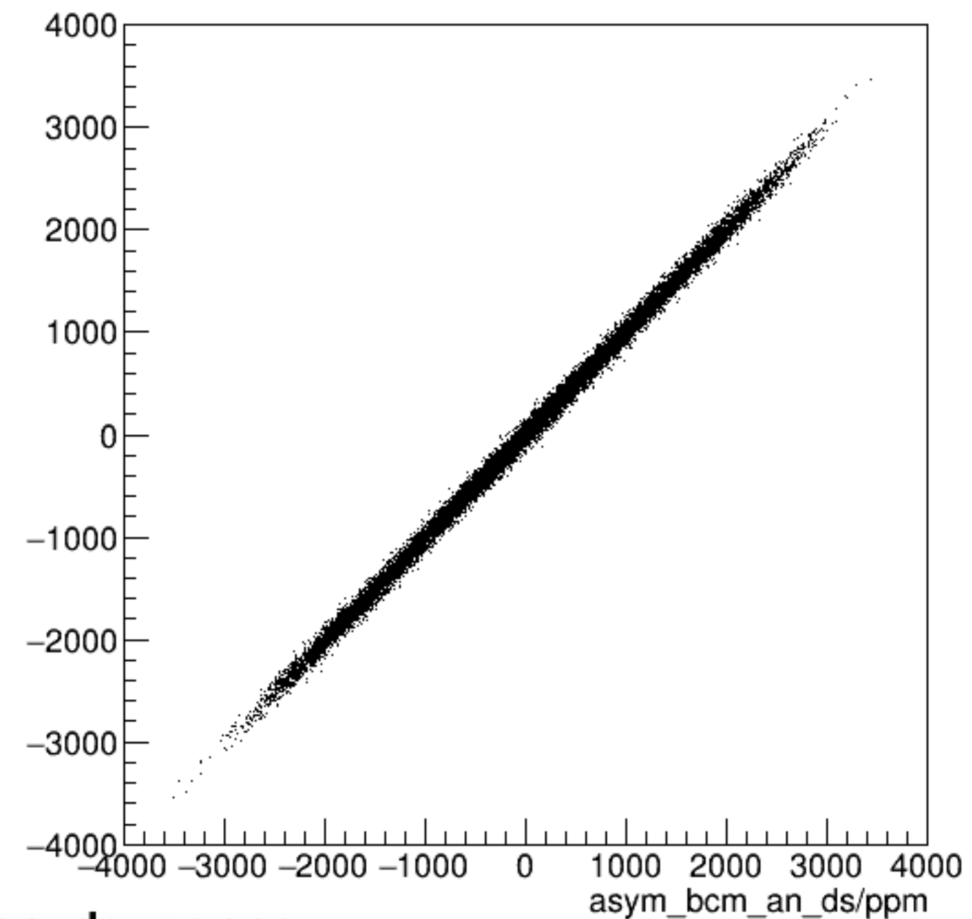
run7268_000_asym_bcm_dg_us_vs_asym_bcm_an_ds_pr.png
