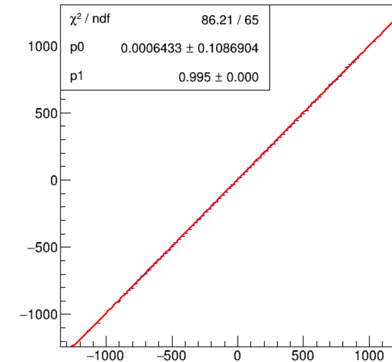
run7268_000_asym_bcm_an_ds_vs_asym_bcm_an_ds3_mul.png
