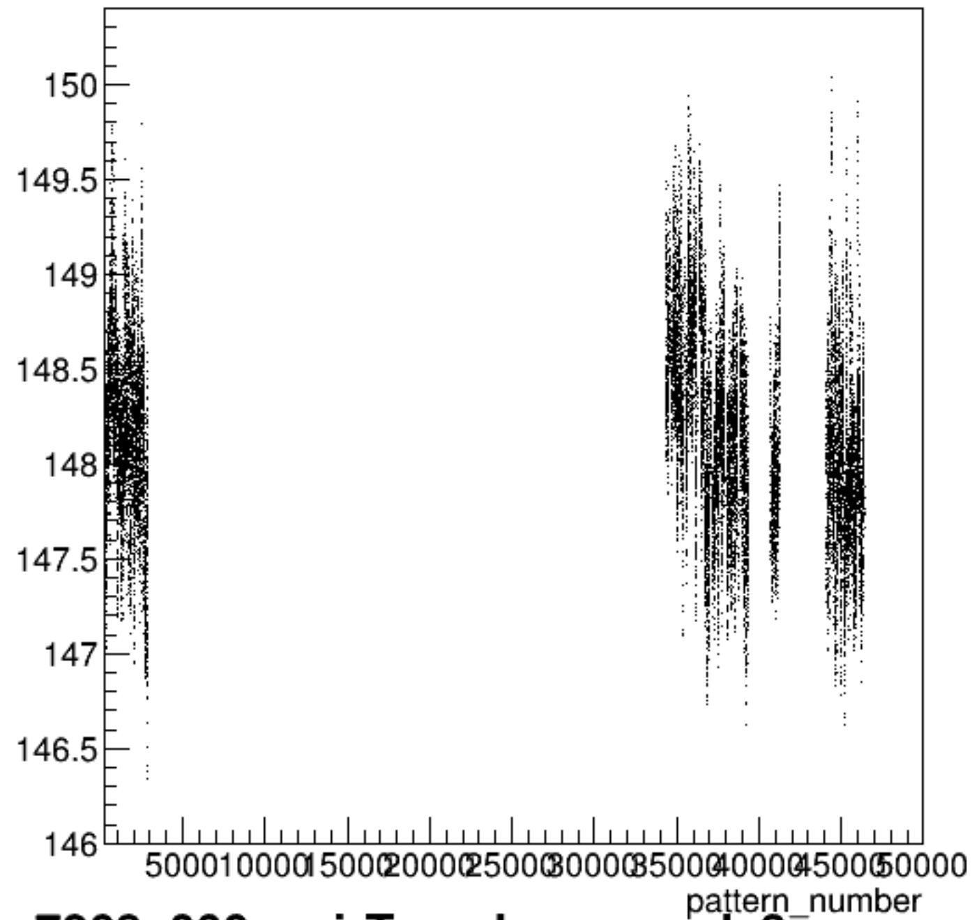
yield_bcm_an_ds3:pattern_number {ErrorFlag==0}
