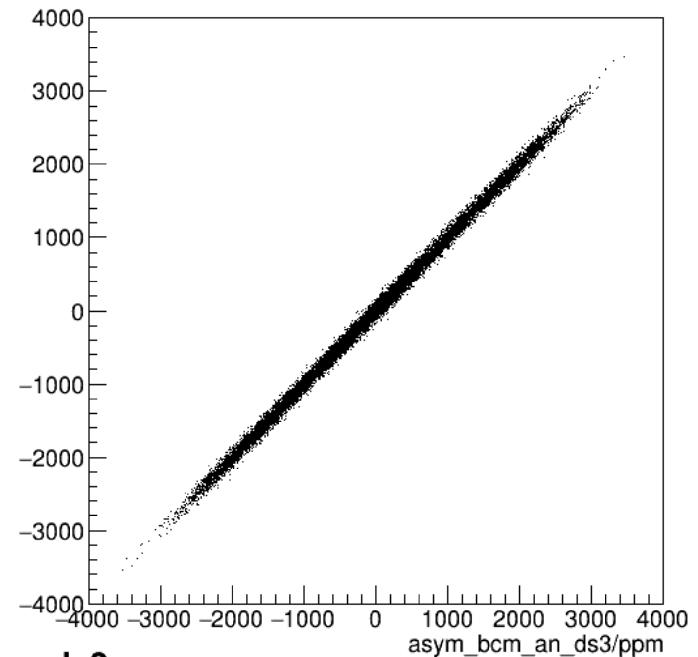
run7268_000_asym_bcm_dg_us_vs_asym_bcm_an_ds3_pr.png
