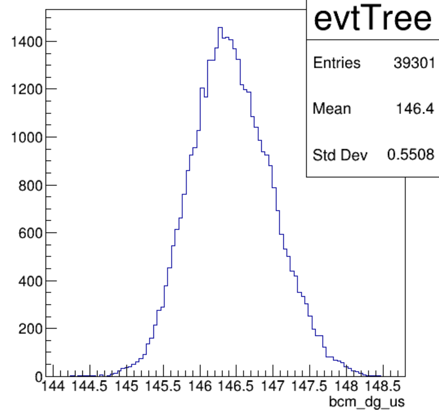
bcm_dg_us {ErrorFlag==0}
