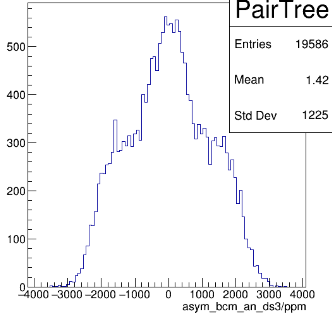
asym_bcm_an_ds3/ppm {ErrorFlag==0}
