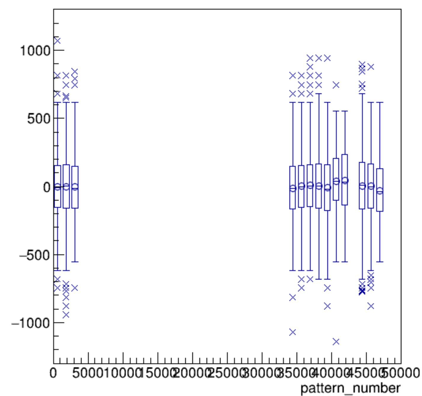
asym_bcm_dg_us/ppm:pattern_number {ErrorFlag==0}
