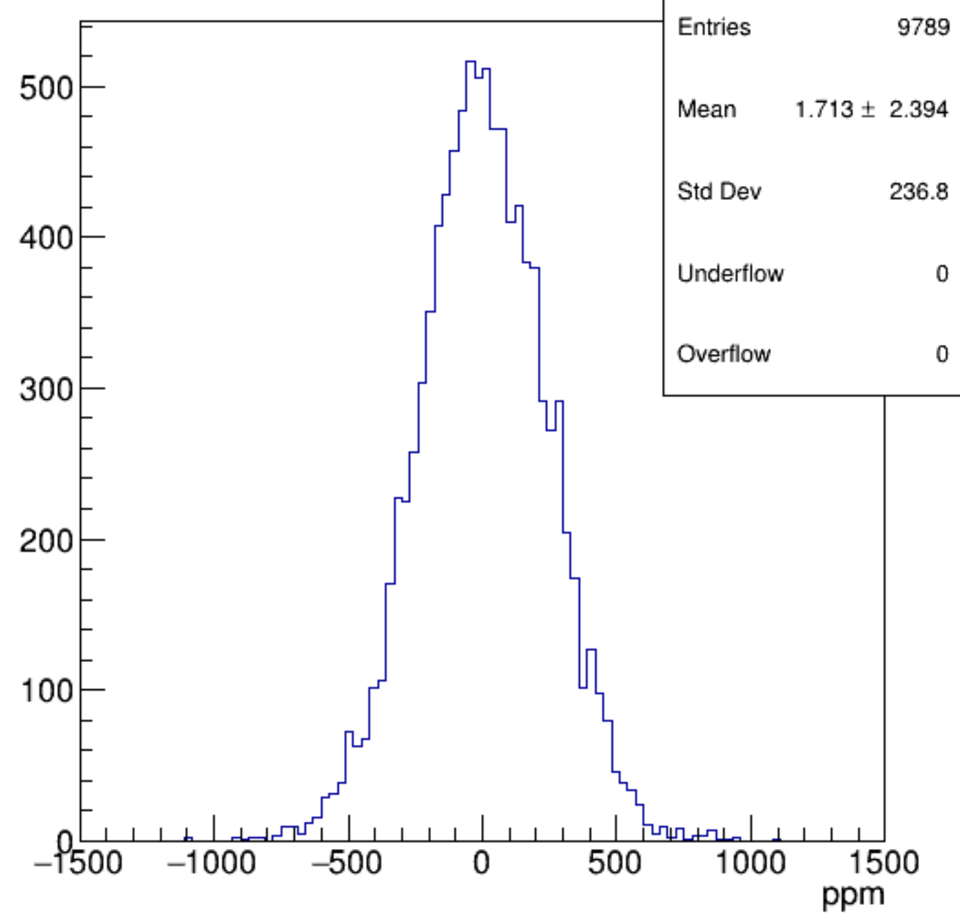
asym_bcm_dg_us
