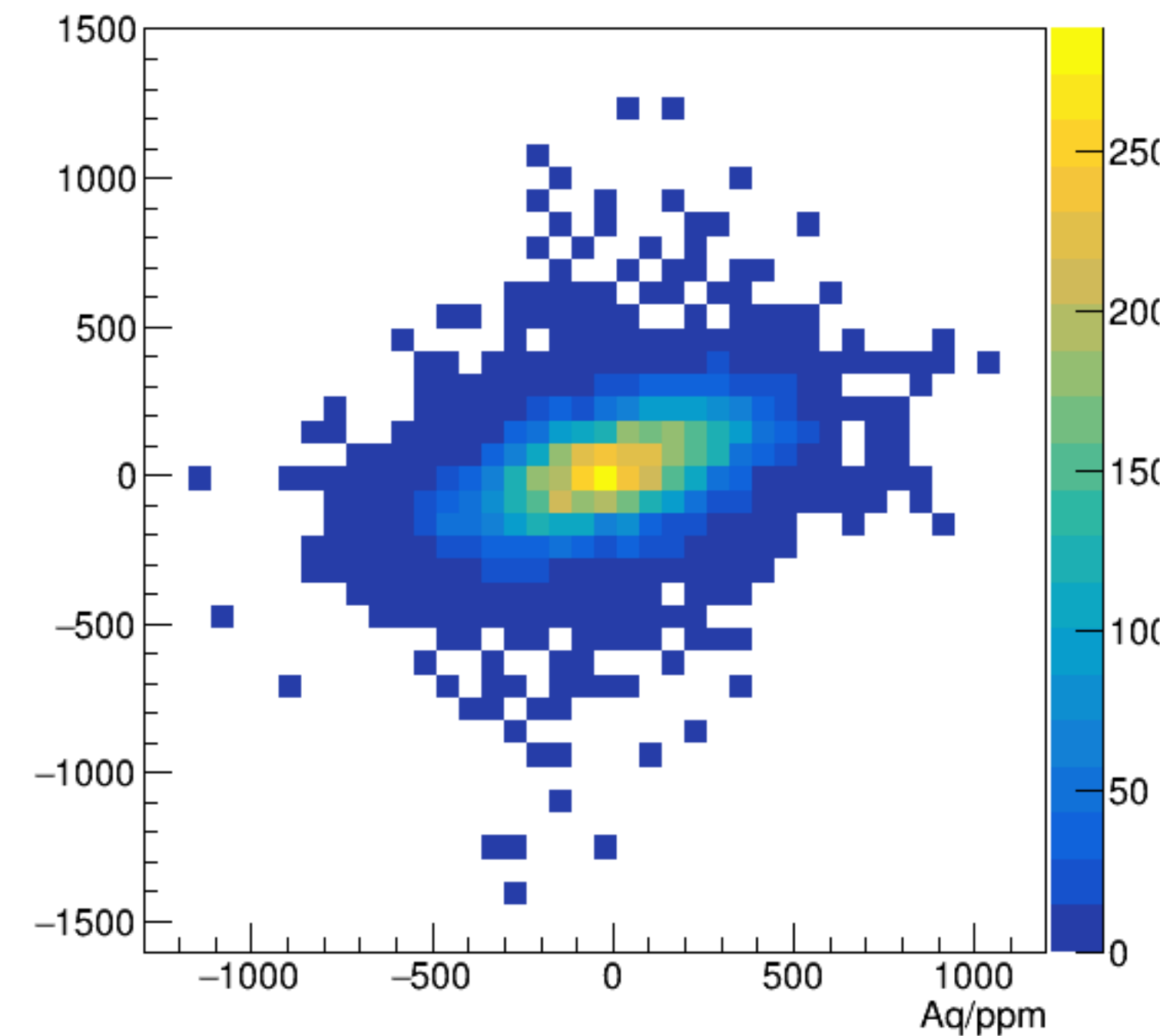
asym_bpm0i01aWS/ppm:Aq/ppm {ErrorFlag==0}
