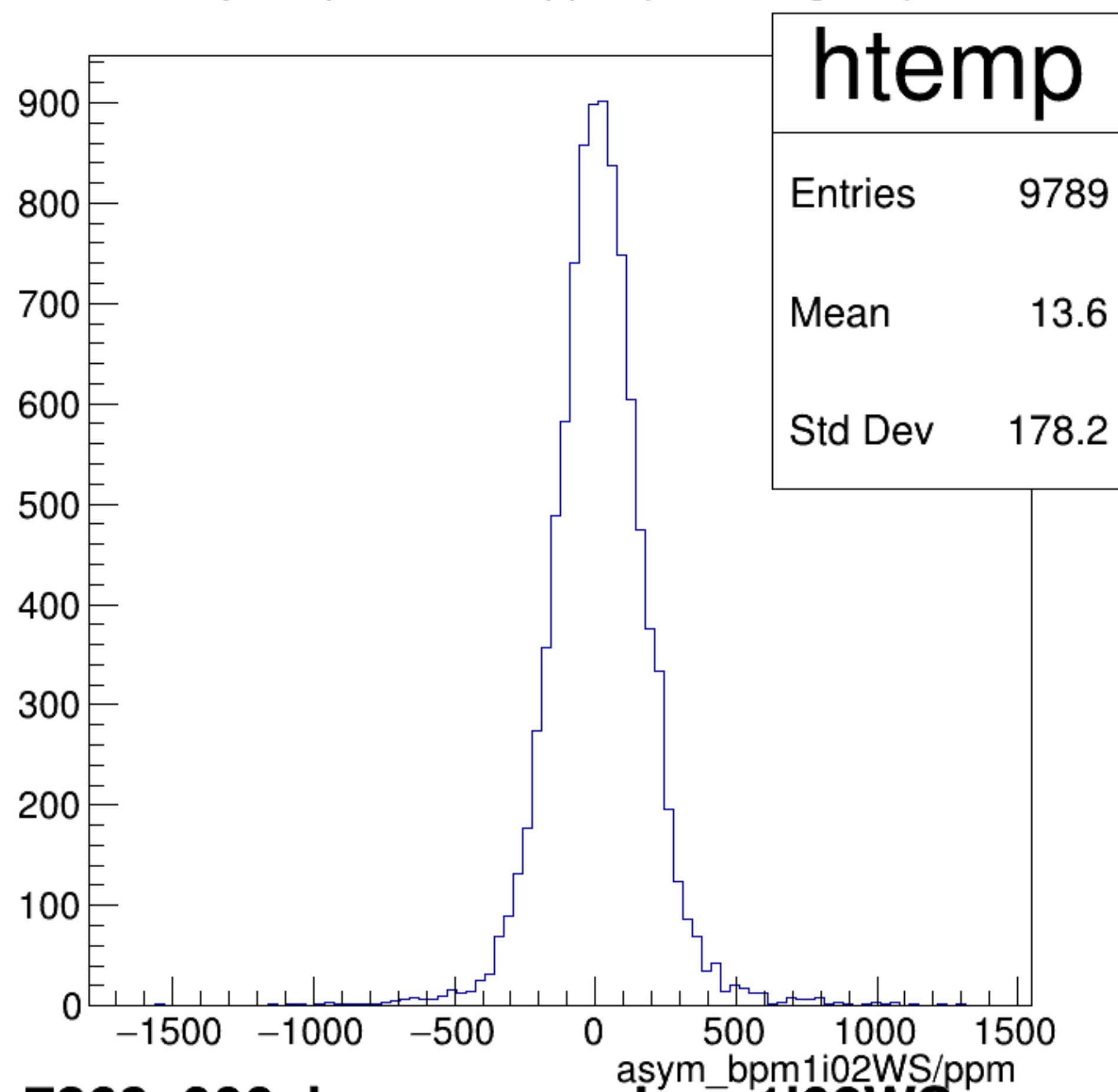
asym_bpm1i02WS/ppm {ErrorFlag==0}
