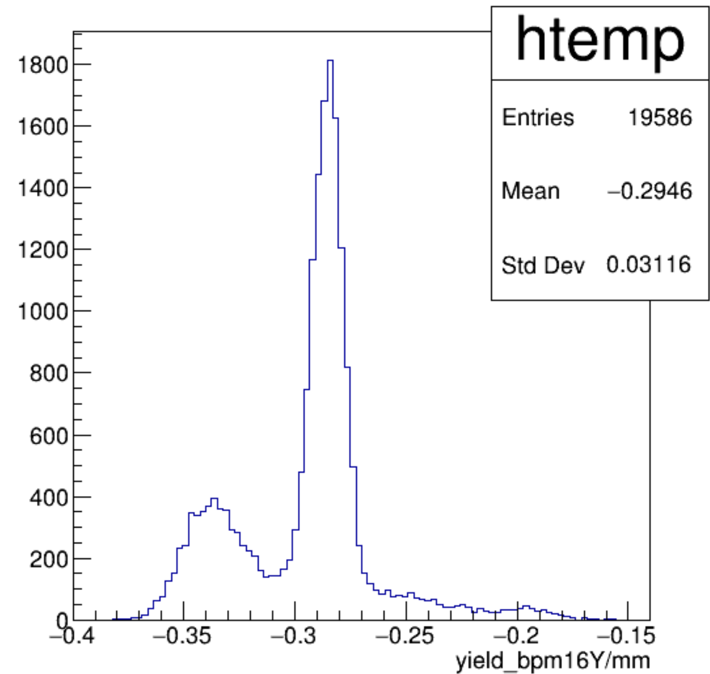
yield_bpm16Y/mm {ErrorFlag==0}
