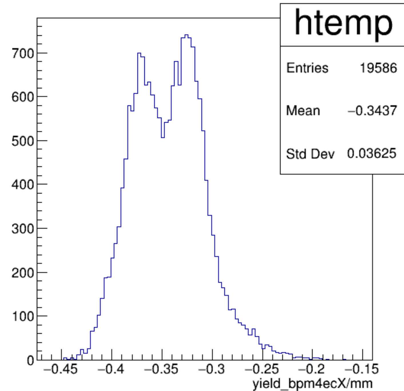
yield_bpm4ecX/mm {ErrorFlag==0}
