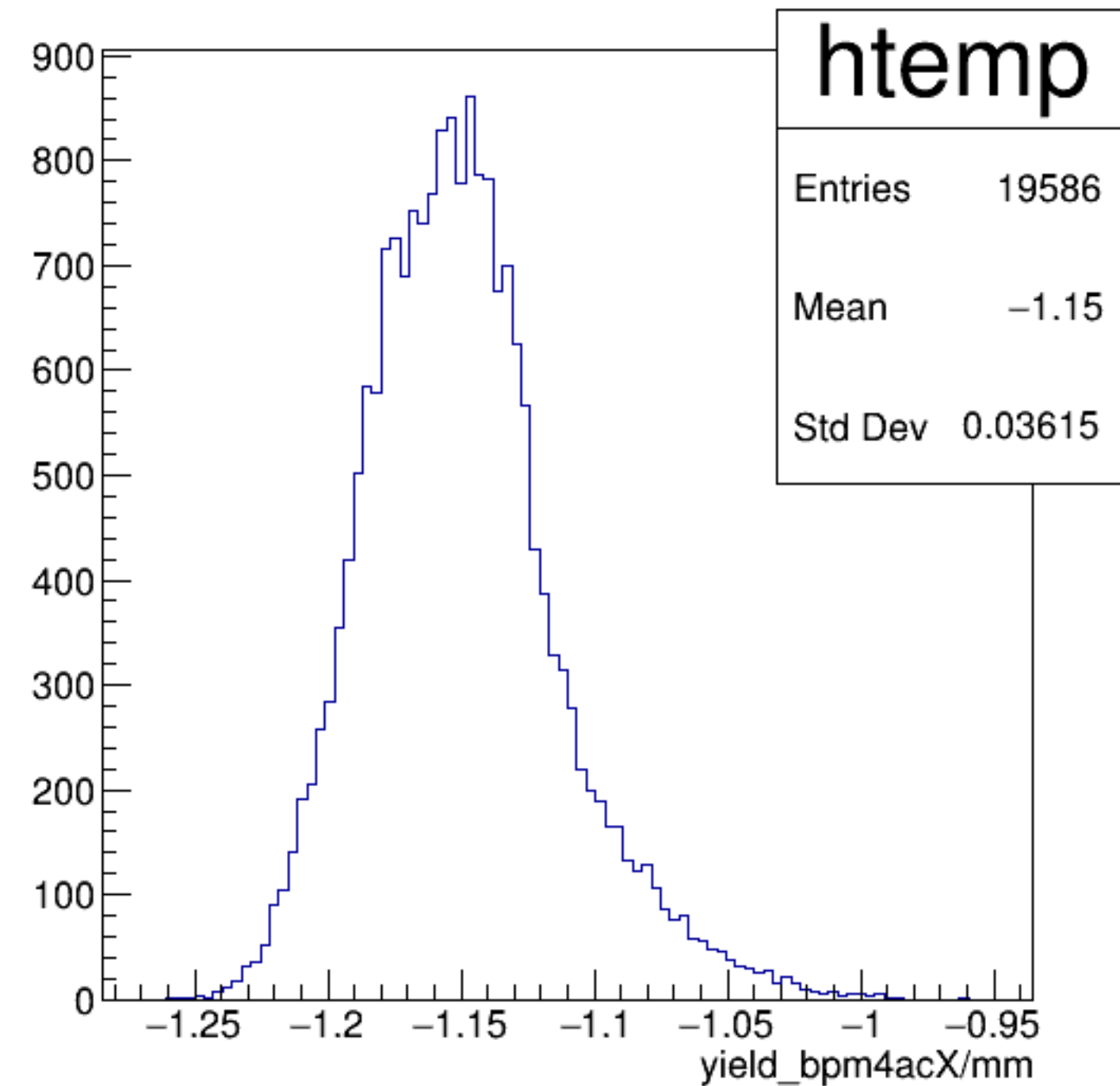
yield_bpm4acX/mm {ErrorFlag==0}
