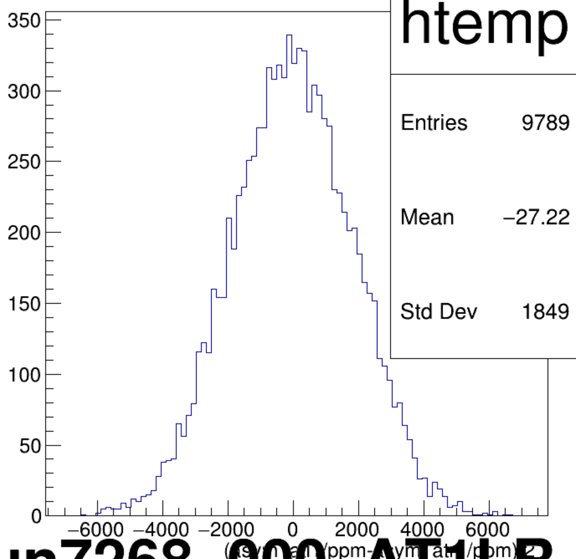
(asym_atl1/ppm-asym_atr1/ppm)/2 {ok_cut}
