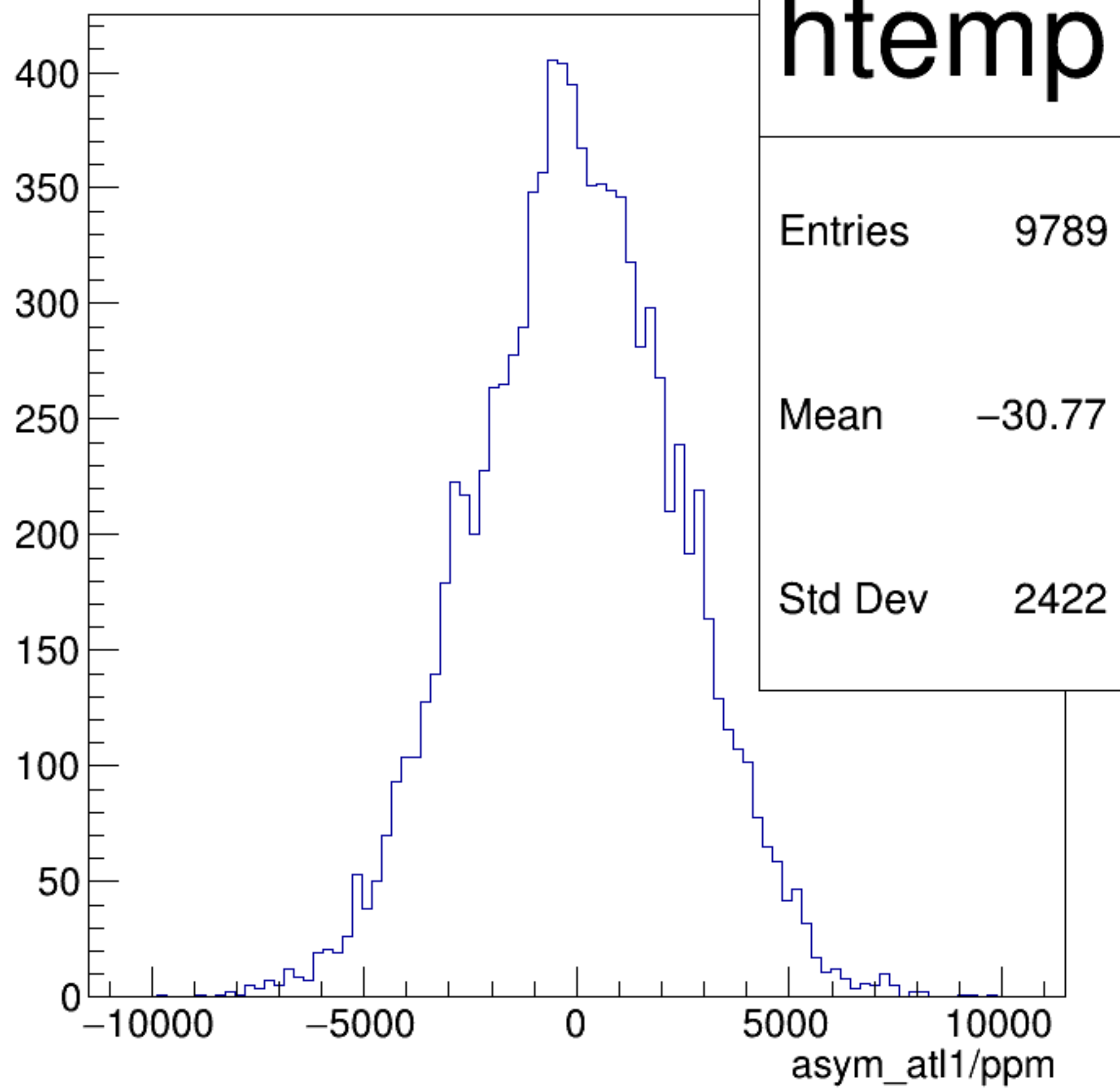
asym_atl1/ppm {ok_cut}
