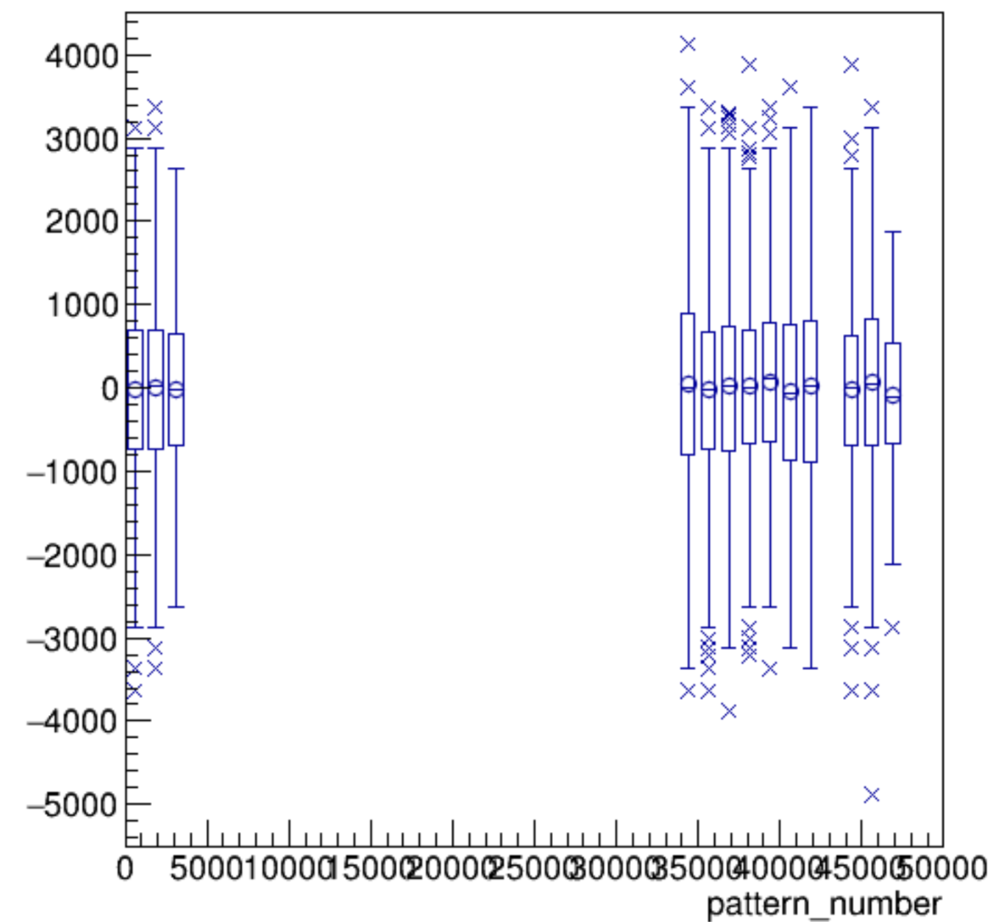
asym_sam5/ppm:pattern_number {ErrorFlag==0}
