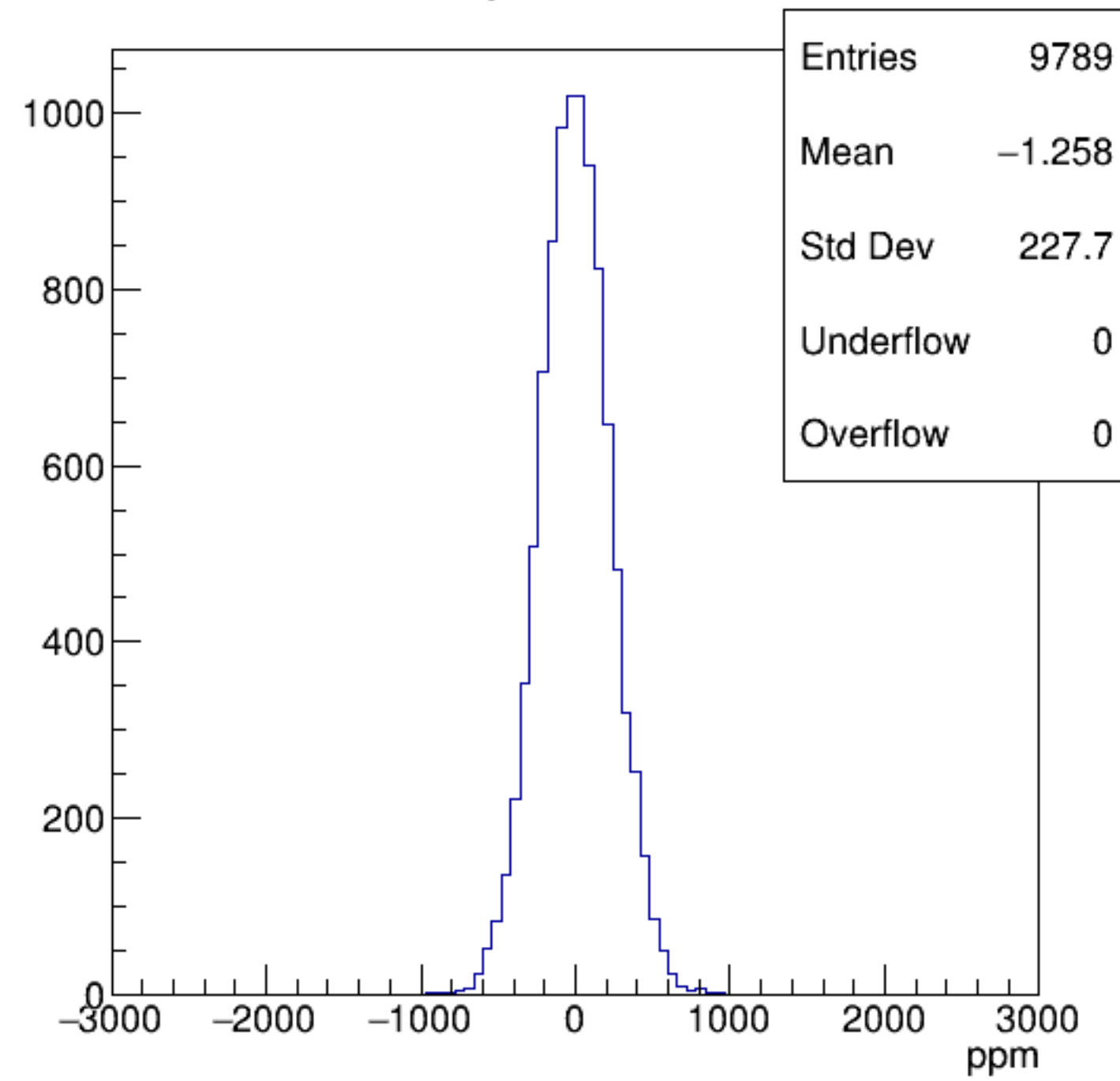
asym_sam8
