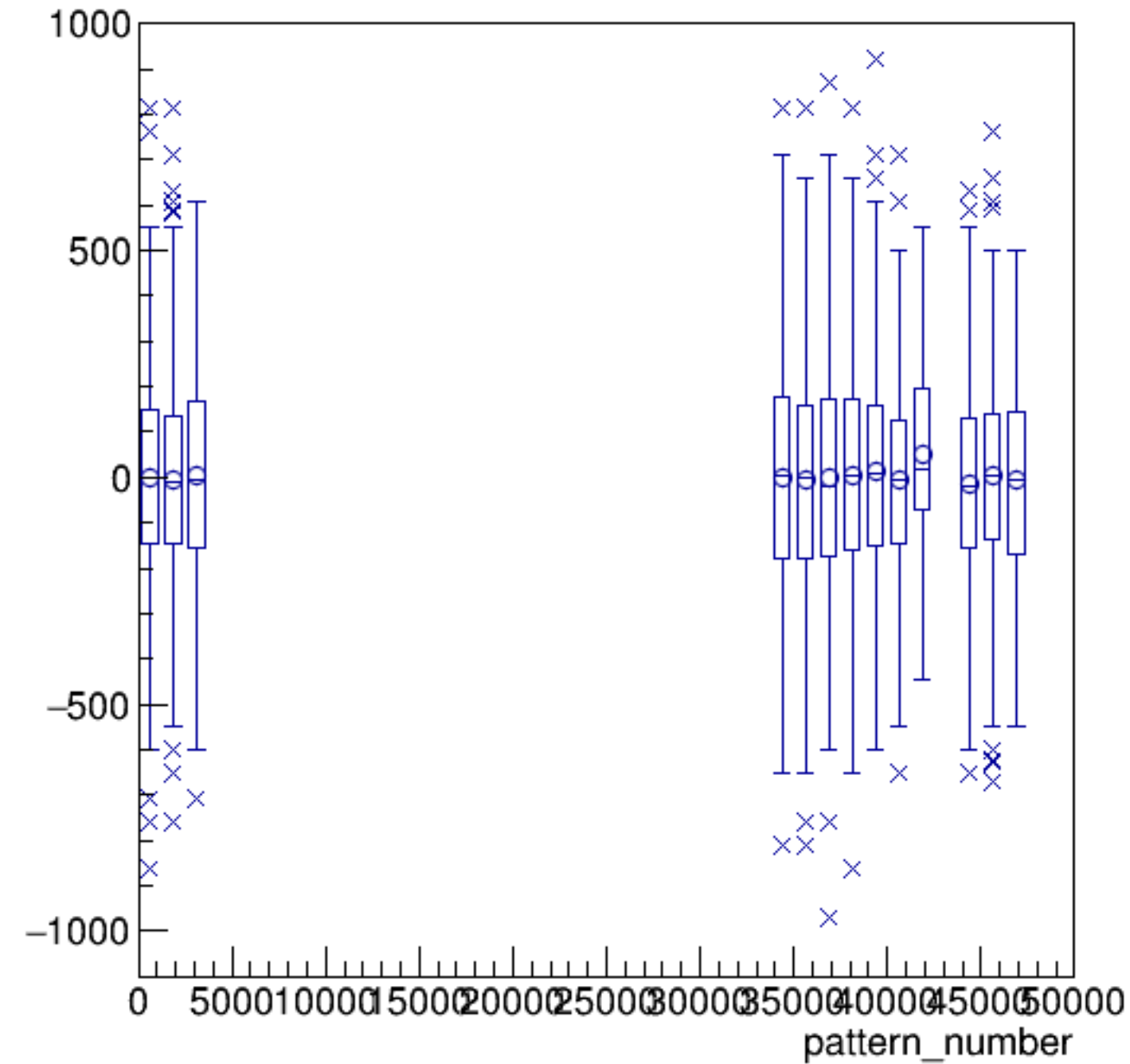
asym_sam8/ppm:pattern_number {ErrorFlag==0}
