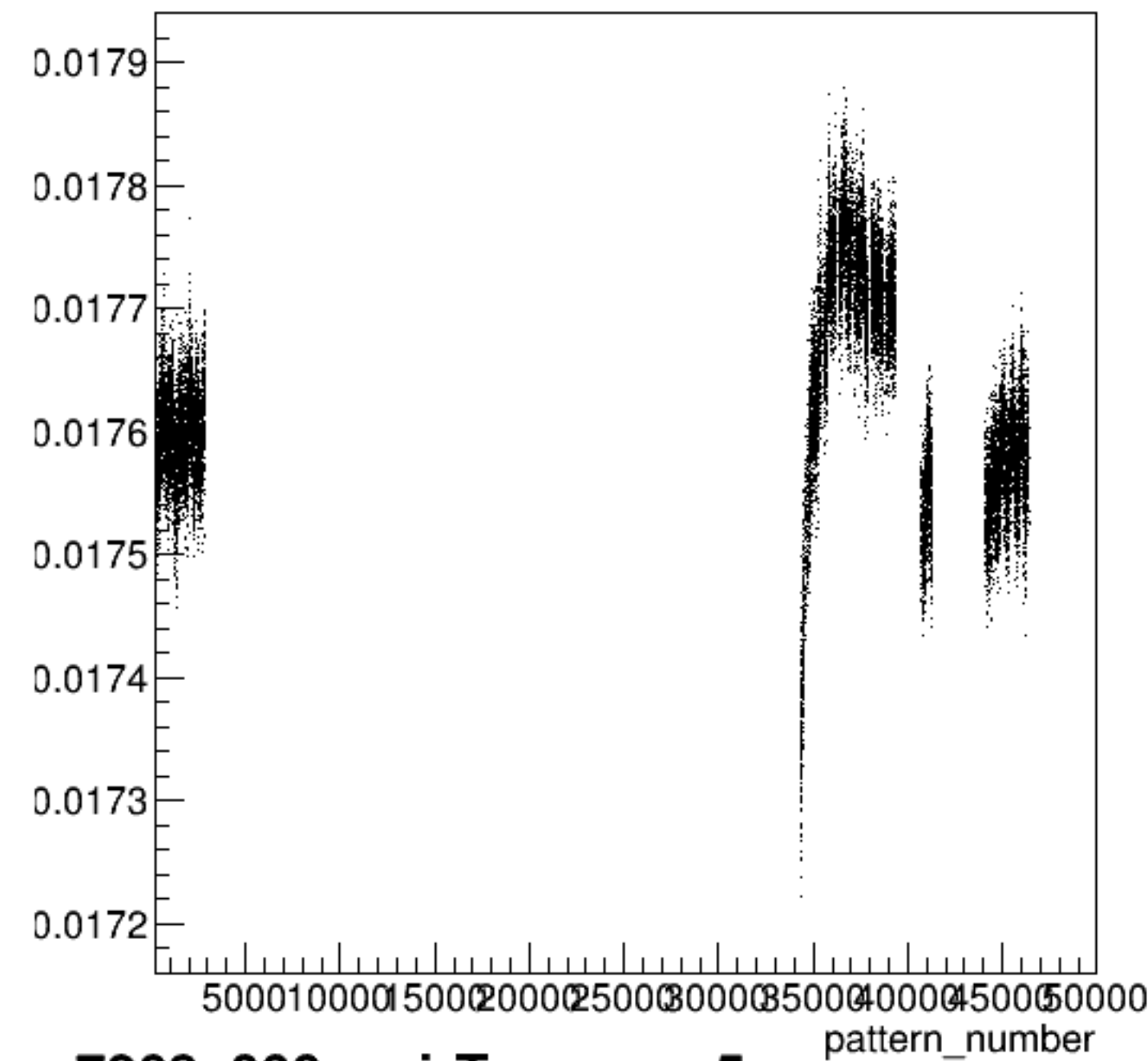
yield_sam5:pattern_number {ErrorFlag==0}
