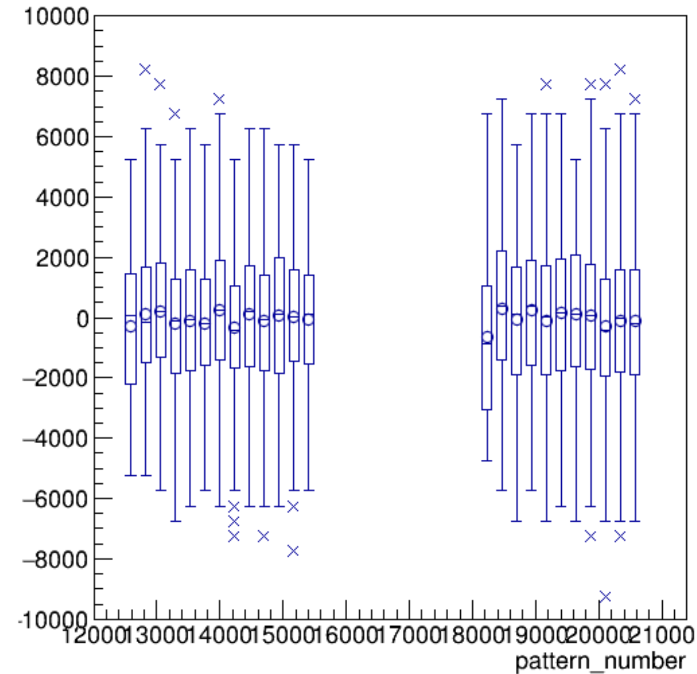
asym_atr1/ppm:pattern_number {ErrorFlag==0}
