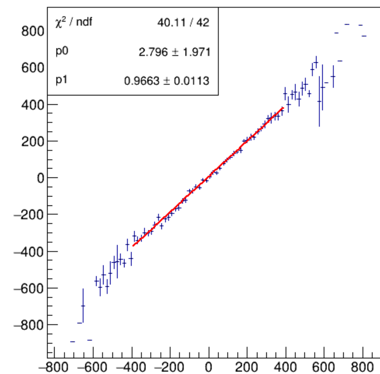
asym_bpm1WS/ppm:Aq/ppm {ErrorFlag==0}
