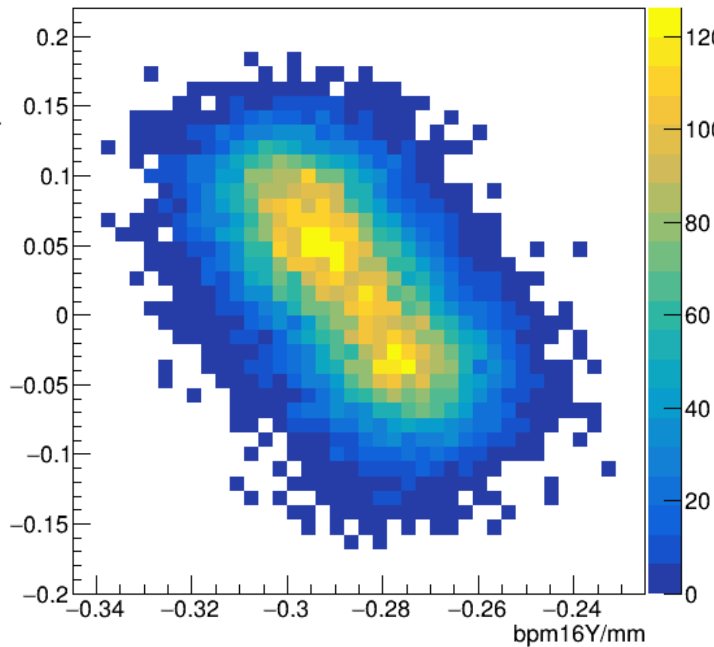
bpm16X/mm:bpm16Y/mm {ErrorFlag==0}
