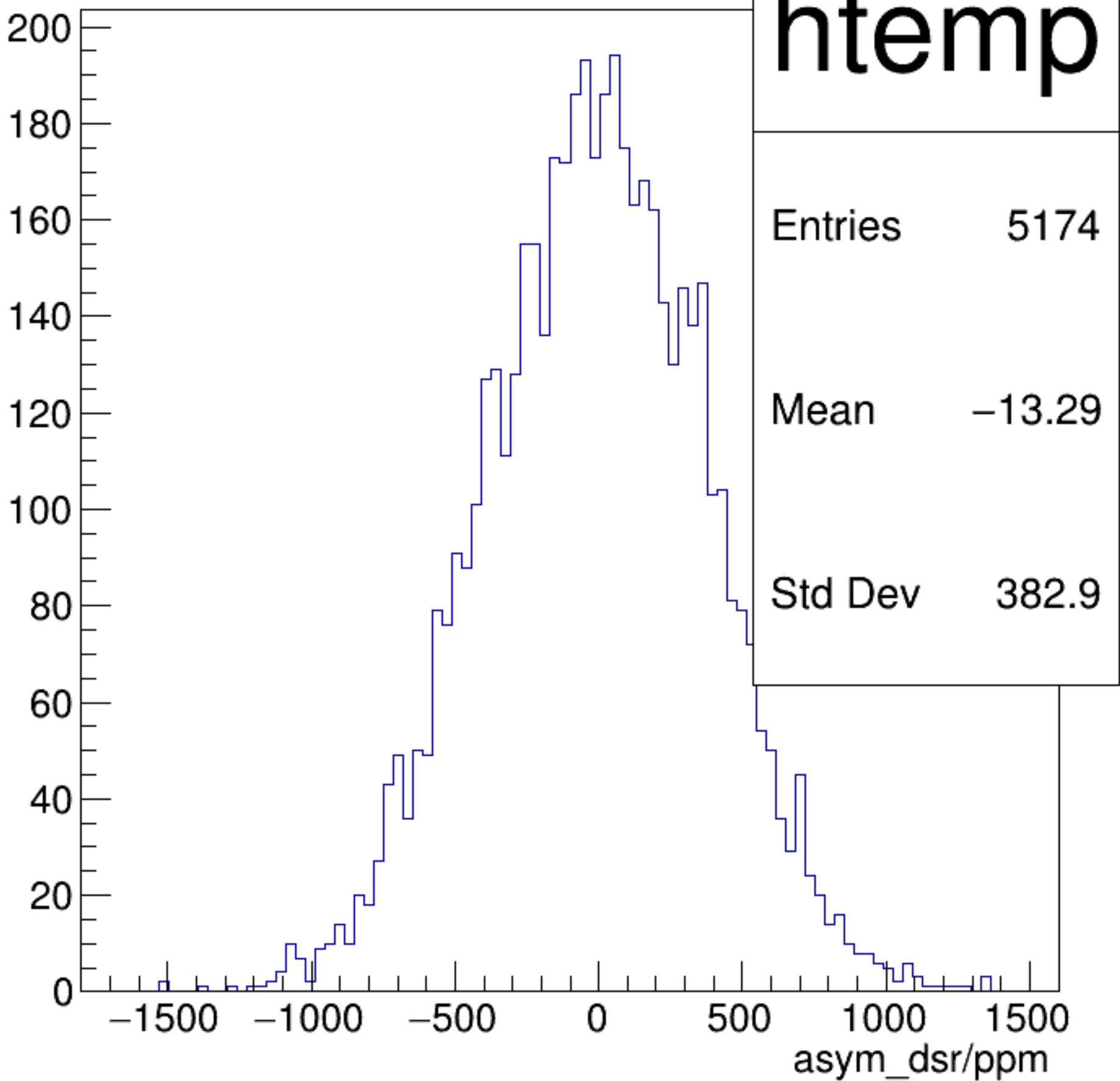
asym_dsr/ppm {ok_cut}
