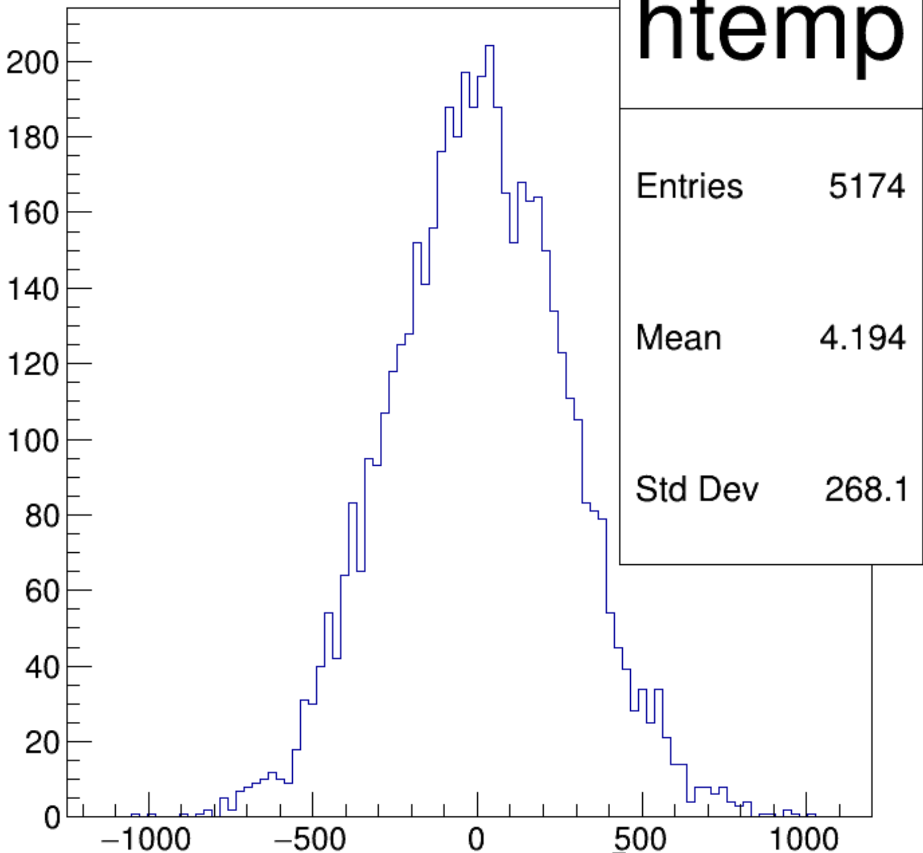
(asym_dsl/ppm-asym_dsr/ppm)/2 {ok_cut}
