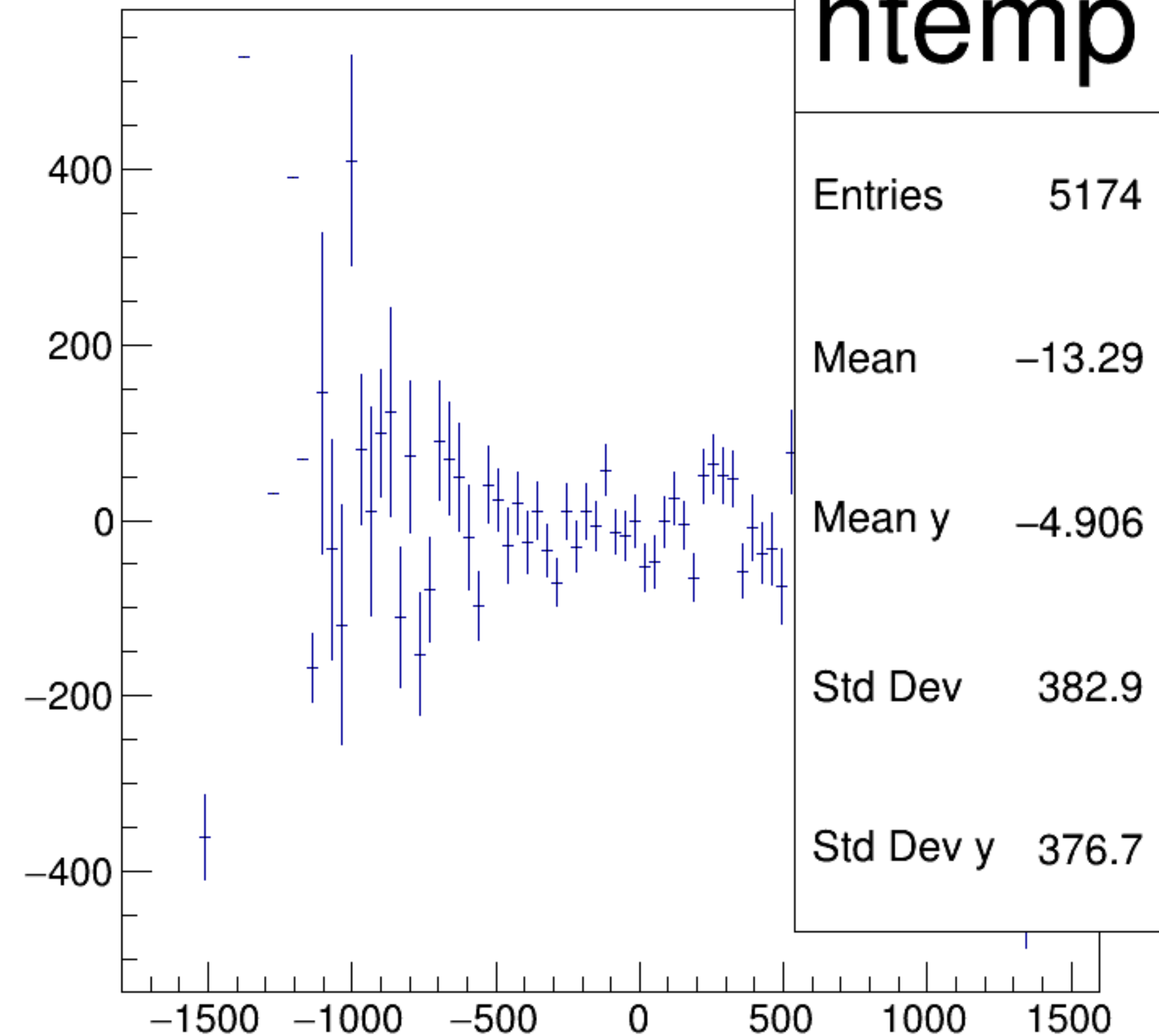
asym_dsl/ppm:asym_dsr/ppm {ok_cut}
