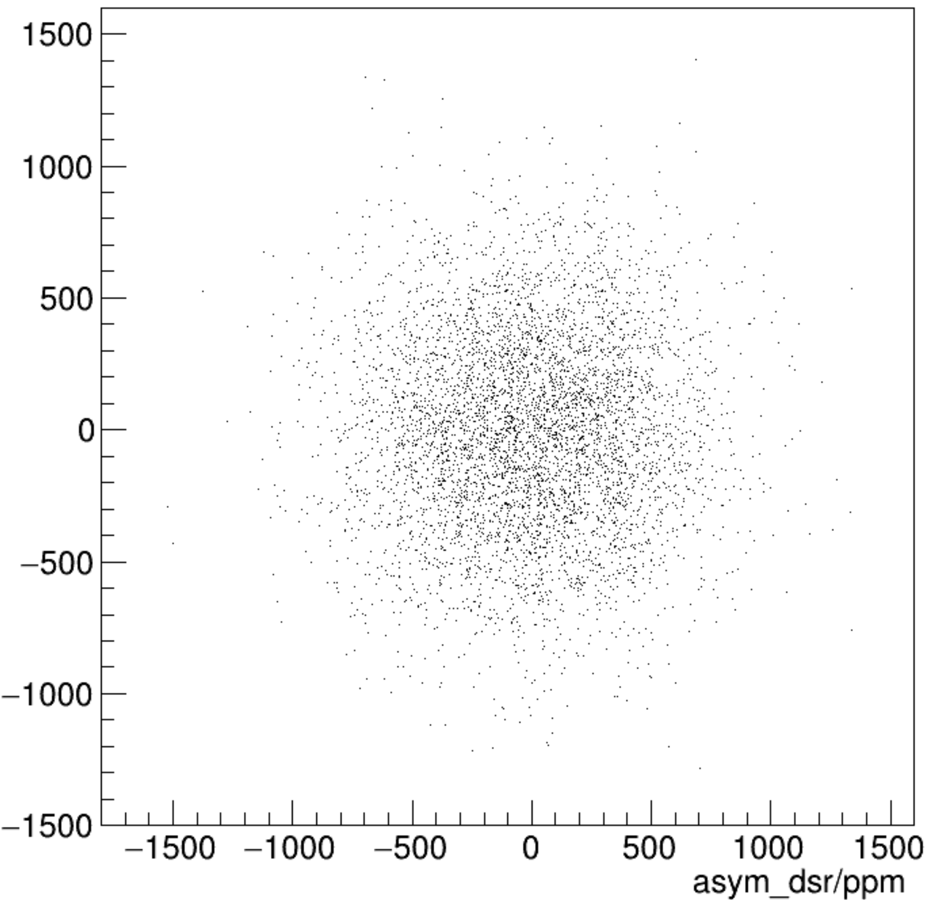
asym_dsl/ppm:asym_dsr/ppm {ok_cut}
