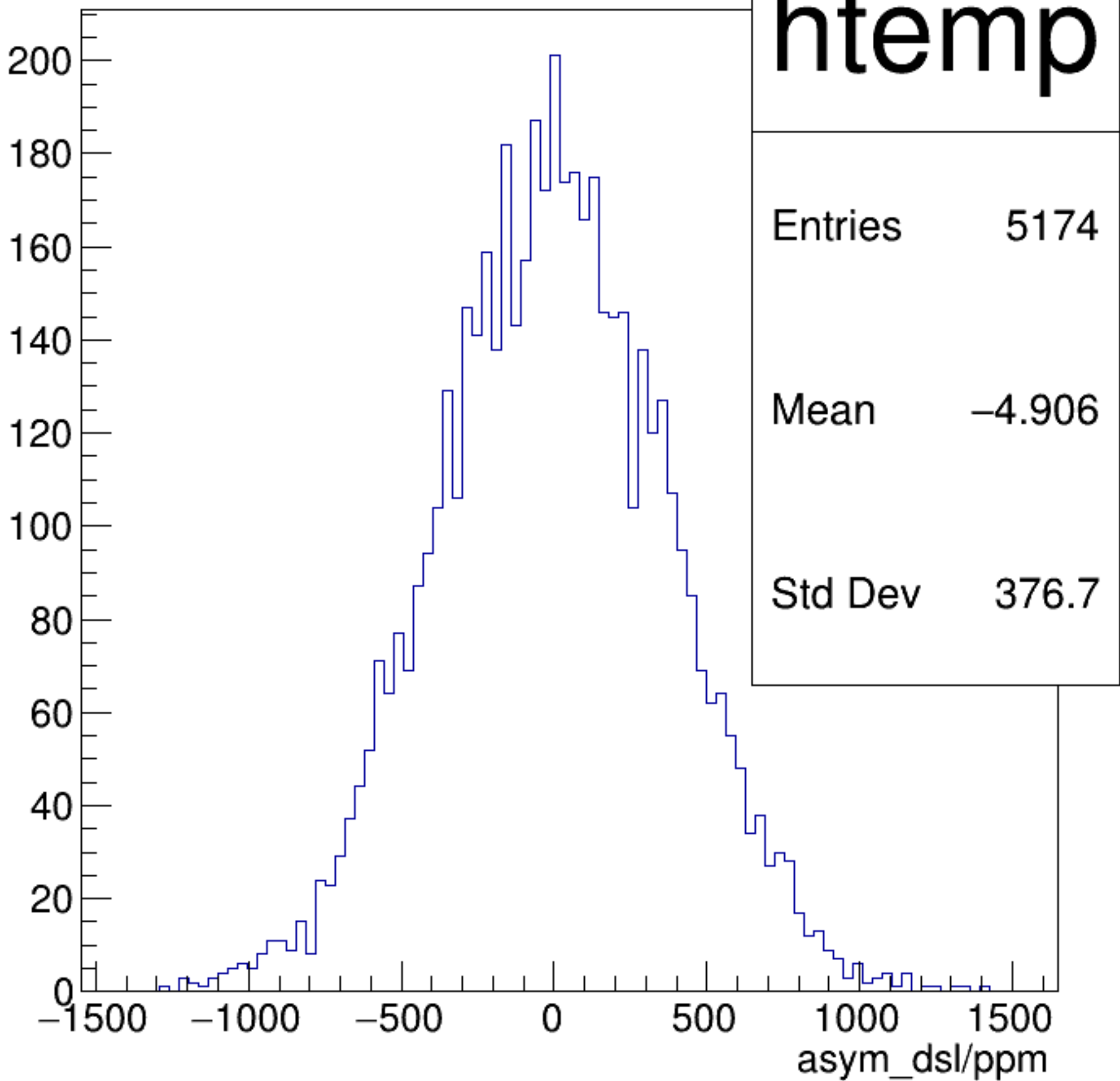
asym_dsl/ppm {ok_cut}
