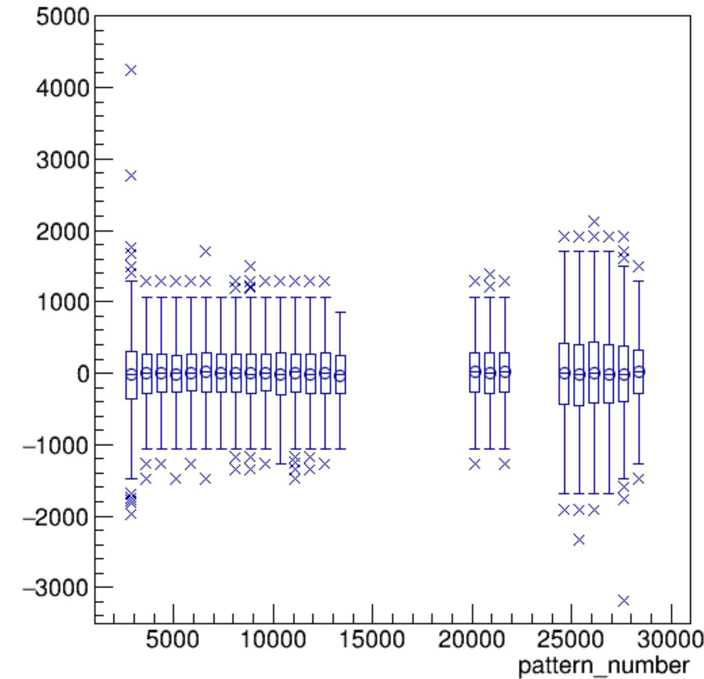
asym_sam7/ppm:pattern_number {ErrorFlag==0}
