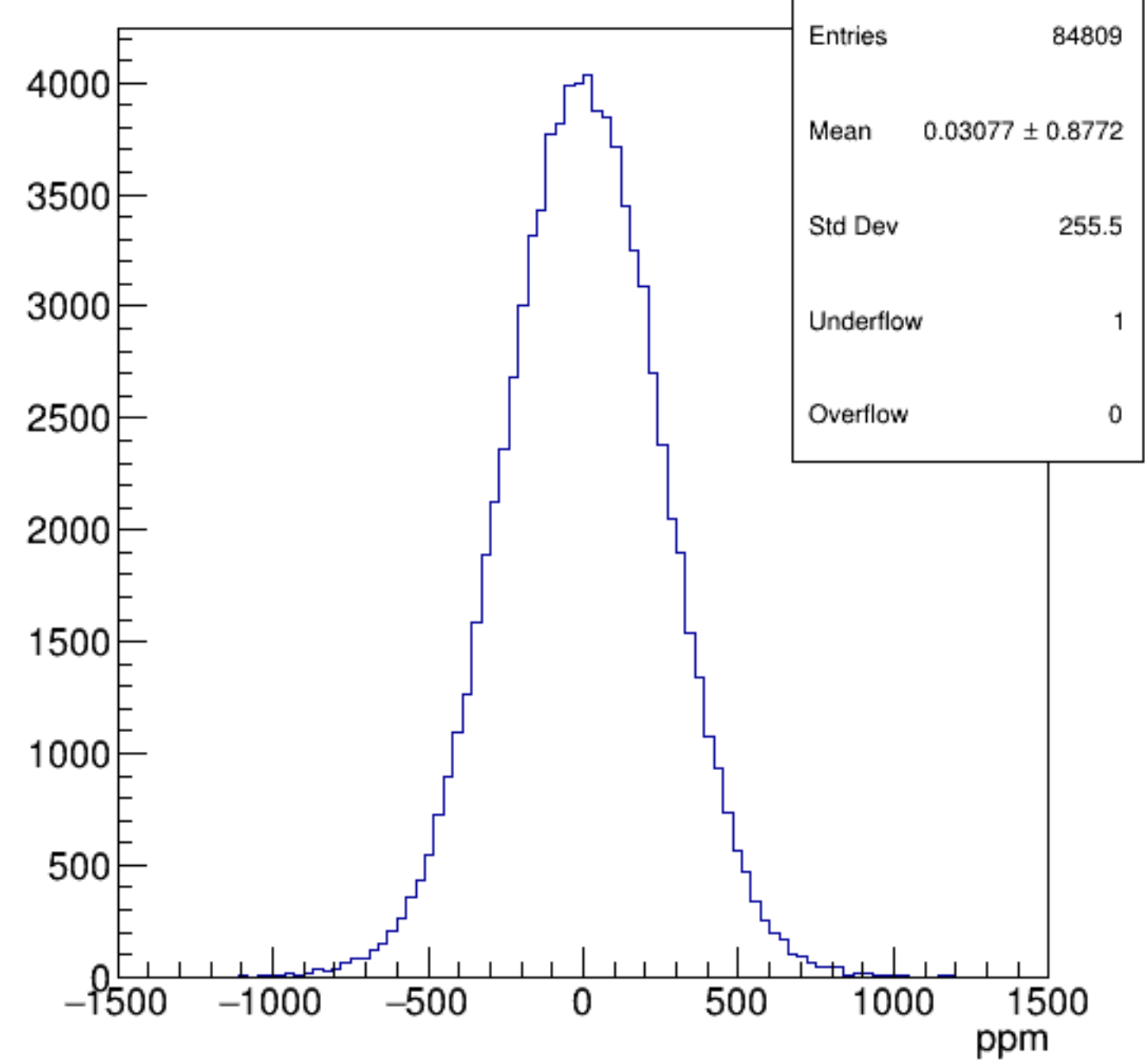
asym_bcm_dg_ds
