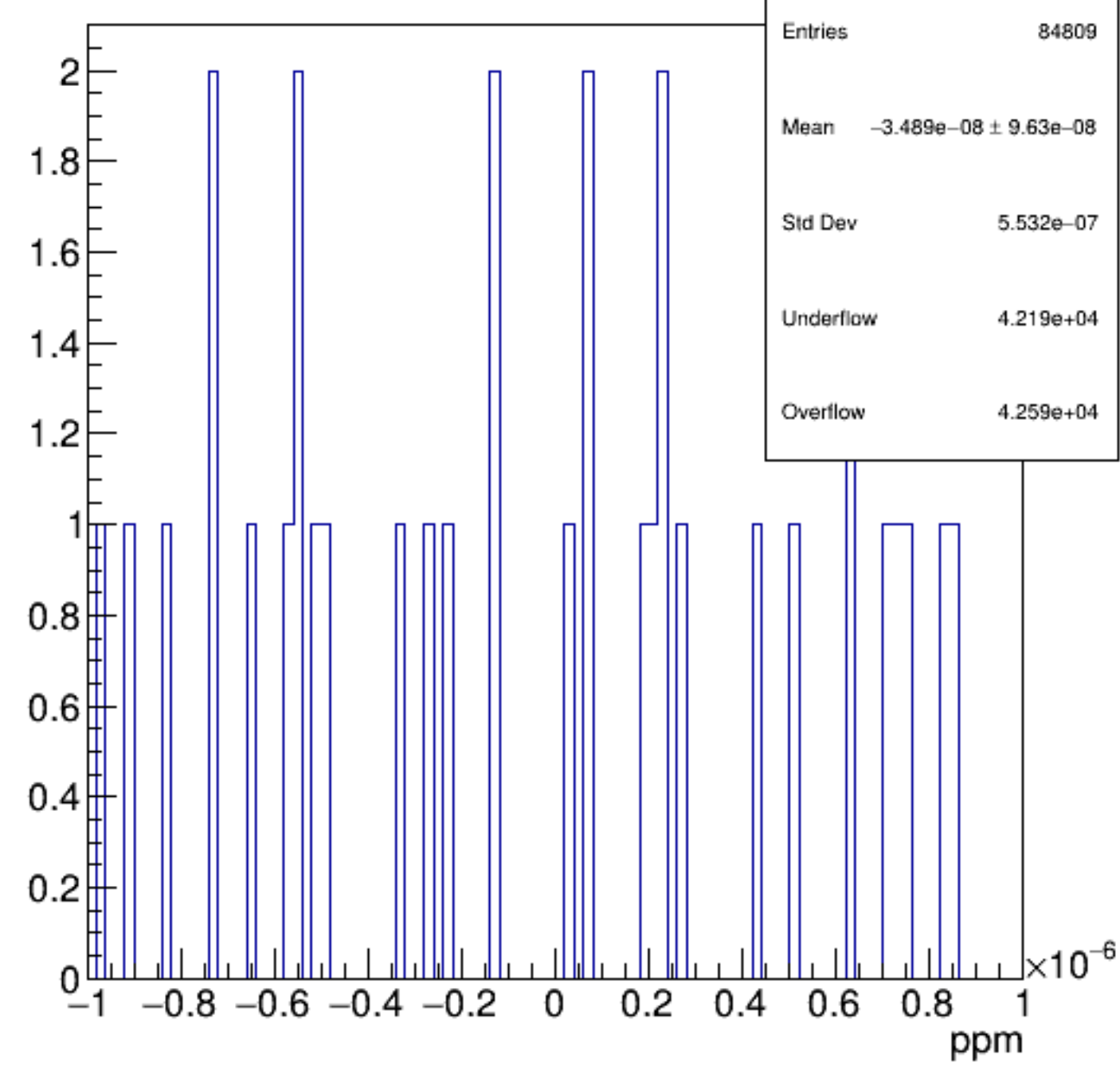
asym_bcm_an_diff
