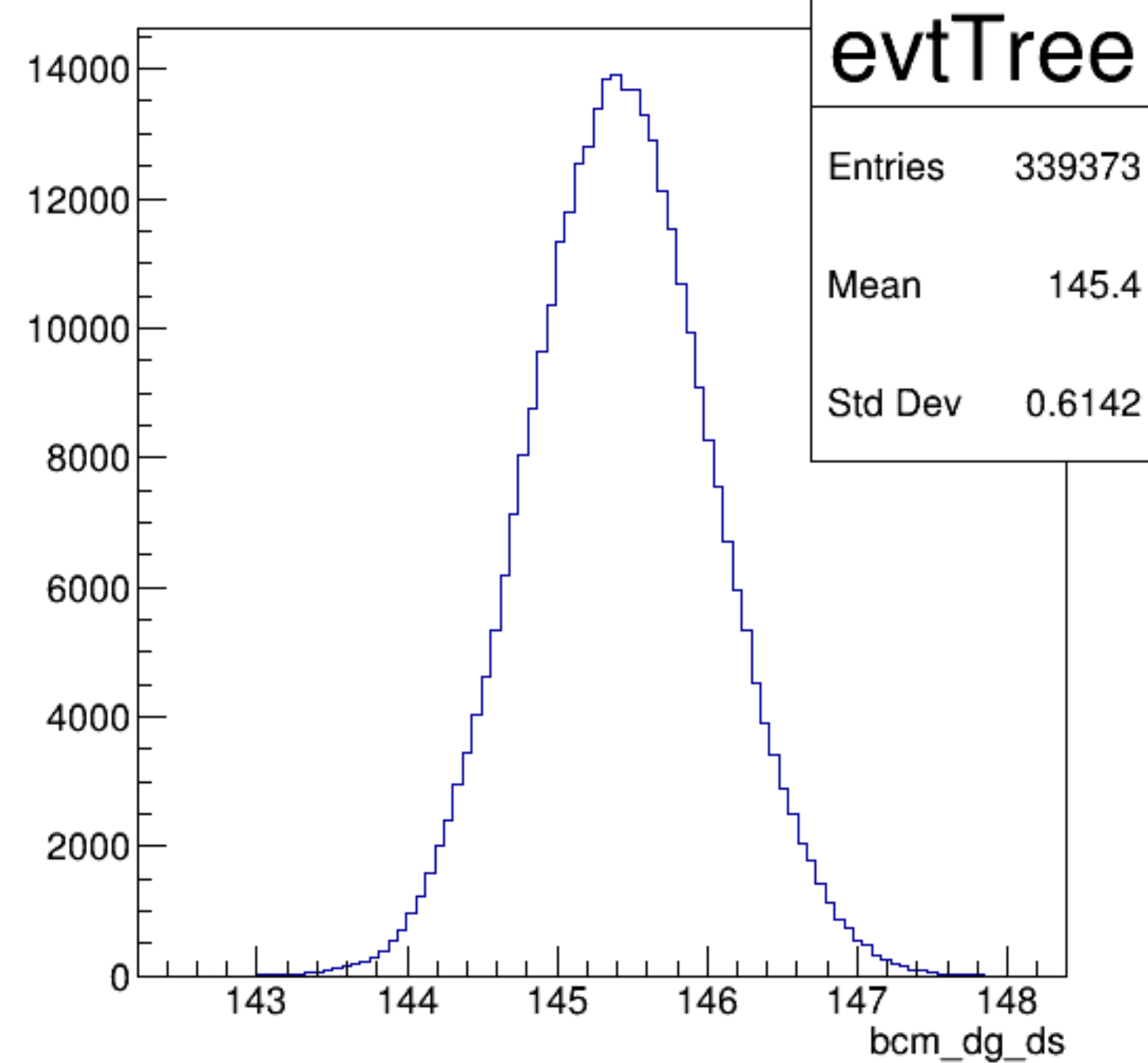
bcm_dg_ds {ErrorFlag==0}
