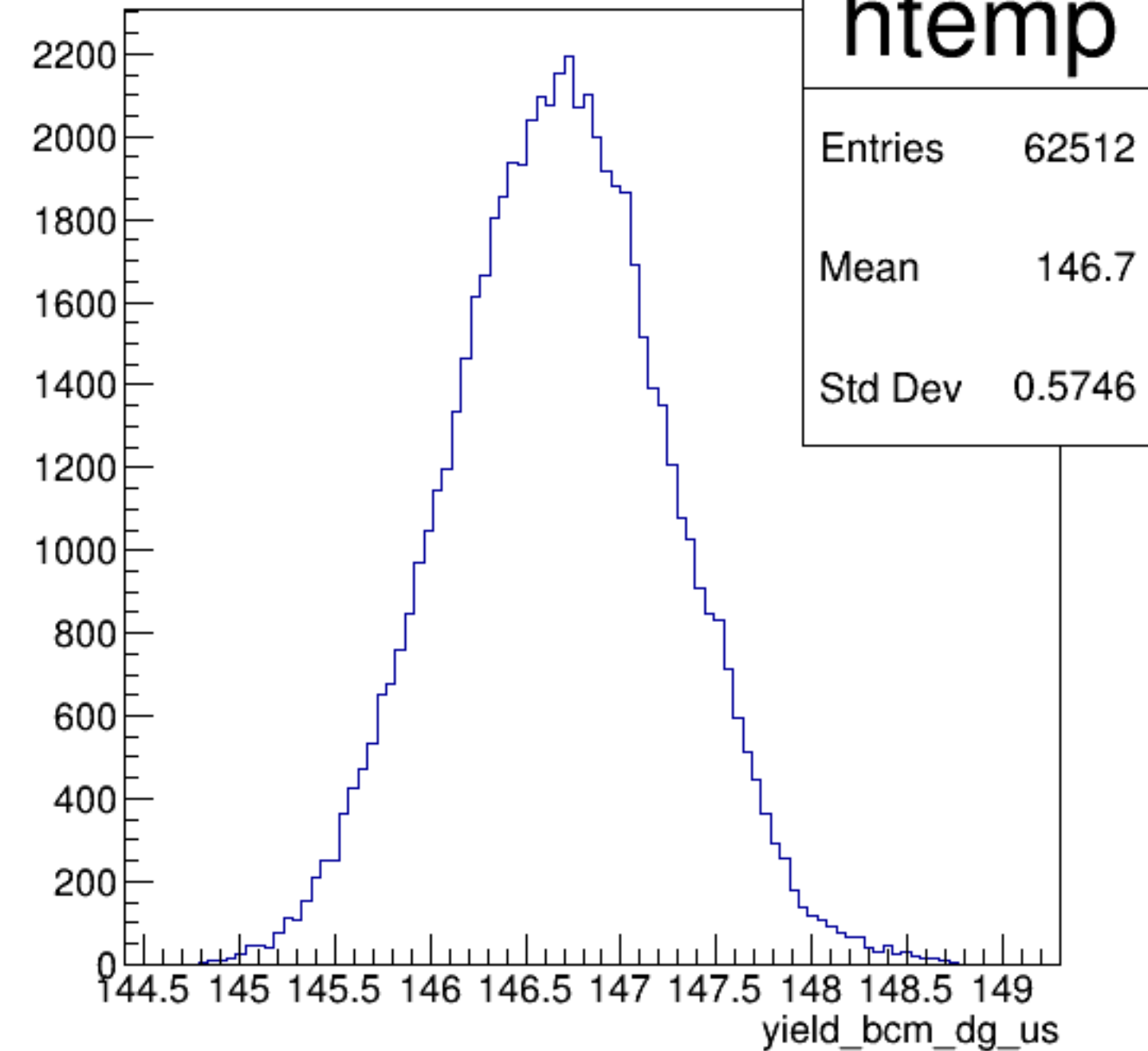
yield_bcm_dg_us {ErrorFlag==0}
