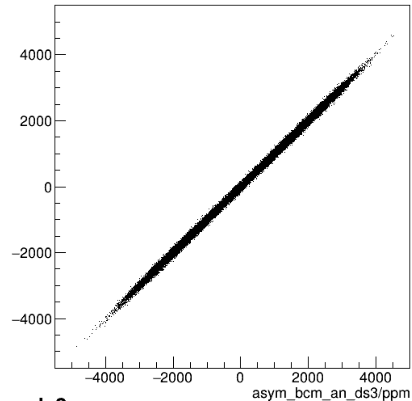
run7284_000_asym_bcm_dg_us_vs_asym_bcm_an_ds3_pr.png
