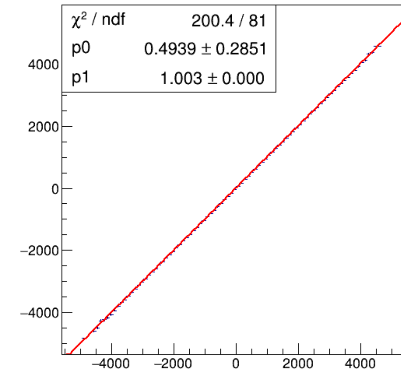
run7284_000_asym_bcm_dg_us_vs_asym_bcm_an_ds3_pr.png
