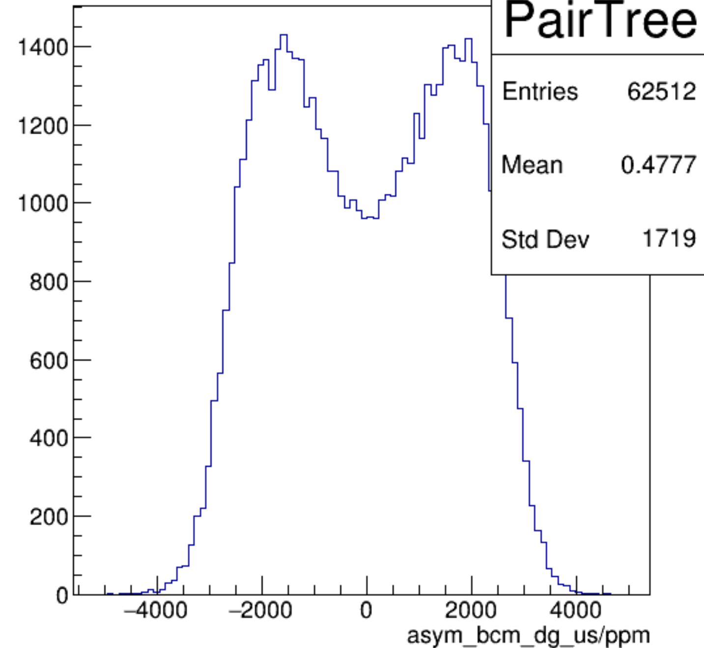
asym_bcm_dg_us/ppm {ErrorFlag==0}
