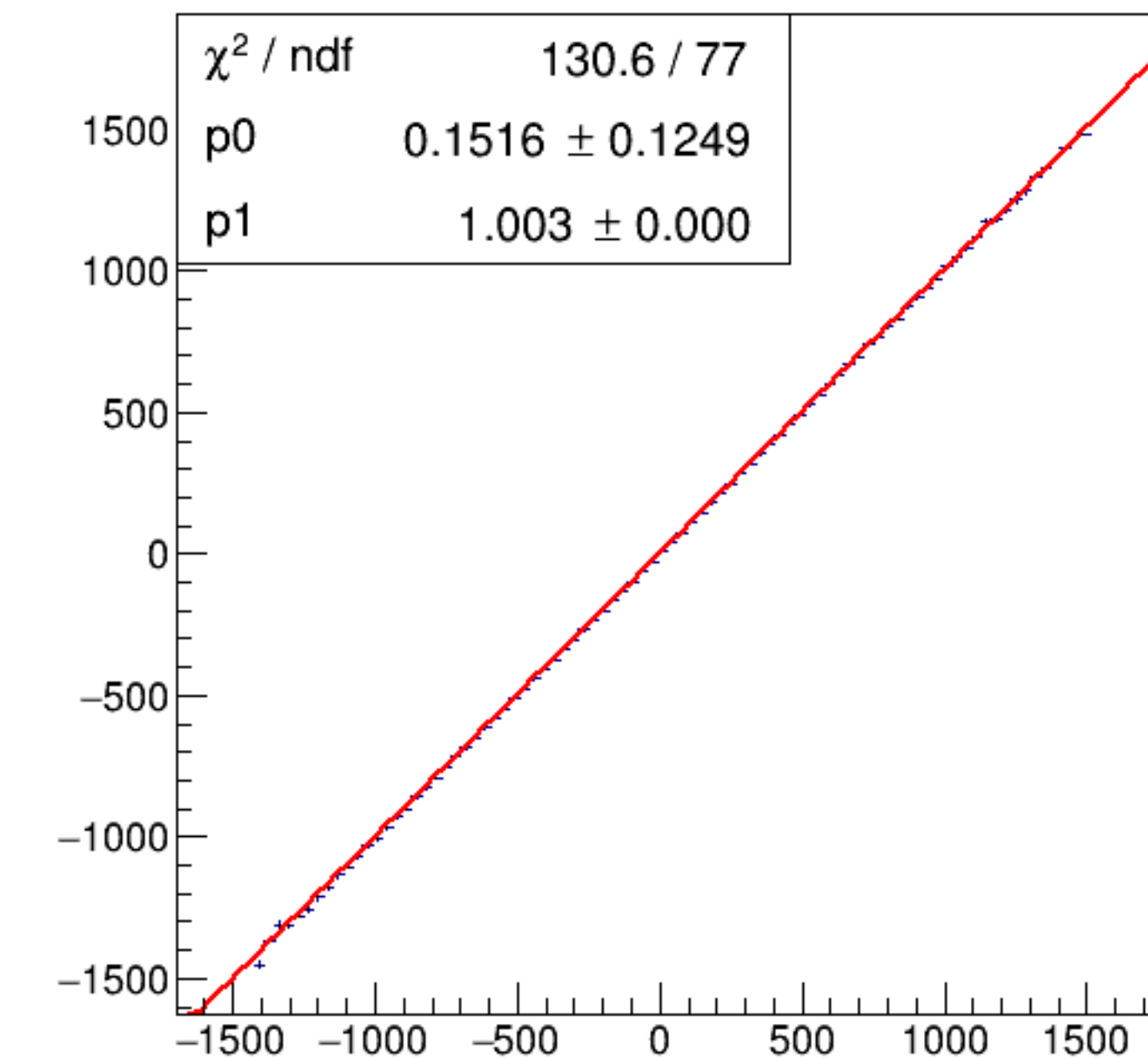
run7284_000_asym_bcm_an_us_vs_asym_bcm_an_ds_mul.png
