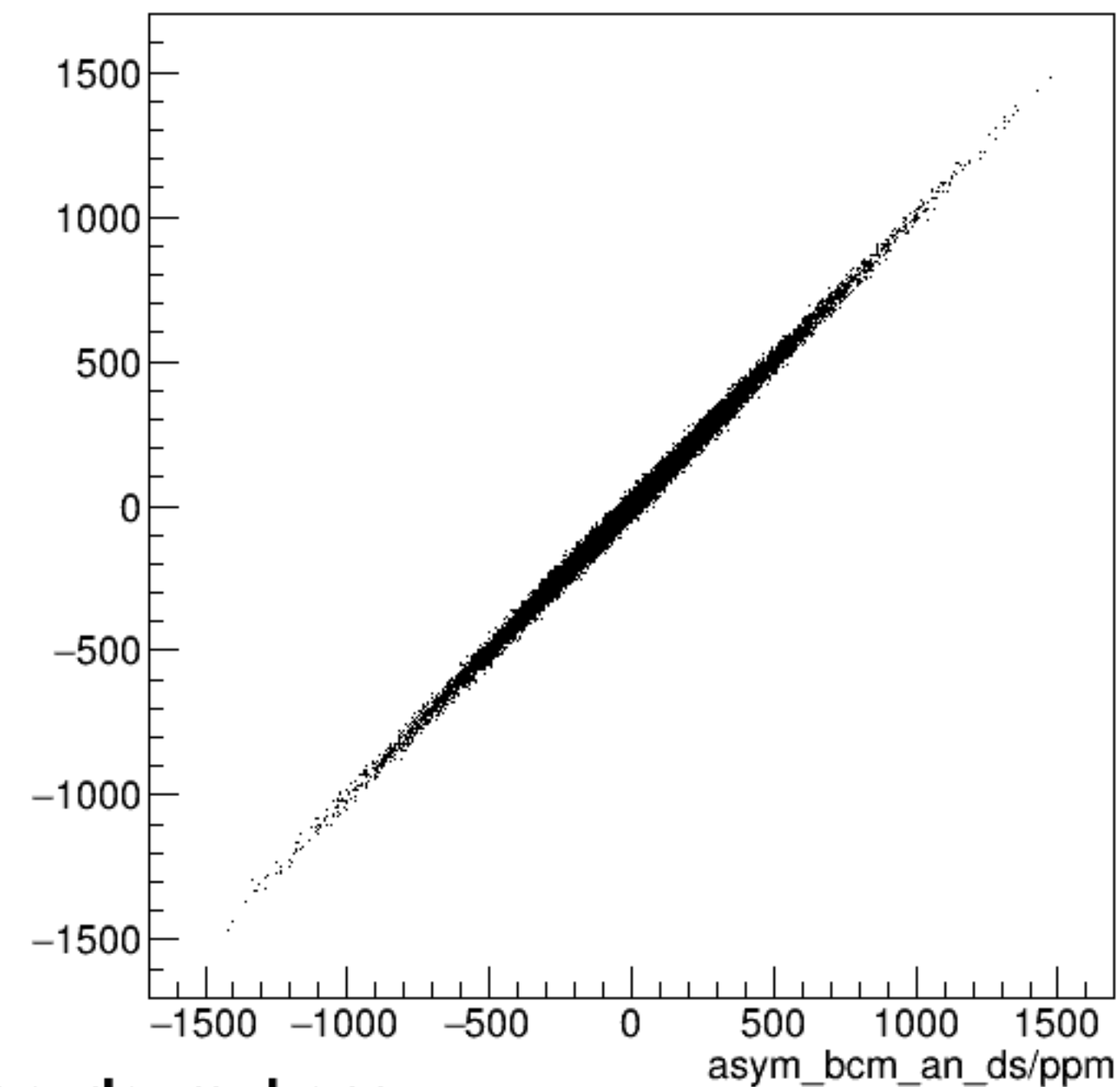
run7284_000_asym_bcm_an_us_vs_asym_bcm_an_ds_mul.png
