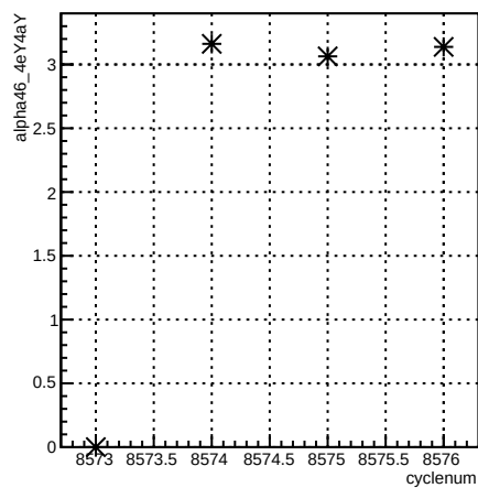
alpha46_4eY4aY:cyclenum {run == 7285}
