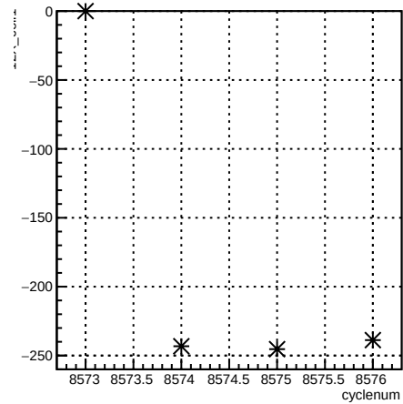
12X_coil1:cyclenum {run == 7285}
