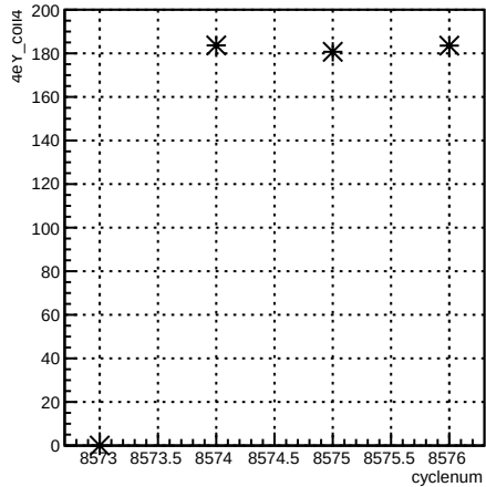
4eY_coil4:cyclenum {run == 7285}
