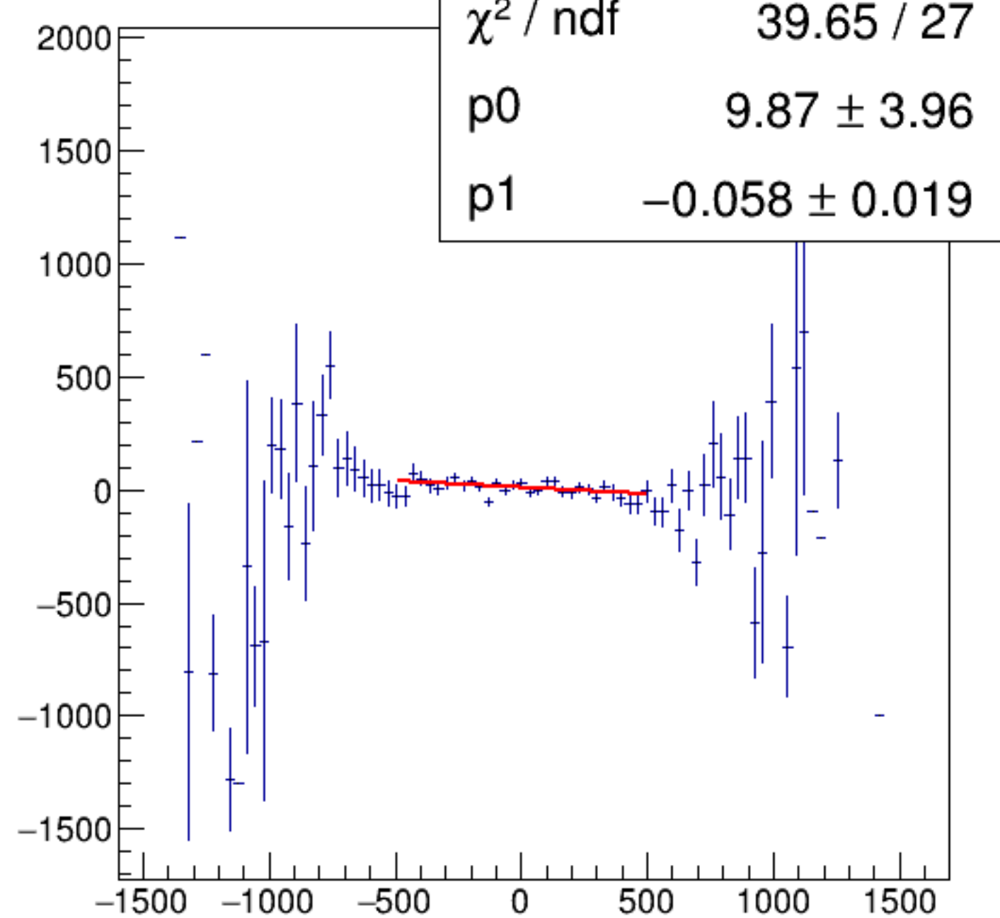
reg_asym_usl/ppm:AqDS/ppm {ok_cut}
