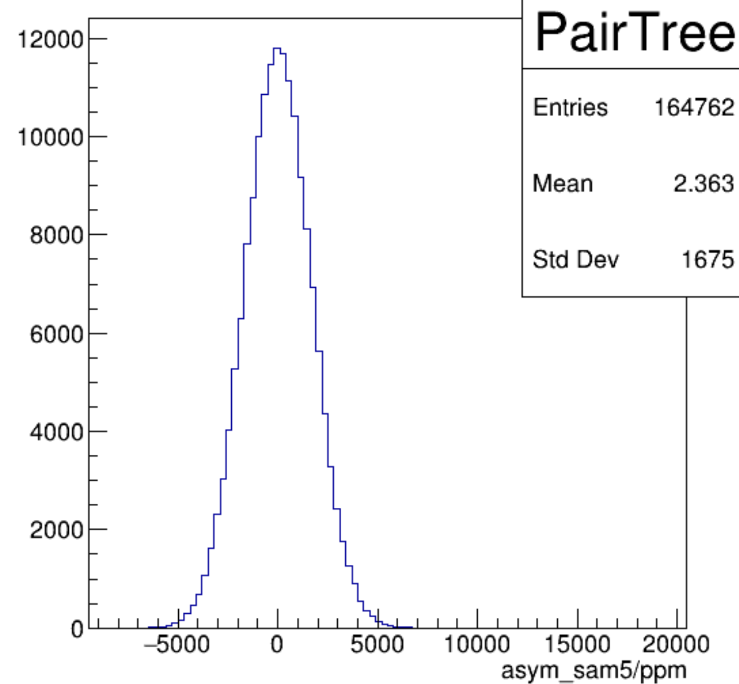
asym_sam5/ppm {ErrorFlag==0}
